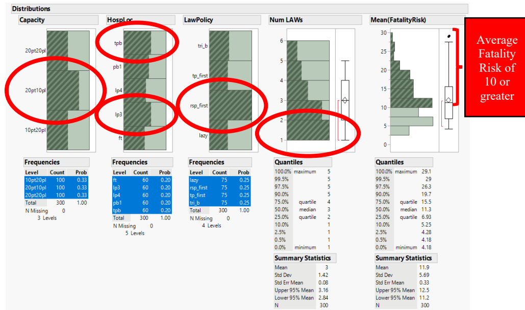
Figure 27. Linked histograms showing the factor settings that correspond to an average of 10 or more fatalities.
