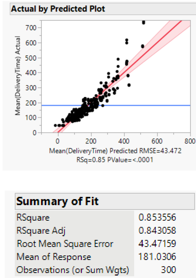
Figure 33. Actual by predicted plot and summary of fit for the regression on Mean(DeliveryTime).
