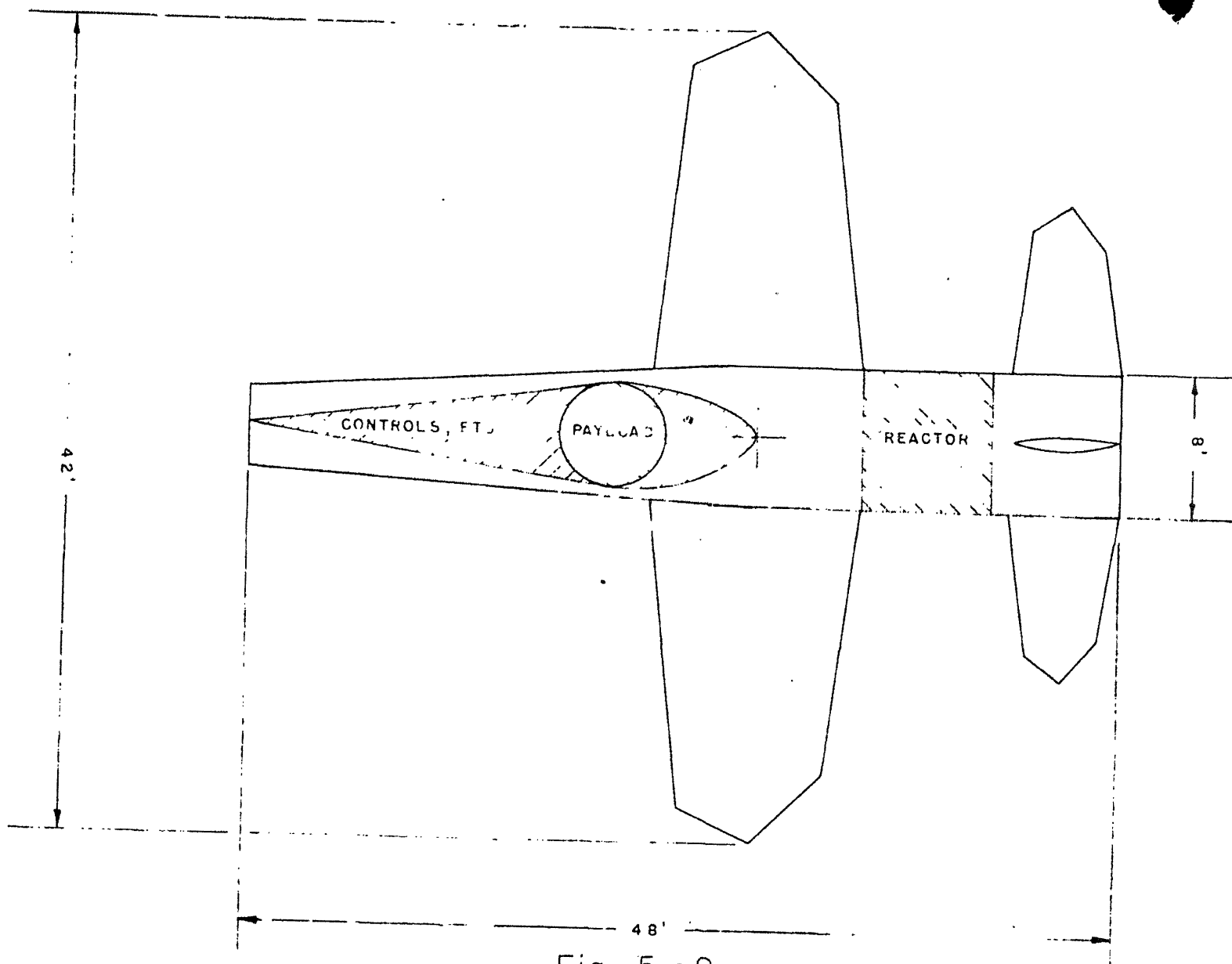
Fig 5-2 SCHEMATIC DIAGRAM NUCLEAR POWERED RAM JET
