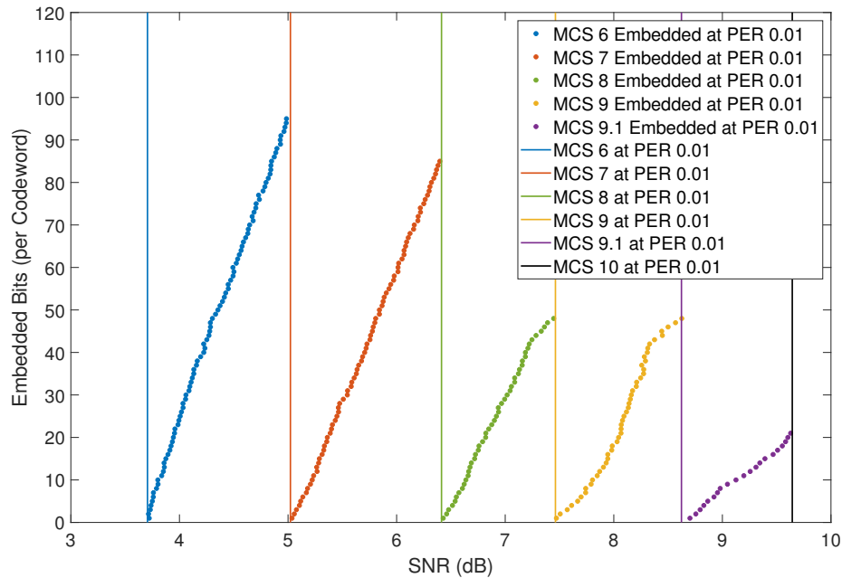
Figure 6.6. Embedded bits-per-codeword versus SNR for all 802.11ad \pi/2 -QPSK modulated MCS indices; embedding conducted in first n parity bits of each LDPC codeword
