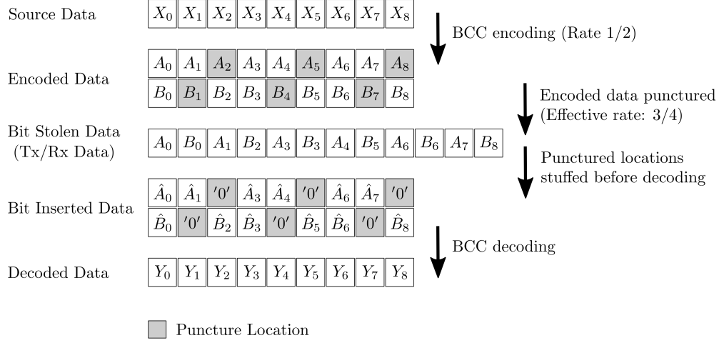
Figure 2.6. Puncturing process for convolutional codes. Adapted from [44].
