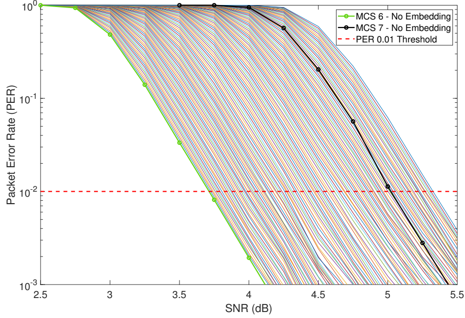
Figure 4.5. Variable rate embedding trials, DMG PHY simulation under AWGN channel. Results for MCS 6, 100000 trials per SNR, 1 to 120 embedded bits per LDPC codeword.
