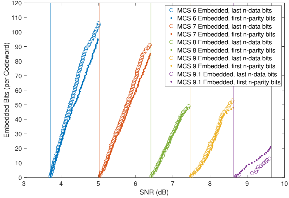
Figure 6.8. Comparison of embedding capacity for all 802.11ad \pi/2 -QPSK modulated MCS indices; embedding conducted in first n parity bits versus last n data bits of each LDPC codeword.
