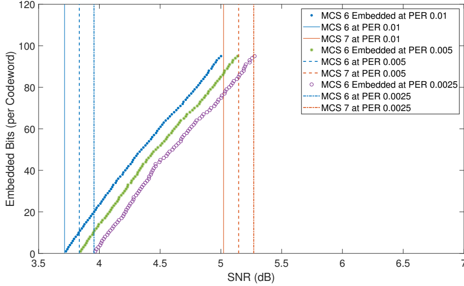
Figure 4.11. Comparison of embedding rates for DMG PHY simulation under AWGN channel at various packet error ratio thresholds. MCS 6, 100000 PSDU per SNR, 1 to 95 embedded bits per LDPC codeword.
