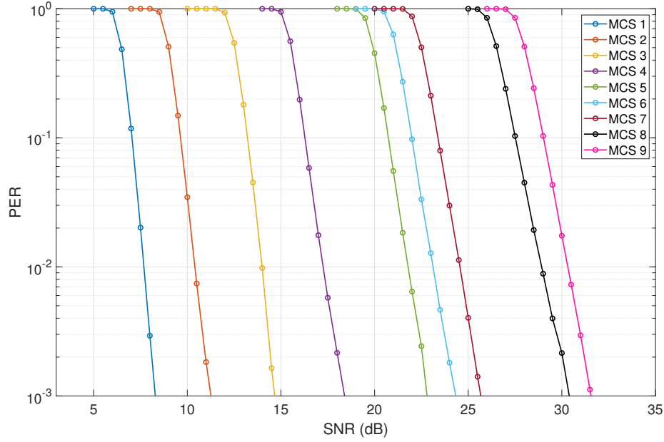
Figure 5.8. PER versus SNR performance curves for 8x8 MIMO IEEE 802.11ac VHT modulation and coding schemes with BW of 80 MHz; performance average of 10000 trials over AWGN channel with single 4096-octet A-MPDU.
