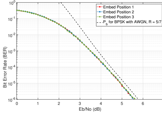
Figure 5.6. Evaluation of embedding location for punctured convolutional codes; BPSK modulation, 100 trials over AWGN: (a) R_{equiv} = 10/14 embedding on base R = 2/3 code and (b) R_{equiv} = 12/15 embedding on base R = 3/4 code.
