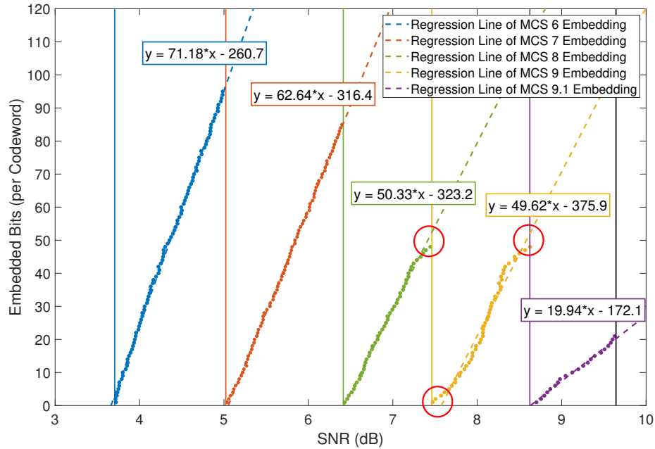
Figure 6.7. Regression lines of embedded bits per codeword versus SNR for all 802.11ad QPSK modulated MCS
