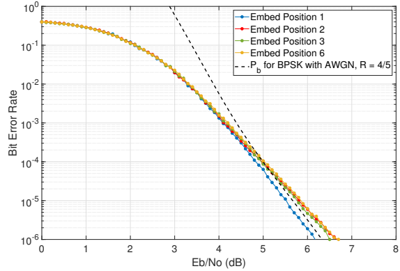
Figure 5.6. Evaluation of embedding location for punctured convolutional codes; BPSK modulation, 100 trials over AWGN: (a) R_{equiv} = 10/14 embedding on base R = 2/3 code and (b) R_{equiv} = 12/15 embedding on base R = 3/4 code.
