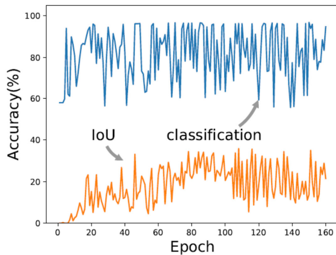
(b) The weights of the softmax and mse: 1e-2 and 1e-3, respectively.
