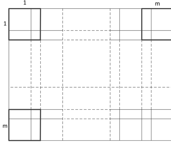
Figure 77: Generalized model size of m \times m
