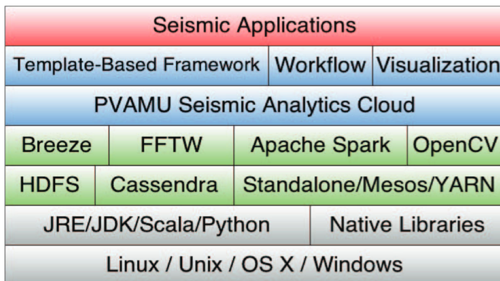
Figure 36: The Software Stack of Seismic Analytics Cloud Platform
