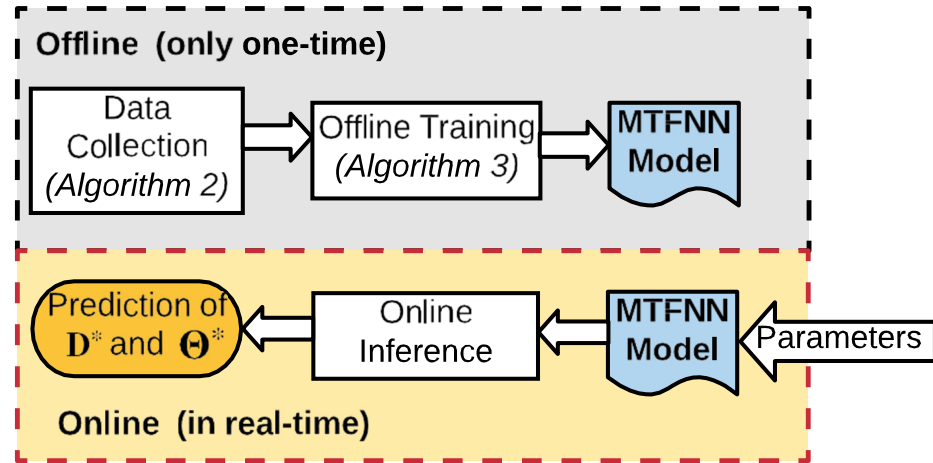
Figure 16: Brief overview of the proposed MTFNN framework
