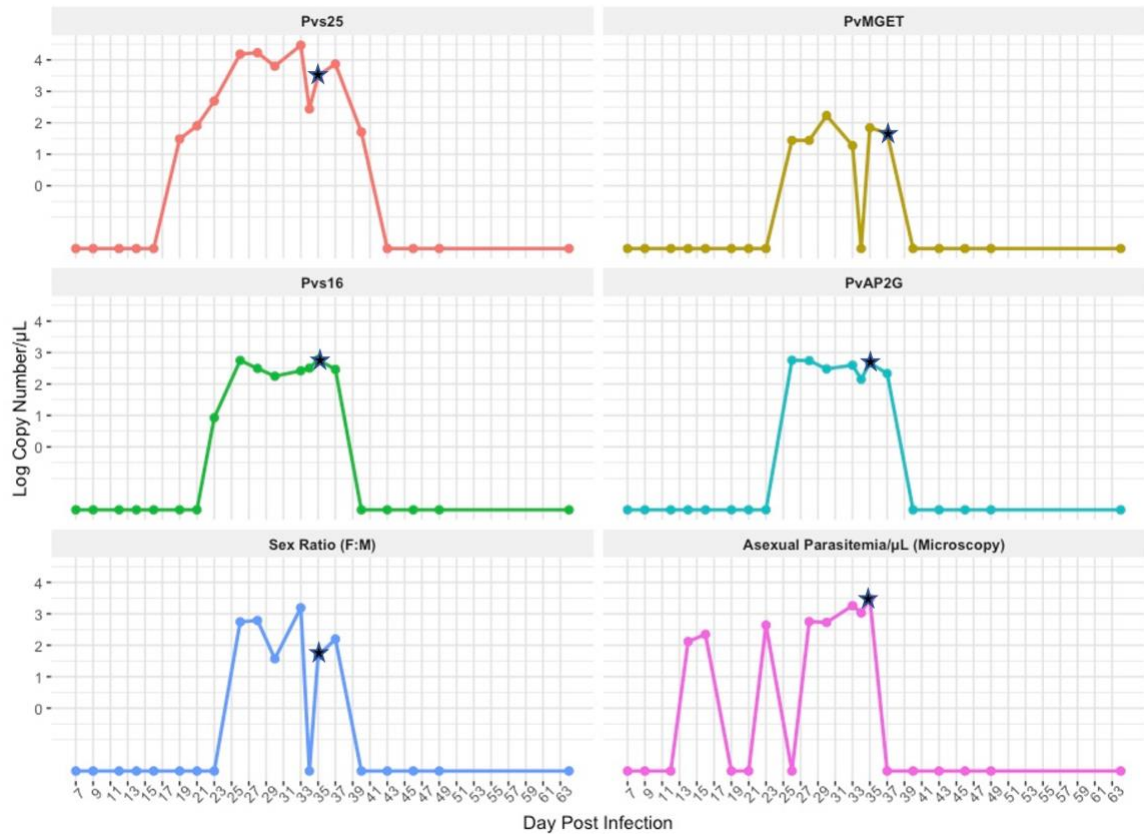
Figure 25. Log Copy Numbers/μL of Each Gametocyte-Specific Transcript Marker on Respective Days Post Infection in Monkey B. The star marks the day that the monkey was treated with MQ.
