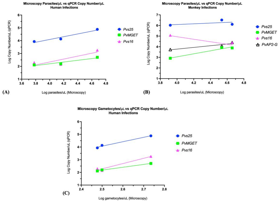
Figure 23. Correlation Between Microcopy Log Parasites or Gametocytes/ \mu\text{L} and qPCR Log Gametocyte-Specific Transcripts Copy Numbers/ \mu\text{L} in Monkey and Human Infections.
