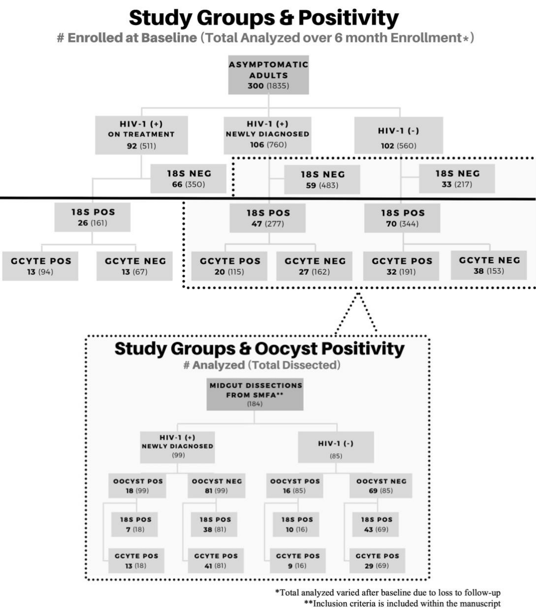
Figure 6. Study Profile Overview Participant enrollment by study group and corresponding molecular data for asexual and sexual parasite biomarkers. Groups below the solid black line were included in this study for gametocyte analysis. A subset of volunteers was enrolled in a transmission study using the Standard Membrane Feed Assay (dotted line). Positive samples are abbreviated as (+) or POS. Negative samples are abbreviated as (-) or NEG. Full details of the study design and complete analyses of asexual stage biomarker data
