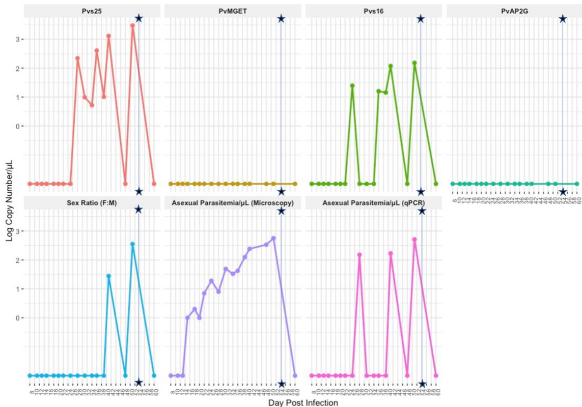
Figure 26. Log Copy Numbers/ \mu L of Each Gametocyte-Specific Transcript Marker on Respective Days Post Infection in Monkey E. The star and line mark the day that the monkey was treated with MQ.
