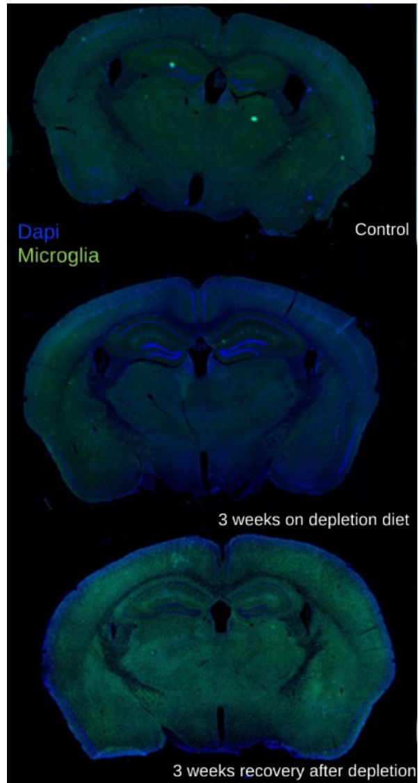
Figure 3. Microglia Depletion.
