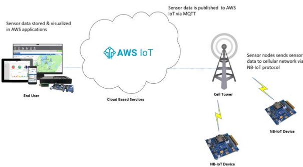
Figure 3: NB-IoT Network
