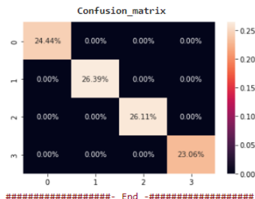
Figure 12. Extra trees classifier
