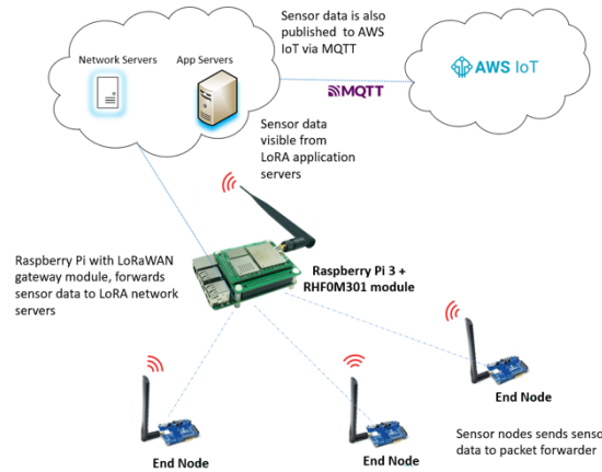
Figure 4: LoRaWAN Network
