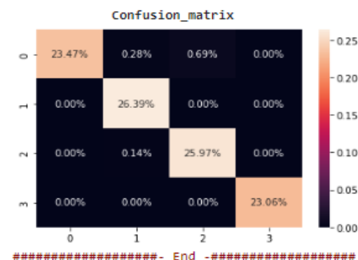
Figure 13. SGD classifier
