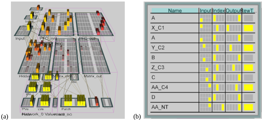
Figure 1. (a) A PBWM network used to learn scene categories. (b) Input to the network representing the contents of each sector (“Input” column) and its location (“Index” column); other columns are described in the text. Here scene classes 1 through 4 are depicted followed by a non-target scene.
