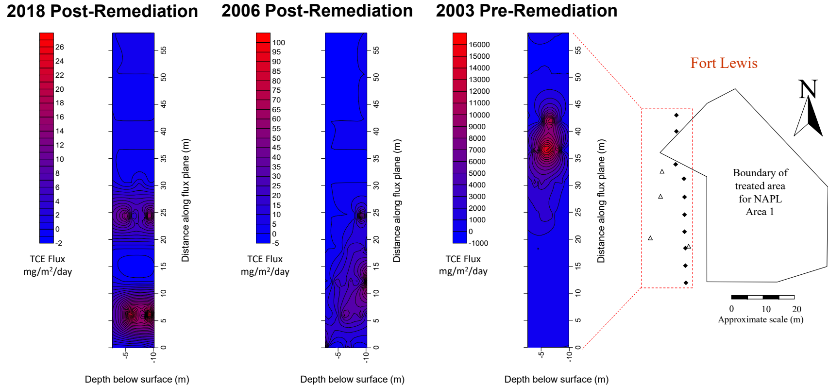
Figure 20. NAPL Area 1 Comparison of Pre-remediation (2003) and Post remediation (2006 and 2018) TCE Mass Flux Distributions.
