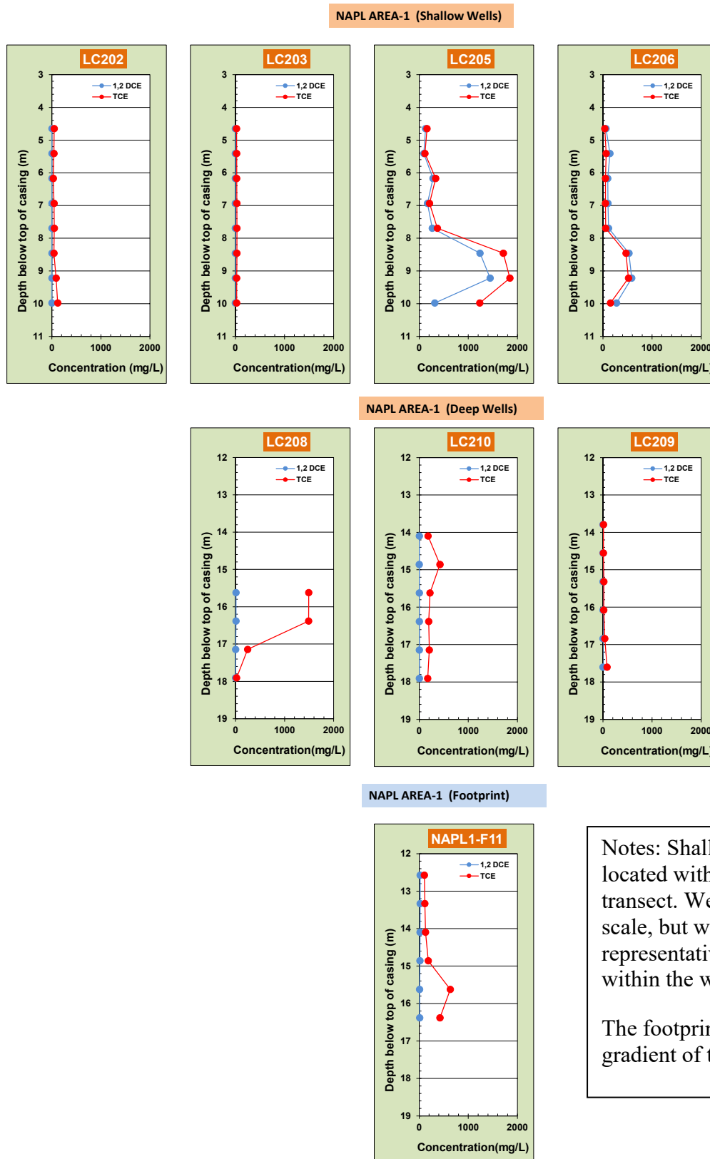
Figure 11. NAPL Area 1 BMLS (2017) Aqueous Contaminant Concentrations.
