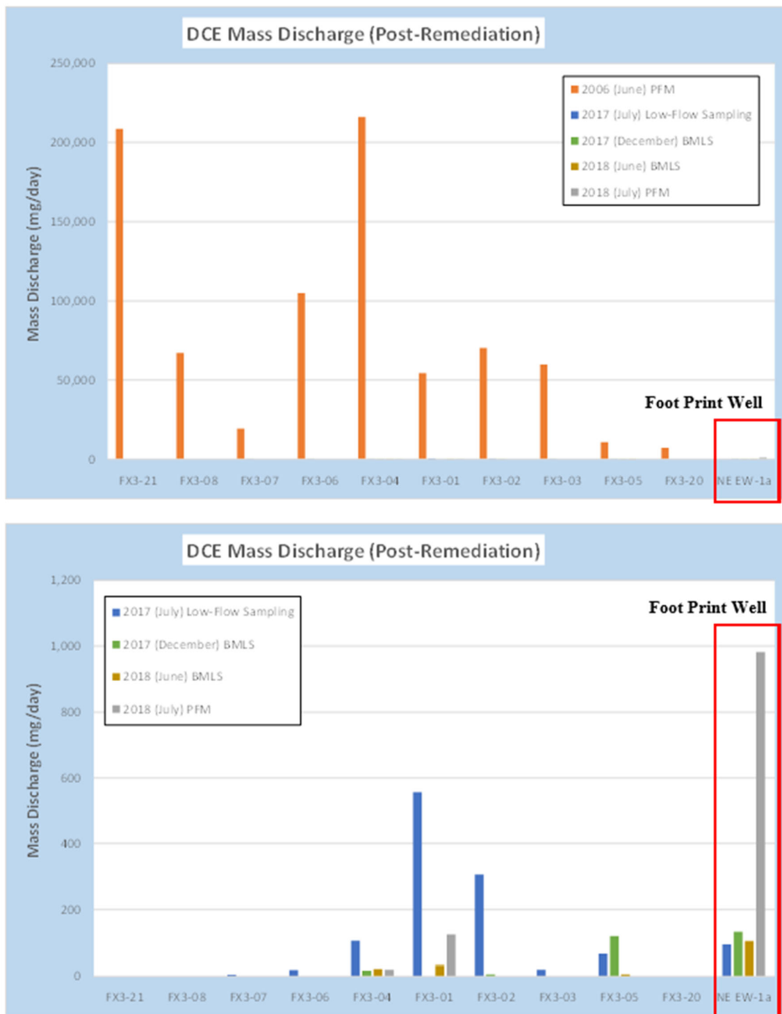
Figure 63. Estimated DCE Mass Discharge for NAPL Area 3 Flux Transect and Foot Print Well.
