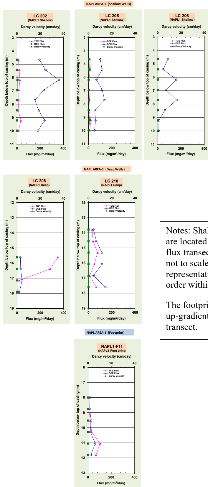
Figure 16. NAPL Area 1 PFM (2018) Fluxes.
