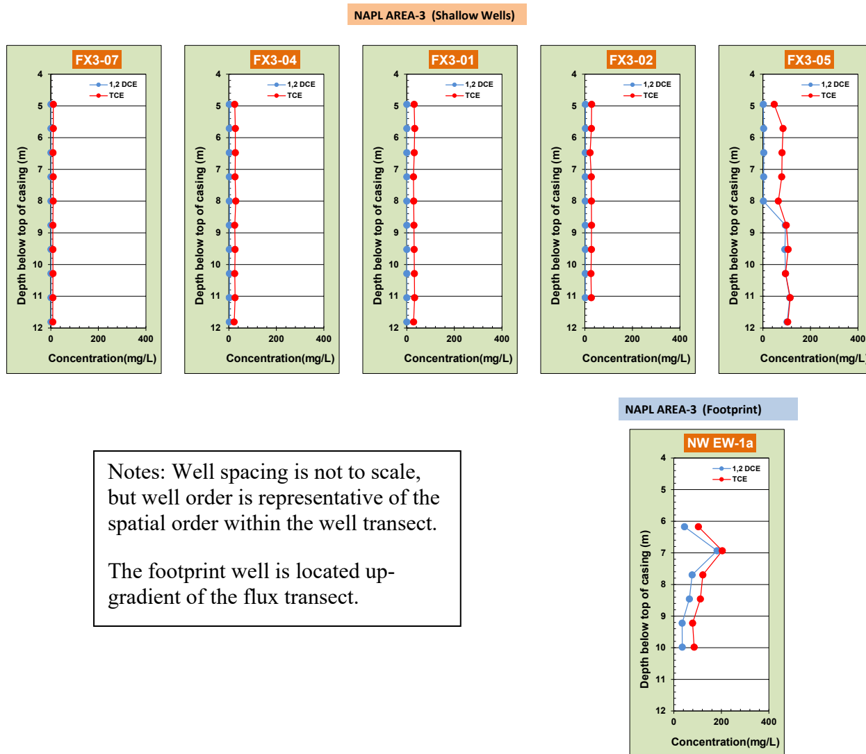
Figure 13. NAPL Area 3 BMLS (2017) Aqueous Contaminant Concentrations.
