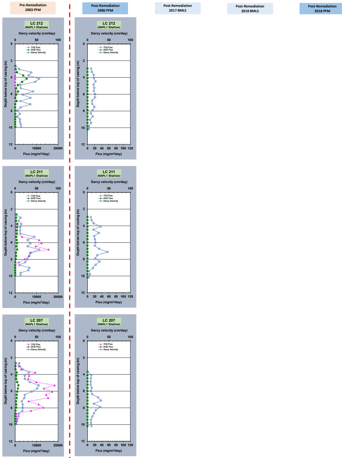
Figure 18. Comparison of Pre- and Post-remedial Fluxes Within the NAPL Area 1 Shallow Well Flux Transect (Right Portion of the Transect When Looking Down-gradient Through the Transect).
