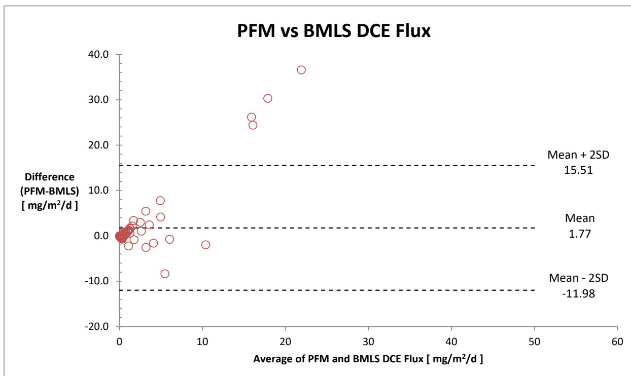
Figure 68. Summary of Statistical Analysis for DCE Flux from PFM and BMLS.
