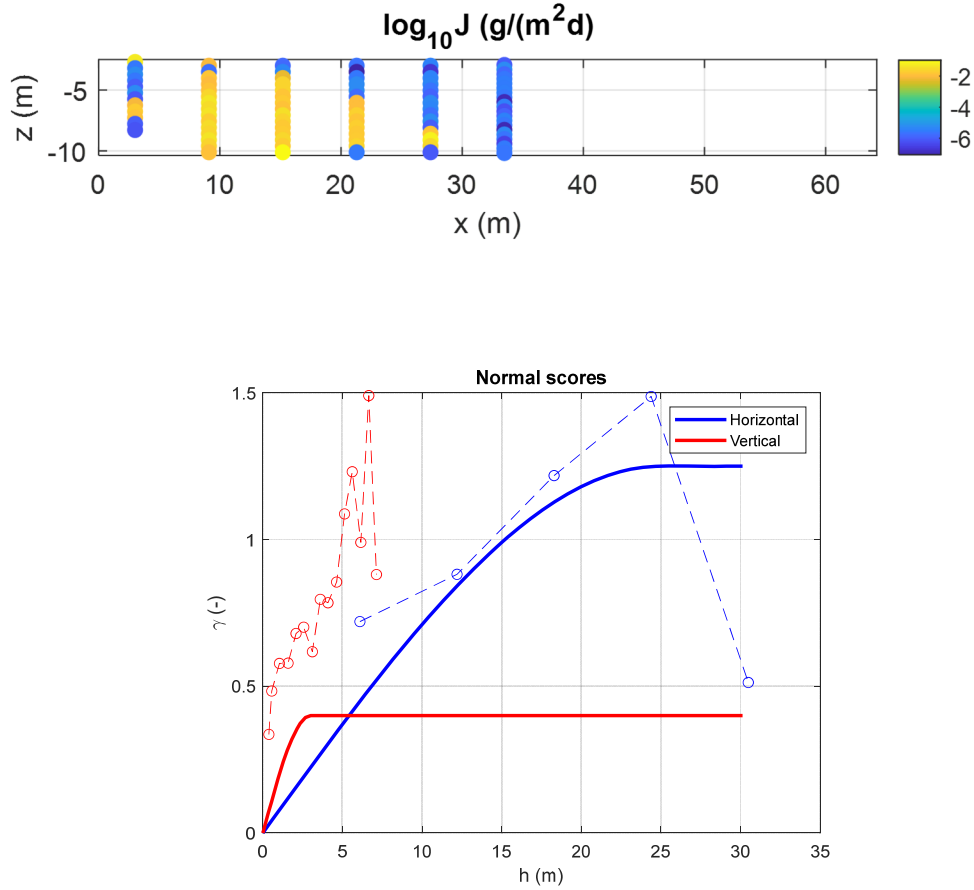
Figure 24. 2006 TCE Log-flux Measurements and Normal Score Variograms.
