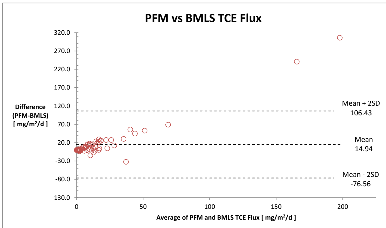
Figure 66. Summary of Statistical Analysis for TCE Flux from PFM and BMLS.
