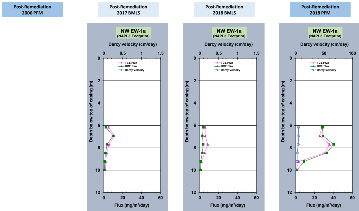
Figure 61. Post-remedial Fluxes within the NAPL Area 3 Foot Print Well NW EW-1.
