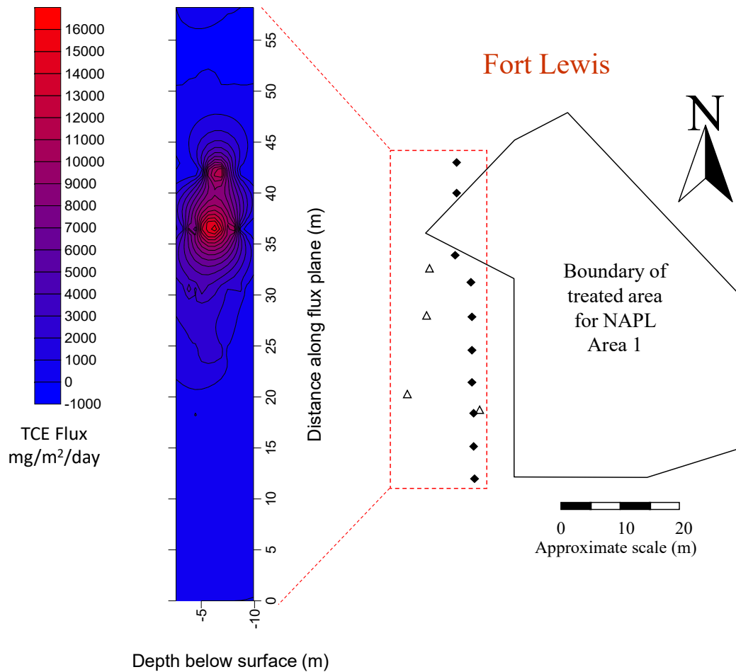
Figure 4. APL Area 1 Comparison of Historical Pre-remediation (2003) and Post Remediation (2006) TCE Mass Flux Distribution.
