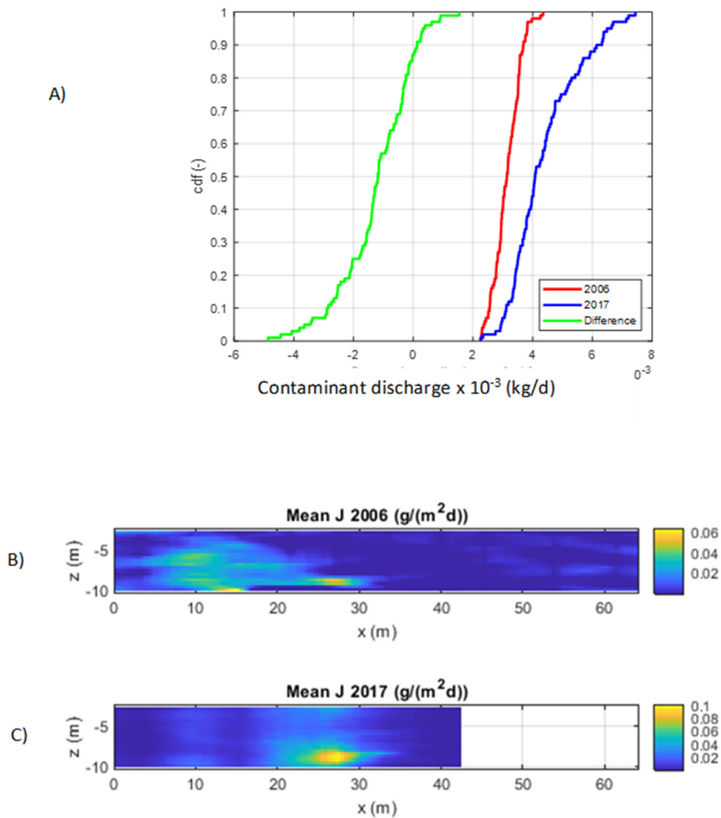
Figure 41. Simulated TCE Fluxes and CDFs of Simulated TCE Discharges and discharge Difference Between 2006 (PFM) and 2017 (BMLS).
