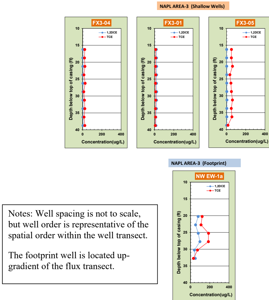
Figure 15. NAPL Area 3 BMLS (2018) Aqueous Contaminant Concentrations.
