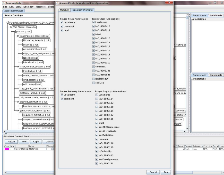
Fig. 1: Profiling interface added to AgreementMaker.
