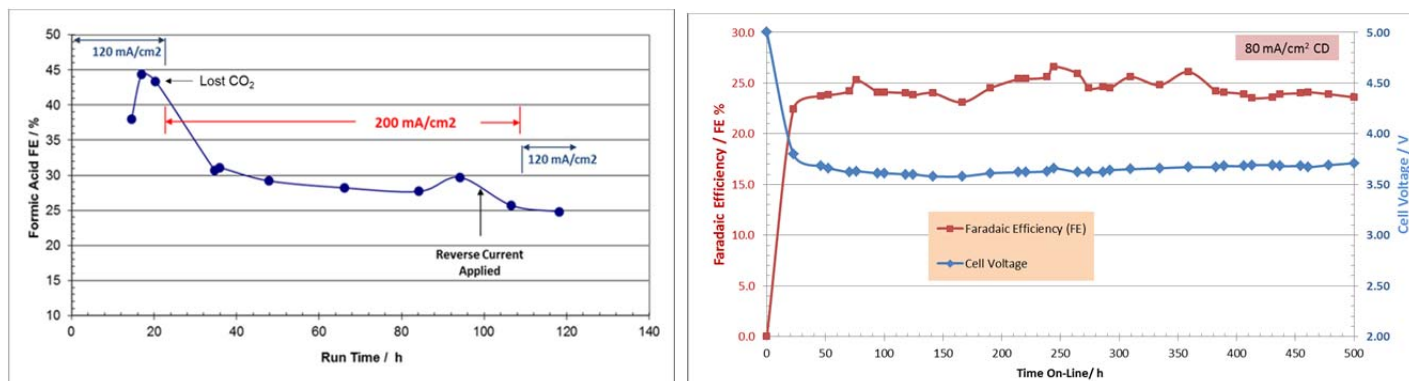
Figure 1. Performance of the two 250 cm 2 formic acid electrolyzer runs.
