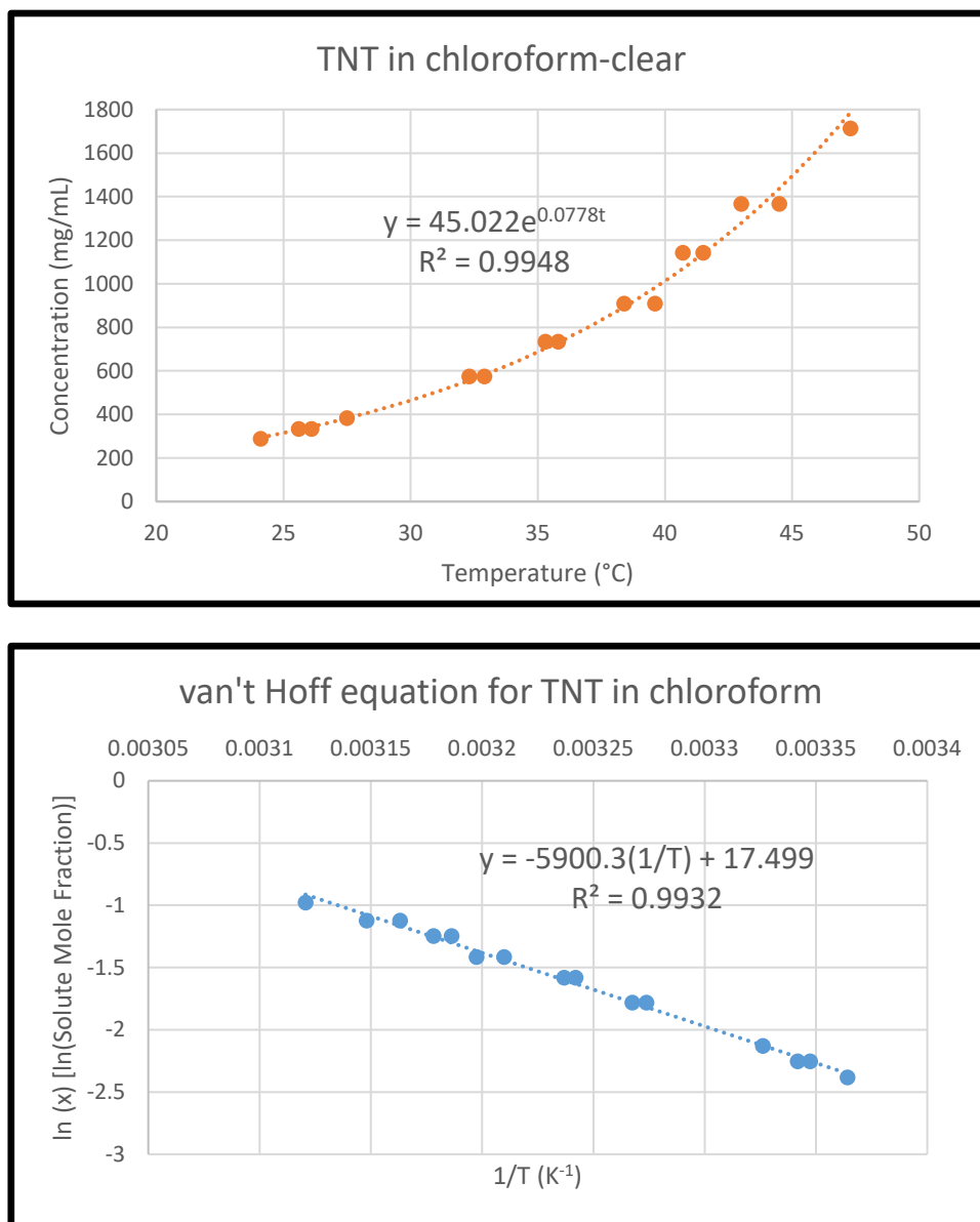
Figure 6 TNT solubility curves in chloroform
