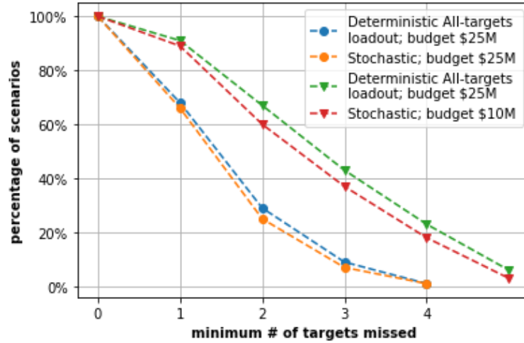
Figure 3. TASOM-1: Exceedance functions for misses for deterministic, fixed loadouts from all-targets scenario and stochastic loadouts, for $25M and $10M budgets
