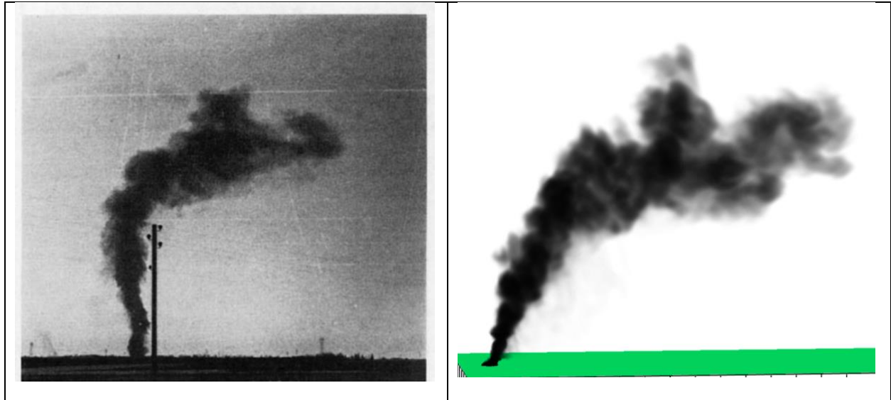
Figure 30. Left: a photograph of the April 1973 Meteotron plume (Benech 1976). Right: an FDS simulation of the experiment. Both images show the plume 300 s after ignition.
