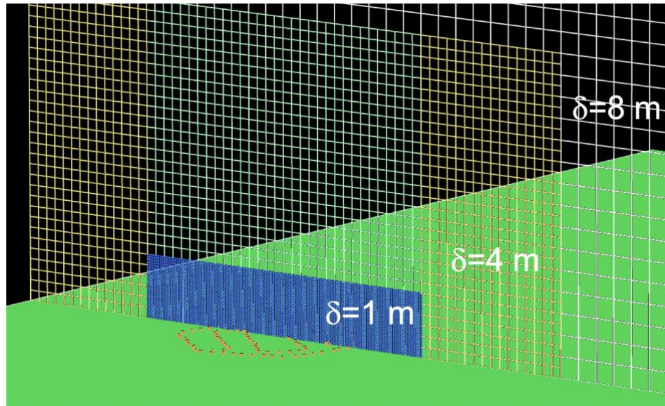
Figure 28. Vertical cross section of computational meshes used in the Meteotron simulations. The burner array is shown at the bottom of the finest mesh (blue grid). Mesh cell sizes are indicated in the image.
