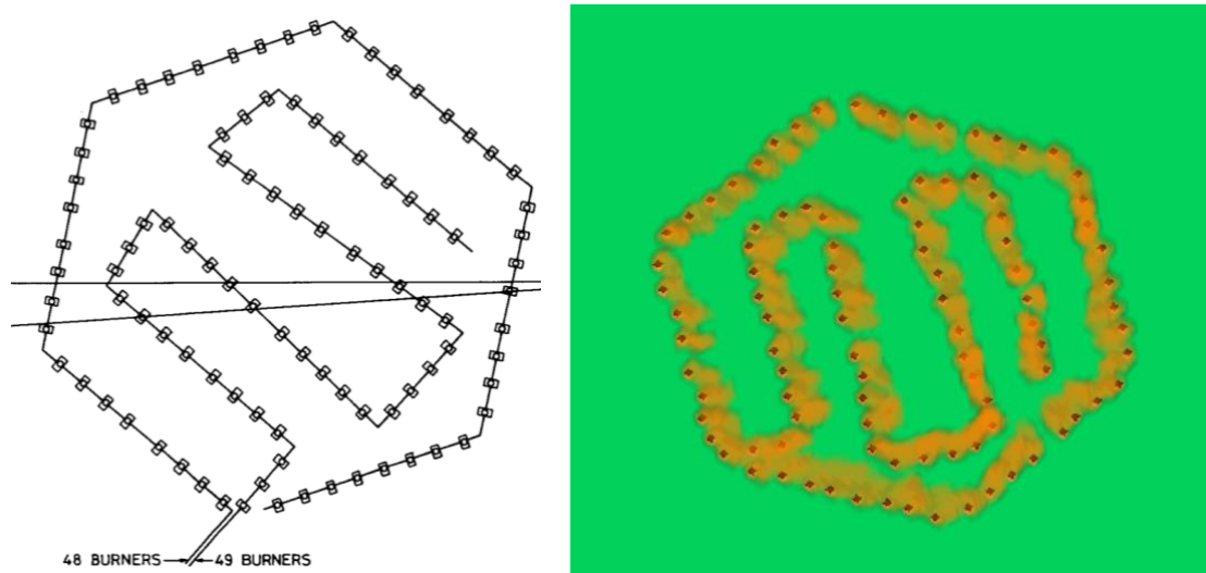
Figure 27. Hexagonal burner array used in the Meteotron experiments. Left: schematic of the array (from Benech 1976). Right: plan view of an active burner array in FDS.
