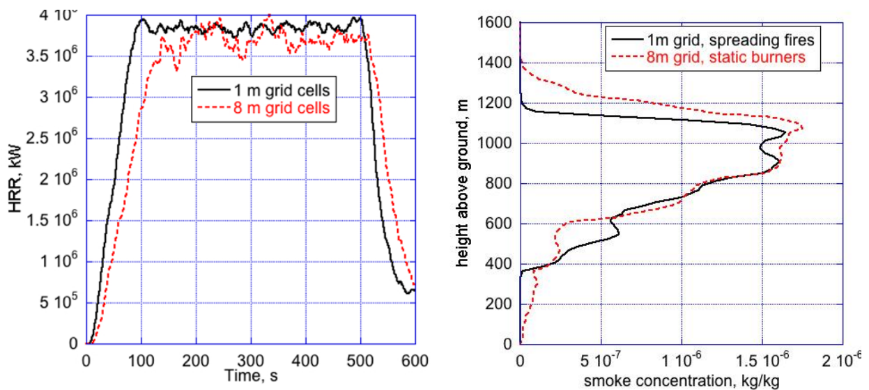
Figure 17: On the left are HRR time histories from WFDS-LS simulations of the smoke plume scenario shown in Figure 16 using two grid resolutions, 1 m and 8 m. On the right are 30 second time averaged smoke concentration profiles 2 km downwind of the middle of the burn plot shown in Figure 16 (see text for details).
