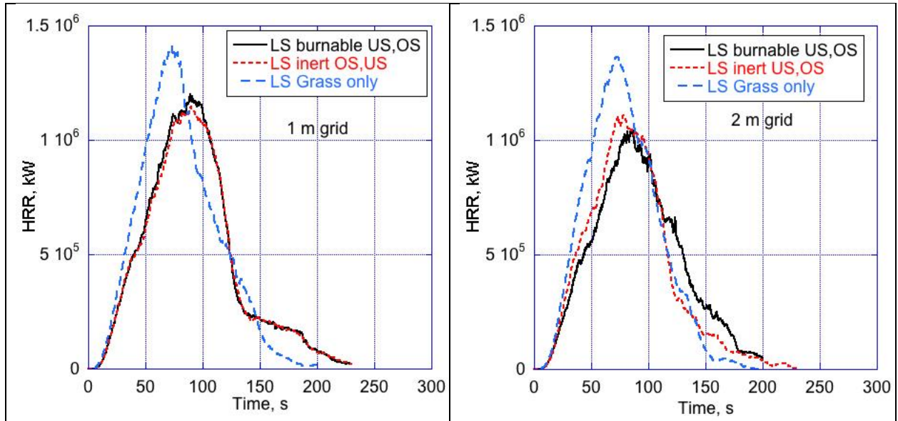
Figure 15: HRR from WFDS-LS prescribed burn simulations with raised vegetation that can burn (black solid curve), raised vegetation that cannot burn (red short-dash), and no raised vegetation (only grass is present, blue long-dash).
