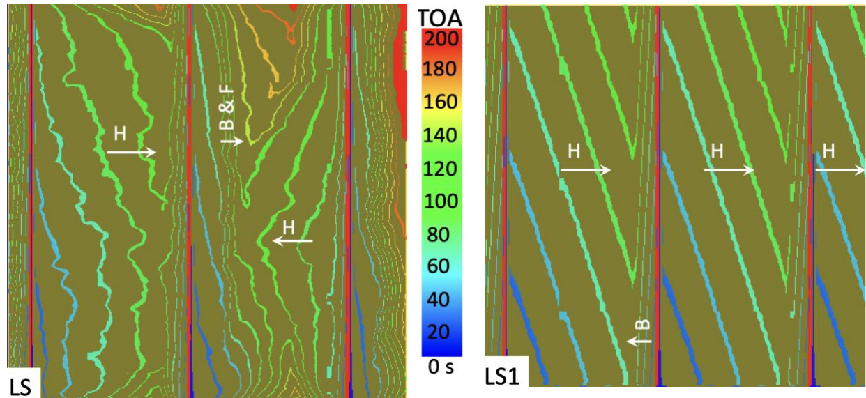
Figure 9: Surface fire time of arrival (TOA) contours in the center 100 m x 100 m area from simulations of the prescribed burn scenario shown in Figure 6 and Figure 8. The raised vegetation is not shown. The ambient wind flows left-to-right. The location of the leading edge of the fire front is plotted every 20 s (see legend). On the left are WFDS-LS predictions; on the right are predictions from the simplest level set implementation, WFDS-LS1, (consistent with FARSITE), both with a 1 m grid resolution. Some locations of head, back, and flank fire spread are identified by H, B, F, respectively. Arrows show direction of fire spread.
