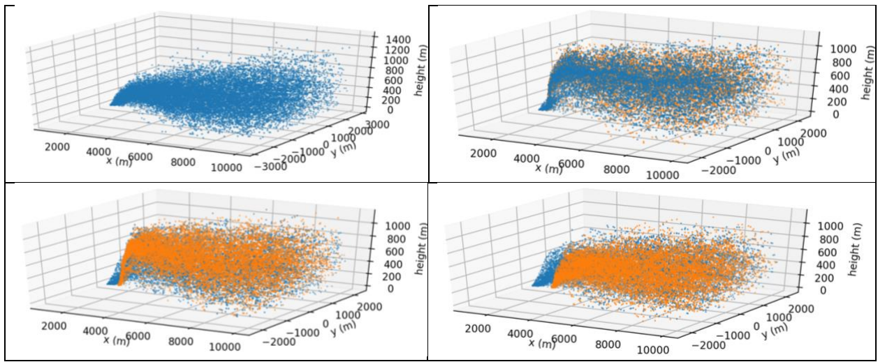
Figure 25. Examples of plume interaction simulations in ALOFT-FT. Plumes separated by 0 m (top left), 200 m (top right), 500 m (lower left) and 900 m (lower right) in the alongwind direction. Lagrangian particles representing the smoke are colored blue for the upwind fire and orange for the downwind fire.
