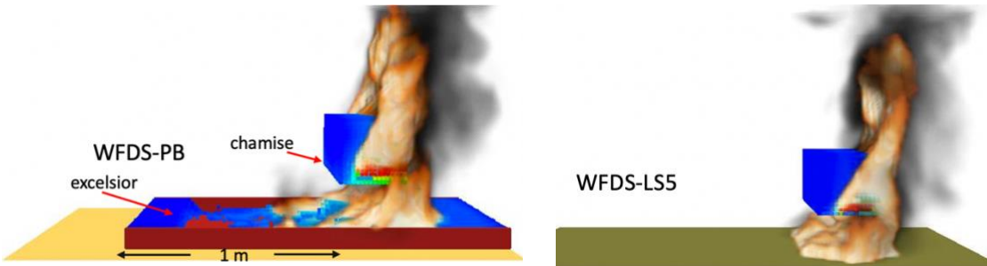
Figure 2: Snapshot of (55 s after ignition of excelsior fire) of WFDS-PB (on left) and WFDS-LS5 (on right) simulations of the Tachajapong et al. (2009) shrub crown fire initiation experimental case with a 1.5 m/s (3.3 mph) impose wind (flowing left to right) and a crown base height of 20 cm (8 inches). The flame surface is shown in orange, smoke in black, and vegetation temperature by colors with blue being the coolest ( \sim 20 C) and red the hottest ( \sim 1300 C). WFDS-LS5 does not explicitly model the presence of the surface vegetation.
