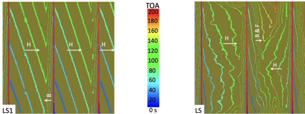
Figure 3: Surface-fire time of arrival contours in the center 100 m x 100 m area from of the prescribed burn scenario. The location of the leading edge of the fire front is plotted every 20 s (see legend). On the left are WFDS-LS1 predictions; on the right are WFDS-LS predictions, both with a 1 m grid resolution. Some locations of head, back, and flank fire spread are identified by H, B, F, respectively. Arrows show direction of fire spread.
