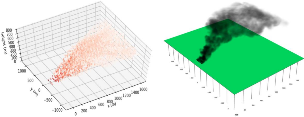
Figure 18. 3D Plumes from line fire simulations. Left: ALOFT-FT, Right: FDS.
