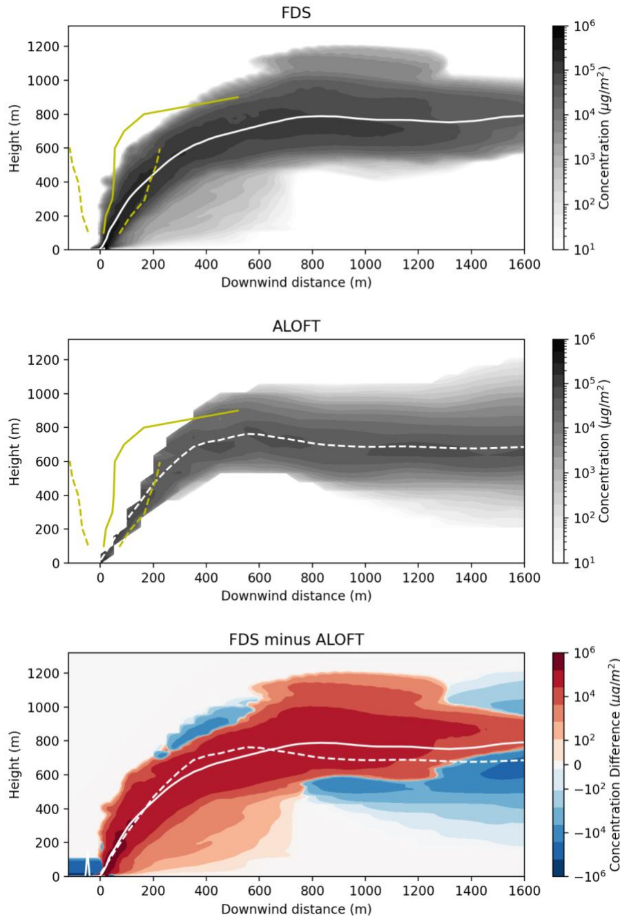
Figure 31. Vertical crosswind-integrated concentration contours from FDS (top) and ALOFT-FT (middle) simulations of the April 1973 Meteotron experiment. The extent of the plume as estimated from photogrammetry is shown in yellow. In most of the experiments, only a portion of the plume extent was estimated. Bottom: difference in CWIC between the FDS and ALOFT-FT simulated plumes. Results from simulations of the same trial at a lower wind speed are given in Appendix 7, p.59.
