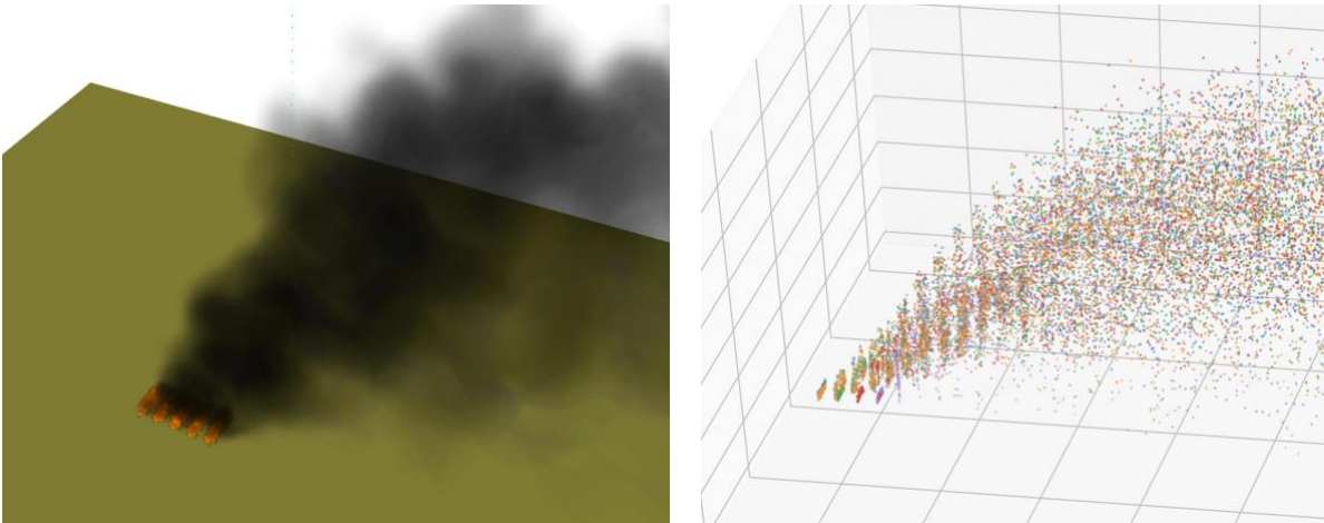
Figure 21. Five simultaneous line fires in FDS (left) and ALOFT-FT (right) simulations. In both cases, the separate plumes merge at short distances above the fires, effectively forming a single plume.
