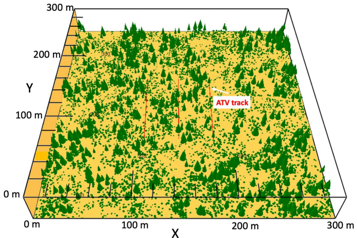
Figure 6: The 300 m x 300 m x 40 m computational domain used for comparing WFDS-PB and level set based predictions of a prescribed burn scenario. The vegetation is the same as was shown in Figure 5. The visualization tool Smokeview (designed for FDS and WFDS) is used. The locations of three simulated ATV ignition lines are shown in red.
