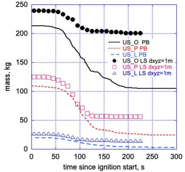
Figure 13: Time history of the dry mass in the understory components.
