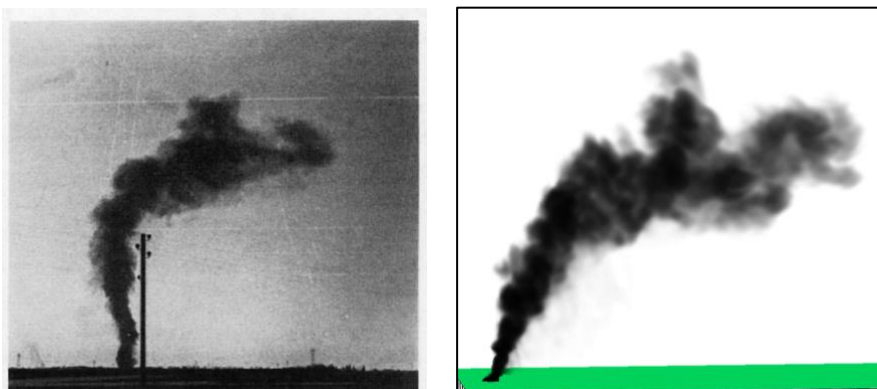
Figure 9. Left: a photograph of the April 1973 Meteotron plume (Benech 1976). Right: an FDS simulation of the experiment. Both images show the plume 300 s after ignition.
