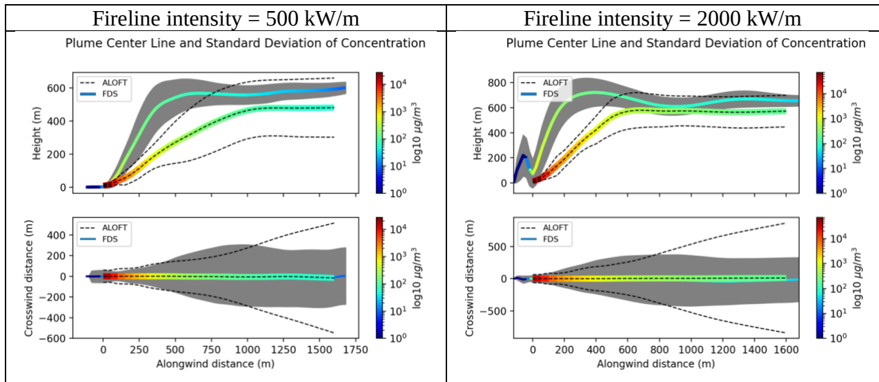
Figure 20. Plume centerlines and standard deviations of concentration in the FDS and ALOFT-FT simulations. Centerlines are colored by concentration (centerlines overlap in the bottom panel). Areas of one standard deviation of concentration from the centerline values are shown as gray shaded areas (FDS) and dashed lines (ALOFT-FT). Top panels: Vertical section of plumes. Bottom panels: Bird's eye view showing crosswind spread of FDS and ALOFT-FT plumes.
