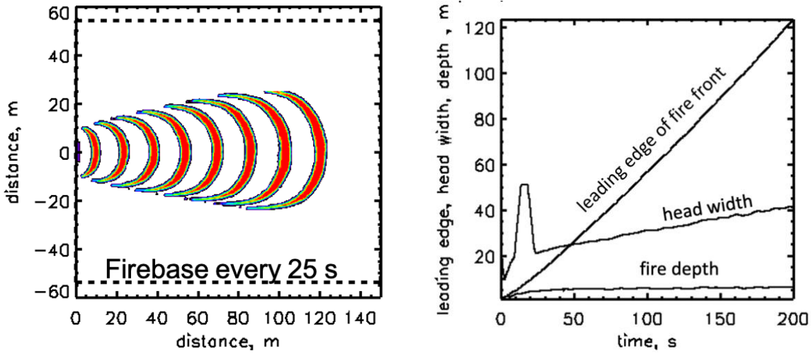
Figure 33: An example case from the WFDS-PB simulation database created to derive a formula for the head fire rate of spread as a function of the local net wind. In this case the ambient wind is 2.5 m/s (2 m above the ground) and the ignition fire line is 20 m long.
