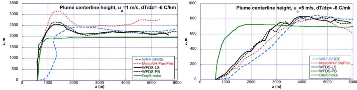
Figure 1: The smoke plume centerline height as a function of the downwind distance from an idealized single static fire line as predicted from five different models (Mell and Linn, 2017). Two different inflow wind speeds are shown: u(z) = u_0(z/2)^{1/7} with u_0 = 1 m/s (on the left) and u_0 = 5 m/s (on the right). The source of heat is a 750 m long, 25 m deep, stationary fire line with a heat release rate per unit area of 2000 \text{ kW m}^{-2} . The fire depth and heat release characteristics are based on fires observed during the International Crown Fire Modeling Experiments (Stocks et al. 2004).
