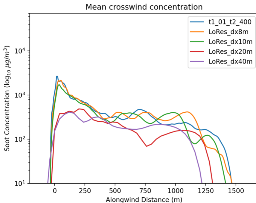
Figure 43. Alongwind concentration profiles. Grid cell sizes greater than 10 m produce lower concentrations than the original higher resolution simulation.
