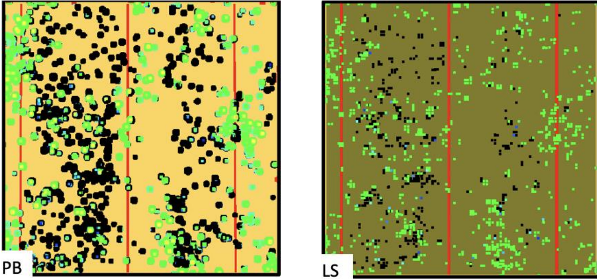
Figure 11: Comparison of the location of understory consumption from WFDS-PB and WFDS-LS (1 m grid resolution). Black denotes complete consumption; green denotes no consumption. The overstory is not shown.
