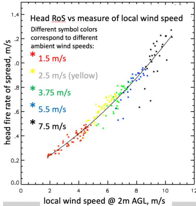
Figure 34: The local head fire rate of spread (RoS) plotted against the local horizontal wind speed normal to the leading edge of the head fire. Derived from five WFDS-PB simulations (each with a different ambient wind as denoted by the different colors) of a grassfire with a 10 m long ignition line
