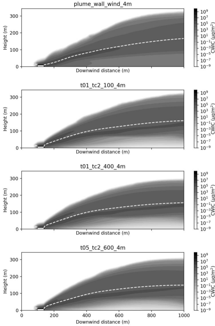
Figure 52. Contours from crosswind-integrated concentrations of plumes. From top down: wall-of-wind simulation; nudging with t_2=100 s, t_2=400 s, and t_2=600 s ( t_1=5 s in the bottom panel).
