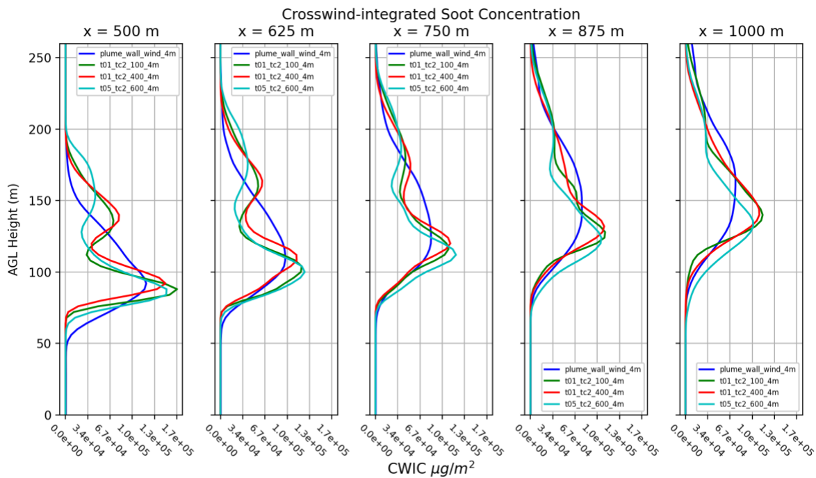
Figure 51. Vertical profiles of crosswind-integrated concentrations at specific downwind locations.
