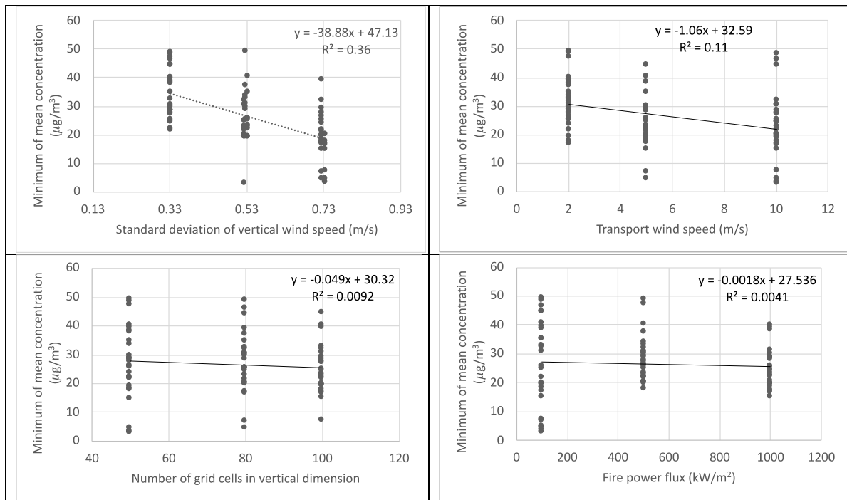
Figure 39. Effect of key parameters on mean far field plume concentration ( \mu\text{g}/\text{m}^2 )
