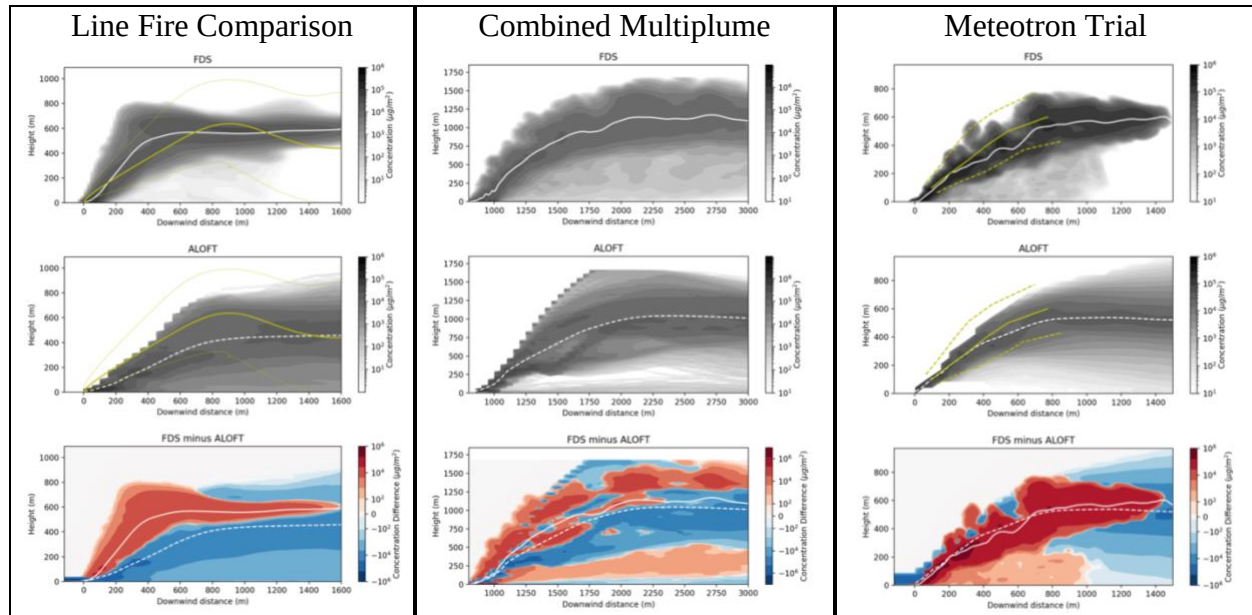
Figure 6. Crosswind-integrated plume concentrations and centerlines. Left column: line fire with intensity of 500 kW/m in FDS (top), ALOFT-FT (middle) and MW94 plumes (top & middle, indicated by yellow lines). Centerlines are indicated by white solid or dashed lines. Middle column: Combined plume from five separate line fires in FDS (top) and ALOFT-FT (middle). Right Column: Comparison to 1971 trial of the Meteotron experiment. Observed plume extent shown in yellow lines. Bottom row, all columns: Differences between the FDS and ALOFT-FT simulated plumes. Red indicates regions in which the FDS concentration values are greater than those simulated by ALOFT-FT; blue indicates the opposite.
