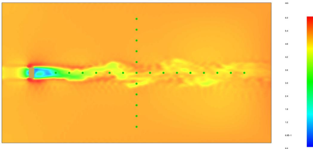
Figure 49. Cross section showing simulated wind flowing past a trip block (left side of image). Flow is from left to right. Green dots indicate locations of velocity measurements.
