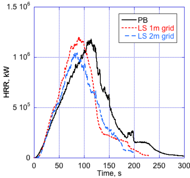
Figure 12: HRR history from the WFDS-PB and WFDS-LS prescribed burn scenario simulations.
