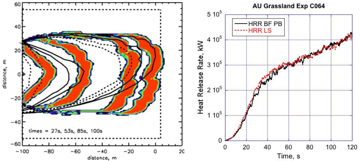
Figure 4: On the left are the fire footprints for the same case shown in Figure 3 for WFDS-PB, but here WFDS-LS predictions are shown by color contours of the heat release rate per unit area, kW/m 2 . On the right is the time history of the HRR from WFDS-PB (black curve) and WFDS-LS (red dashed curve).
