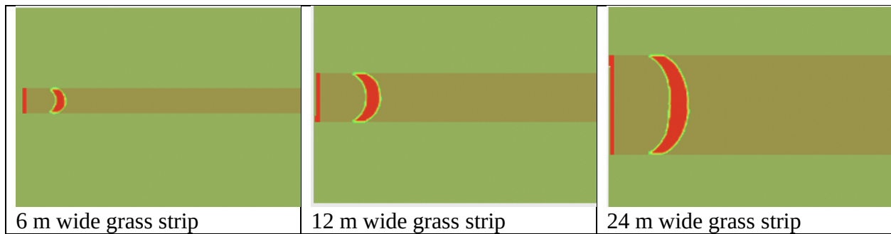
Figure 35: Configuration of grass-strip test cases to compare WFDS-PB and WFDS-LS. Ambient with of 2.6 m/s (2 m AGL) flow left to right.
