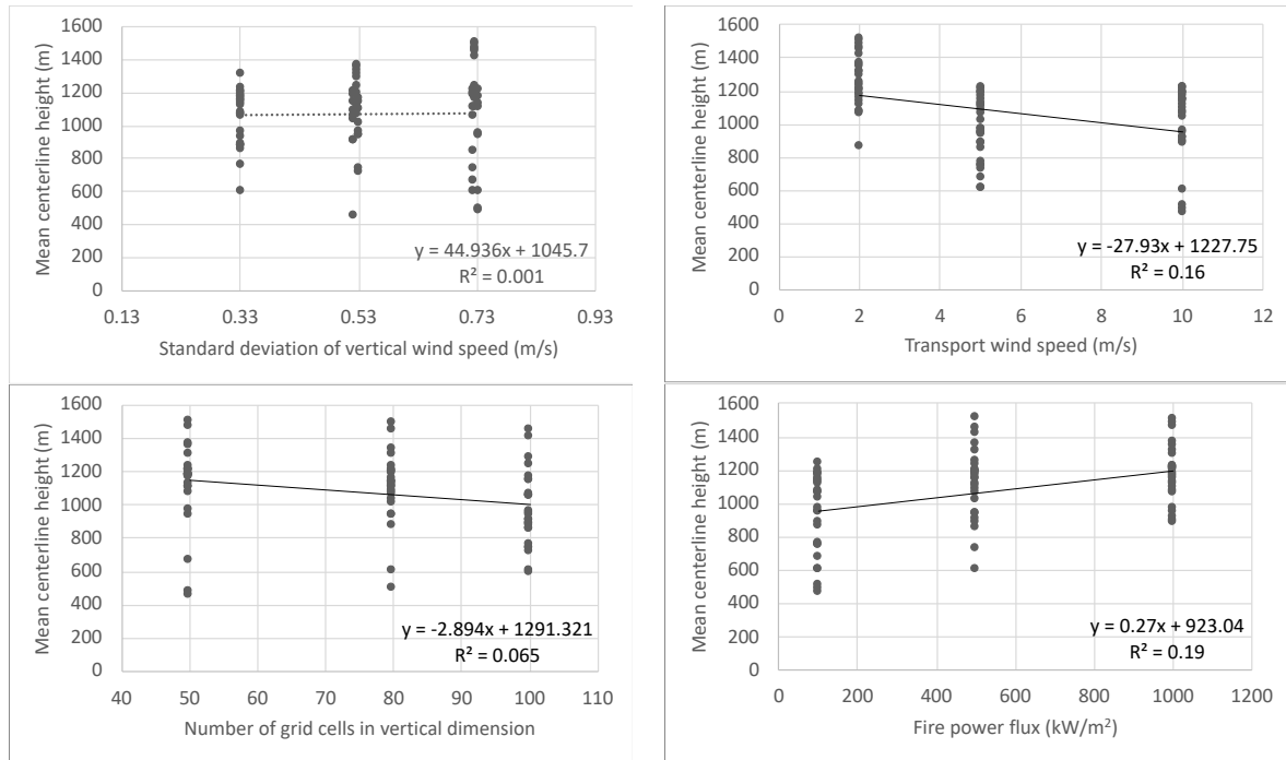
Figure 38. Effect of key parameters on mean plume centerline height (m)
