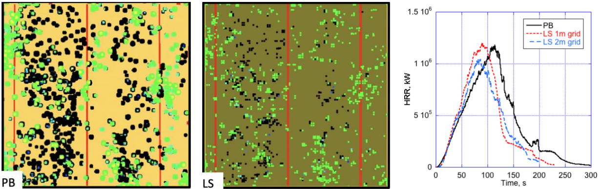
Figure 4: Comparison of the location of understory consumption from WFDS-PB and WFDS-LS (1 m grid resolution). Black denotes complete consumption; green denotes no consumption. The overstory is not shown. Rightmost plot is the time history of the global heat release rate (HRR).
