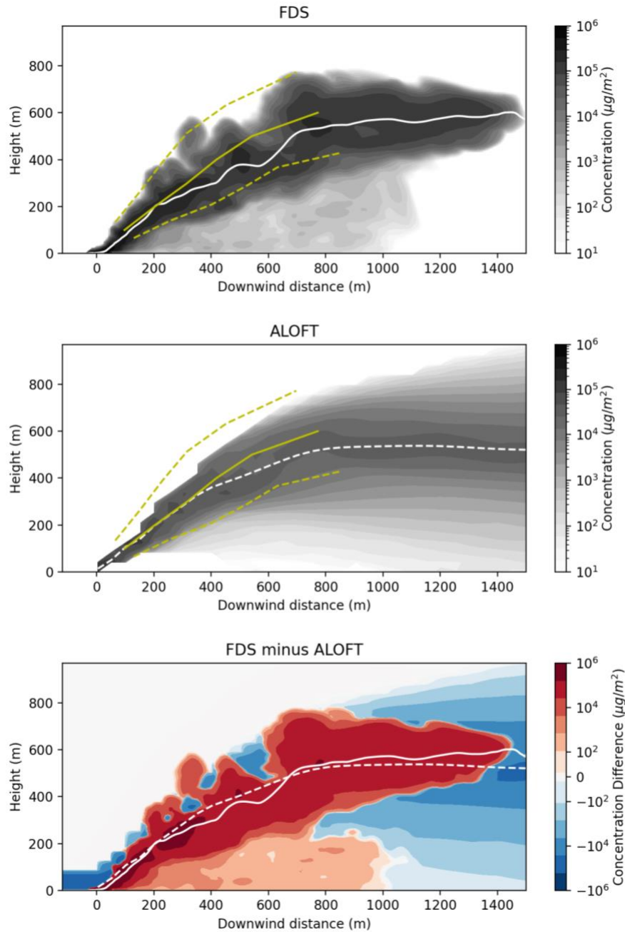
Figure 29. Crosswind-integrated concentration contours from FDS (top) and ALOFT-FT (middle) simulations of the October 1971 Meteotron experiment. The extent of the plume as estimated from photogrammetry is shown in yellow. In most of the experiments, only a portion of the plume extent was estimated. Bottom: difference in CWIC between the FDS and ALOFT-FT simulated plumes.
