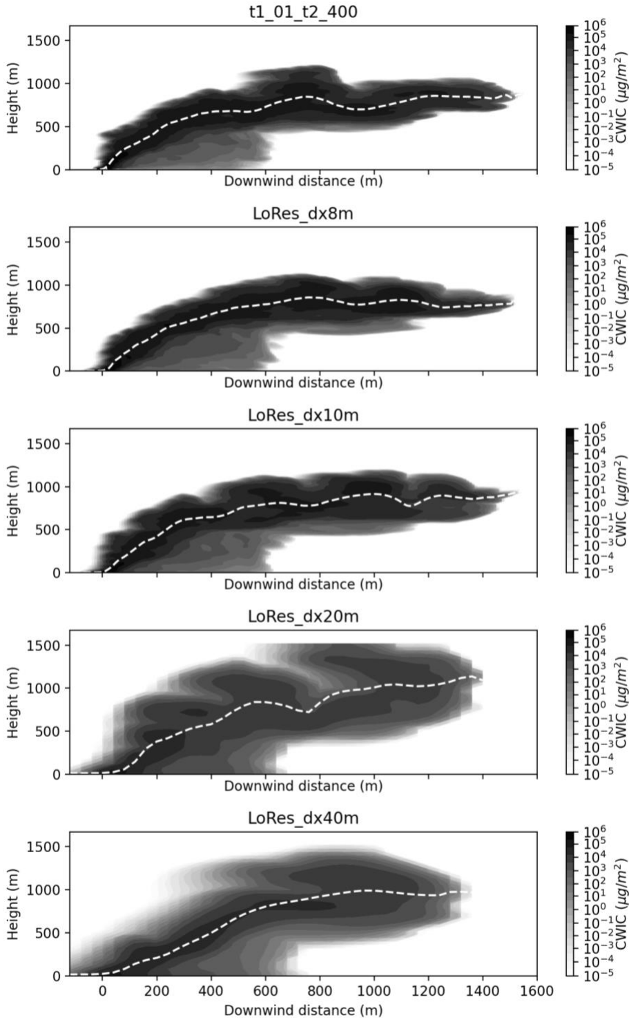
Figure 44. Concentration contour plots from FDS simulations of the April 1973 Meteotron plume experiment. Grid cells sizes increase from top to bottom in the figure.
