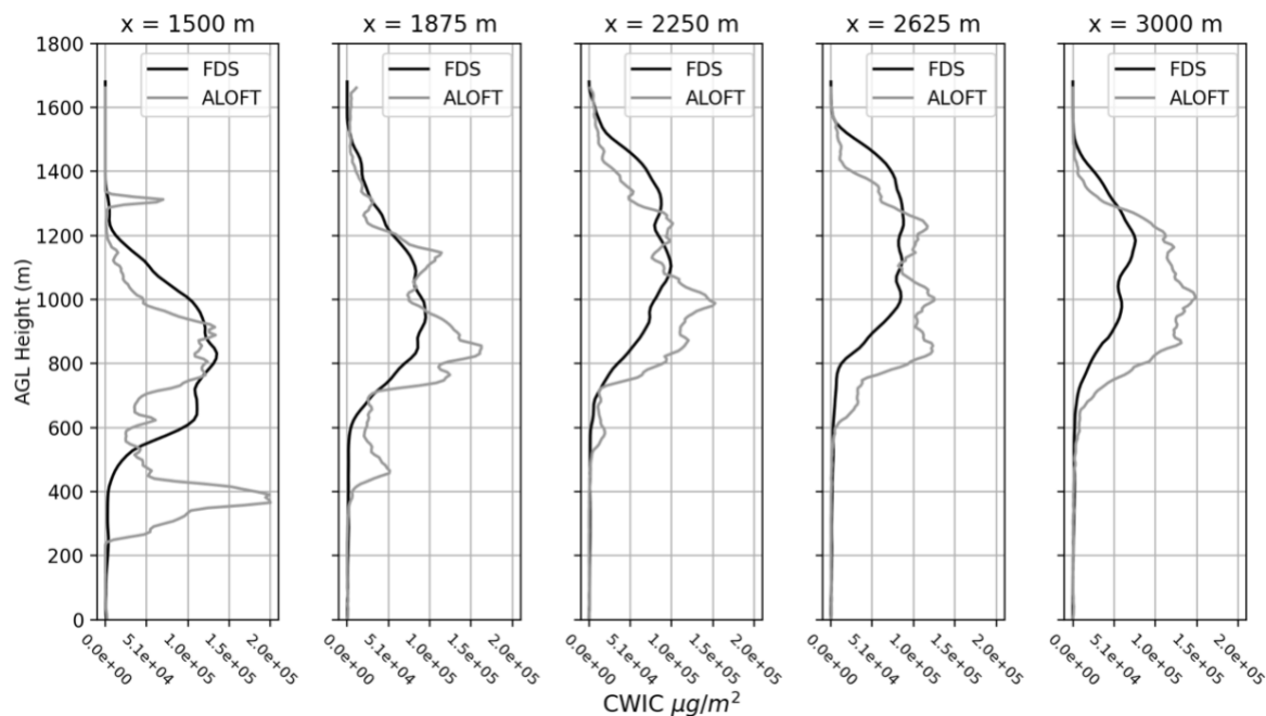
Figure 24. Vertical profiles of crosswind-integrated smoke (soot) concentrations at five downwind locations.
