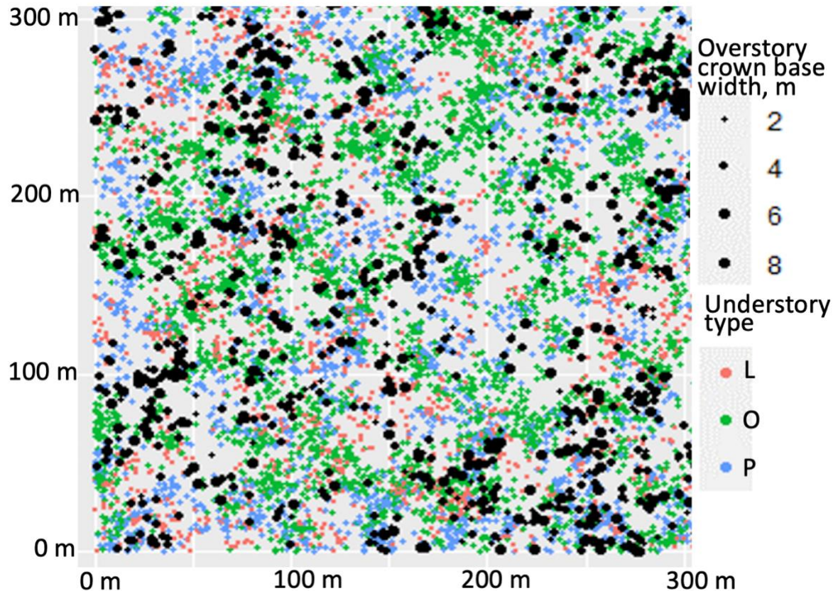
Figure 5: Distribution of raised vegetation used in the WFDS simulations. Black objects show location of longleaf pine and turkey oak overstory with the size of the object giving a measure of the crown base width (see legend). Colored objects denote the type of understory as shown in legend with L = longleaf pine, O = turkey oak, and P = persimmon.
