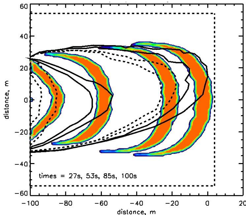
Figure 3: Observed (dashed or solid lines) and WFDS-PB predicted (color contours of mass loss rate, kg/s) footprints of the fire base at four times after the start of the ignition procedure in the AU grassland experiment C064 (Mell et al., 2009).
