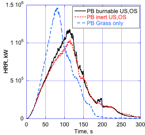
Figure 14: HRR history from WFDS-PB prescribed burn simulations with raised vegetation that can burn (black solid curve), raised vegetation that cannot burn (red short-dash), and no raised vegetation (only grass is present, blue long-dash).
