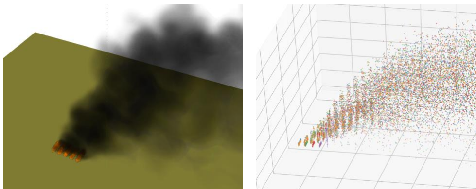
Figure 7. Multi-line fires in FDS (left) and ALOFT-FT (right) simulations. In both cases, the separate plumes merge at short distances above the fires, effectively forming a single plume.
