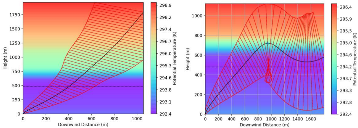
Figure 37. Plumes from MW94 model. The dotted horizontal line in both panels indicates the beginning of a temperature inversion above a mixed layer. Air temperature is indicated by the background colors in the plots. On the left is a plume from the original model before the effects of atmospheric stability are accounted for. On the right, using the same plume parameters, the plume from the modified model penetrates the temperature inversion and then oscillates around an equilibrium level. (Temperature and height scales differ between panels.)
