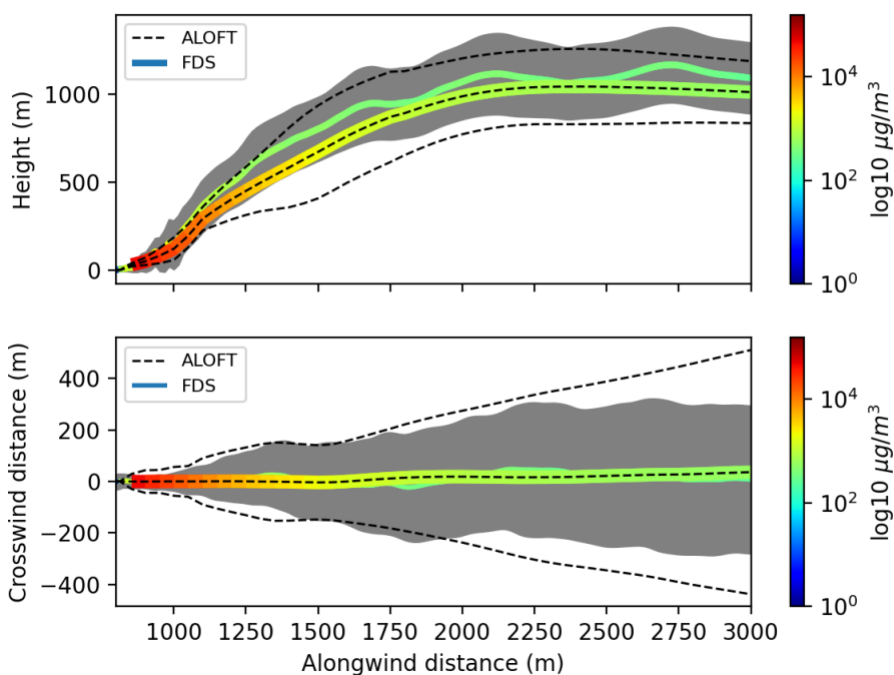
Figure 23. Plume centerlines and standard deviations of concentration in the FDS and ALOFT-FT simulations. Centerlines are colored by concentration (centerlines overlap in the bottom panel). Locations of one standard deviation of concentration from the centerline values are shown as gray shaded areas (FDS) and dashed lines (ALOFT-FT). Top: Vertical section of plumes. Bottom: Plan view showing crosswind spread of FDS and ALOFT-FT plumes.
