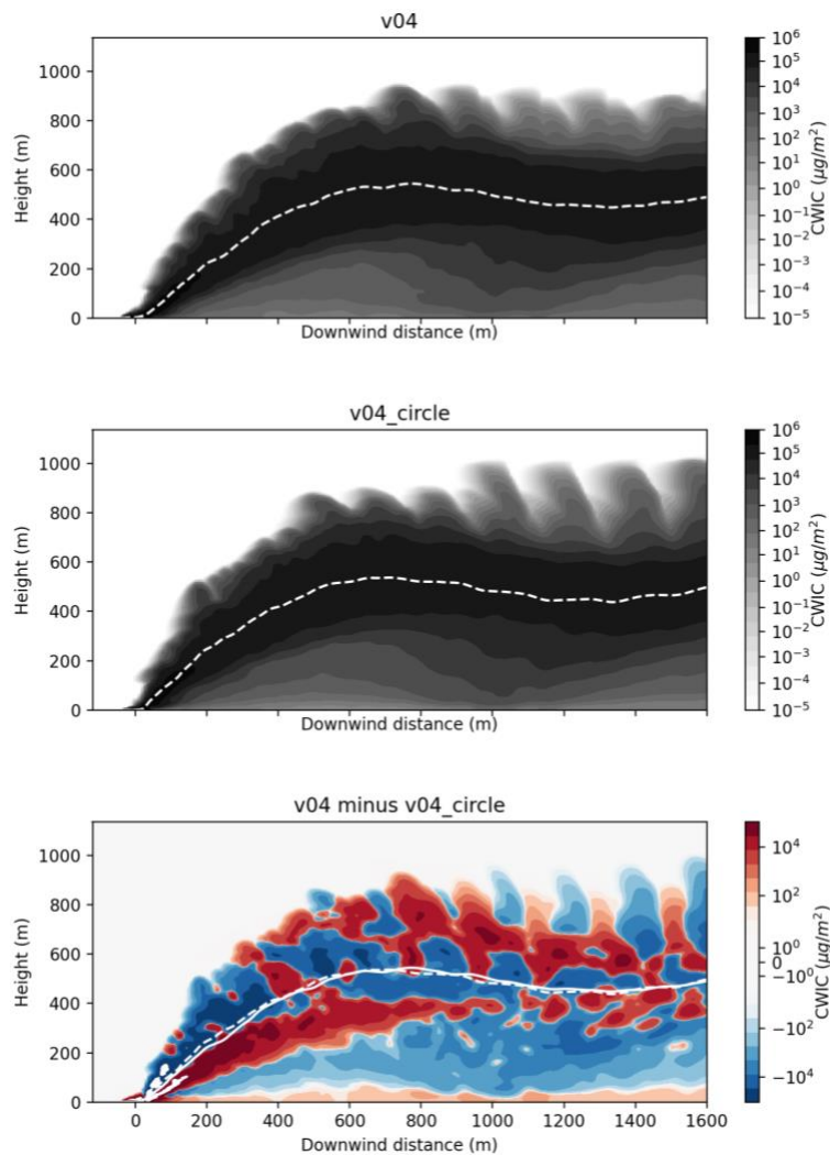
Figure 40. Crosswind-integrated concentration contours of plumes from the original burner array (top) and equivalent circular burner (middle). Bottom: differences between the detailed and circular burner concentrations. The largest variations are only about 20% of the maximum values of CWIC.
