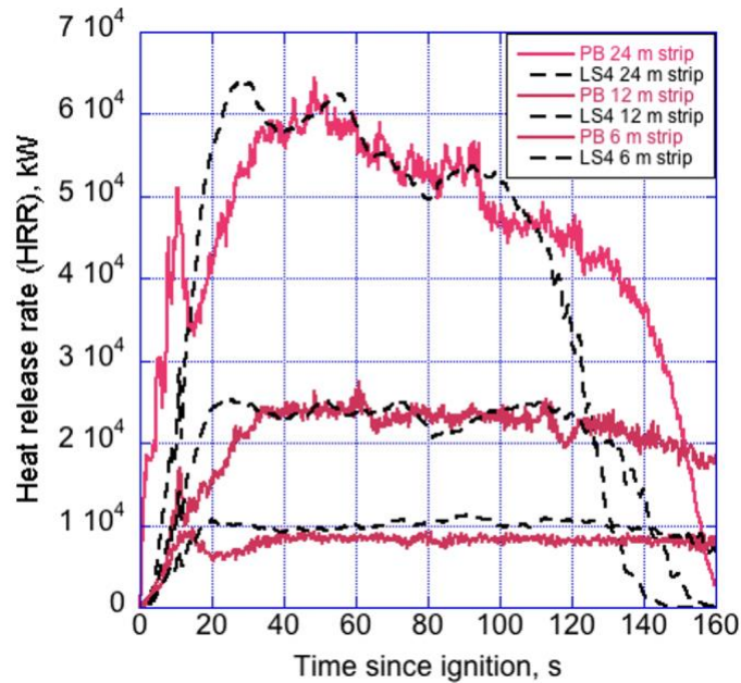
Figure 36: HRR for WFDS-PB (red line) and WFDS-LS (dashed black line) simulations of the grass-strip fire test cases shown in Figure 35. The higher magnitude HRR histories are for the wider grass strips.
