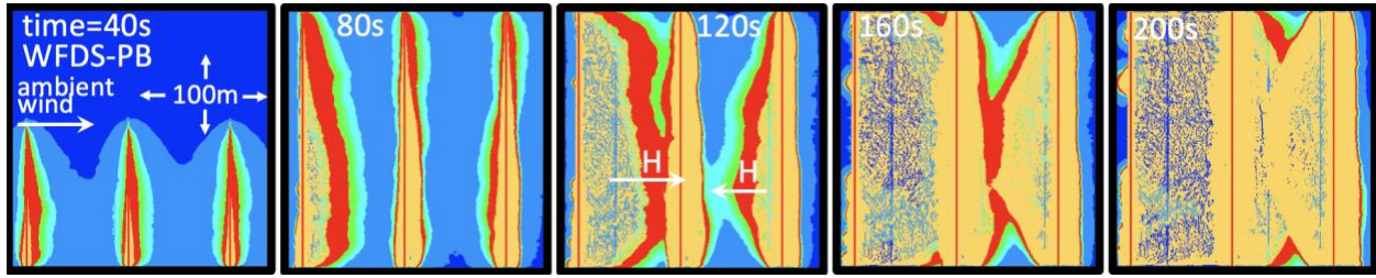
Figure 2: Color contours of the grass temperature at five times (every 40 s) from the PB simulation of the prescribed burn scenario shown in Figure 1 (only the center 100 m x 100 m is shown here). Red denotes the location of the flaming base of the fire; dark blue is ambient. The straight red lines are the simulated ATV tracks. The letter H denotes a head fire.
