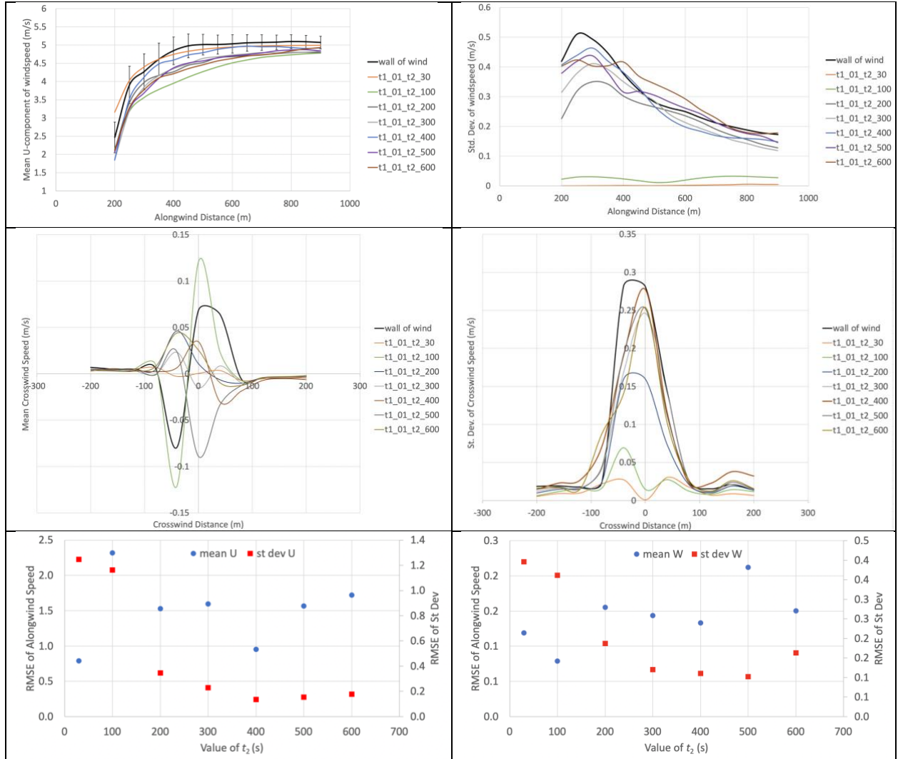
Figure 50. Effect of relaxation time on wind speeds and turbulence. Top left: mean wind speed in the alongwind direction downwind of the trip. Error bars show standard deviation of wind speed in the wall of wind simulation. Top right: Standard deviation of wind speed. Middle left: mean wind speed in crosswind direction. Middle right: standard deviation of crosswind speed. Bottom left: root mean squared errors of mean alongwind speed and standard deviation (note secondary scales). Bottom right: root mean squared errors of crosswind speed and standard deviation.
