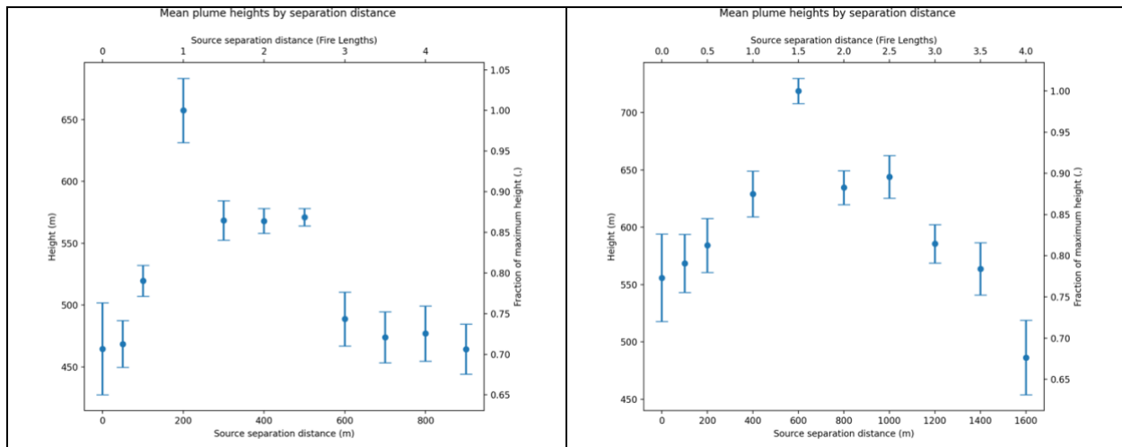
Figure 26. Mean far-field centerline heights of the combined plumes. Standard deviations are shown as vertical error bars. Secondary axes show separation distance normalized by fire line length (upper x-axes) and the fractions of maximum height (right y-axes). Left: 200 m x 10 m static fire lines. Right: 400 m x 10 m static fire lines.
