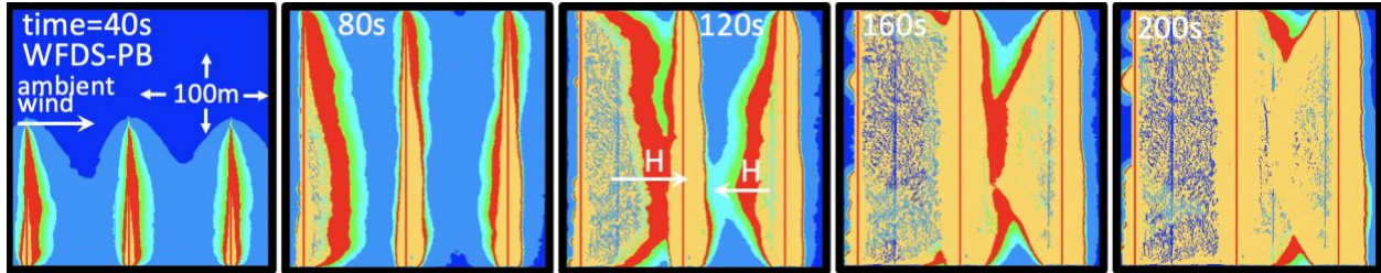
Figure 7: Color contours of the grass temperature at five times from the PB simulation of the prescribed burn scenario shown in Figure 6. Red denotes the location of the flaming base of the fire. The straight red lines are the simulated ATV tracks.
