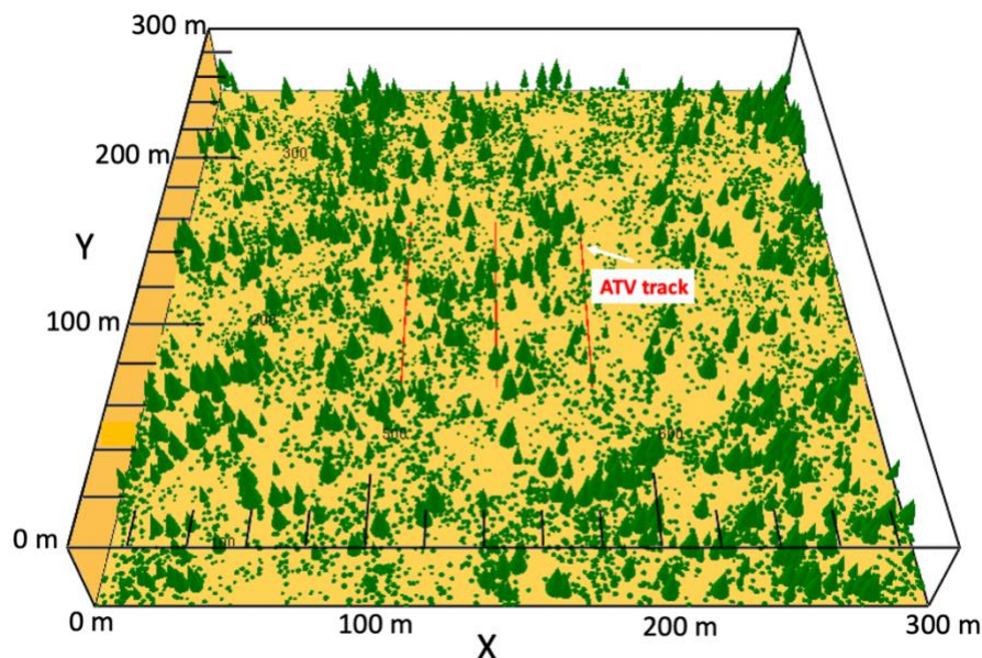
Figure 1: The 300 m x 300 m x 40 m computational domain used for comparing WFDS-PB and WFDS-LS predictions of a prescribed burn scenario. The visualization tool Smokeview (designed for FDS and WFDS) is used. The locations of three simulated ATV ignition lines are shown in red.
