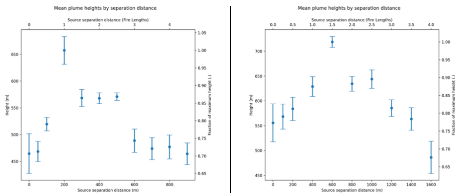
Figure 8. Mean far-field centerline heights of the combined plumes from line fires. Standard deviations are shown as vertical error bars. Secondary axes show separation distance normalized by fire line length (upper x-axes) and the fractions of maximum height (right y-axes). Left: 200 m x 10 m static fire lines. Right: 400 m x 10 m static fire lines.
