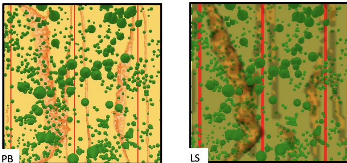
Figure 8: Comparison of simulated fire lines from WFDS-PB and WFDS-LS (2 m grid resolution) 84 s after start of ignition.
