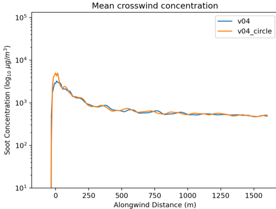
Figure 42. Mean crosswind concentrations are almost identical between the detailed (blue) and circular (orange) burner simulations.
