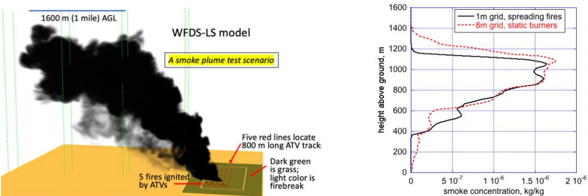
Figure 5: Smoke plume test scenario (on left) and resulting vertical smoke concentration profiles (30 s average, 2 km downwind of burn plot center) from WFDS-LS with spreading fires (1 m grid) and WFDS with a simplified representation of the fire (8 m grid).
