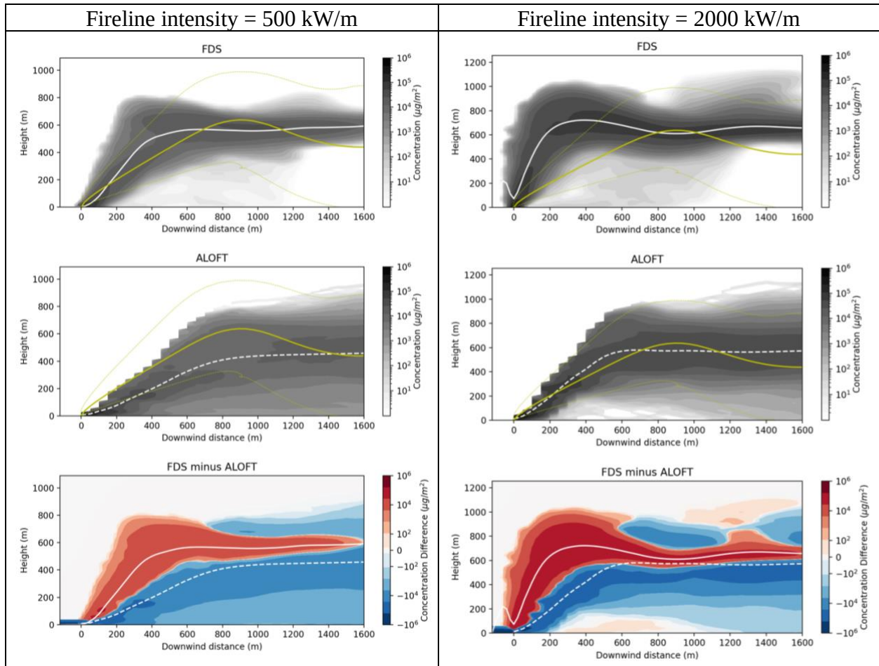
Figure 19. Crosswind-integrated plume concentrations from line fires with intensities of 500 kW/m ( left column ) and 2000 kW/m ( right column ). Centerlines are indicated by white solid or dashed lines. MW94 plumes are indicated by yellow lines. Top row: FDS plumes with MW94 plumes. Middle row: ALOFT-FT plumes with MW94 plumes. Bottom row: Differences between the FDS and ALOFT-FT simulated plumes. Red indicates regions in which the FDS concentrations are greater than those simulated by ALOFT-FT; blue indicates the opposite.
