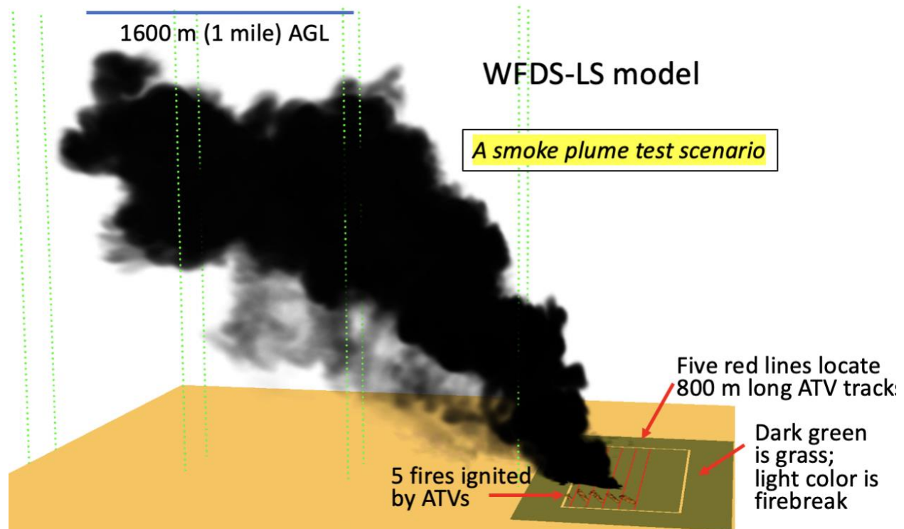
Figure 16: A smoke plume test scenario using WFDS-LS. The green dotted vertical lines are locations where the smoke concentration is output.
