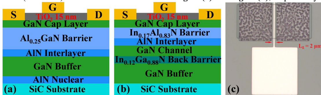
Fig. 38. Schematic of TiO 2 /AlGa N /Ga N (a) and TiO 2 /InAlN/Ga N (b) MISHEMT cross-section; (c) Microscope image of a fabricated device top-view with the gate length of 2 \mu\text{m} ;
