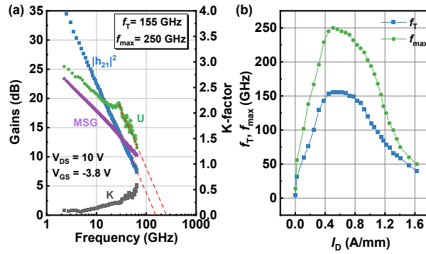
Fig. 34 (a) High-frequency gains ( |h_{21}|^2 , U and MSG), stability factor (k), (b) f_T/f_{max} versus I_D of HZO/InAlN/GaN MISHEMT with L_G of 50 nm.
