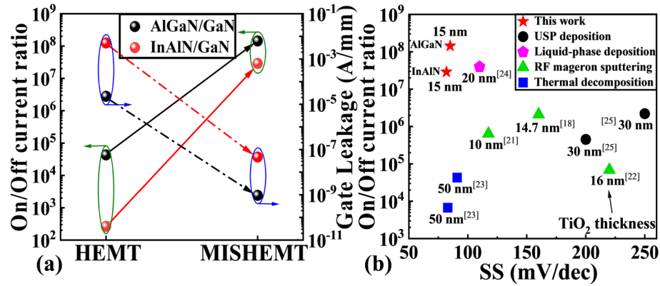
Fig. 41. (a) The on/off ratio and gate leakage current of AlGaIn/GaN, InAlN/GaN HEMT and HEMTs; (b) Comparison of on/off ratio and SS for MISHEMTs with TiO 2 dielectric.
