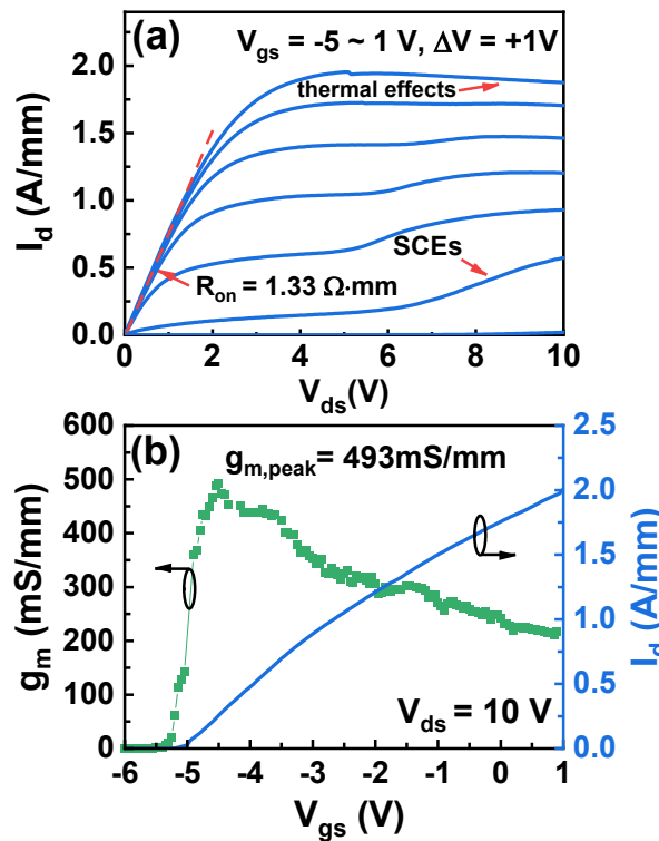
Figure 22. (a) Output characteristic, (b) the extrinsic transconductance g_m , and the transfer characteristic at V_{\text{ds}} = 10 V of the InAlN/GaN HEMT with a 50-nm gate length.
