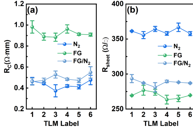
Fig. 10. (a) Ohmic contact resistance ( R_C ) and (b) sheet resistance ( R_{\text{sheet}} ) under N_2 annealing, FG annealing, and FG/ N_2 two-step annealing with six sets of TLM patterns ("I" represents the error bar).
