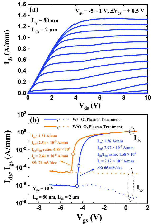
Fig. 1. (a) I - V output characteristic, (b) the semi-log-scale transfer curves and the gate leakage current as a function of V_{gs} at V_{ds} = 10 V of InAlN/GaN HEMT ( L_g = 80 nm) with and without O_2 plasma treatment.
