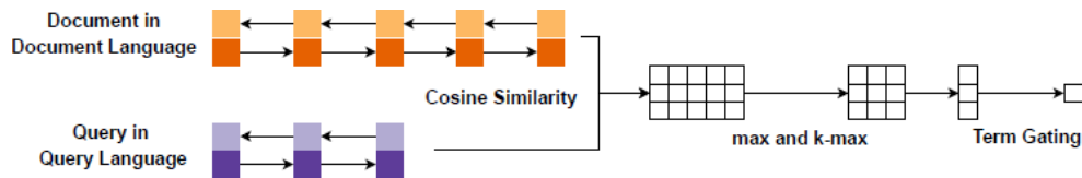
Figure 12. Bilingual POSIT-DRMM.
