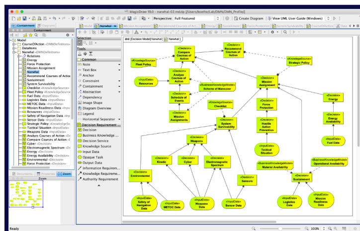
Figure 4 - A Decision Requirements Diagram loaded into the Decision Modeler running within MagicDraw
