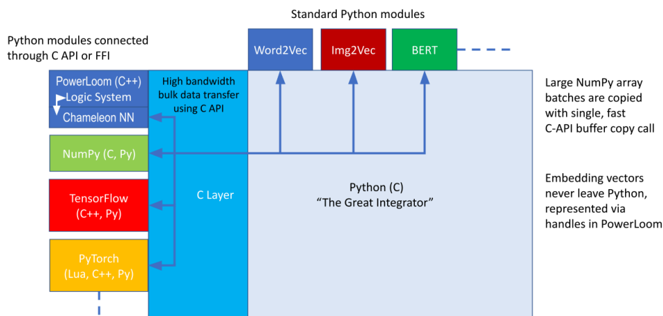
Figure 17: Chameleon 2.0 system architecture
