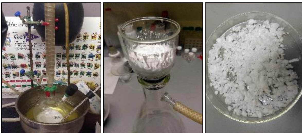
Figure 6. HGMs being reacted with HMDSO (left), being dried using vacuum filtration (center), and final product obtained (right)
