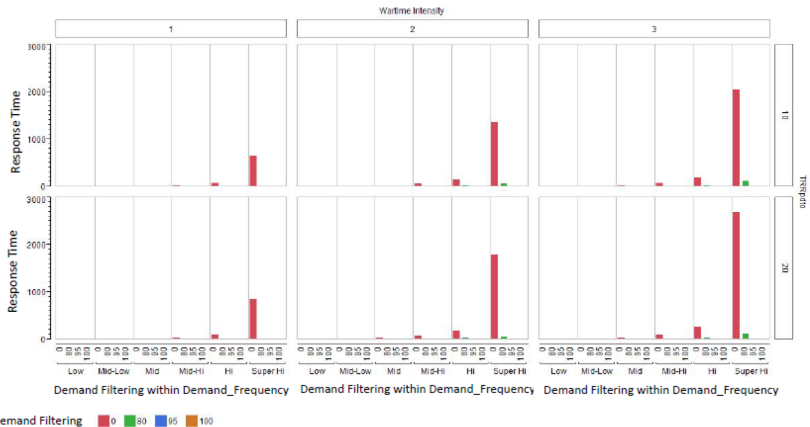
Figure 5-3. FOB Main Comparison
