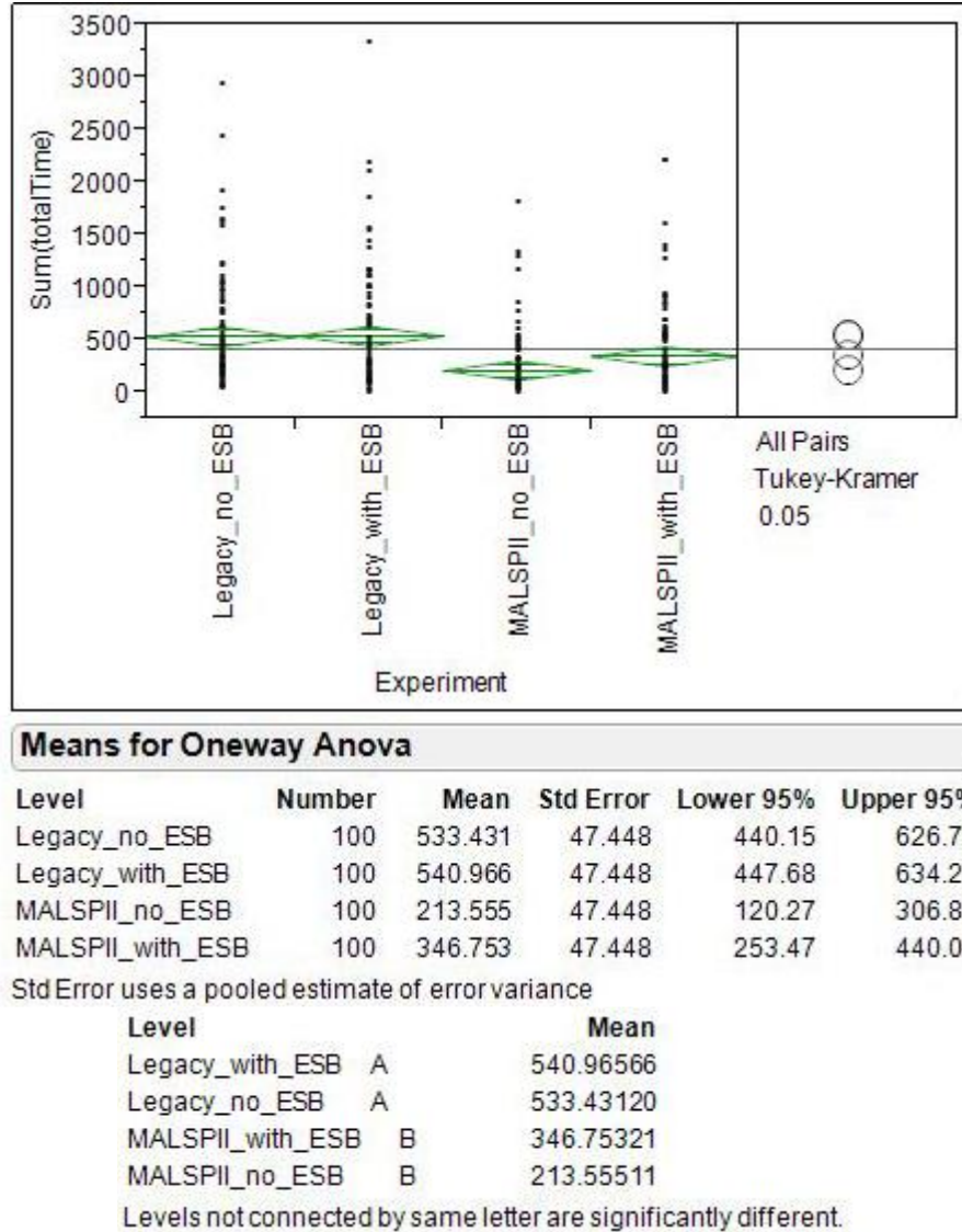
Figure A-6. ANOVA for Configuration _c; High TRR
