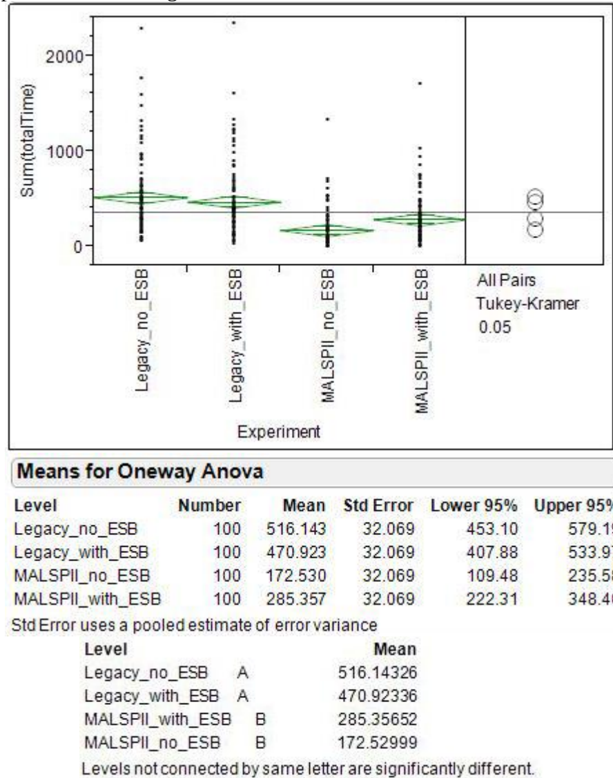
Figure A-8. ANOVA for Configuration_b; Low TRR
