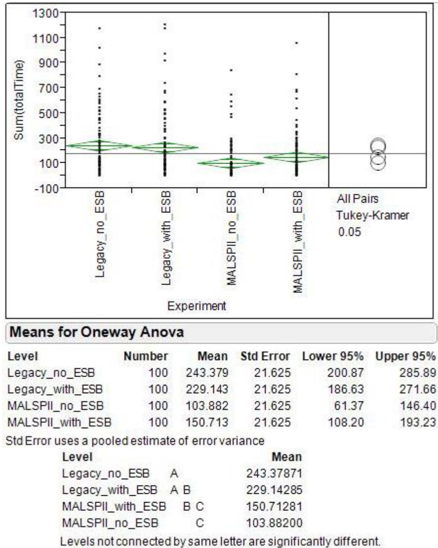
Figure A-9. ANOVA for Configuration _c; Low TRR
