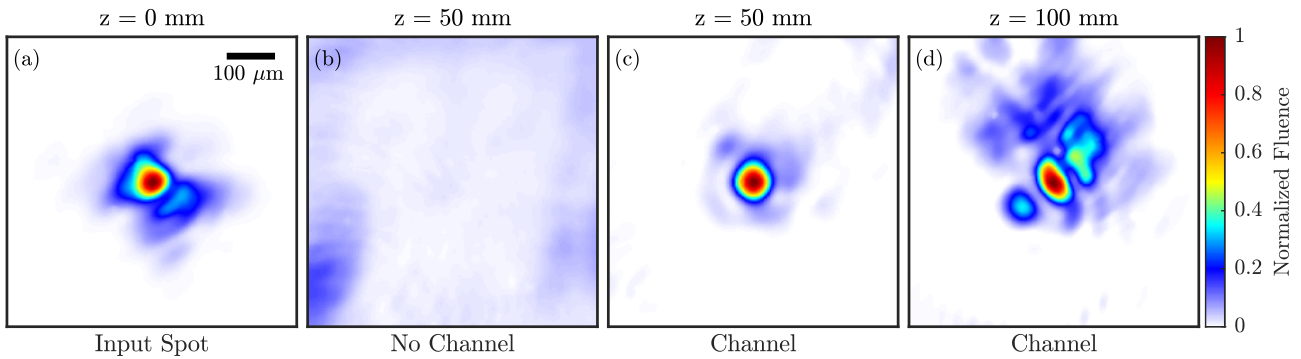
Figure 10: Measured transverse fluence profiles of the guided beam at: (a) focus, in vacuum; (b) z = 50 \text{ mm} , in vacuum; (c) z = 50 \text{ mm} , for P = 68 \text{ mbar} and \tau = 3.0 \text{ ns} ; (d) z = 100 \text{ mm} , for P = 26 \text{ mbar} and \tau = 2.7 \text{ ns} . The transverse scale is the same for all plots, as indicated by the scale bar shown in (a). For plots (a), (c), and (d) the fluence is normalized to the peak value in that plot; the fluence scale for (b) is the same as in (a). Compared to (a), the fluence scales of (c) and (d) were increased by factors of approximately 4 and 7 respectively.
