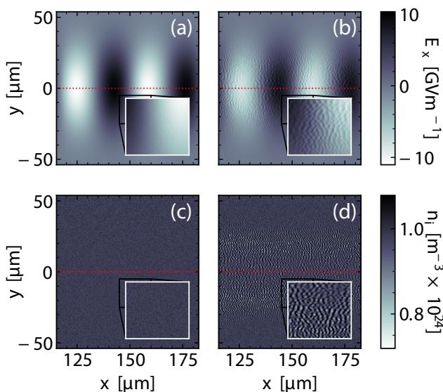
Figure 6: (a-b) Longitudinal electric field strength E_x(x, y) as a function of longitudinal ( x ) and transverse ( y ) position, (a) 0.32 ps and (b) 2.56 ps after wake excitation, showing the development of high-frequency modulations of the field envelope, magnified in the inset. (c-d) Corresponding ion density n_i(x, y) , showing the development of high-frequency modulations. The red line indicates the axis of initial laser propagation.
