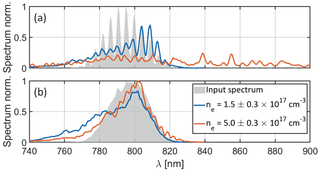
Figure 5: Preliminary analysis of experiments to demonstrate resonant excitation of plasma waves in a HOFI plasma channel. (a) Comparison of the spectrum of the pulse train at the entrance (grey) of a 110 mm long HOFI plasma channel with that at its exit for: (i) an on-axis density close to resonance, n_{e0} = (5.0 \pm 0.3) \times 10^{17} \text{ cm}^{-3} (red); and (ii) away from resonance, n_{e0} = (1.5 \pm 0.3) \times 10^{17} \text{ cm}^{-3} (blue). (b) As for (a), but for an unmodulated laser pulse of energy 2.5 J and duration 1 ps.
