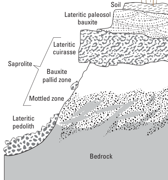
B. Lateritic bauxite deposits
