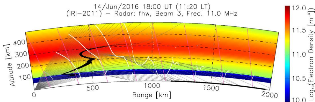
Figure 2. Numerical ray-tracing of radio waves through a model ionosphere along a particular beam of the Fort Hays radar
