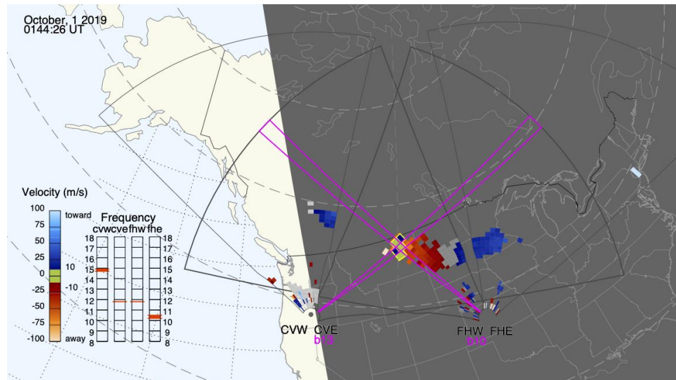
Figure 10. SuperDARN observations for a 1-min period beginning at 01:44 UT on 1 October 2019 during a bistatic campaign
