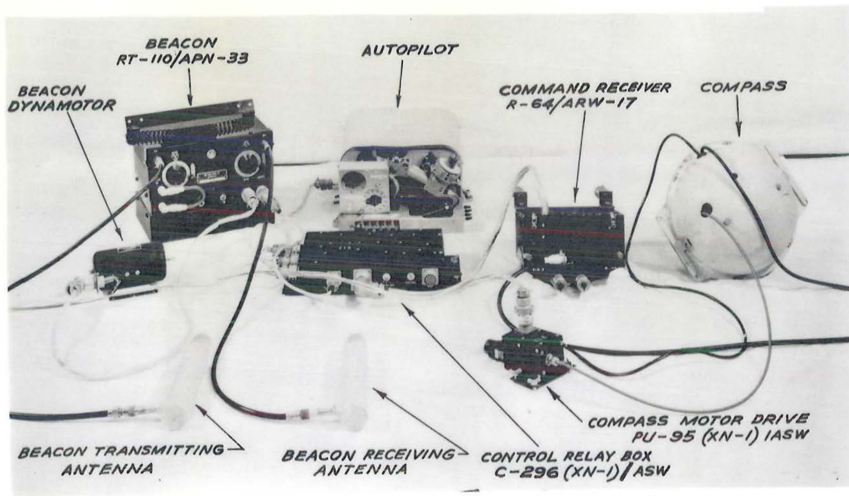
JB-2 ELECTRONIC AND FLIGHT CONTROL EQUIPMENT
