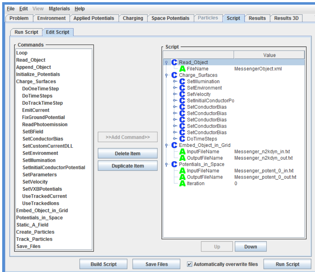
Figure 37. Edit Script Subtab: Making Problem Changes by Directly Modifying the Script
