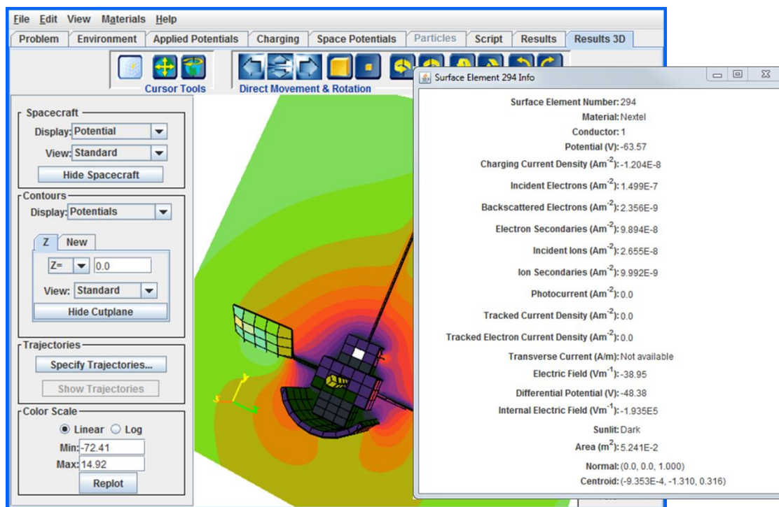
Figure 41. Results 3D tab: Displaying Potentials on a Plane through the Center of the Box, Together with Results for a Selected Surface Element
