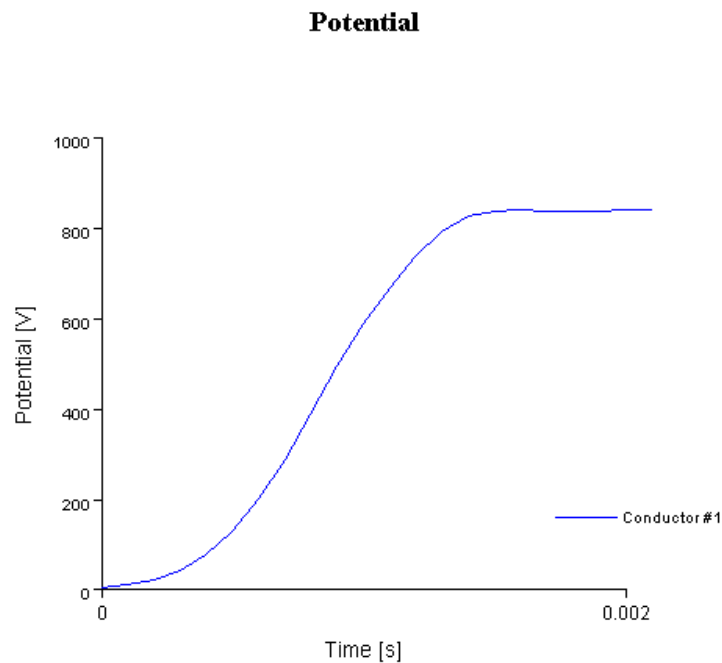
Figure 159. Potential versus Time for the Emitter Example.
