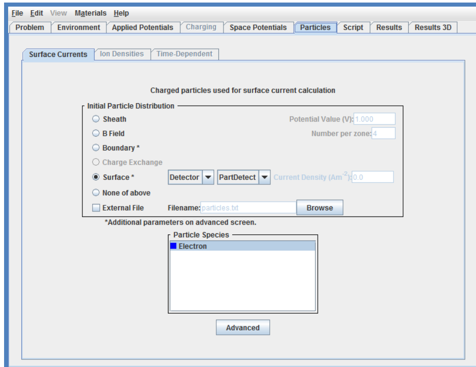
Figure 147. Particles Tab for the “Detector” Example
