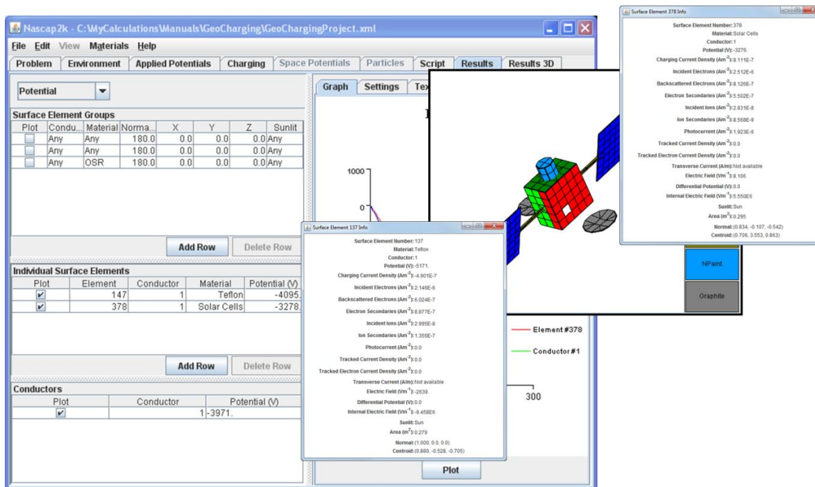
Figure 39. Results tab: Plotting Values at Surface Elements
