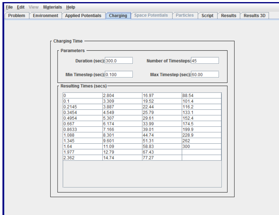
Figure 52. Charging Tab for the “GeoCharging” Example
