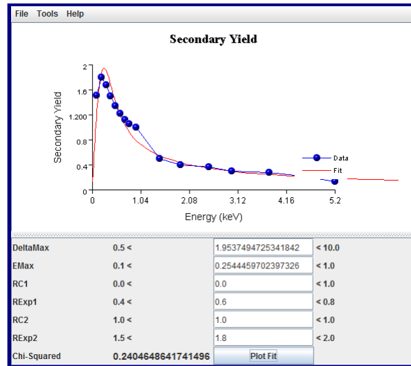
Figure 174. Yield Fitting Tool User Interface
