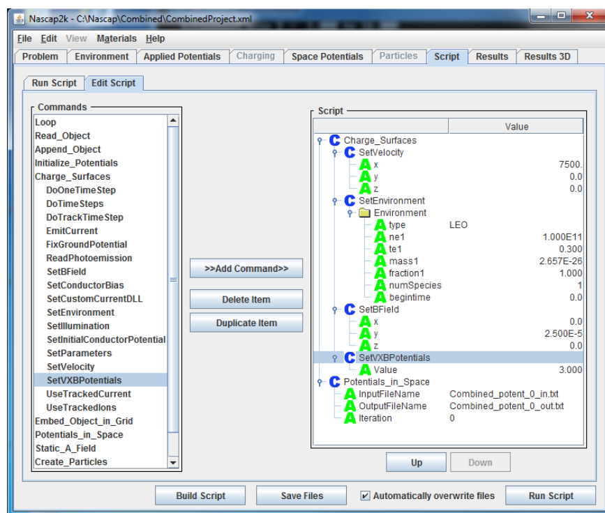
Figure 191. Script for Calculating Potentials
