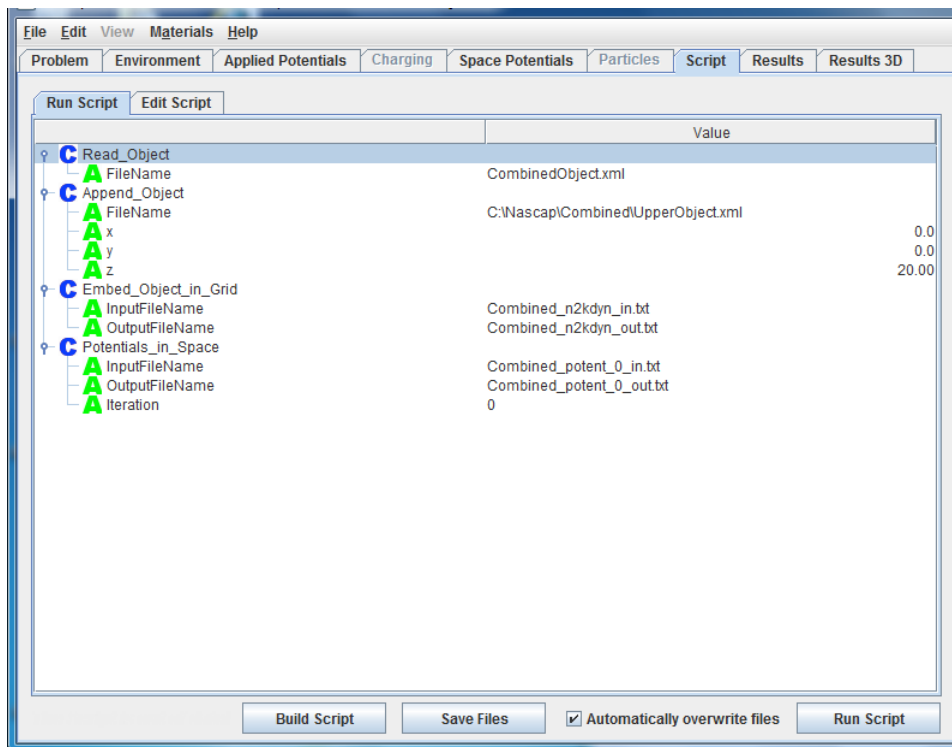
Figure 188. Script Used to Append “Upper” Object
