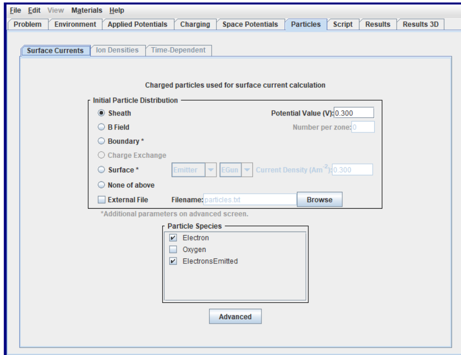
Figure 157. Particles Tab Specification for Sheath Electrons
