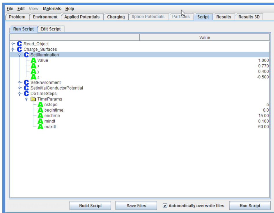
Figure 180. Script with Sun Direction Specified and 15 Seconds of Charging with Five Timesteps
