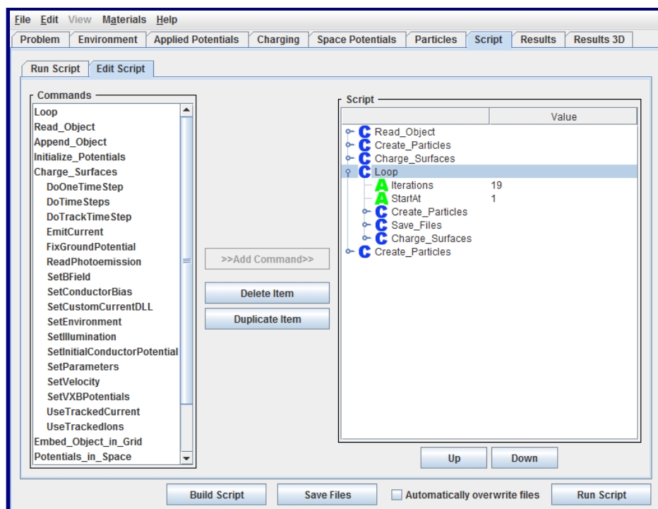
Figure 156. Edited Script Used to Write Input Files for Creating Macroparticles to Represent those Originating at the Emitter
