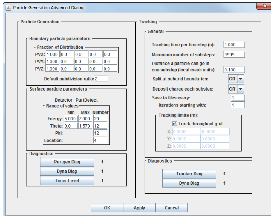
Figure 148. Advanced Particle Parameters Dialog Box for “Detector” Example
