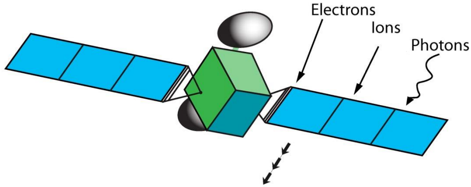
Secondary, Backscattered, Photo Electrons
