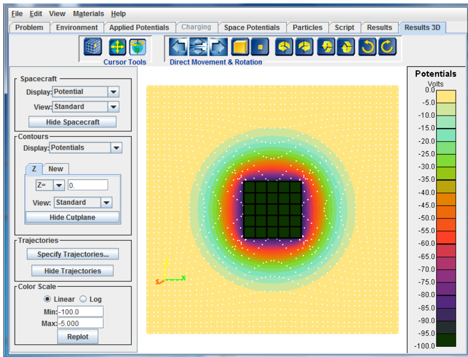
Figure 142. Particle Distribution for Case 3 of the “Dynamic” Example at t=10 \mu s
