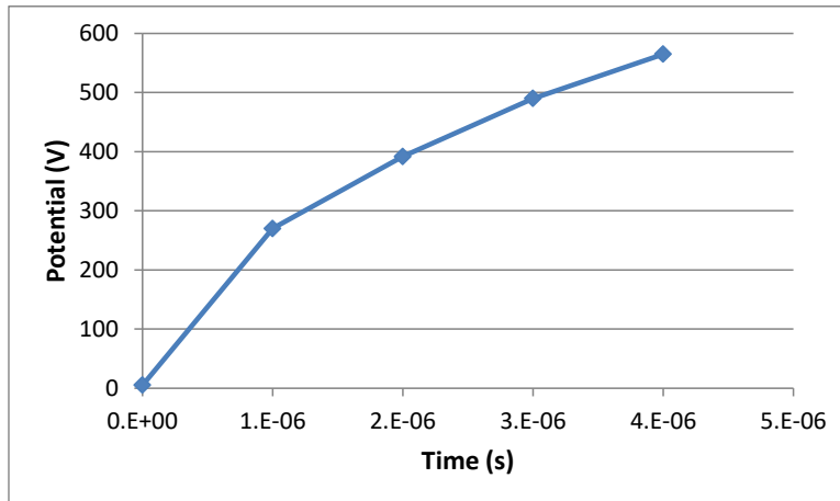
Figure 161. Charging Dynamics with the Stabilizing Current Derivatives Set to Zero.
