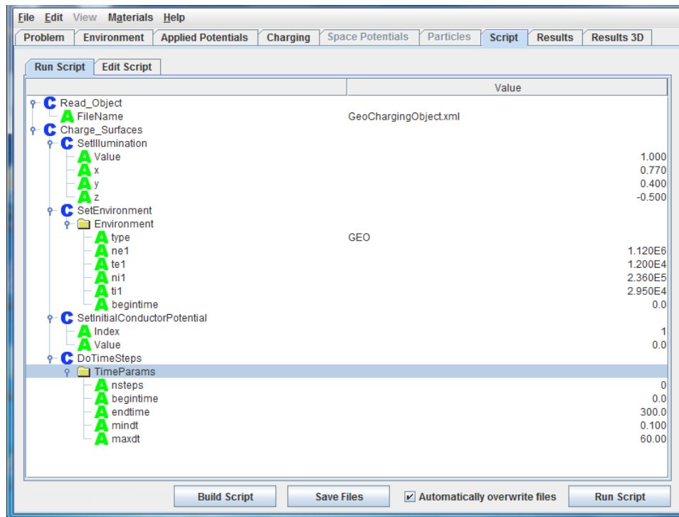
Figure 53. Script for Case 1 of the “GeoCharging” Example
