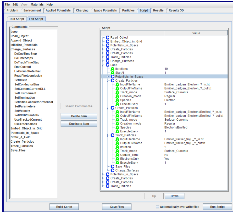
Figure 158. Final Script for Current Balance Calculation
