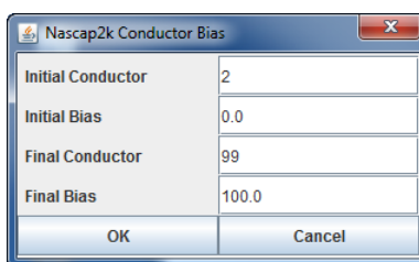
Figure 176. User Interface for Stand-alone Tool, Apply Distributed Bias
