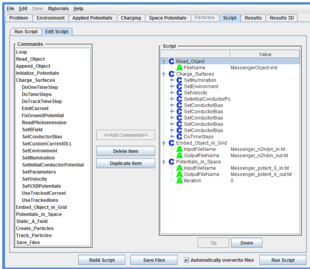
Figure 183. Edit Script Subtab of Script Tab Showing “Save Files” Button at the Bottom of the Screen
