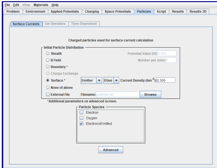
Figure 155. Particles Tab Specification for Emitter Electrons.
