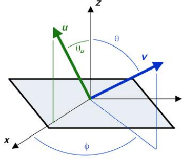
Figure 8. Coordinate System Used for Convected Maxwellian Environment, in Spacecraft Frame.
