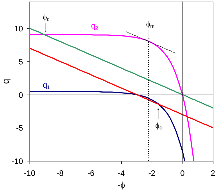
Figure 21. Plots of Space Charge (Curves q_1 and q_2 ) as a Function of Potential as Given by Equation (167). The Straight Lines Represent the Maximum Allowable Charge for Non-oscillatory Potentials. The “Natural” Space Charge, q_1 or q_2 is Acceptable for Cases for Which Slopes of the Curves and the Corresponding Line Are Equal.
