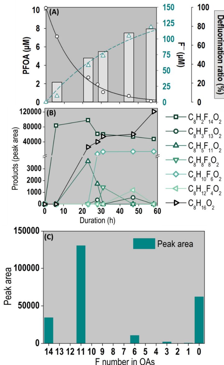
Figure 36. (A) Concentrations of PFOA and F - released in the batch test of catalytic reductive defluorination of ~10-μM PFOA in the MCfR with 5-mM Pd 0 NPs at pH ~ 4 with H 2 of 20 psig. (B) Products detected in the bulk liquid. (C) Compounds adsorbed on the Pd surface.
