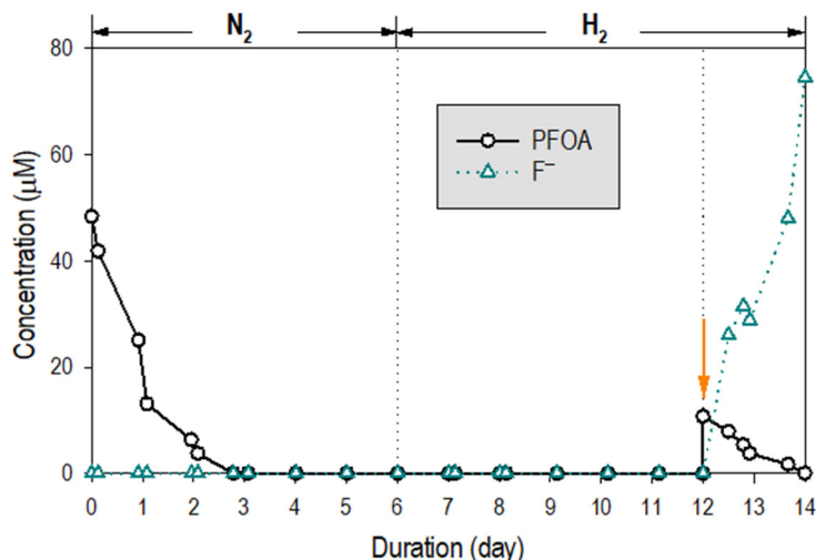
Figure 34. PFOA and \text{F}^- concentrations over time in the extended batch test for 0.9 \text{ g/m}^2 \text{ Pd}^0 at pH 4 in the MCfR supplied with 20 psig \text{N}_2 for 6 days followed by 20 psig \text{H}_2 for 8 days. The orange arrow refers to PFOA re-spiking into the liquid in the MCfR on day 12.
