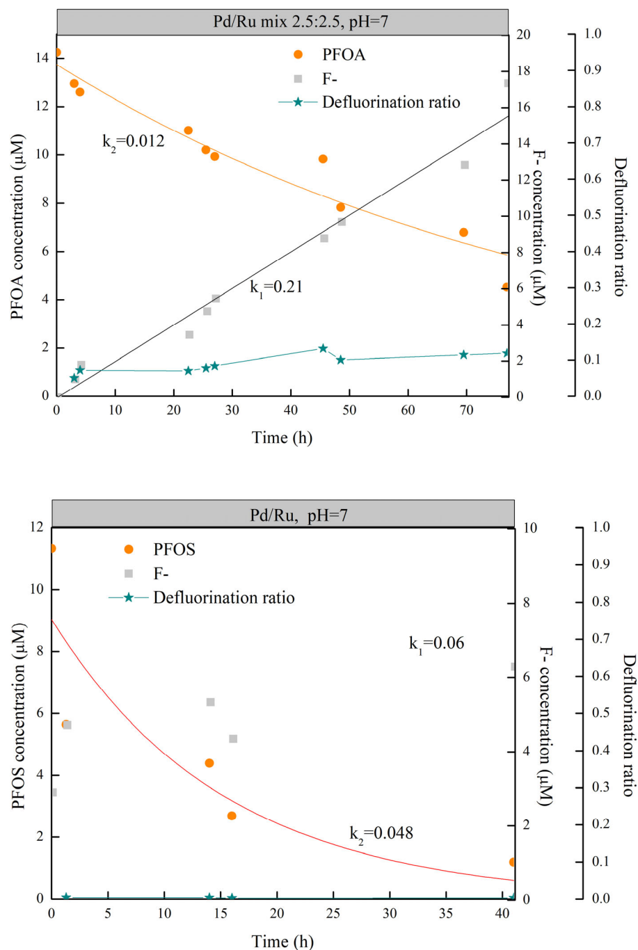
Figure 22. Concentrations of PFOA, PFOS, and F^- released and defluorination ratio in the batch test of catalytic reductive defluorination in the MCfRs with 2.5/2.5-mM Pd^0/Ru^0 NPs at pH \sim 7 with H_2 of 20 psig. (A) 10-μM PFOA (B) 10-μM PFOS.
