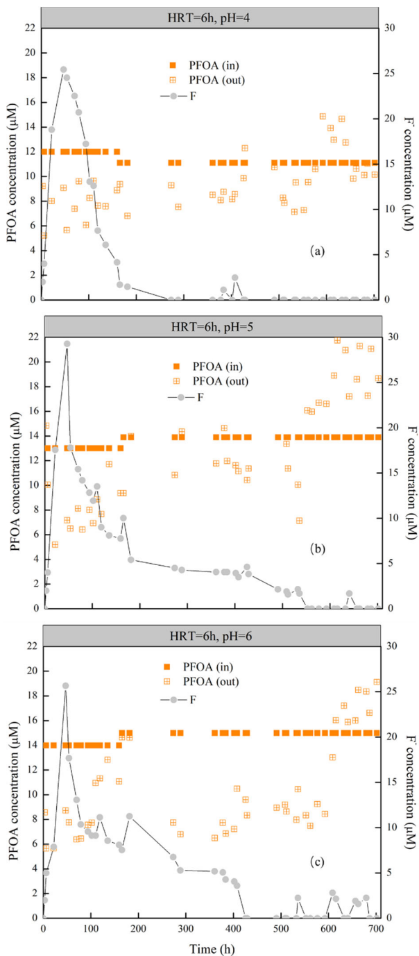
Figure 39. Concentrations of PFOA and F^- released in the continuous operation of catalytic reductive defluorination of \sim 10\text{-}\mu M PFOA in the MCfR with 5-mM Pd^0 NPs at pH \sim 4 (a), pH \sim 5 (b), pH \sim 6 (c) with H_2 supplied at 20 psig.
