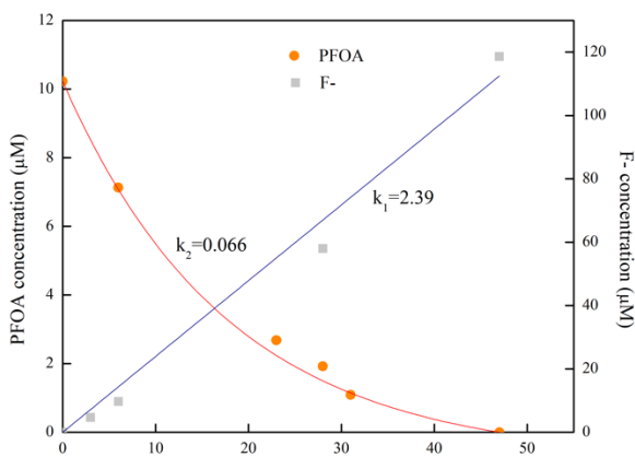
Figure 17. Concentration of PFOA and F - released in the batch test of catalytic reductive defluorination of \sim 10\text{-}\mu\text{M} PFOA in the MCfR with 1.2\text{ g-Pd}^0/\text{m}^2 at pH 4 with H 2 supply at 20 psig.
