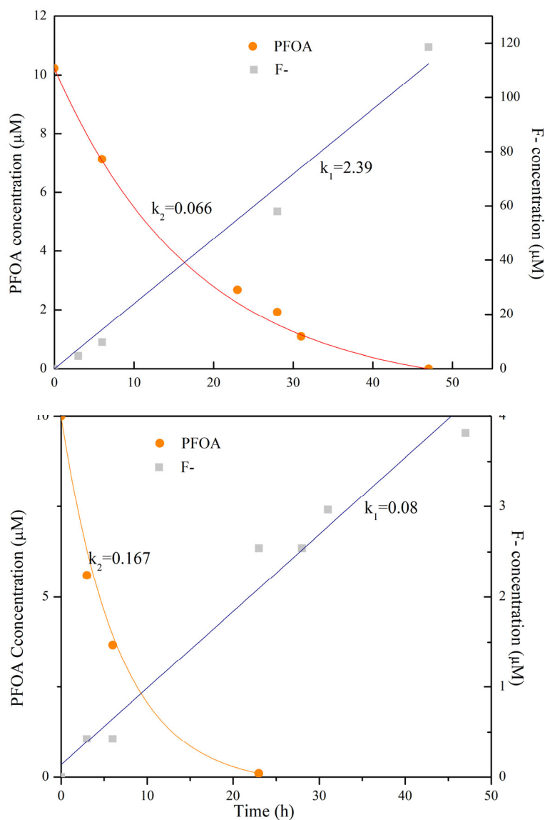
Figure 10. Concentrations of PFOA and \text{F}^- released in the batch test of catalytic reductive defluorination of \sim 10\text{-}\mu\text{M} PFOA in the MCfR with 1.2\text{ g/m}^2 or 11\text{ mM/m}^2 \text{Pd}^0 at pH 4 (top) and 7 (bottom) with \text{aH}_2 supplied at 20 psig.
