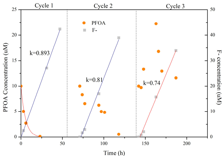
Figure 8. Concentration of PFOA and F - release in series batch tests of catalytic reductive defluorination of ~10-μM PFOA in the MCfR at pH ~ 6 with H 2 of 20 psig. Orange dots: PFOA in the H 2 -MCfR; Grey squares: F - in the H 2 -MCfR. Zero-order rate coefficients for F - release (k) are in units of μM/h.
