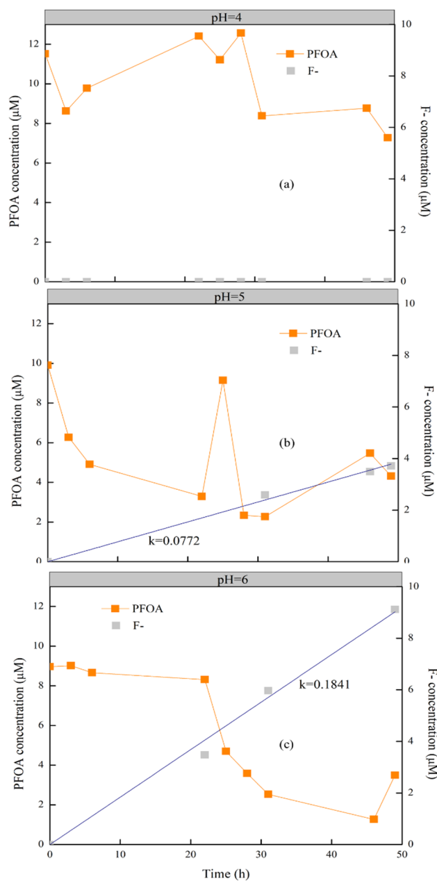
Figure 41. Concentrations of PFOA and F - released in the batch test of catalytic reductive defluorination of ~10-μM PFOA in the MCfR with 5-mM Pd 0 NPs at pHs 4 (a), 5 (b), and 6 (c) with H 2 supplied at 20 psig.
