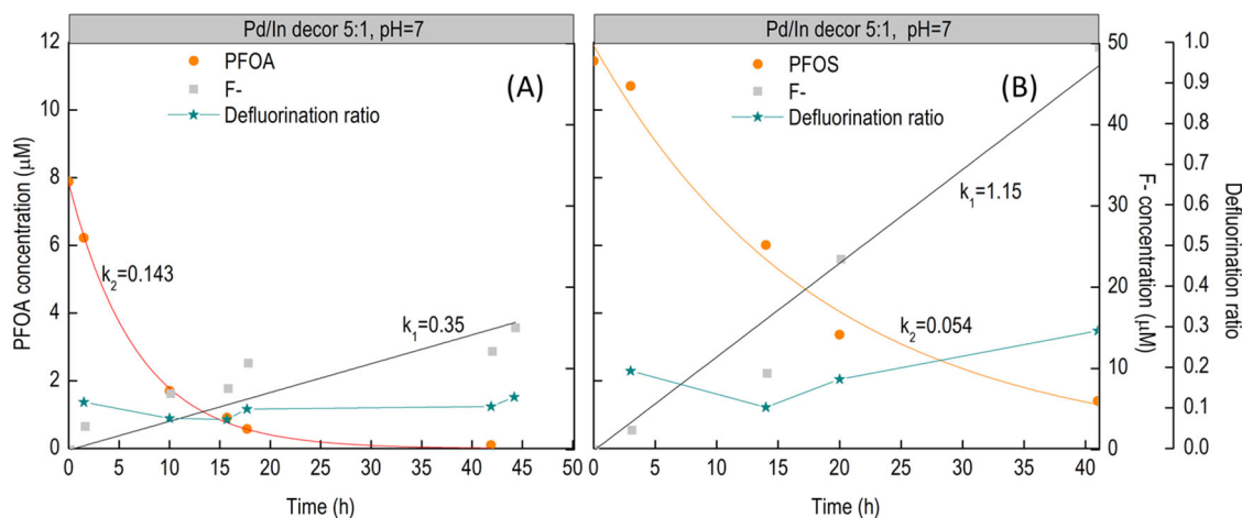
Figure 29. Batch tests of catalytic reductive defluorination of 10- \mu\text{M} PFOA (A) and 10- \mu\text{M} PFOS (B) in the MCFRs with 5/1-mM Pd 0 /In 0 NPs, pH \sim 7, and 20 psig H 2 supply.
