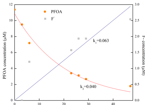
Figure 18. Concentration of PFOA and F - released in the batch test of catalytic reductive defluorination of \sim 10\text{-}\mu\text{M} PFOA in the MCfR with 2.3\text{ g-Pd}^0/\text{m}^2 at pH 4 with H 2 supply at 20 psig.
