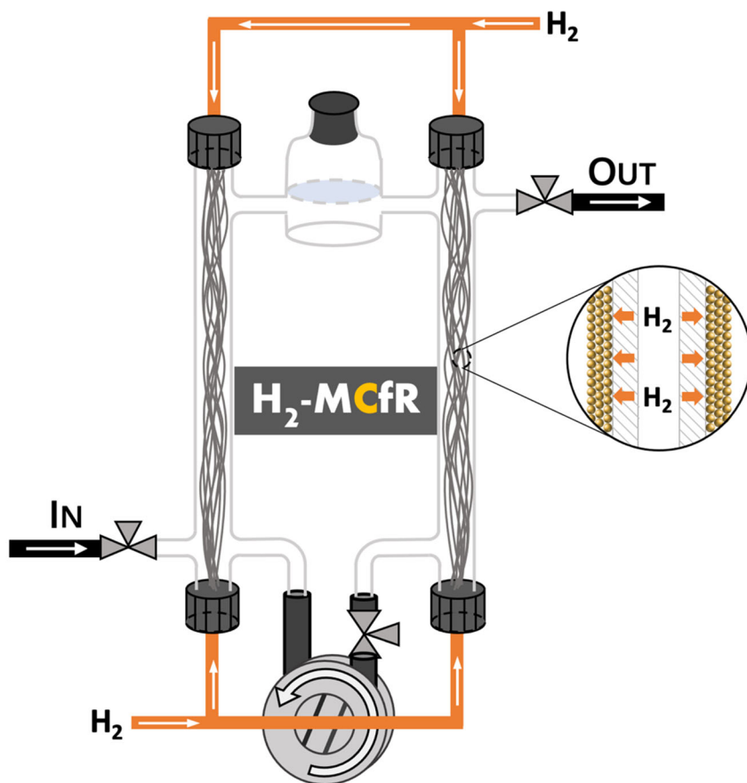
Figure 1. Schematic of the \text{H}_2 -MCfR (from Luo et al. (2021))
