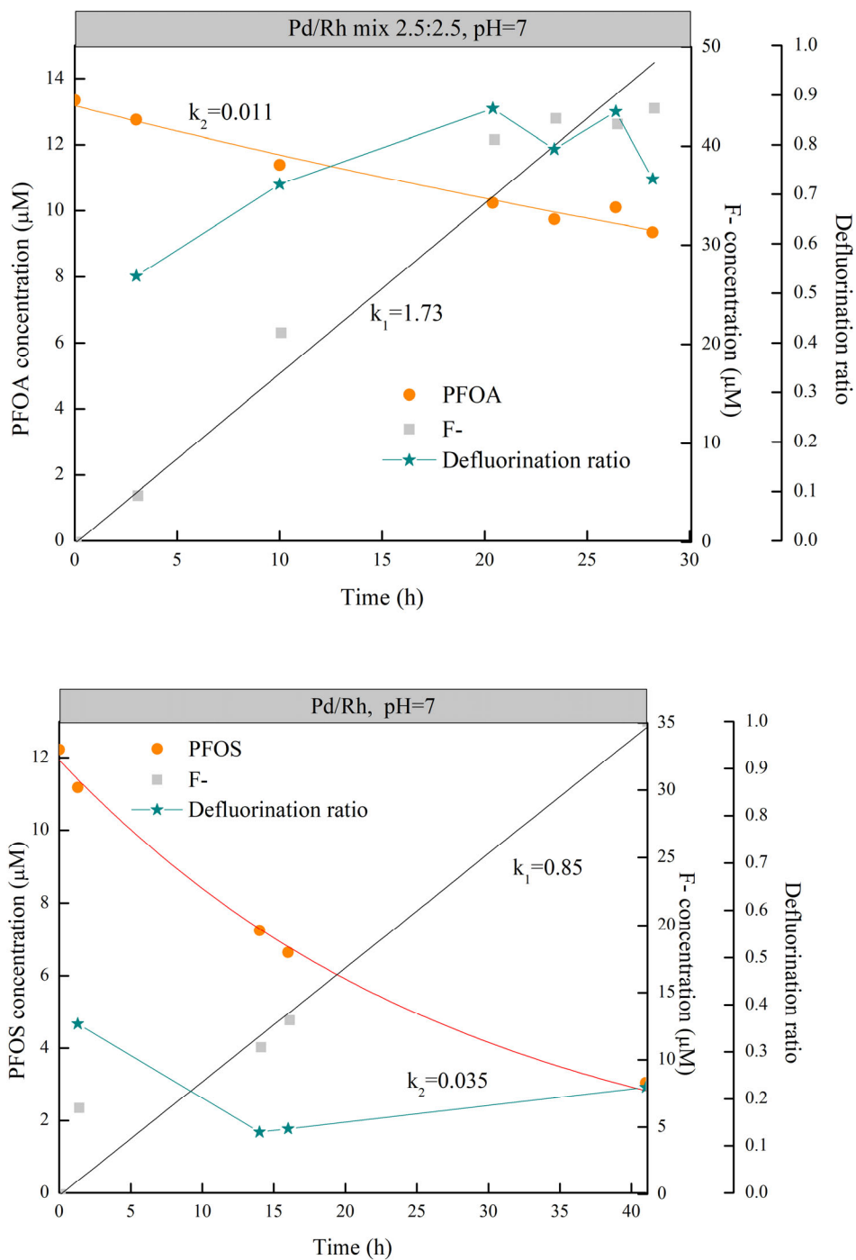
Figure 21. Concentrations of PFOA, PFOS, and F - released and defluorination ratio in the batch test of catalytic reductive defluorination in the MCfRs with 2.5/2.5-mM Pd/RhNPs at pH ~ 7 with H 2 of 20 psig. (A) 10-μM PFOA (B) 10-μM PFOS.
