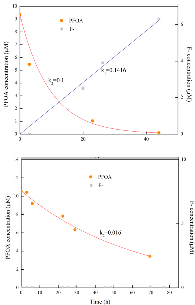
Figure 12. Concentrations of PFOA and F^- released in the batch test of catalytic reductive defluorination of \sim 10\text{-}\mu\text{M} PFOA in the MCfR with 11\text{ mM/m}^2\text{ Ru}^0 at pH 4 (top) and 7 (bottom) with H_2 supplied at 20 psig.
