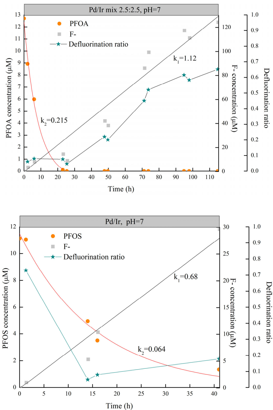
Figure 24. Concentrations of PFOA, PFOS and F^- released and defluorination ratio in the batch test of catalytic reductive defluorination in the MCfRs with 2.5/2.5-mM Pd^0/Ir^0 NPs at pH \sim 7 with H_2 of 20 psig. (A) 10- \mu M PFOA (B) 10- \mu M PFOS.
