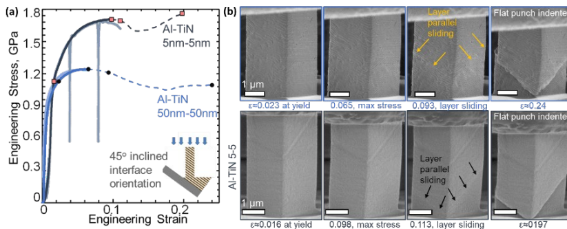
Fig 21. (a) Stress-strain response of Al(50nm)-TiN(50nm) and Al(5nm)-TiN(5nm) multilayer nanolaminate in 45° (45° inclined interface orientation) loading conditions. (b) SEM micrograph of pillars showing the deformation at different strain levels.
