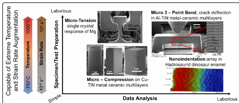
Fig 1. Overview of expanded testing capabilities of the Alemnis in-situ micro-mechanical system. Insets show FIB fabricated 3D test geometries for micro-compression, micro-tension, and micro 3 pt. bend showing crack deflection in layered composites.
