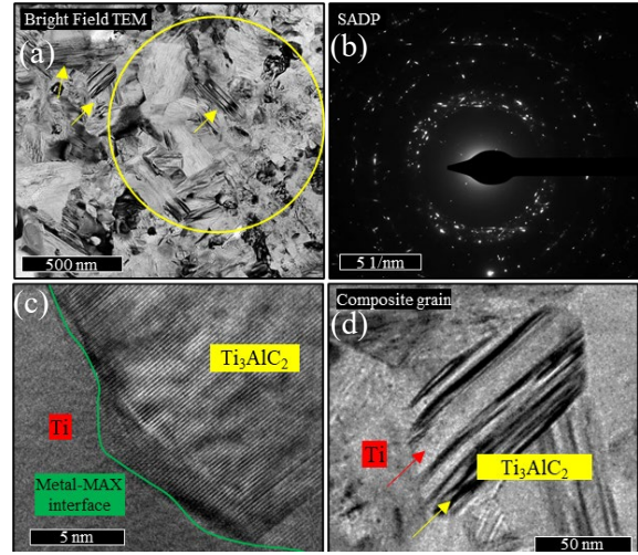
Fig 5. Bright field TEM (a) showing nanocrystalline grain structure with associated selective area diffraction pattern (SADP) (b). Region showing Ti and MAX Ti 3 AlC 2 nanocomposite (c) as well as Ti-Ti 3 AlC 2 nanocomposite grain (d)
