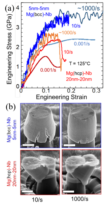
Fig 13. (a) Micropillar compression of 5 – 5 nm Mg-Nb multilayers and 20 – 20 nm Mg-Nb multilayers low to high strain rates at elevated temperatures of 125^\circ\text{C} . (b) SEM micrographs of post deformed micropillars
