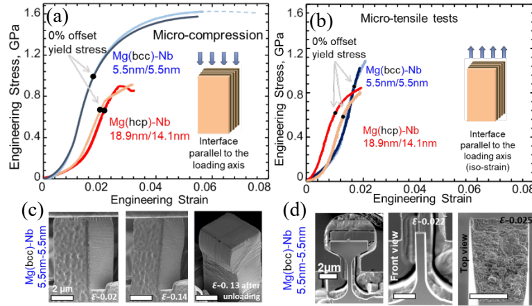
Fig 15. Stress-strain plots in microcompression (a) and microtension (b) of the 5.5 – 5.5 nm Mg-Nb and 18.9 – 14.1 nm Mg-Nb multilayers with insets showing the loading schematic of the layers. SEM micrographs of the 5.5 – 5.5 nm Mg-Nb multilayers at various strains during microcompression (c) and microtension (d)
