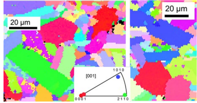
Fig 2. Electron backscattered diffraction maps of different areas on the Ta 2 AlC sample. The inset IPF triangle indicates the selected orientations from both maps.
