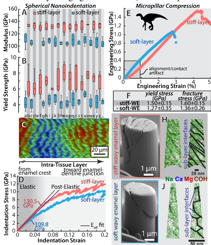
Fig 25. Combined structure-property maps of (A) elastic (modulus) and (B) plastic (indentation yield strength) of WE. (C) Optical profilometry of WE. (D) Representative indentation stress-strain responses from alternating harder (stiffer) and softer WE tissue layers. (E, F, G, I) Fracture response of harder and softer tissue layers of WE using in-situ SEM micro-compression testing. (H, J) APT results from harder and softer WE layers showing sub-layer interfaces.
