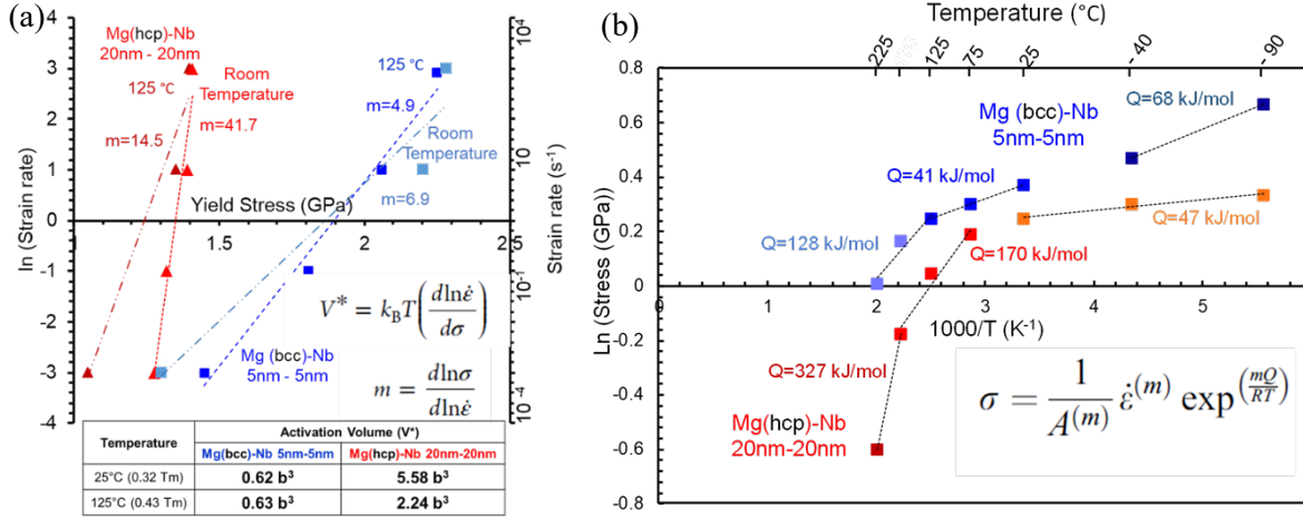
Fig 14. Normalized strain rate vs yield stress plot with calculated SRS values at room temperature and elevated temperatures of 125°C (a). Normalized yield stress vs. normalized inverse temperature plot with determined the activation energy values (b)
