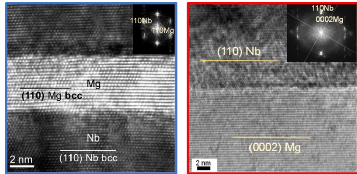
Fig 11. High resolution TEM images of the 5.5 – 5.5 nm Mg-Nb multilayer (a) and 35 – 35 nm Mg-Nb multilayers. Insets represent the associated FFT.
