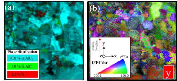
Fig 6. Precession electron diffraction map showing the phase distribution (a) and orientation (b) of Ti 3 AlC 2 in a local region)
