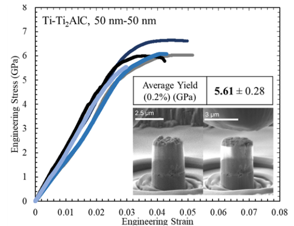
Fig 7. Stress-strain response of Ti-Ti n+1 AlC n nanocomposite. Inset shows pillar compression before and after compression before catastrophic failure.
