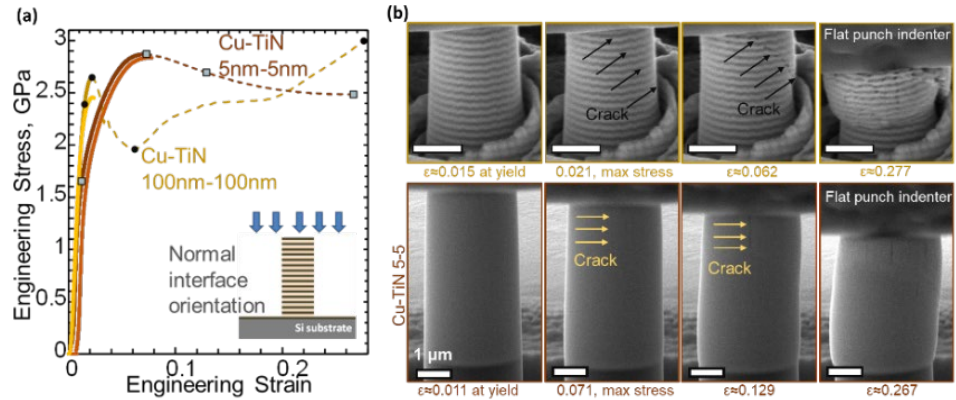
Fig 17. (a) Stress-strain response of Cu(100nm)-TiN(100nm) and Cu(5nm)-TiN(5nm) multilayer nanolaminate in normal (Normal interface orientation) loading conditions. (b) SEM micrograph of pillars showing the deformation at different strain levels.
