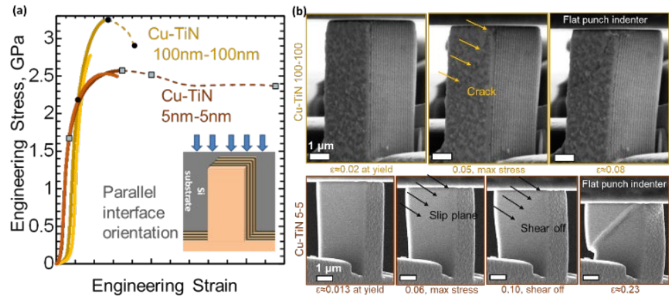
Fig 18. (a) Stress-strain response of Cu(100nm)-TiN(100nm) and Cu(5nm)-TiN(5nm) multilayer nanolaminate in parallel (parallel interface orientation) loading conditions. (b) SEM micrograph of pillars showing the deformation at different strain levels.
