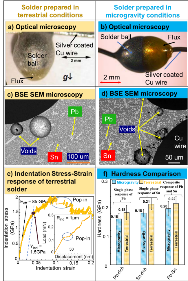
Fig. 22. Comparison of the structure and properties of terrestrial vs. microgravity Pb-Sn solders using (a, b) optical microscopy vs. (c, d), backscattered electron (BSE) maps and (e, f) local property information using indentation analysis.
