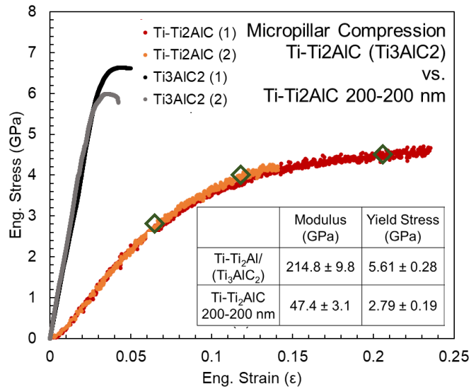
Fig 10. Stress-strain plot comparing the two Ti-Ti 2 AlC deposited nanocomposite and nanolaminate systems. Square indicators represent breakpoints for the different regions in the curves
