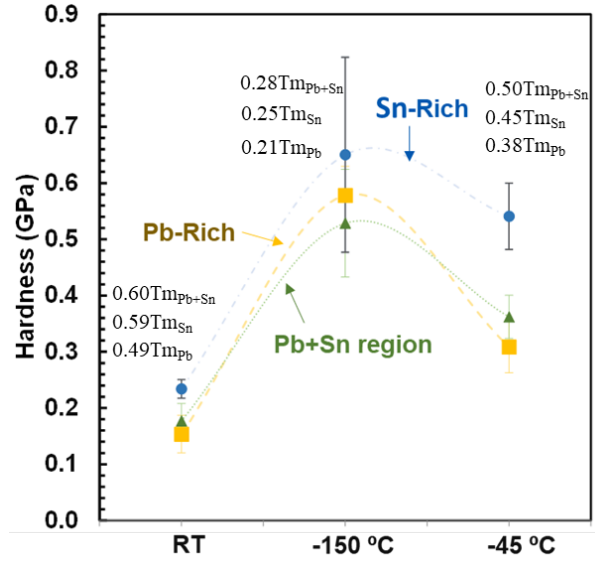
Fig 24. Hardness response from Pb-rich phase, Sn-rich phase and Pb+Sn regions obtained from in-Situ SEM nanomechanical testing at RT, -45°C, -150°C. Hardness from different regions increases with decreasing the temperature below the room temperature.
