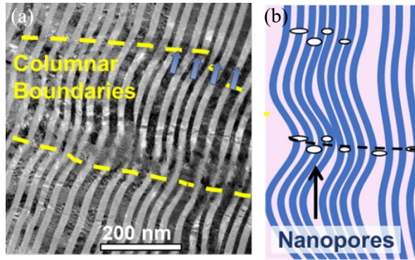
Fig 16. Bright field TEM of the 18.9 – 14.1 nm Mg-Nb multilayers (a) showing waviness and columnar boundaries. A schematic showing nanopores associated with the columnar boundaries (b)
