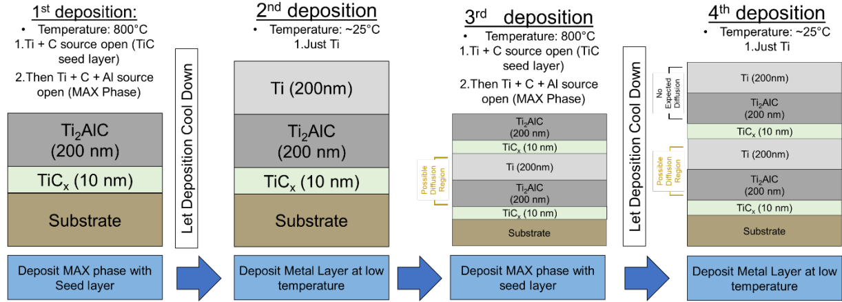
Fig 8. Schematic and process flow of the 4-step deposition of Ti-Ti 2 AlC system incorporating a TiC seed layer and deposition cooldown steps between the depositions to minimize diffusion.
