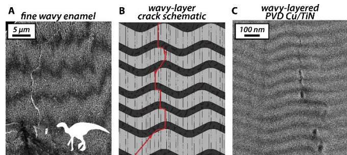
Fig 26. (A) Experimental results and (B) schematic of crack deflection in hadrosaurid WE, which inspired our (C) PVD deposited wavy 50nm-50nm metal-ceramic Cu-TiN multilayers. showing crack undulation (strain energy loss) and controlled crack propagation along the waviness between the layers.
