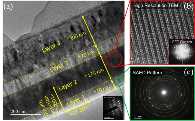
Fig 9. Bright-field TEM showing the microstructure of the film (a). High resolution TEM shows the signature lattice fringe structure for MAX phase (b), and SAED pattern shows the nanocrystalline nature of the film with slight texture (c).
