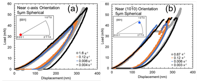
Fig 3. Load vs. displacement curves of nanoindentation at different strain rates using a 5 μm radius spherical tip on an orientation near parallel (a) and near perpendicular (b) to the basal orientation of Ta 2 AlC.
