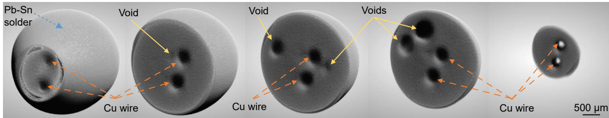
Fig 23. 3-D distribution of voids in microgravity Pb-Sn solder using micro-computed tomography.
