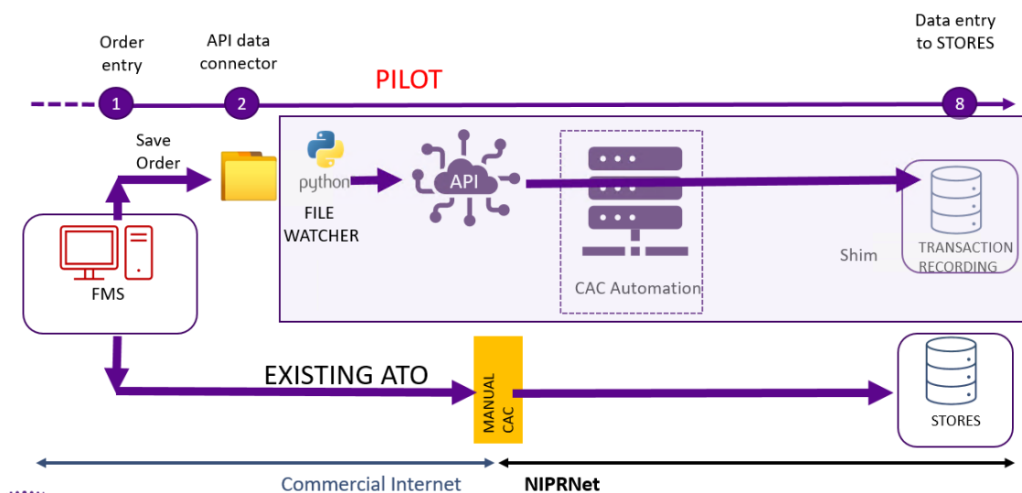
Figure 26: Computation Solution Architecture
