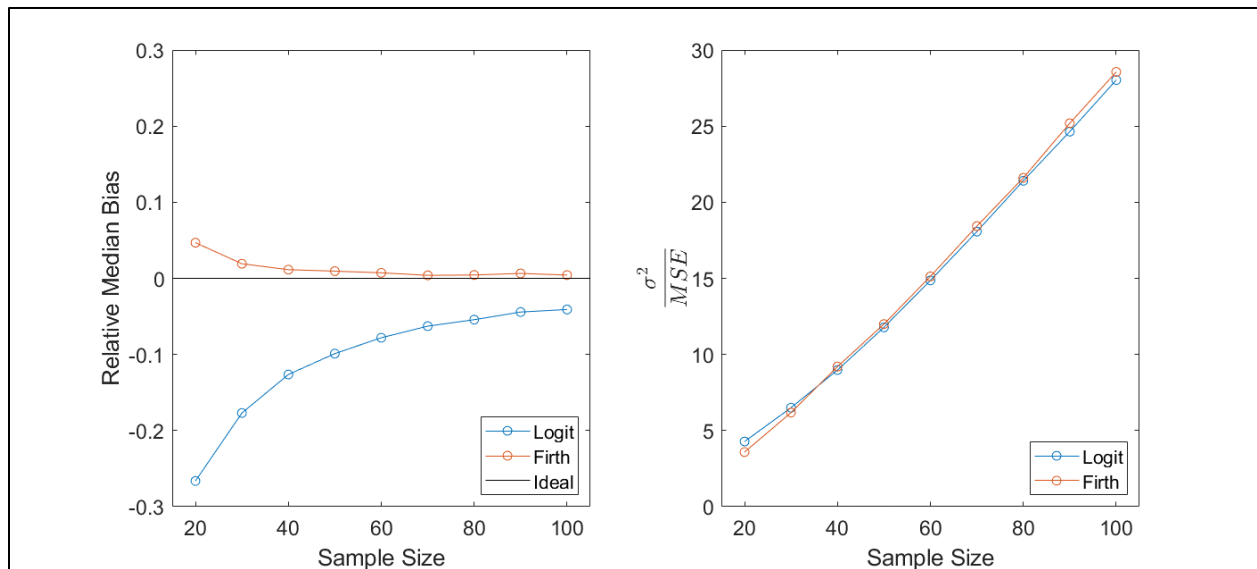
Figure 23. Relative median bias and MSE for sigma
