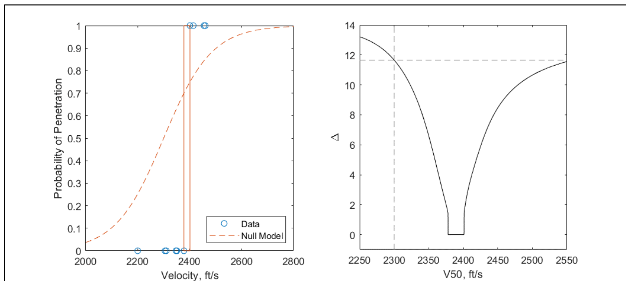
Figure 5. Example of the one-sample LRT on V50 with separation.
