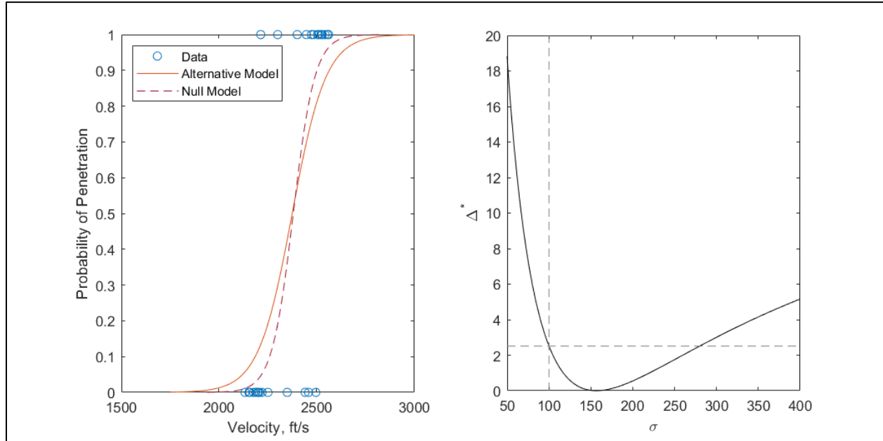
Figure 15. Example of one-sample PLRT on sigma.
