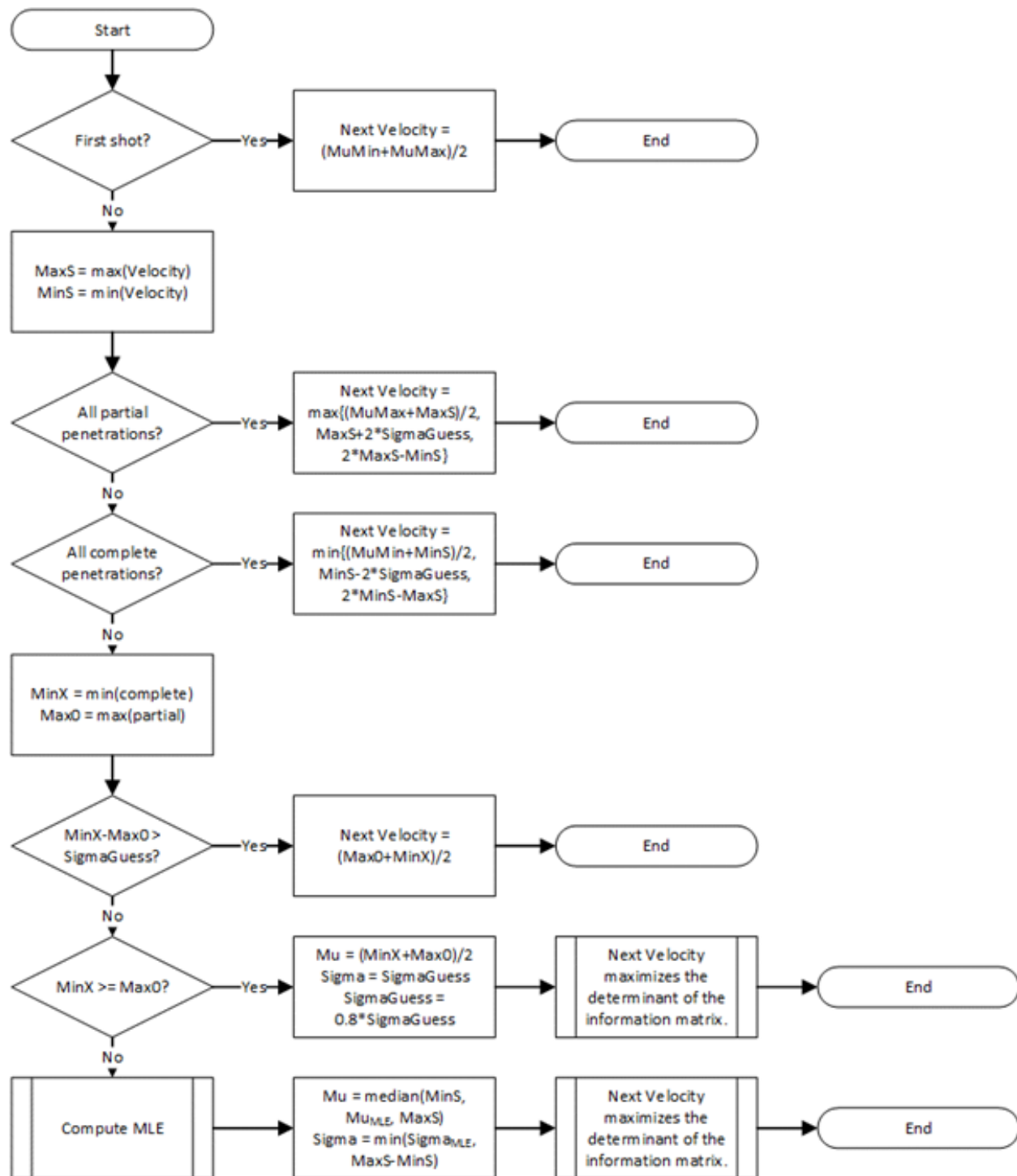
Figure 2. Flow chart for the Neyer D-Optimal Method.
