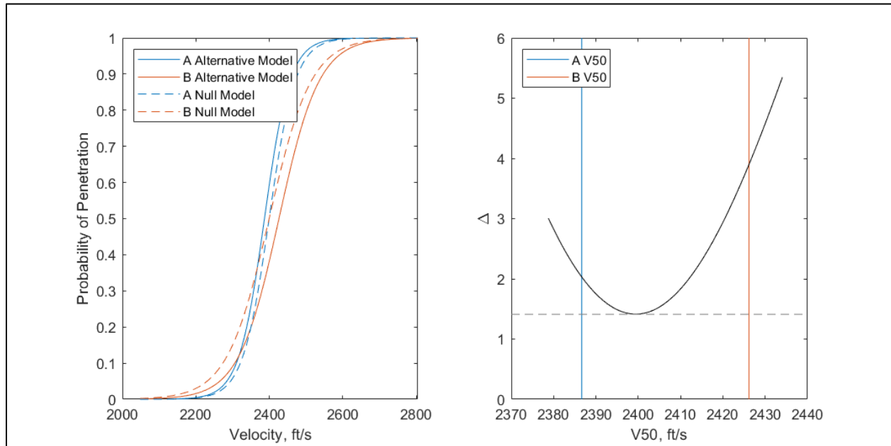
Figure 6. Example of the two-sample LRT on V50.
