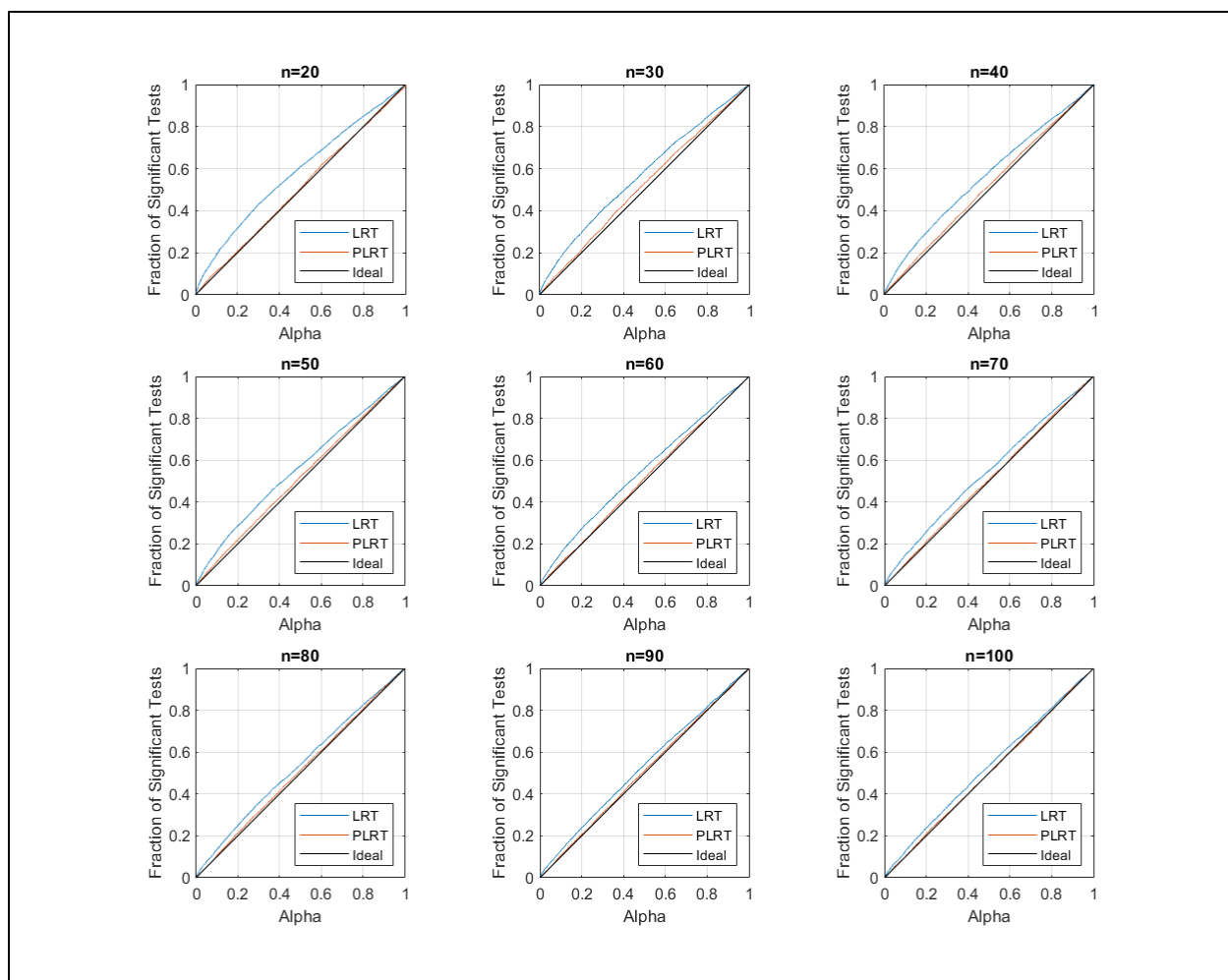
Figure 28. Q-Q plot for two-sample test on V10.
