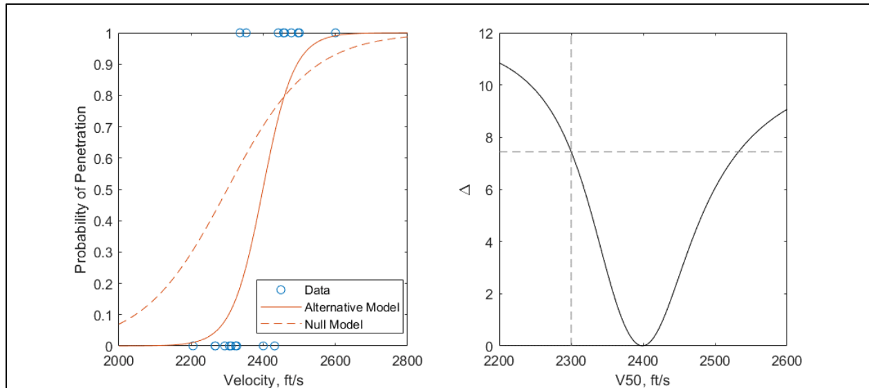
Figure 4. Example of the one-sample LRT on V50.
