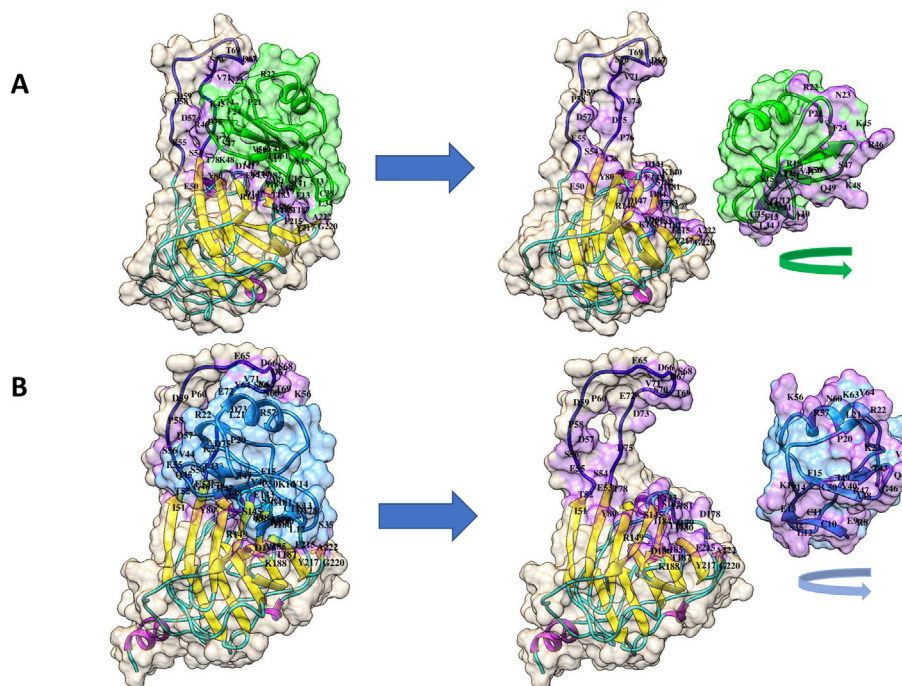
Fig. 3 Interface of vCCI and its chemokine ligands as predicted by molecular dynamics simulations. The surface area is shown for (A) vCCI when bound to CCL4 and (B) vCCI when bound to CCL17. The structure used in A comes from the PDB ID 2FFK [31], in which the CCL4 ligand was mutated back to wildtype and molecular dynamics was run for 1 \mu s. In B, the vCCI:CCL17 structure was built by modeling the complex, starting with 2FFK and replacing the chemokine by aligning the C \alpha backbone. To visualize the intermolecular interactions, each component has been moved apart and rotated to reveal the binding face. vCCI (beige) is on the left, the chemokine ligand is on the right (green for the CCL4, blue for CCL17). The contact surface area between vCCI and each chemokine is colored in purple. The residues involved in the interface on both vCCI and the chemokine are labeled. Contact surface area identified on the CCL17 \alpha helix suggests non-canonical binding with the vCCI acidic loop compared to other chemokines.
