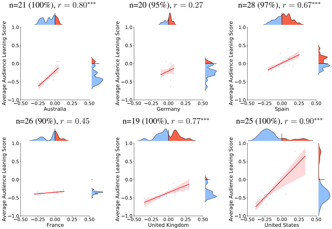
Figure 16: Correlation between our average audience leaning score(y-axis) versus those from [44] (x-axis). We use Pearson’s r correlation test. *** P < 0.001 . n=xx shows the number of overlapped domain with [44], ( xx\% ) is the coverage of all domains from [44]. For domains shared in multiple countries, we calculate the average leaning scores in each country independently.
