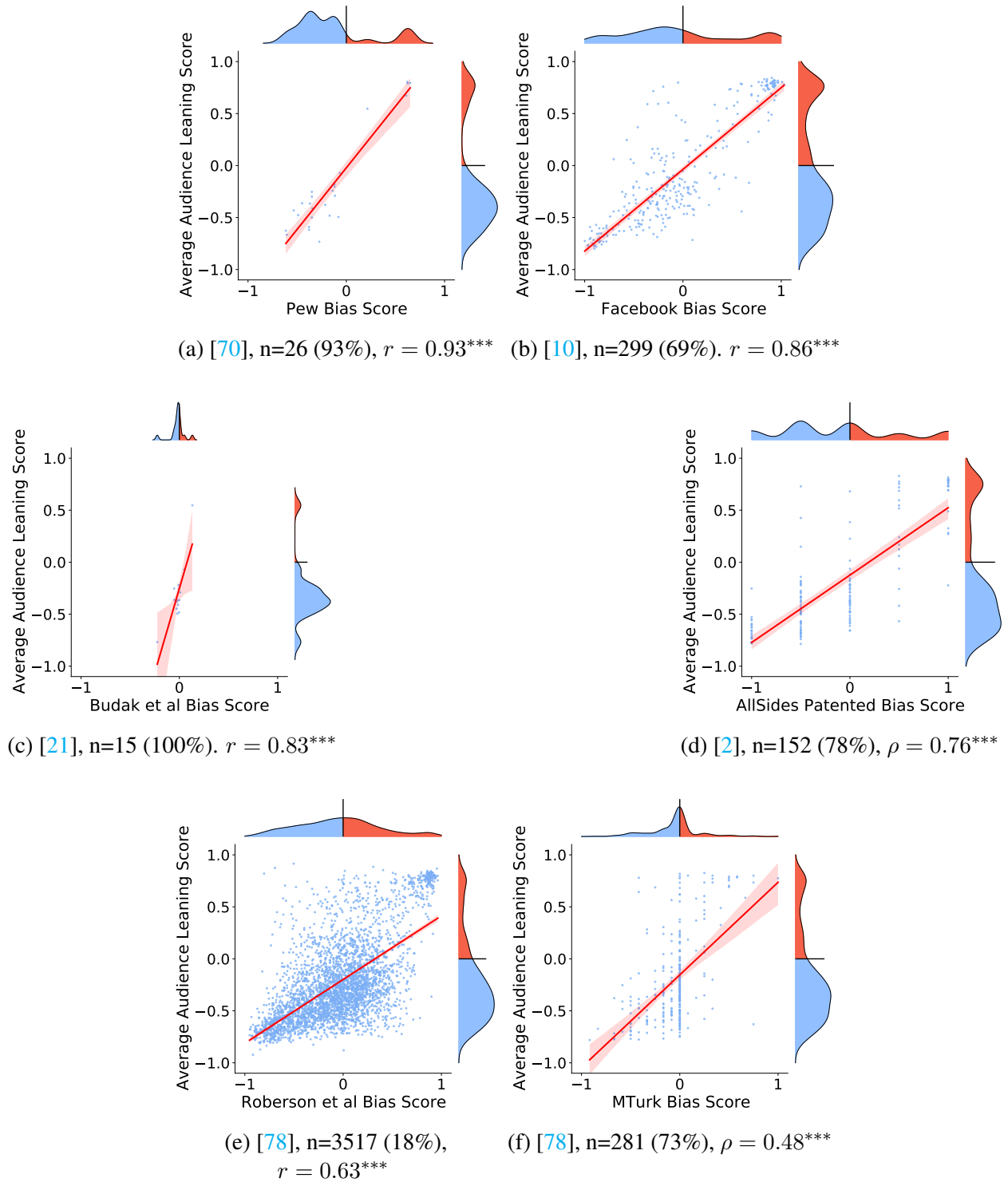
Figure 14: Correlation between average audience leaning from our data versus bias scores from other sources, each with “[reference], n =number of overlapped domains (fraction covered in the other source), correlation score” – Pearson’s r for continuous scores and Spearman’s \rho for ordinal scores. *** denotes p < 0.001 . Ordered chronologically (oldest to newest) from (a)–(f). Side densities represent the distribution of domain leaning scores from either source.
