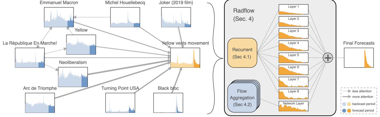
Figure 3: Overview of the Radflow model, centered around the WIKITRAFFIC subgraph of Yellow vests movement (a social movement in France since 2018, shown on the left). Each node is a page with a time series of view counts, shown in its individual mini-panel. Edge strengths correspond to average attention scores in the forecast period. The final forecast is produced by summing over the output from eight layers of the recurrent component and the network flow aggregation component (shown on the right). Radflow correctly predicts a sharp drop in traffic volume for Yellow vests movement from 3 June 2020 to 30 June 2020, due to information from neighboring nodes such as Black bloc and Turning Point USA .
