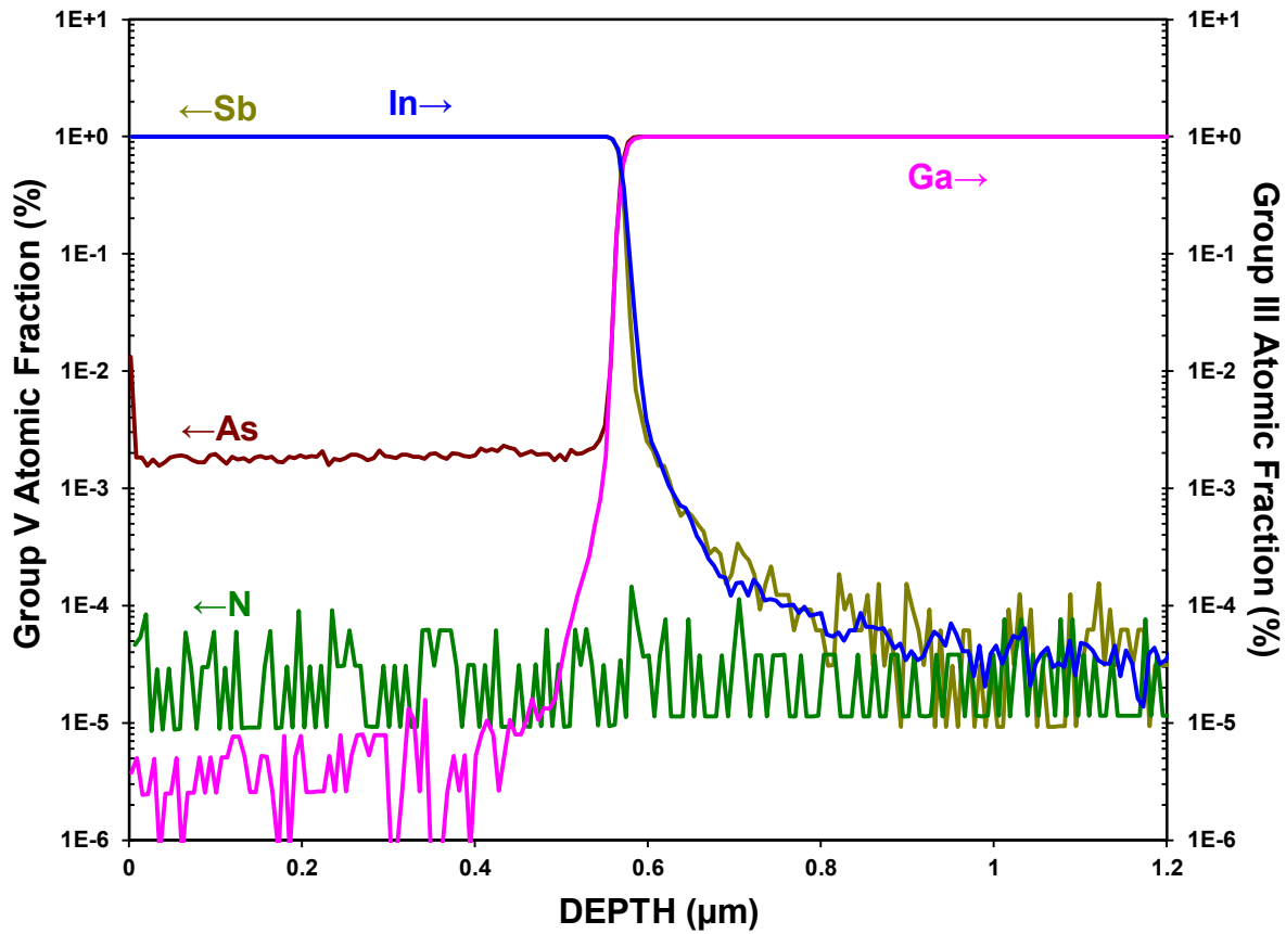
Figure 4.6. SIMS depth profile of 0.6 \mu\text{m} InSb/GaAs heterostructure.
