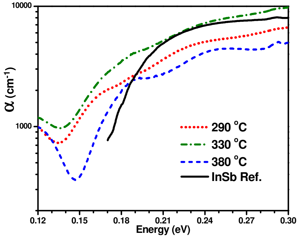
Figure 6.8. \alpha vs energy plots for InSbN epilayers grown at different temperatures compared with InSb reference. 30
