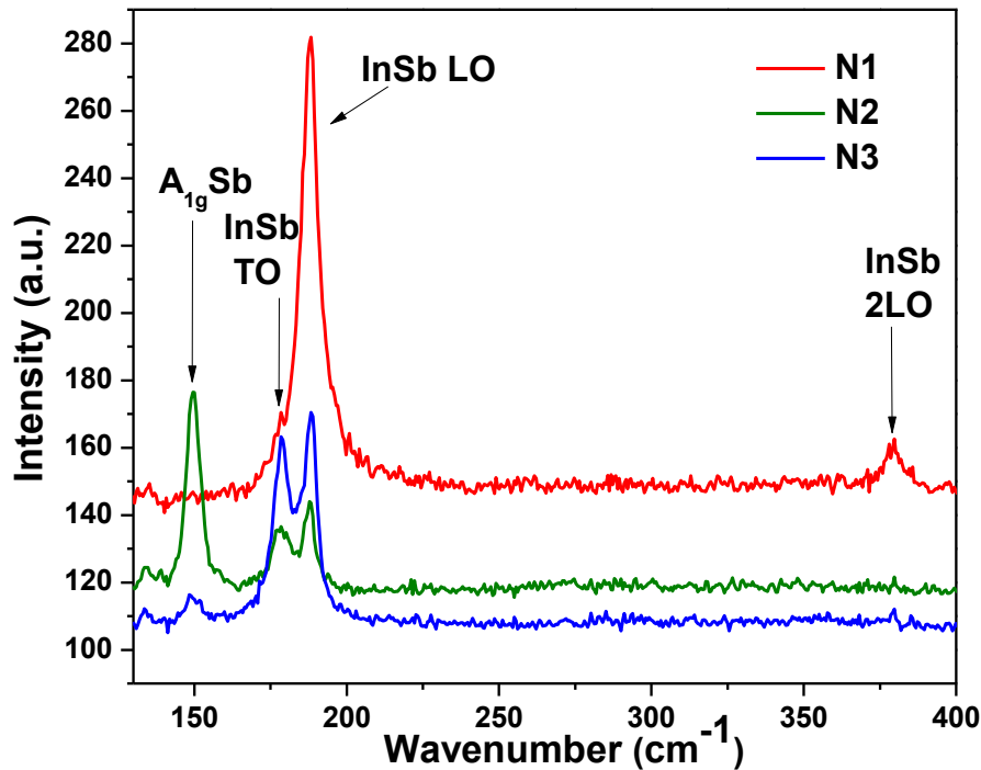
Figure 5.4. RT micro-Raman spectra of InSbN heterostructures grown under different N BEP at T_s 380\text{ }^{\circ}\text{C} .
