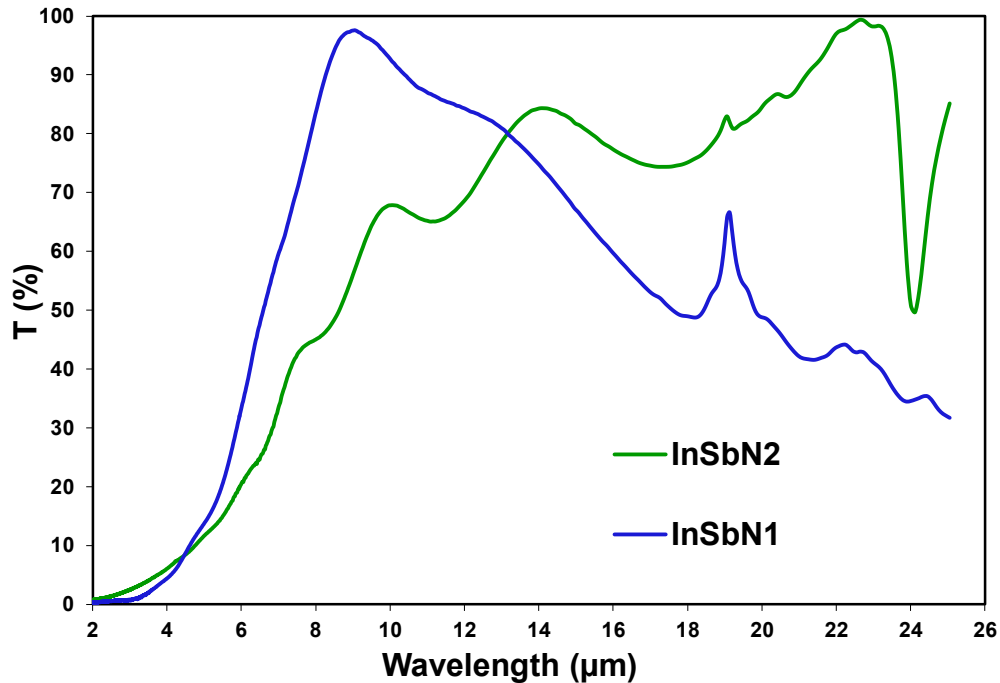
Figure 3.4. FTIR RT transmission spectrum of two InSbN heterostructures.
