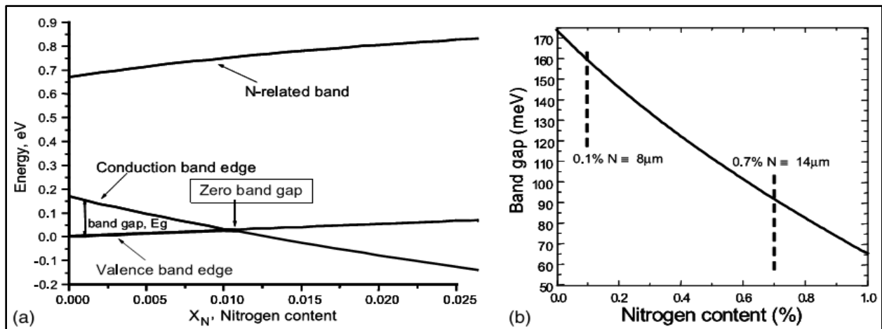
Figure 2.2. (a) the calculated band structure as a function of nitrogen composition, (b) the band gap variation over the mid to long wavelength IR range for \text{InSb}_{1-x}\text{N}_x . 21
