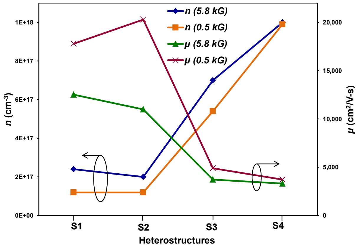
Figure 8.11. The comparison of RT n and \mu for different InSbN heterostructures measured at low and high magnetic fields.
