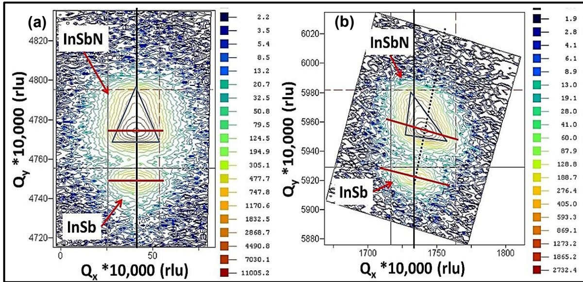
Figure 8.7. (a) (004) and (b) (115) reciprocal space maps of the heterostructure S4.
