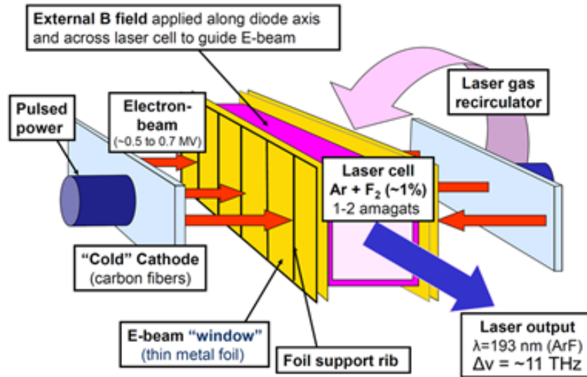
Fig. 1 — Schematic of argon fluoride (ArF) laser amplifier: Details of a modular, rep-rate, efficient ArF electron beam amplifier. Counter-propagating electron beams, from left and right, are used to create the laser gain medium, center of picture, with a gas recirculator for thermal management at high frequency operation. Picture of actual device in Fig. E1.
