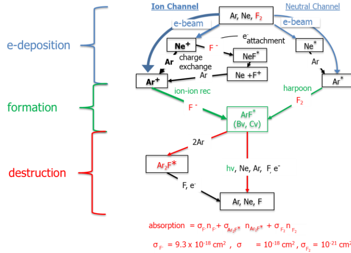
Fig. 2 — Schematic of argon fluoride (ArF) laser amplifier kinetics: Depicting the dominant reactions from both the ion channel and the neutral channel.
