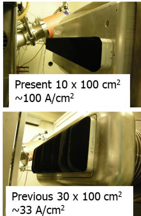
Figure 3. Modifications to the Electra electron beam laser system to allow higher current density and higher electron beam power deposition per unit volume with a cathode height reduction from 30 cm (below) to 10 cm (above).
