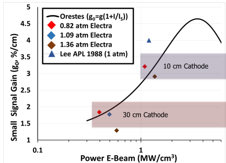
Figure 5. Measured small signal gain from the Electra facility using two different cathodes (10 cm, higher electron beam power and 30 cm, lower electron beam power). Comparison of the ArF Orestes code (solid line) with the Electra results as well as results from Lee et al. [26].
