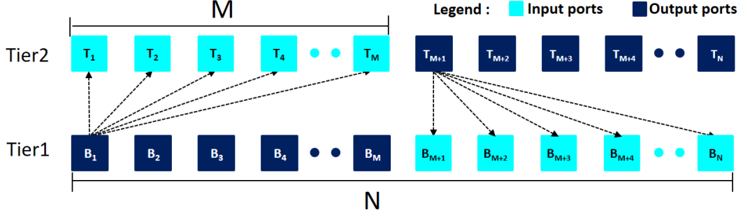
Fig. 7 Possible vertical connections between output ports in Tier1 and input ports in Tier2 and vice versa. Only connections from B_1 and from T_{M+1} are shown for clarity.
