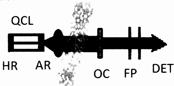
Fig. 1. (left) Schematic of Hyperdog. A LWIR QCL at room temperature has HR and AR coatings and an external cavity is formed using a collimating optic (orange) and an output-coupling flat mirror (OC). The cavity is open to the flow of target vapors (green) with characteristic sharp absorption lines. The outcoupled mode spectrum is analyzed using a scanning FP spectrometer. The signal is detected using a room temperature piezo-electric detector.
