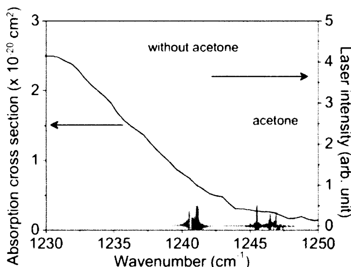
Fig 2. Emission spectrum of the external cavity QCL together with absorption cross section of acetone. The QCL was operated CW at 940 mA excitation current. The spectral resolution of the spectrometer is 0.5\text{ cm}^{-1} . Two separate laser spectra are plotted, one without, and one with acetone vapor in the cavity. When the open laser cavity is exposed to acetone vapor, the spectrum blueshifts, as indicated by the arrow.
