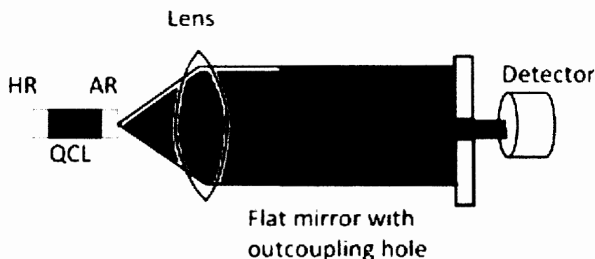
Fig 4: Schematic of external cavity QCL using a lens system.
