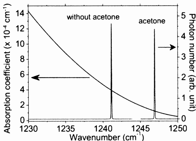
Fig 3: Calculated laser emission spectra without (left) and with (right) acetone inside the cavity. The acetone profile was quadratic with a concentration of 5.4 \times 10^{15} \text{ cm}^{-3} , or 165 mTorr pressure. The spectrum with acetone shows a clear 6 \text{ cm}^{-1} shift to higher wavenumbers.
