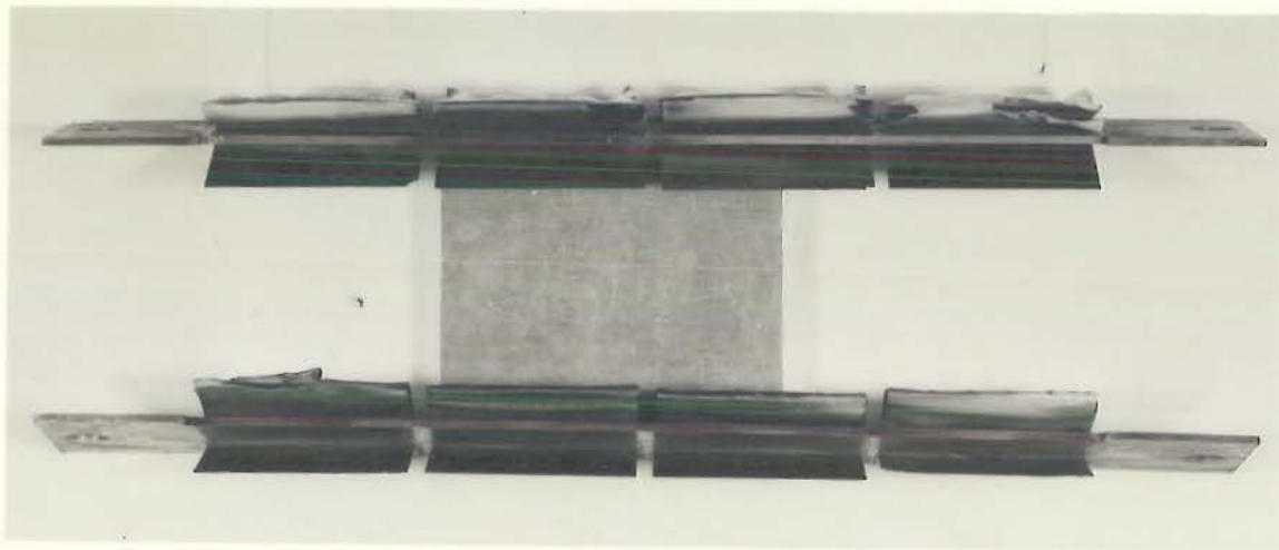
SAMPLES OF VANES PROTECTED WITH POLY-F PLASTIC TIME OF RUN 31 MIN. (.006" VANES)
