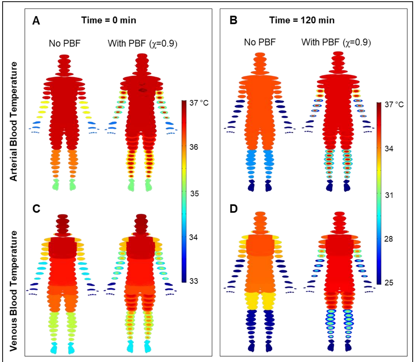
Fig. 3: Simulated spatial variation of blood temperature within the 3-D virtual human model for the extreme cold-stress condition in Study 1 (ambient temperature of 1 °C and wind speed of 0.8 m/s) at the beginning [t = 0 minutes, Panels (A and C)] and at the end [t = 120 minutes, Panels (B and D)] of the simulation. (Note that we used different color scales to illustrate the temperature distribution at the two time points.) Each of the four panels illustrates the blood temperature variation with and without the passing blood flow (PBF) mechanism for the arterial vessels (A and B) and venous vessels (C and D). Note the spatial variation of blood temperatures
