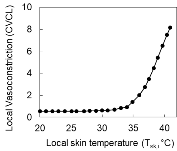
Fig. A4: Local vasoconstriction as a function of local skin temperature (22).
