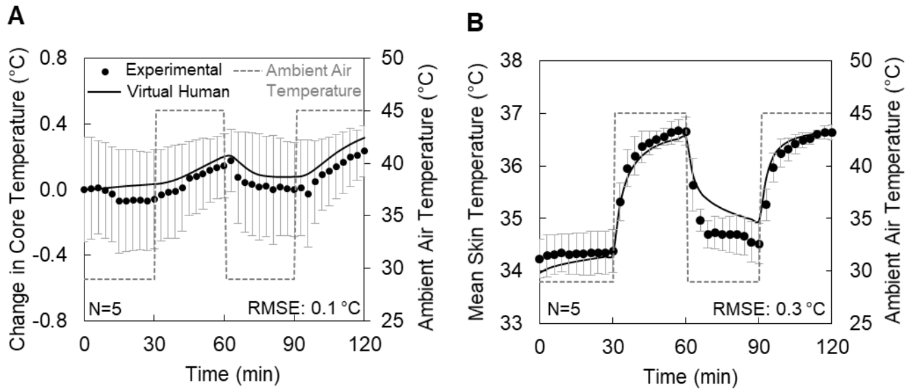
Fig. A2: Model validation of (A) the core body temperature and (B) the mean skin temperature for an environmental heat-stress study in which five subjects wearing shorts sat in an environmental chamber for 120 minutes, while the air temperature changed drastically from neutral to very hot (29 to 45 to 29 to 45 °C and 40% relative humidity) (Study 8, Table 1). The filled circles represent the average of the measured changes in core body temperature (A) or the mean skin temperature (B), the vertical gray bars indicate two standard errors of the mean, the gray dashed lines represent the ambient air temperature, and the solid black lines denote the 3-D virtual human model predictions for core body temperature change (A) or the mean skin temperature (B). RMSE: root mean squared error.
