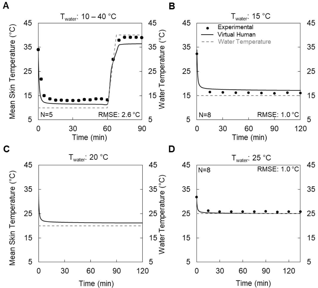
Fig. 8: Model validation of the mean skin temperature collected during water-immersion experiments in Study 5 [panel (A), very cold to very hot], Study 6 [panels (B) and (D), very cold and temperate, respectively], and Study 7 [panel (C), mild], with subjects immersed up to the neck level and sitting quietly for 90 to 135 minutes while wearing minimal clothing (Table 1). The filled circles represent the average of the measured mean skin temperature values, the dashed gray lines indicate the water temperature, and the solid black lines denote the mean skin temperatures predicted by our virtual human model. Experimental data were not available for
