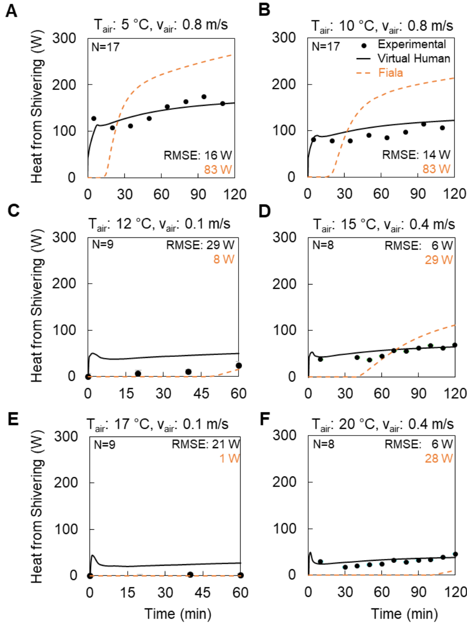
Fig. 6: Model validation of the heat generated from shivering for mild, moderate, and very cold environmental conditions in Study 2 [panels (A) and (B)], Study 3 [panels (C) and (E)], and Study 4 [panels (D) and (F)], while subjects sat quietly for 60 or 120 minutes wearing minimal clothing (Table 1). The filled circles represent the average of the measured heat generated from shivering, and the solid black lines denote the changes predicted by the virtual human model.
