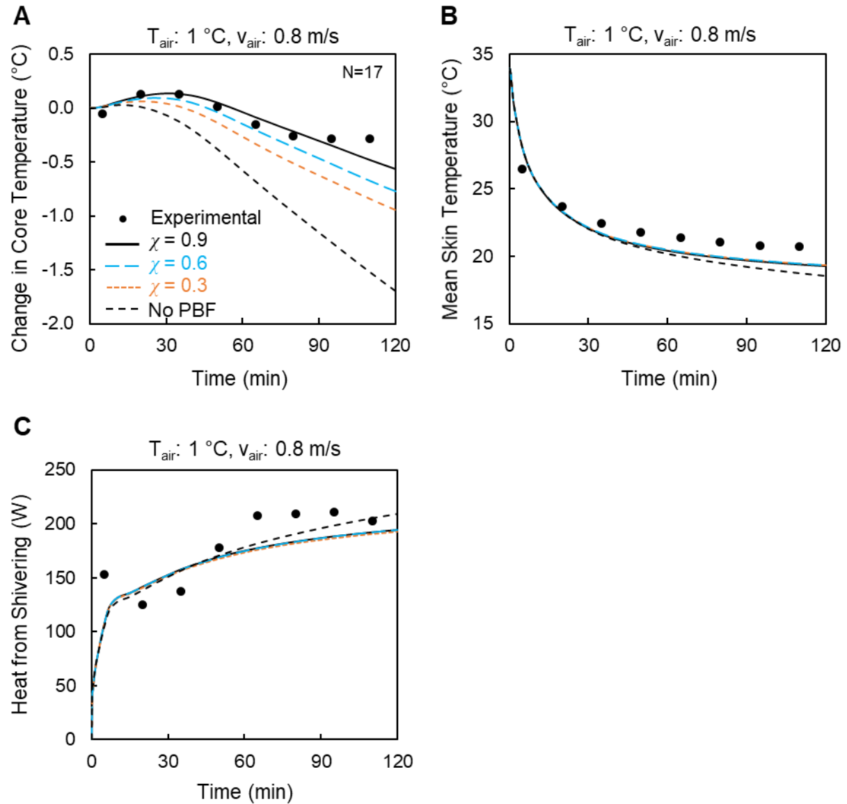
Fig. 2: Model calibration to estimate the value of the passing blood flow (PBF) efficiency \chi , using data from the extreme cold-stress condition in Study 1 ( 1^\circ\text{C} ambient temperature T_{\text{air}} and 0.8\text{ m/s} wind speed v_{\text{air}} , Table 1). Shown are the average values of the experimental data along with the model-predicted (A) changes in core body temperature, (B) mean skin temperature, and (C) heat generated from shivering, as a function of different values of \chi (0.3, 0.6, and 0.9), as well as predictions without the PBF mechanism. Experimental measurement uncertainty was not available for Study 1.
