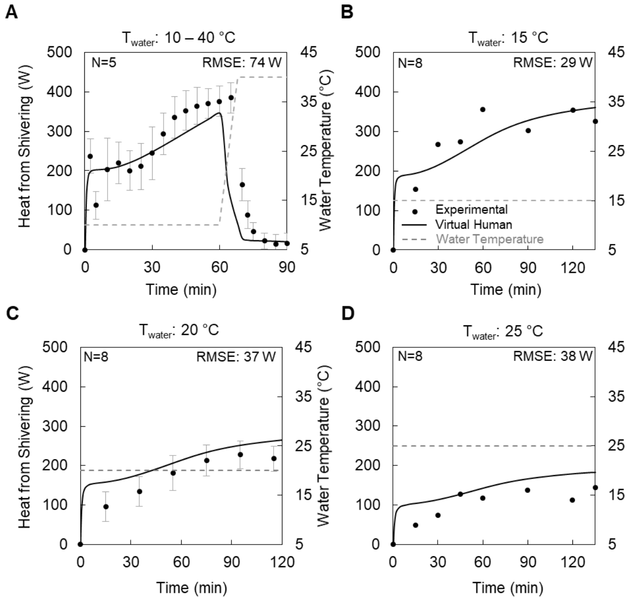
Fig. 9: Model validation of the heat generated from shivering collected during water-immersion experiments in Study 5 [panel (A), very cold to very hot], Study 6 [panels (B) and (D), very cold and temperate, respectively], and Study 7 [panel (C), mild], with subjects immersed up to the neck level and sitting quietly for 90 to 135 minutes while wearing minimal clothing (Table 1). The filled circles represent the average of the measured heat generated from shivering, the vertical gray bars indicate two standard errors of the mean (not available for Study 6), the dashed gray lines indicate the water temperature, and the solid black lines denote the heat generated
