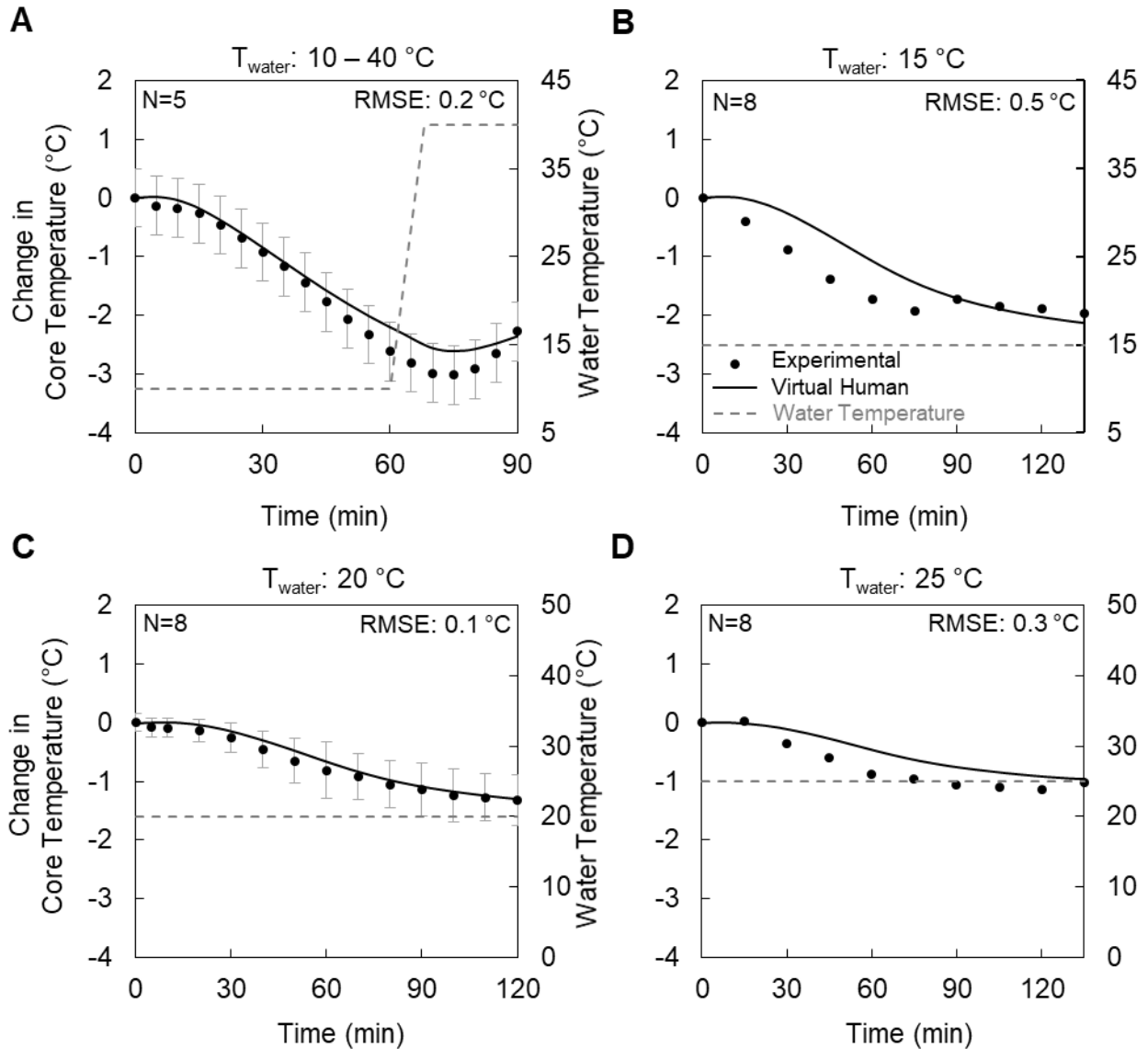
Fig. 7: Model validation of the changes in core body temperature collected during water-immersion experiments in Study 5 [panel (A), very cold to very hot], Study 6 [panels (B) and (D), very cold and temperate, respectively], and Study 7 [panel (C), mild], with subjects immersed up to the neck level and sitting quietly for 90 to 135 minutes while wearing minimal clothing (Table 1). The filled circles represent the average of the measured changes in core body temperature values, the vertical gray bars indicate two standard errors of the mean (not available for Study 6), the dashed gray lines indicate the water temperature, and the solid black lines
