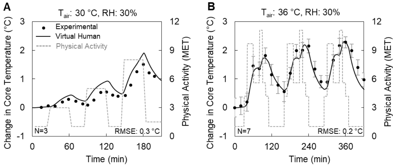
Fig. A3: Model validation of the core body temperature for two exertional and environmental heat-stress conditions in which (A) three subjects wearing shorts pedaled on a bicycle ergometer at three different intensities for 210 minutes at 30 °C and 30% relative humidity (RH) (Study 9, Table 1) and (B) seven subjects wearing a T-shirt and shorts ran on a treadmill while performing three strenuous exercise bouts of varying intensities for 420 minutes at 36 °C and 30% RH (Study 10, Table 1). The filled circles represent the average of the measured changes in core body temperature, the vertical gray bars indicate two standard errors of the mean, the gray dashed lines represent the physical activity level, and the solid black lines denote the 3-D virtual human model predictions for core temperature change. MET: metabolic equivalent; RMSE: root mean squared error; T_{\text{air}} : ambient air temperature.
