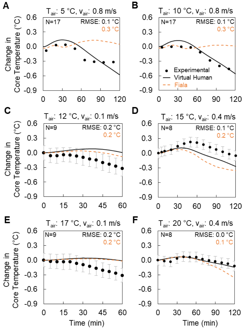
Fig. 4: Model validation of the core body temperature for mild, moderate, and very cold environmental conditions in Study 2 [panels (A) and (B)], Study 3 [panels (C) and (E)], and Study 4 [panels (D) and (F)], while subjects sat quietly for 60 or 120 minutes wearing minimal clothing (Table 1). The filled circles represent the average of the measured changes in core body temperature values, the vertical gray bars indicate two standard errors of the mean (not available
