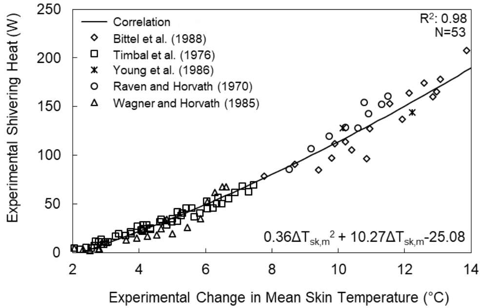
Fig. A1: Correlation between experimentally observed heat due to shivering (“shivering heat”) and changes in mean skin temperature obtained by collating experimental data from multiple cold-stress studies conducted in air (29, 49-51). This correlation was used as part of the input to the 3-D virtual human model to predict heat due to shivering for t > 30 minutes, when simulating cold-air exposures [see Eq. (11)]. Open symbols denote mean experimental values ( N = 53 ), while the solid line denotes the computed correlation function. R^2 : coefficient of determination; \Delta T_{sk,m} : change in mean skin temperature from an initial thermoneutral state.
