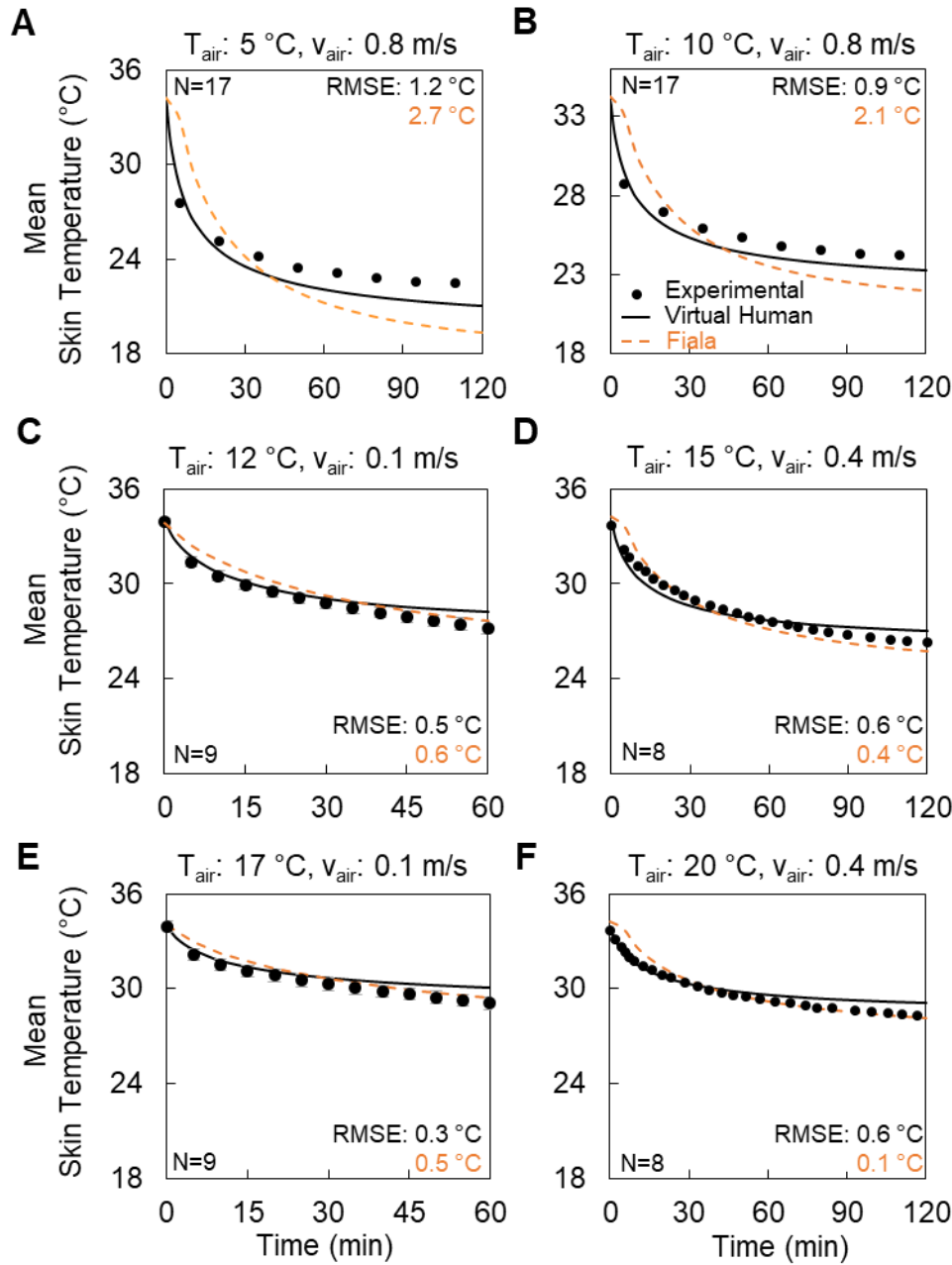
Fig. 5: Model validation of the mean skin temperature for mild, moderate, and very cold environmental conditions in Study 2 [panels (A) and (B)], Study 3 [panels (C) and (E)], and Study 4 [panels (D) and (F)], while subjects sat quietly for 60 or 120 minutes wearing minimal clothing (Table 1). The filled circles represent the average of the measured mean skin temperature values, and the solid black lines denote the changes predicted by the virtual human
