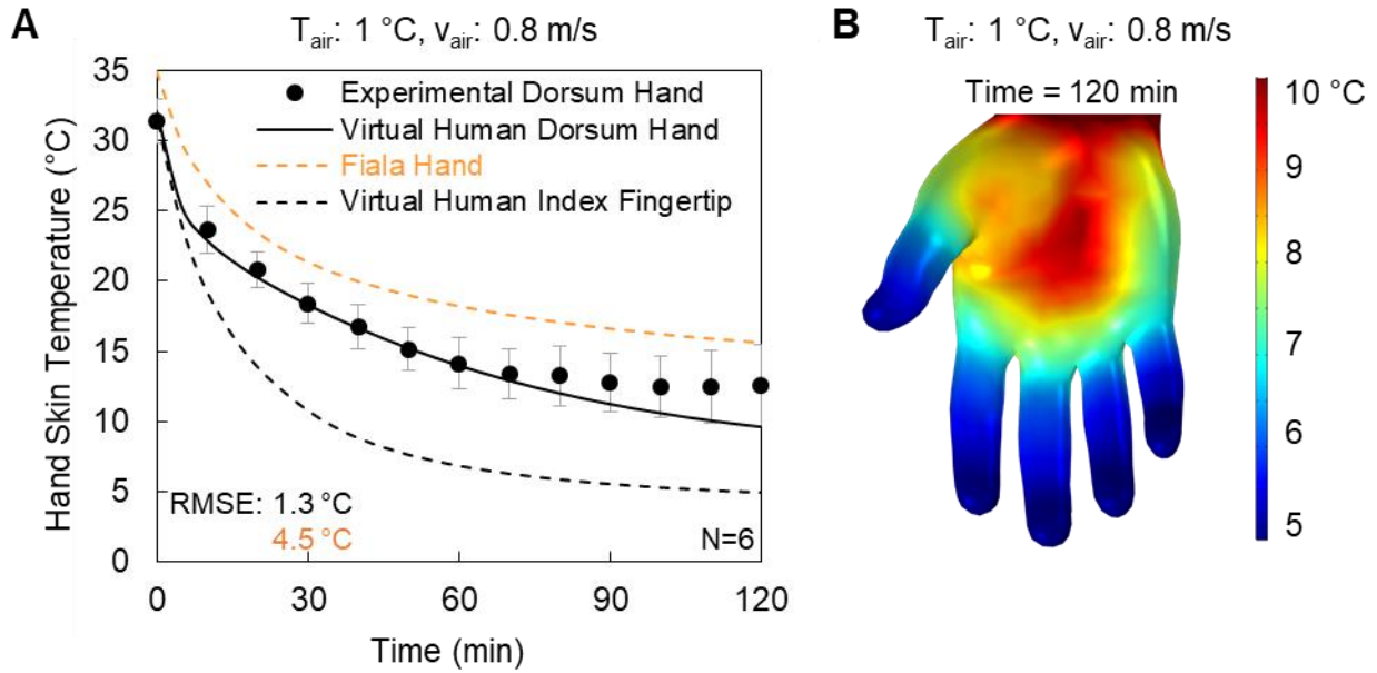
Fig. 10: (A) Model validation of the dorsum hand temperature and fingertip temperature for the extreme cold-stress condition in Study 1, in which subjects sat bare-handed at 1\text{ }^{\circ}\text{C} air temperature ( T_{air} ) and 0.8\text{ m/s} wind speed ( v_{air} ) for a period of 120 minutes while wearing trunks (Table 1). The filled circles represent the average of the measured dorsum hand temperature, the vertical gray bars indicate two standard errors of the mean, the solid and dashed black lines denote the dorsum hand and fingertip temperature predictions from the virtual human model, respectively, and the orange dashed line represents the hand skin temperature predicted by the Fiala model (39, 44). The latter model provides one lumped-parameter value for the entire hand, as it does not have the spatial resolution to distinguish different parts of the hand. (B) Model-predicted spatial temperature distribution of the hand at the end of the exposure for the conditions described in (A). Note the large differences in temperature between the palm of the hand and the fingertips. RMSE: root mean squared error.
