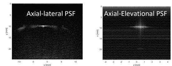
Figure 3: 3D PSF estimated from fine wire target experiment
