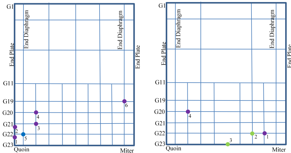
Figure 13. Land (left) and river (right) side leafs showing CFRP applications. Purple: Cracks with CFRP repairs, Blue: Cracks welded and repaired with CFRP. Green: No cracks, poor welds strengthened with CFRP.
