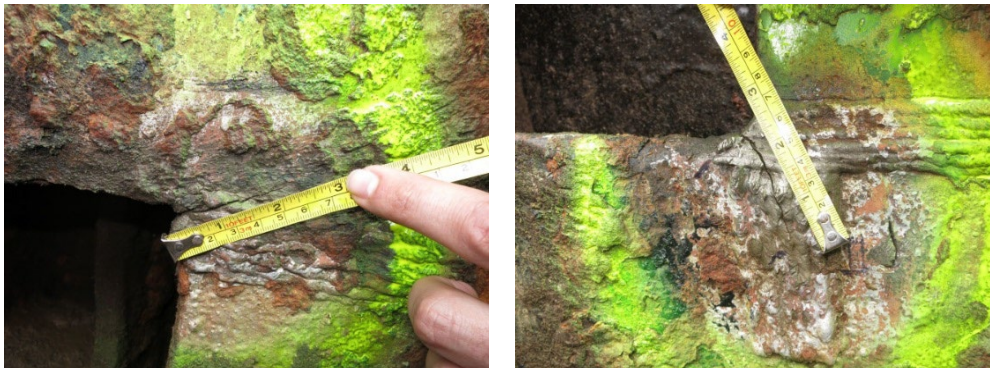
Figure 5. Cracks at intersection of intermediate diaphragm and girder flanges.
