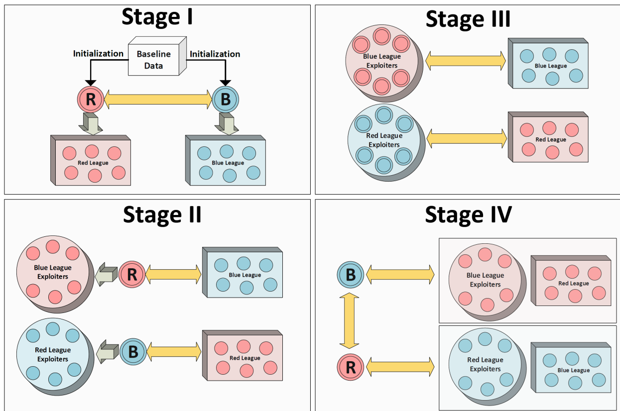
Figure 5: The four-stage training scheme.
