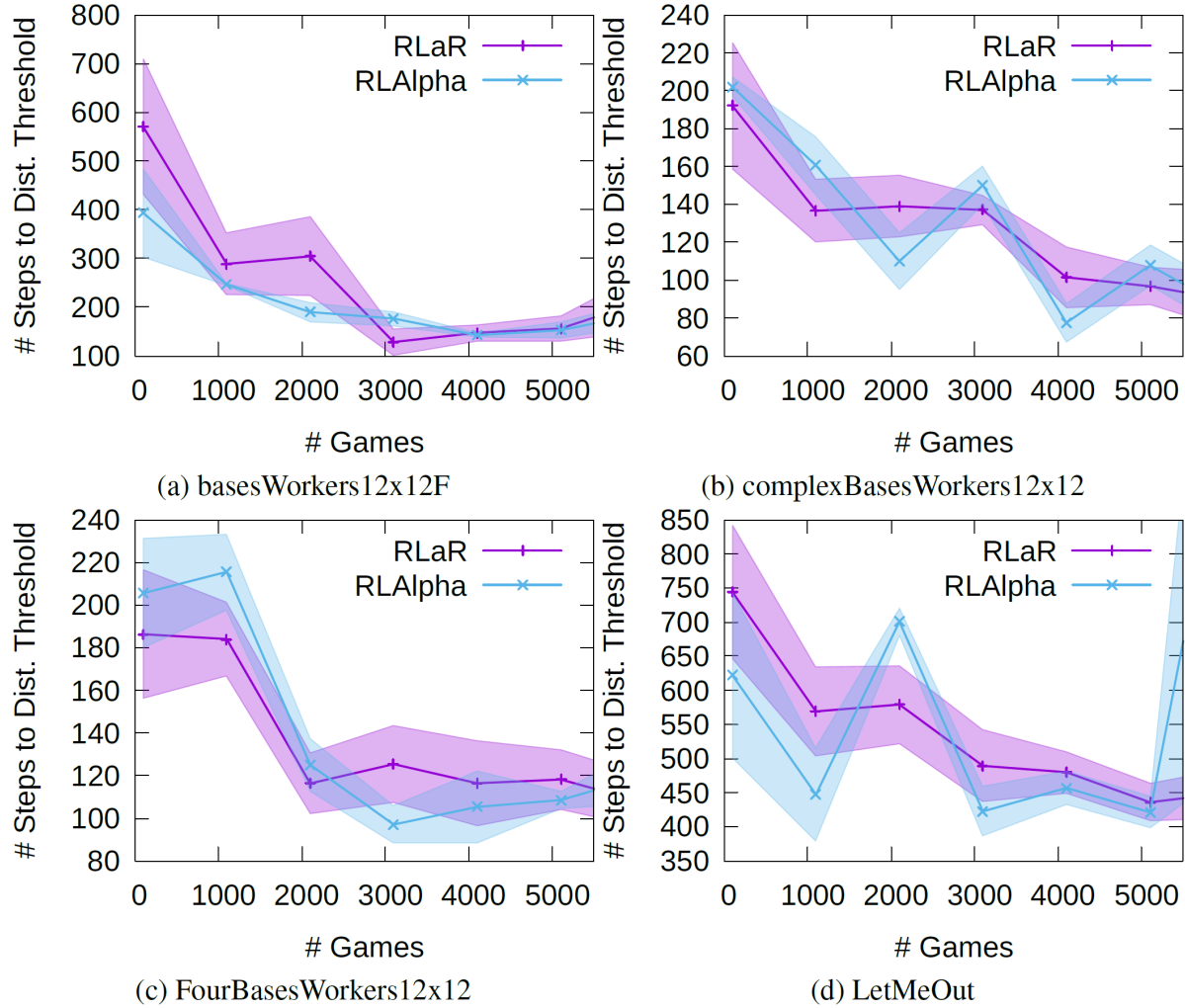
Figure 9: Plots showing the number of steps that the learner needs before at least one of its units gets within a distance threshold of 4.0 of the opponent’s base, thereby bringing it within the radius of the learner’s visibility.
