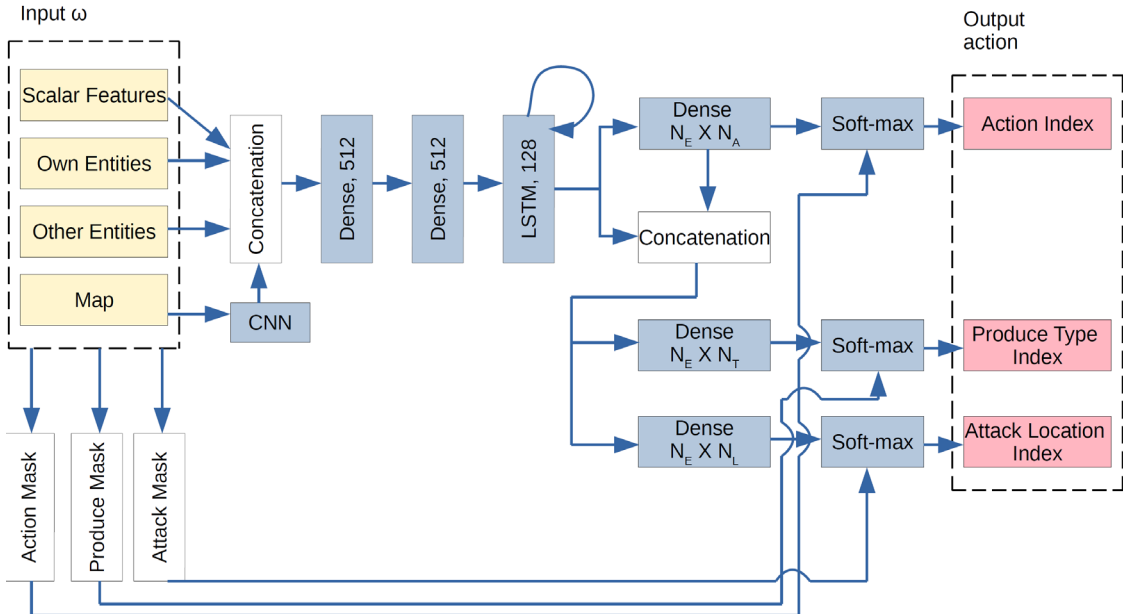
Figure 2: The actor network architecture.
