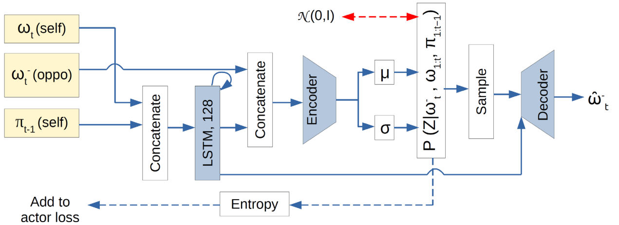
Figure 4: The prediction network architecture.
