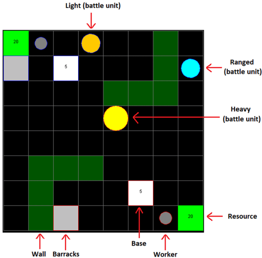
Figure 1: An 8X8 map of MicroRTS showing various kinds of units and features. This project focused on maps that are 16×16 or smaller.
