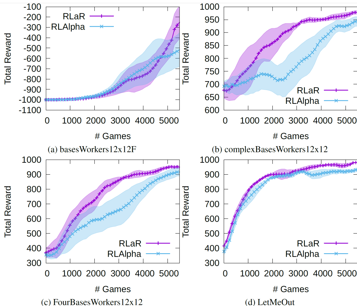
Figure 8: Learning curves of RLAlpha (RLAlpha+A2C+SIL) and RLaR (RLaR+A2C+SIL) against MicroPhantom in the 4 maps of Figures 6, 7. Baseline RL (A2C+SIL) is excluded due to poor performance. The terminal rewards for win/loss/draw are +1000/-1000/+50. The initial policy/actor was trained by supervised learning from games between MentalSeal and MicroPhantom on large set of maps, but performs poorly in (a).
