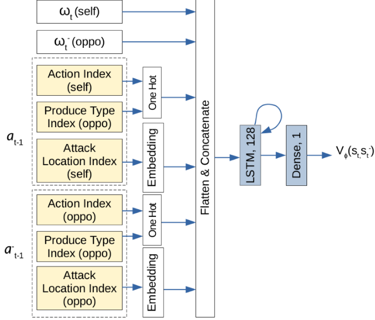
Figure 3: The critic network architecture.
