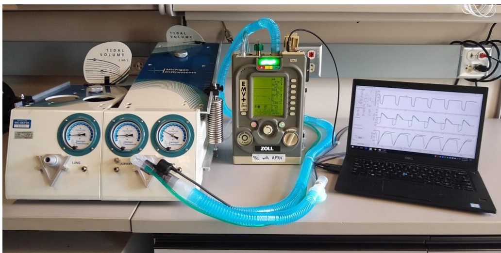
Figure 9: Photograph of the ZOLL EMV+ ® 731 Series ventilator with prototype firmware, delivering an airway pressure release ventilation (APRV) waveform to a Michigan Instruments test lung.
