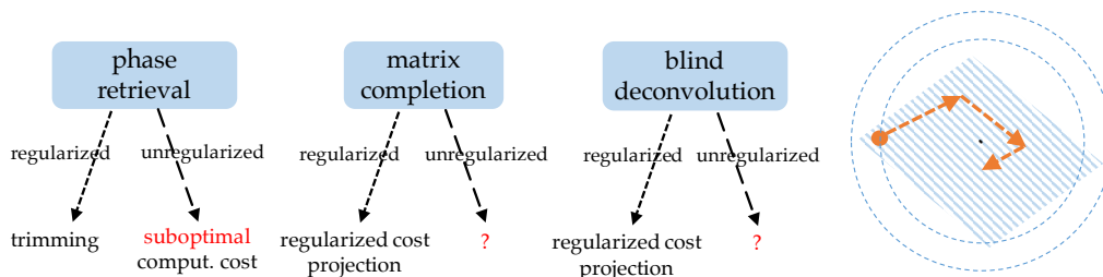
Figure 1: (Left) prior literature often requires sophisticated model-specific regularization in order to achieve fast convergence; (right) our results show that simple first-order methods implicitly regularize their iterates, thus achieving the fastest possible convergence without any explicit regularization.
