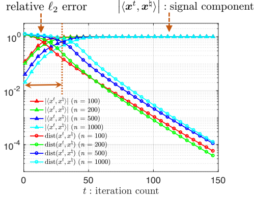
Figure 2: Numerically convergence of randomly initialized gradient methods.
