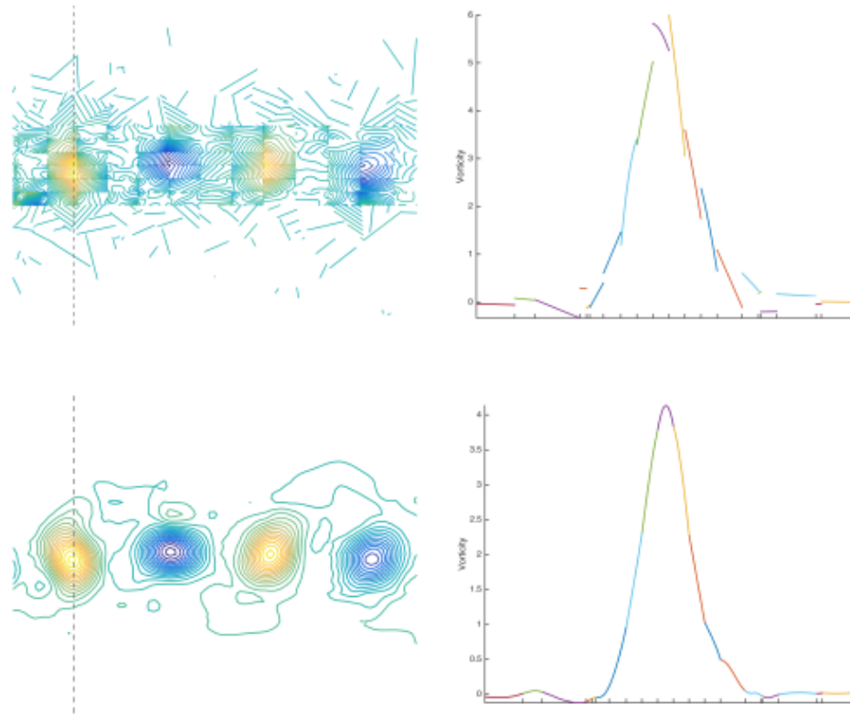
Figure 1: Images from Cylinder Flow. Comparison between calculating vorticity using dG data vs L-SIAC. The first row of images are calculated using raw dG data at fine grid resolution. Second Row of images are vorticity calculated L-SIAC.
