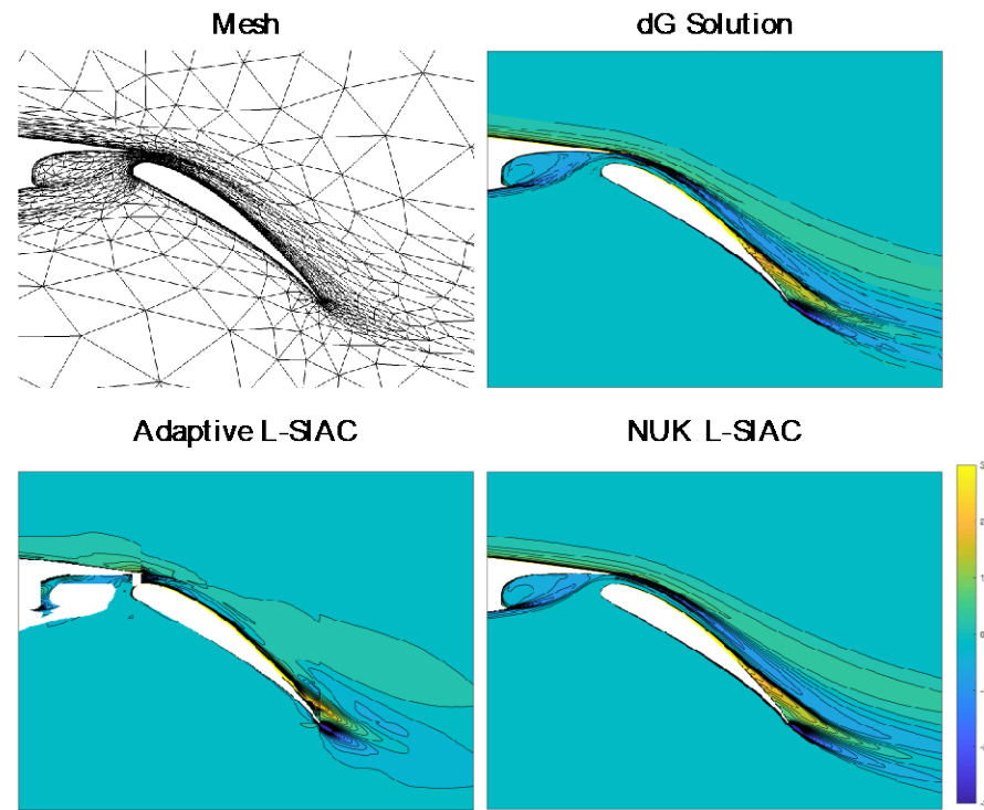
Figure 1: Vorticity from a P^2 dG RANS solution for a multi-element airfoil from Ref. [14] [15].
