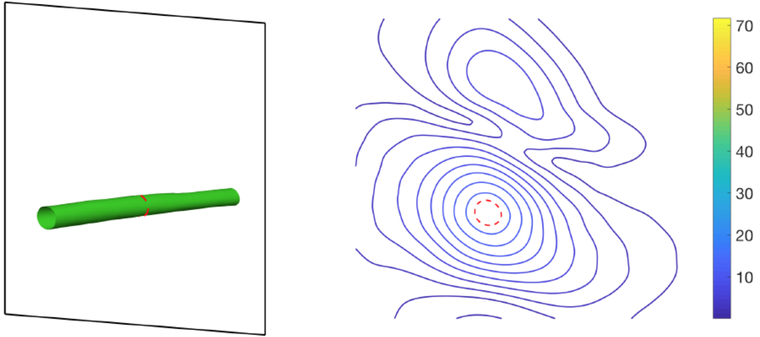
Figure 11: The above vortex tube is obtained by applying the L-SIAC filter using constant characteristic length equal to local maximum edge length. We observe the noise is reduced, but there is only one iso-contour indicated by dotted redline.
