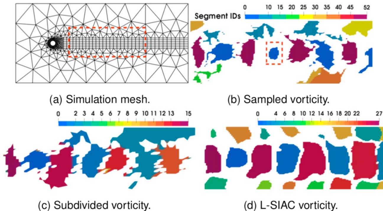
Fig. 16: Segmentation of the vorticity for the flow past a cylinder shown in (a). The segmentation for the sampled and the subdivided vorticity are computed using the contour tree along with a persistence threshold of 0.04. In the case of L-SIAC vorticity, the value of persistence threshold used is 0.001.
