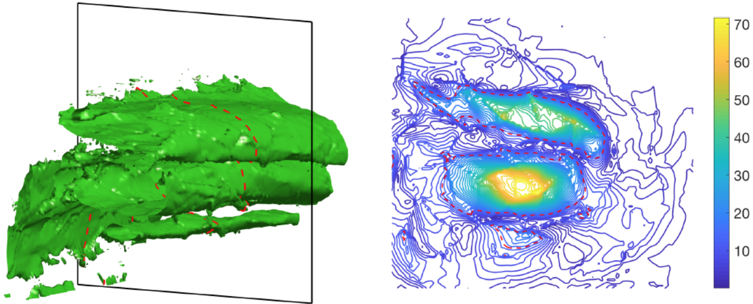
Figure 10: On the left of the image above, we show vortex tube taken from a three-dimensional contour-rotating vortex from Figure 9. The black lines represent the cutting plane for analysis. On the right, we show a contour plot of vorticity computing in an element-wise fashion from the raw data. Note data is noisy, but we observe two iso-contours indicated by dotted redlines.
