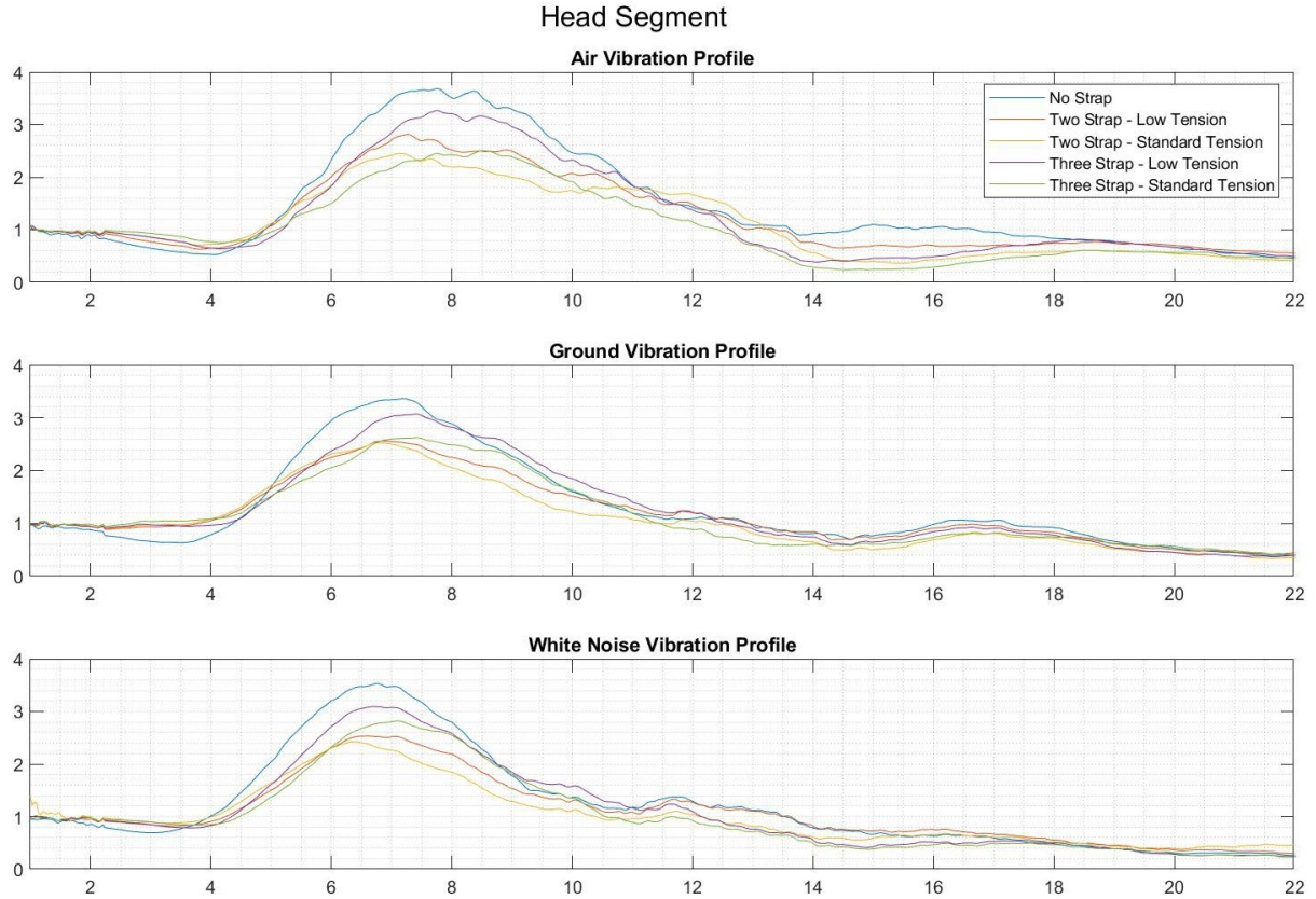
Figure 7: Transmissibility (meaning the frequency response) plots concerning the manikin's head segment. Results for all five strap conditions and all three vibration profiles are shown. The X-axis is frequency (Hz) and the Y-axis is the transmissibility ratio.
