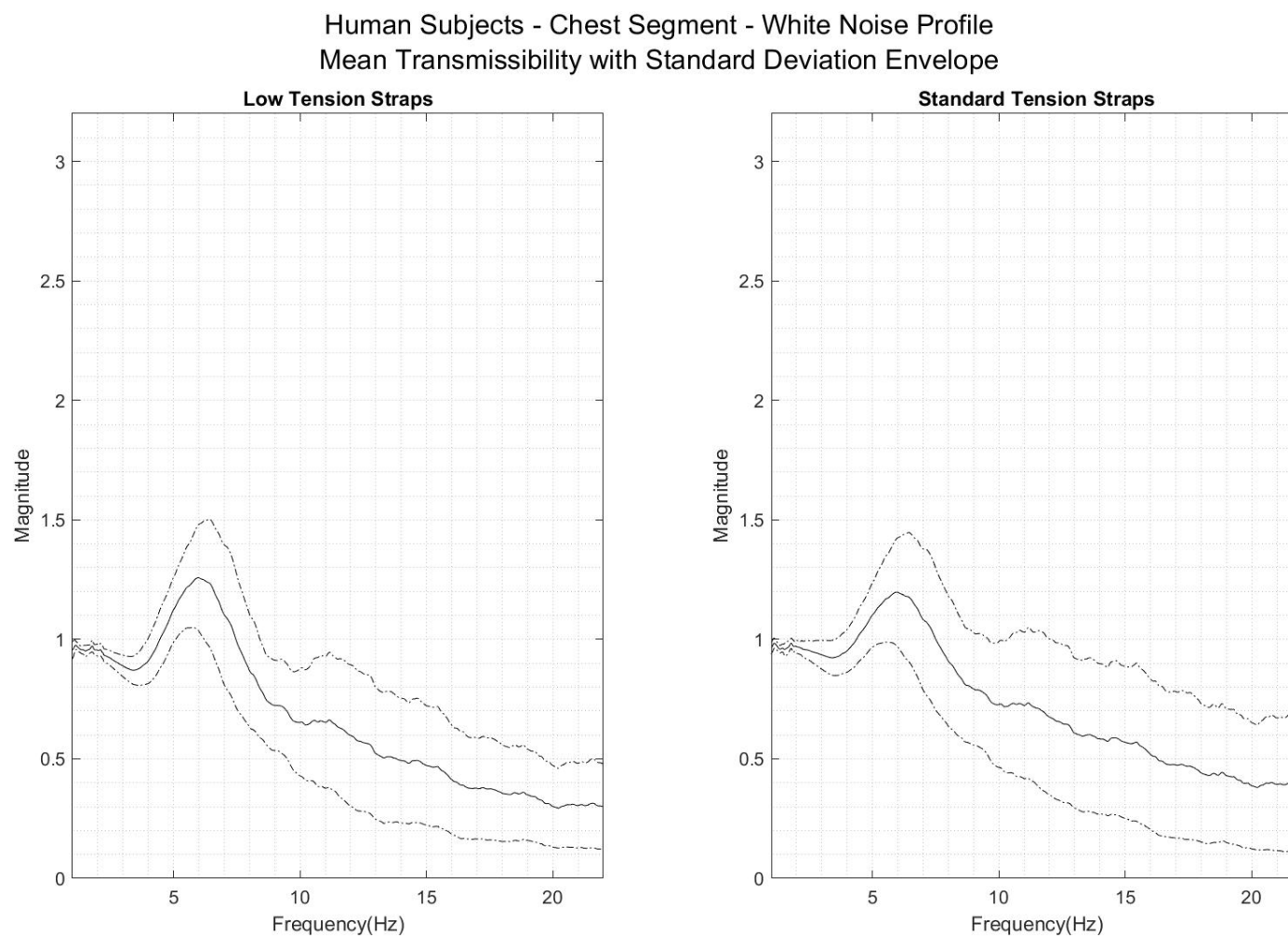
Figure 31: Plots of human subject mean transmissibility (solid line) with the corresponding standard deviation envelope (dashed lines). The results of the chest segment in the white noise vibration profile are shown here. The left graph depicts the low tension strap condition, and the right graph depicts the standard tension strap condition.
