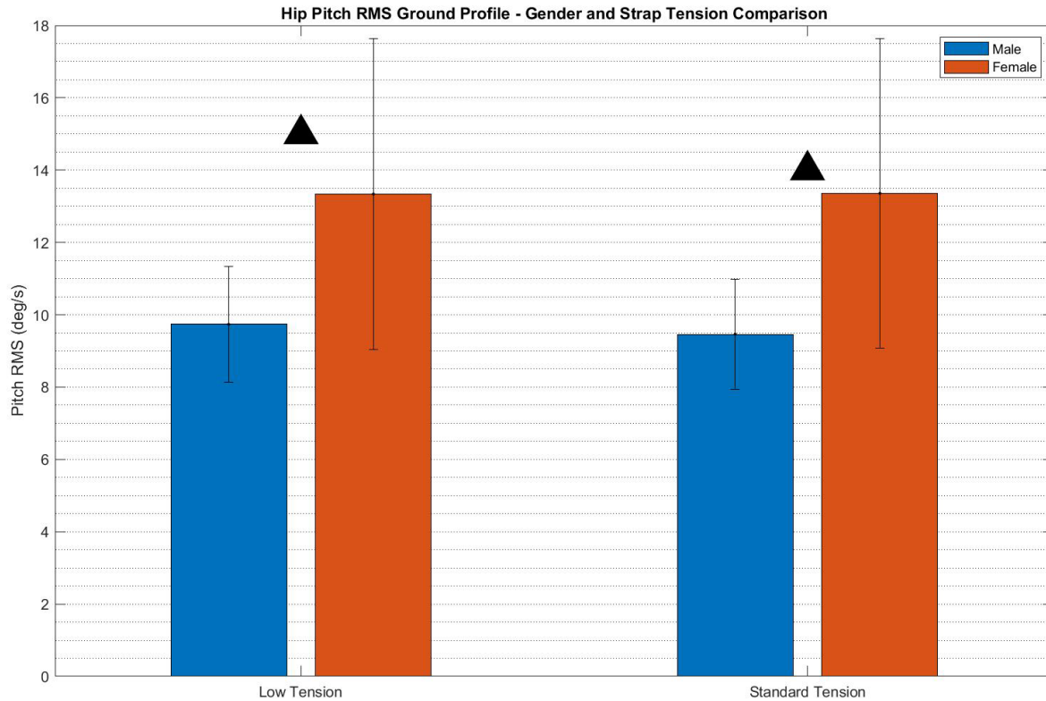
Figure 38: This figure shows how the pitch motion of the hip segment in the ground vibration profile varied based on gender and strap tension. The results are reported as root mean square (RMS) values. Intra-subject normalization was not applied. The black triangle signifies statistical significance, and the black square signifies marginal statistical significance (this plot shows that the male and female data sets differed in a statistically significant manner under both the low and standard tension conditions).
