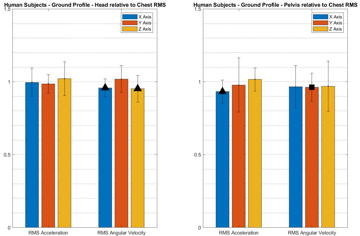
Figure 22: This figure depicts the mean ratio values and corresponding standard deviations of the relative segment motion metrics (RMS Acceleration and RMS Angular Velocity) for Ground vibration profile. On the left the metrics concerning the motion of the head relative to the chest are shown, and on the right the pelvis relative to the chest. The bar shows the mean ratio, the black brackets show the corresponding standard deviation, the black triangles denote statistically significant results, and the black squares denote results of marginal statistical significance.
