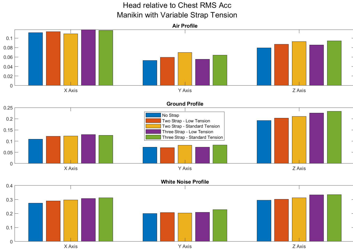
Figure 13: Bar plots showing the RMS accelerations for the relative motion of the manikin head segment with respect to the manikin chest segment. The RMS accelerations are broken out into its three axes, five strap conditions, and three vibration profiles.
