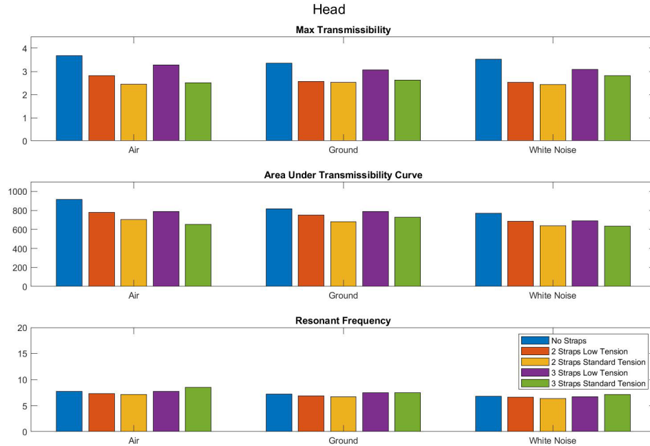
Figure 10: Bar plot comparing metrics calculated from the manikin's head transmissibility plots. Variation in the metrics of max transmissibility, area under the transmissibility curve, and resonant frequency are shown. The results are organized by both strap condition and input vibration profile.
