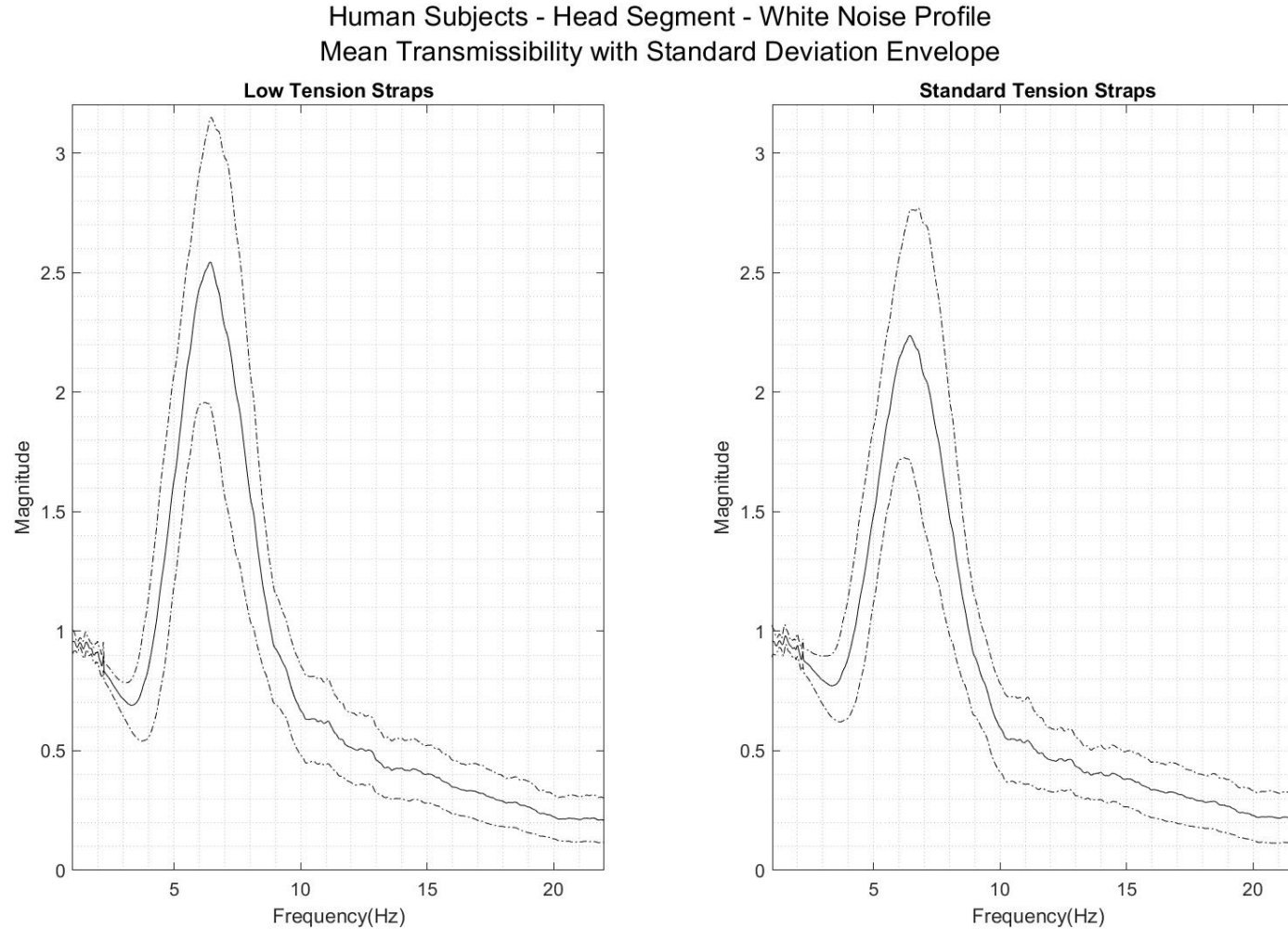
Figure 30: Plots of human subject mean transmissibility (solid line) with the corresponding standard deviation envelope (dashed lines). The results of the head segment in the white noise vibration profile are shown here. The left graph depicts the low tension strap condition, and the right graph depicts the standard tension strap condition.
