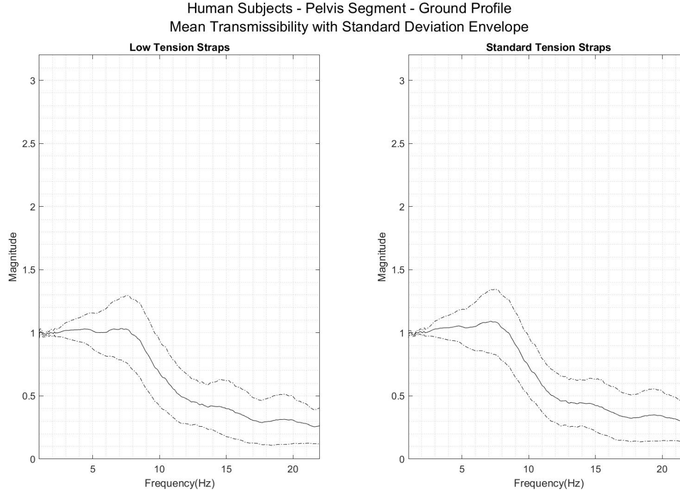
Figure 29: Plots of human subject mean transmissibility (solid line) with the corresponding standard deviation envelope (dashed lines). The results of the pelvis segment in the ground vibration profile are shown here. The left graph depicts the low tension strap condition, and the right graph depicts the standard tension strap condition.
