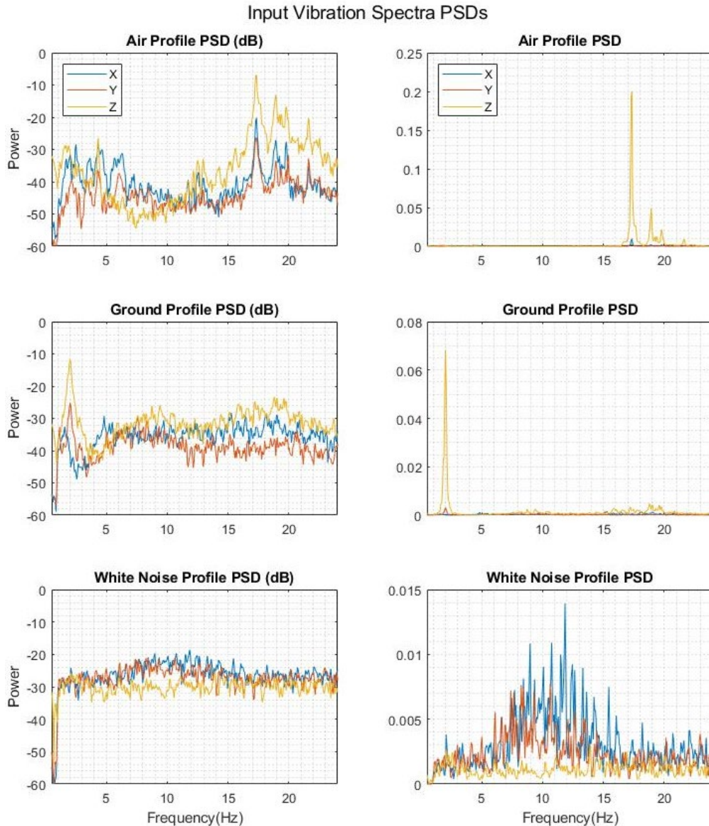
Figure 16. Power spectral densities for the three input vibration spectra expressed on a logarithmic scale as decibels (left column) and on a standard linear scale (right column).
