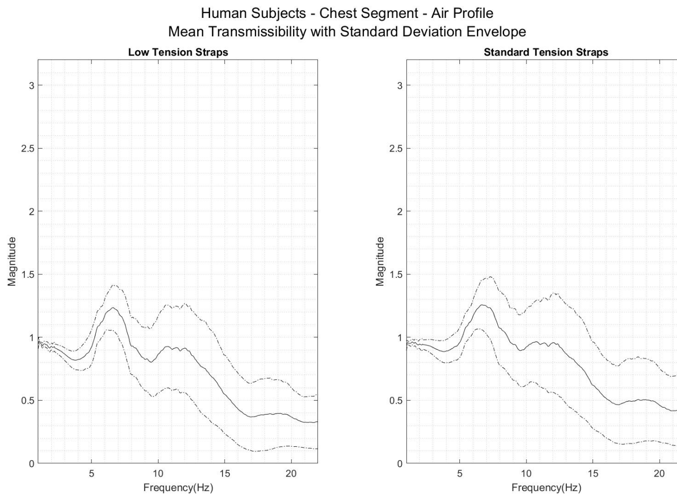
Figure 25: Plots of human subject mean transmissibility (solid line) with the corresponding standard deviation envelope (dashed lines). The results of the chest segment in the air vibration profile are shown here. The left graph depicts the low tension strap condition, and the right graph depicts the standard tension strap condition.
