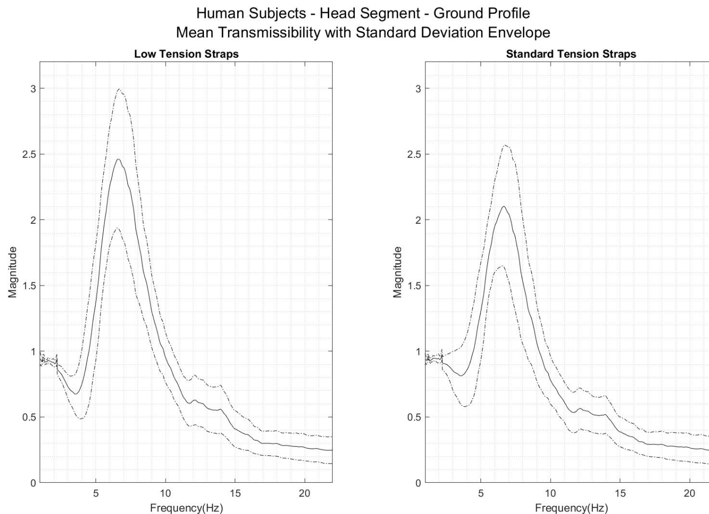
Figure 27: Plots of human subject mean transmissibility (solid line) with the corresponding standard deviation envelope (dashed lines). The results of the head segment in the ground vibration profile are shown here. The left graph depicts the low tension strap condition, and the right graph depicts the standard tension strap condition.
