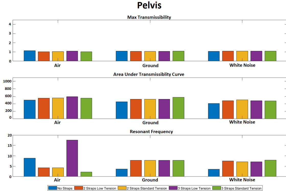
Figure 20. Bar plots comparing metrics calculated from the manikin's pelvis transmissibility plots.
