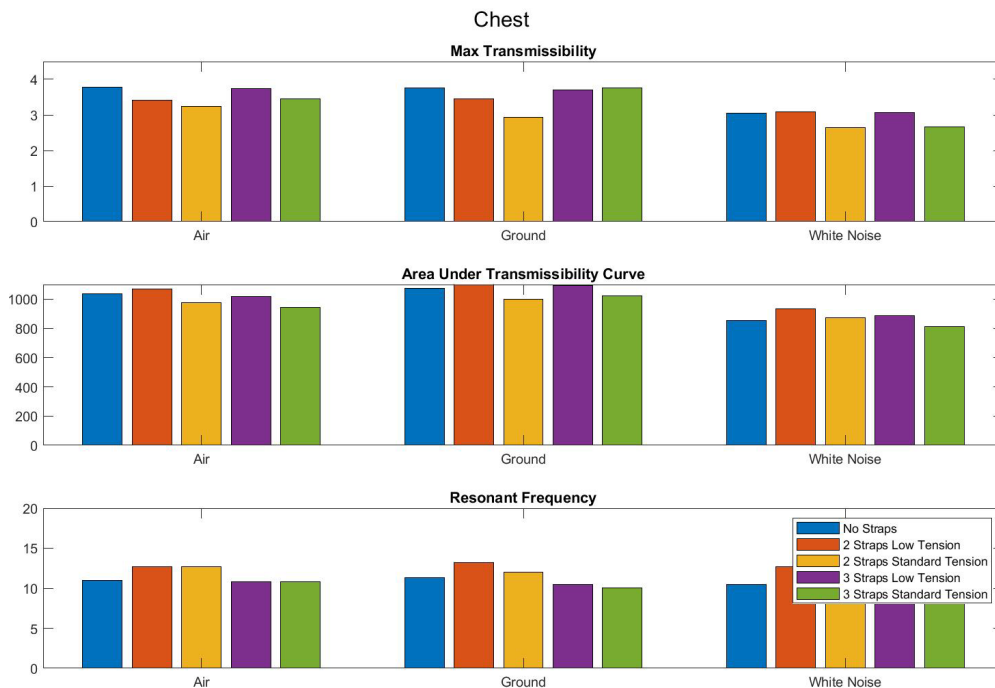
Figure 11: Bar plot comparing metrics calculated from the manikin's chest transmissibility plots. Variation in the metrics of max transmissibility, area under the transmissibility curve, and resonant frequency are shown. The results are organized by both strap condition and input vibration profile.
