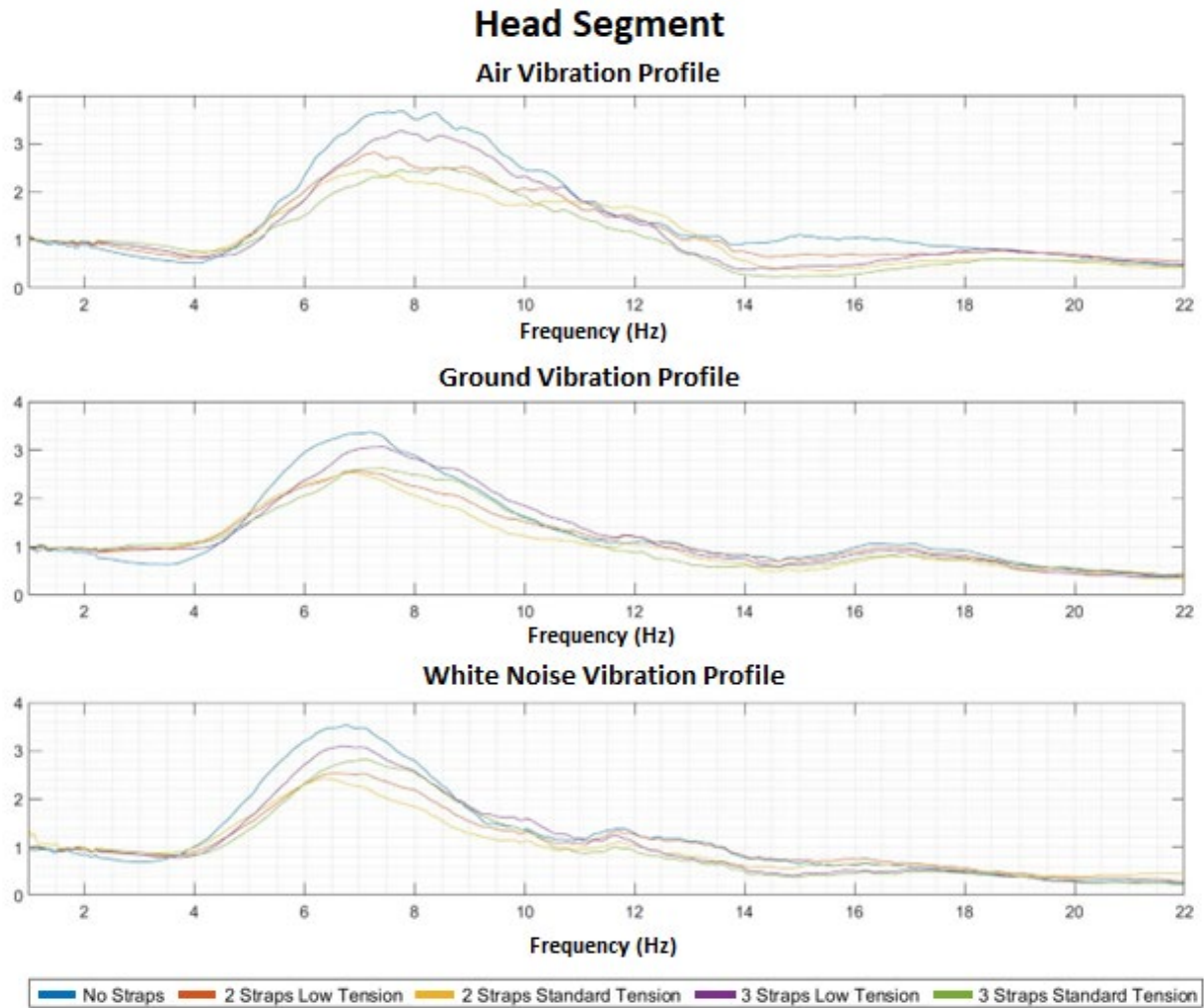
Figure 17. Transmissibility plots for the manikin's head segment.
