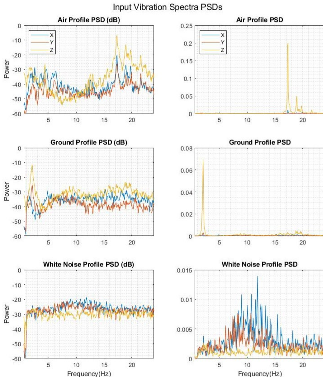
Figure 5: Power spectral densities for the three input vibration spectra expressed on a logarithmic axis as decibels (left column) and on a standard linear axis (right column).
