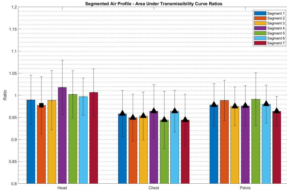
Figure 19: This figure depicts the mean ratio values and corresponding standard deviations of the area under the transmissibility curve ratios for the head, chest, and pelvis body segments over the seven segments of the Air vibration profile. The bar shows the mean ratio, the black brackets show the corresponding standard deviation, the black triangles denotes statistically significant results, and the black squares denote results of marginal statistical significance.
