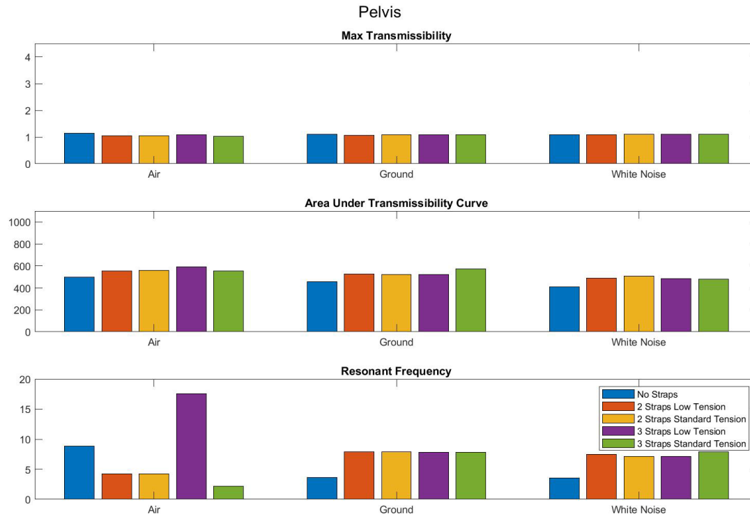
Figure 12: Bar plot comparing metrics calculated from the manikin's pelvis transmissibility plots. Variation in the metrics of max transmissibility, area under the transmissibility curve, and resonant frequency are shown. The results are organized by both strap condition and input vibration profile.
