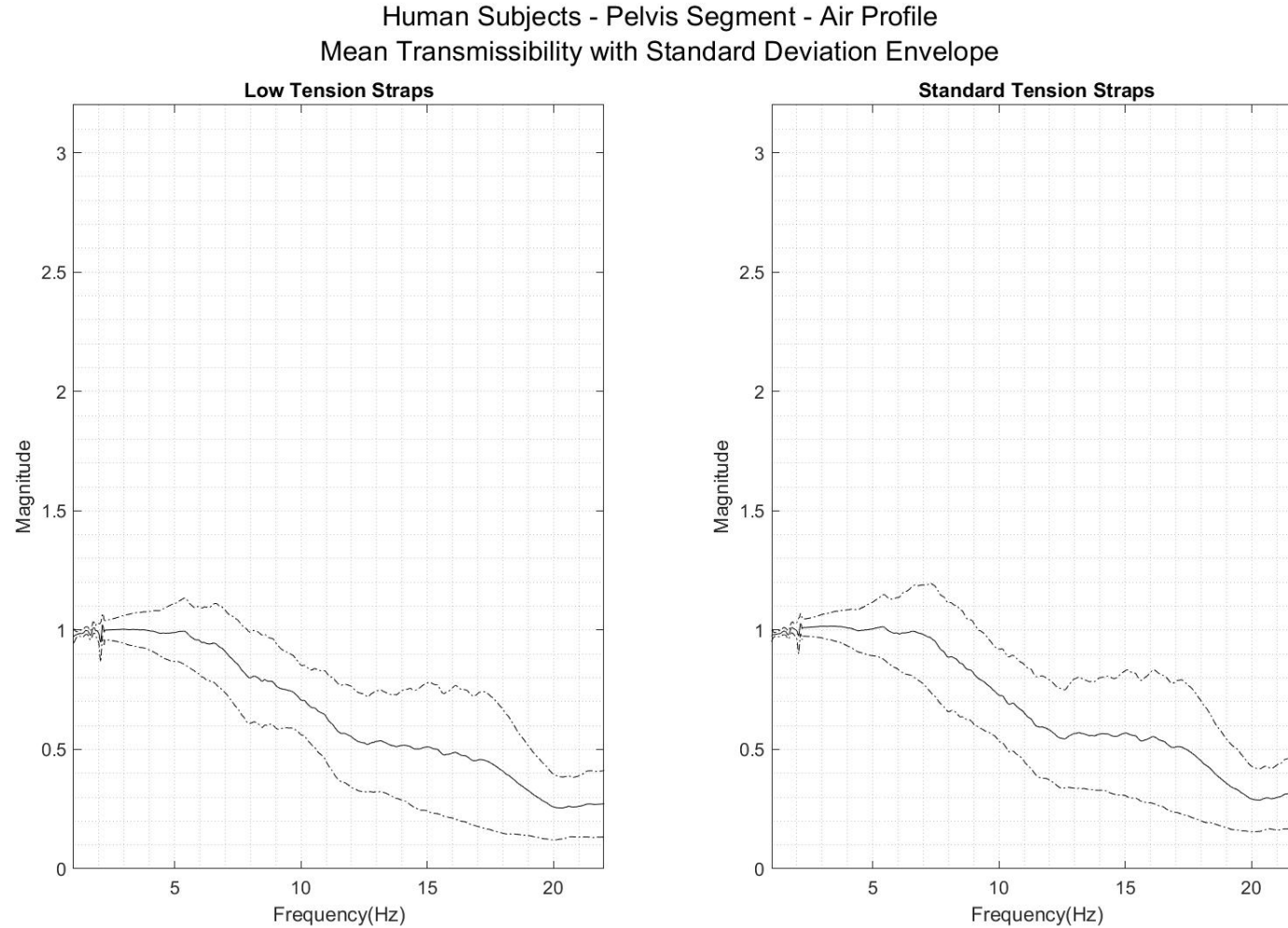
Figure 26: Plots of human subject mean transmissibility (solid line) with the corresponding standard deviation envelope (dashed lines). The results of the pelvis segment in the air vibration profile are shown here. The left graph depicts the low tension strap condition, and the right graph depicts the standard tension strap condition.
