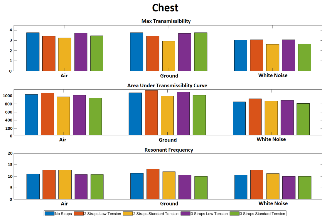
Figure 19. Bar plots comparing metrics calculated from the manikin's chest transmissibility plots.
