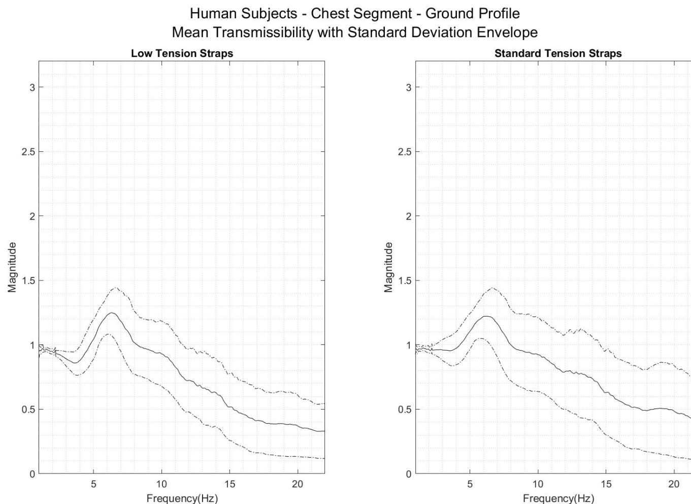
Figure 28: Plots of human subject mean transmissibility (solid line) with the corresponding standard deviation envelope (dashed lines). The results of the chest segment in the ground vibration profile are shown here. The left graph depicts the low tension strap condition, and the right graph depicts the standard tension strap condition.
