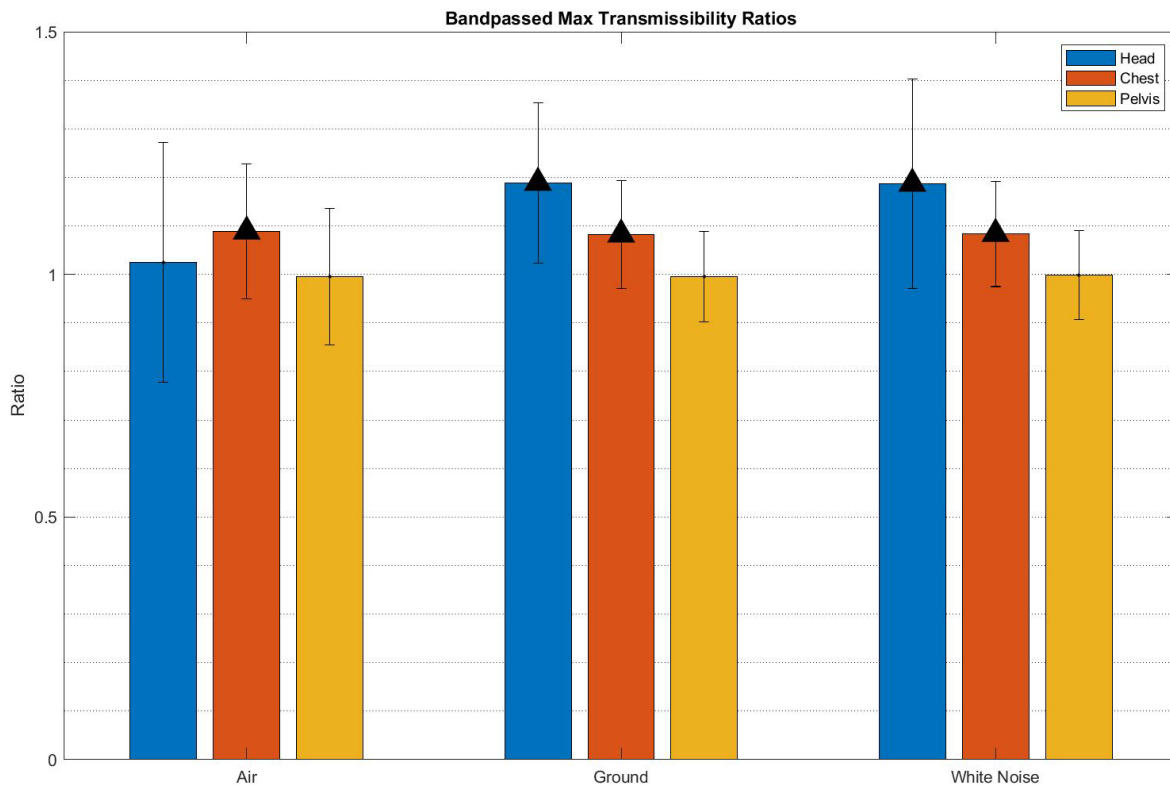
Figure 33: This figure depicts the mean ratio values and corresponding standard deviations of the bandpassed max transmissibility ratios for the head, chest, and pelvis body segments. The bar shows the mean ratio, the black brackets show the corresponding standard deviation, and the black triangles denote statistically significant results.
