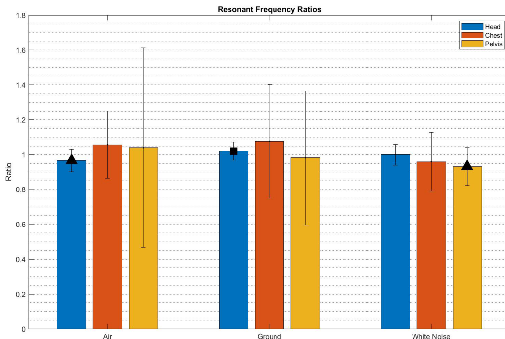
Figure 17: This figure depicts the mean ratio values and corresponding standard deviations of the resonant frequency ratios for the head, chest, and pelvis body segments. The bar shows the mean ratio, the black brackets show the corresponding standard deviation, the black triangles denotes statistically significant results, and black squares denote marginal statistical significance.
