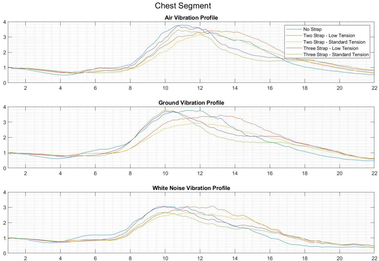
Figure 8: Transmissibility (meaning the frequency response) plots concerning the manikin's chest segment. Results for all five strap conditions and all three vibration profiles are shown. The X-axis is frequency (Hz) and the Y-axis is the transmissibility ratio.
