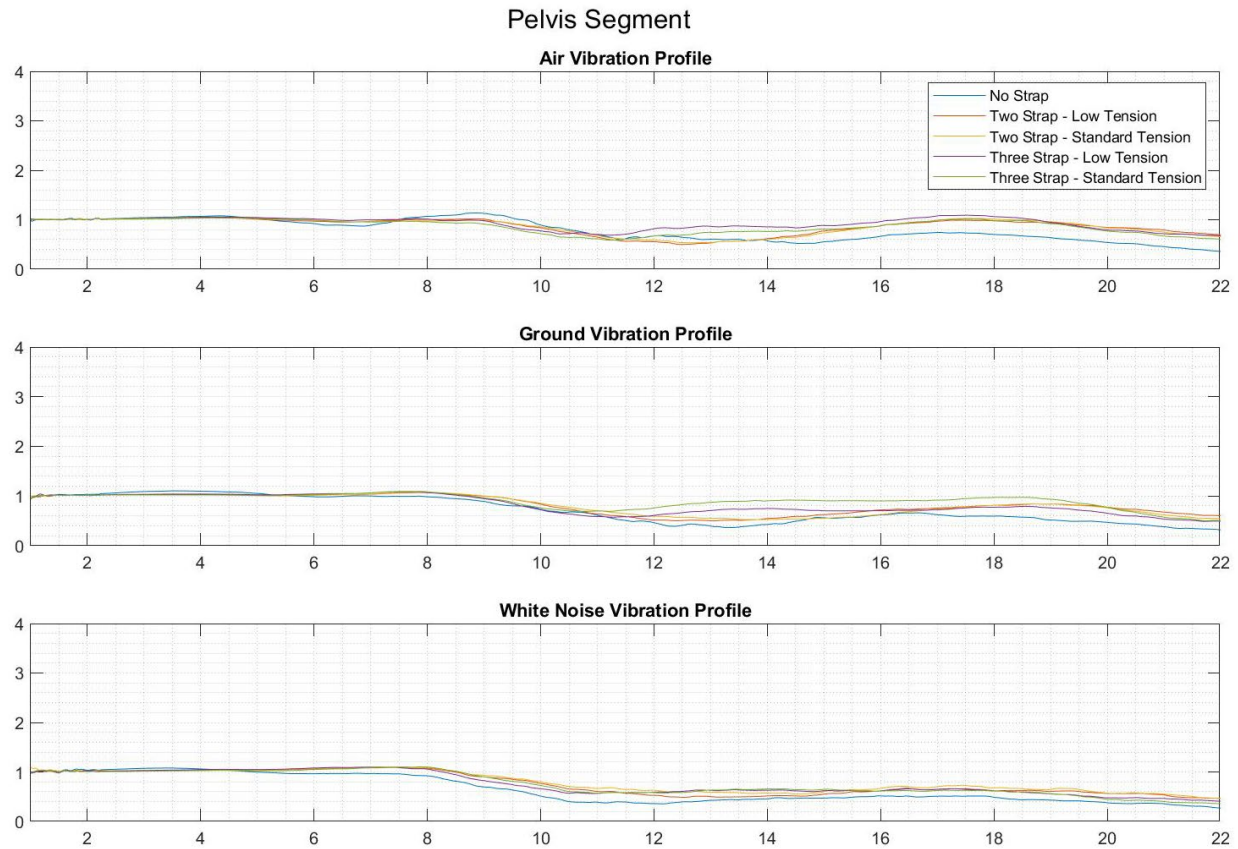
Figure 9: Transmissibility (meaning the frequency response) plots concerning the manikin's pelvis segment. Results for all five strap conditions and all three vibration profiles are shown. The X-axis is frequency (Hz) and the Y-axis is the transmissibility ratio.
