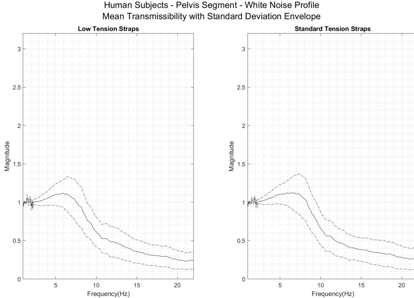
Figure 32: Plots of human subject mean transmissibility (solid line) with the corresponding standard deviation envelope (dashed lines). The results of the pelvis segment in the white noise vibration profile are shown here. The left graph depicts the low tension strap condition, and the right graph depicts the standard tension strap condition.
