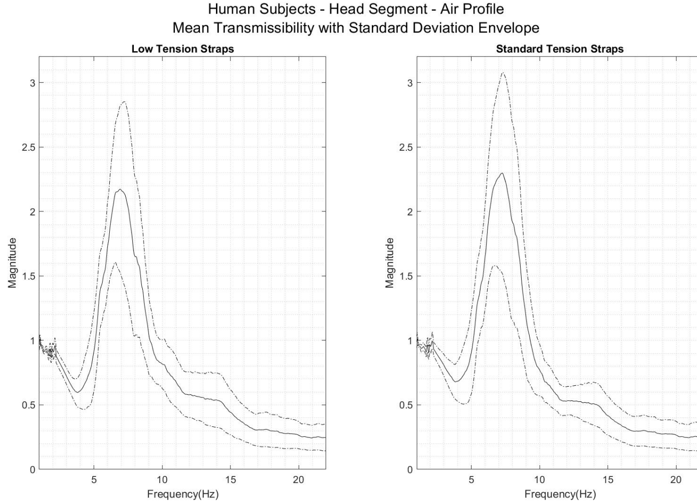
Figure 24: Plots of human subject mean transmissibility (solid line) with the corresponding standard deviation envelope (dashed lines). The results of the head segment in the air vibration profile are shown here. The left graph depicts the low tension strap condition, and the right graph depicts the standard tension strap condition.
