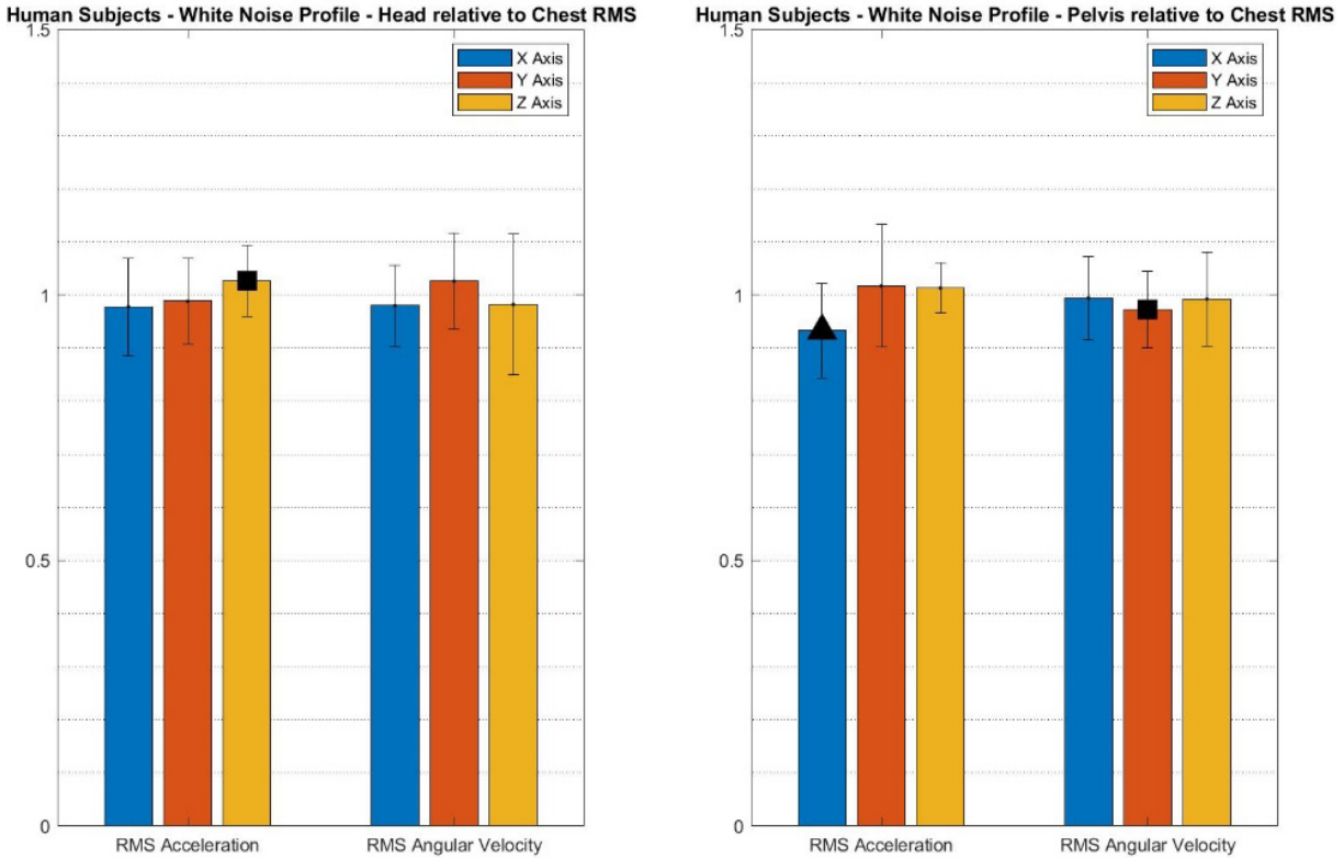
Figure 23: This figure depicts the mean ratio values and corresponding standard deviations of the relative segment motion metrics (RMS Acceleration and RMS Angular Velocity) for White Noise vibration profile. On the left the metrics concerning the motion of the head relative to the chest are shown, and on the right the pelvis relative to the chest. The bar shows the mean ratio, the black brackets show the corresponding standard deviation, the black triangles denote statistically significant results, and the black squares denote results of marginal statistical significance.
