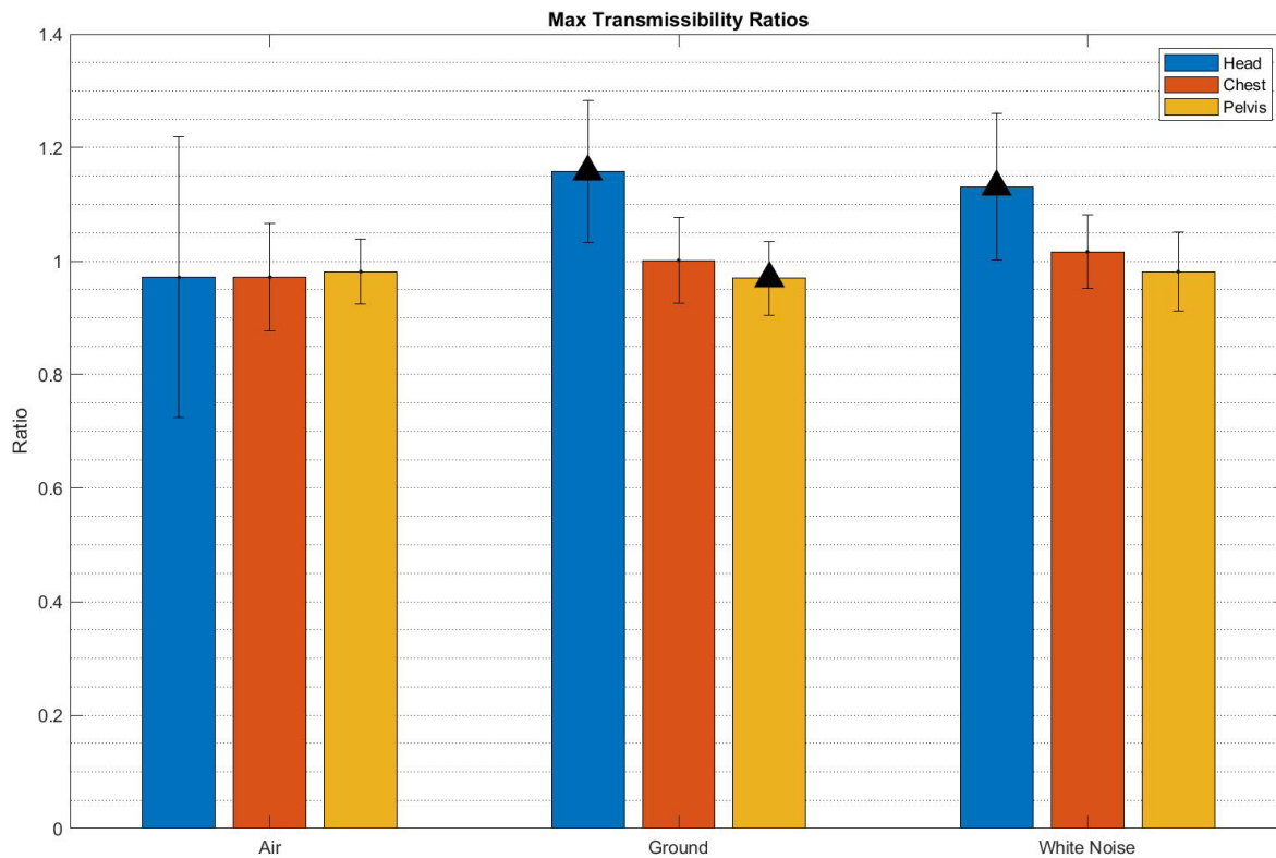
Figure 15: This figure depicts the mean ratio values and corresponding standard deviations of the max transmissibility ratios for the head, chest, and pelvis body segments. The bar shows the mean ratio, the black brackets show the corresponding standard deviation, and the black triangles denote statistically significant results.
