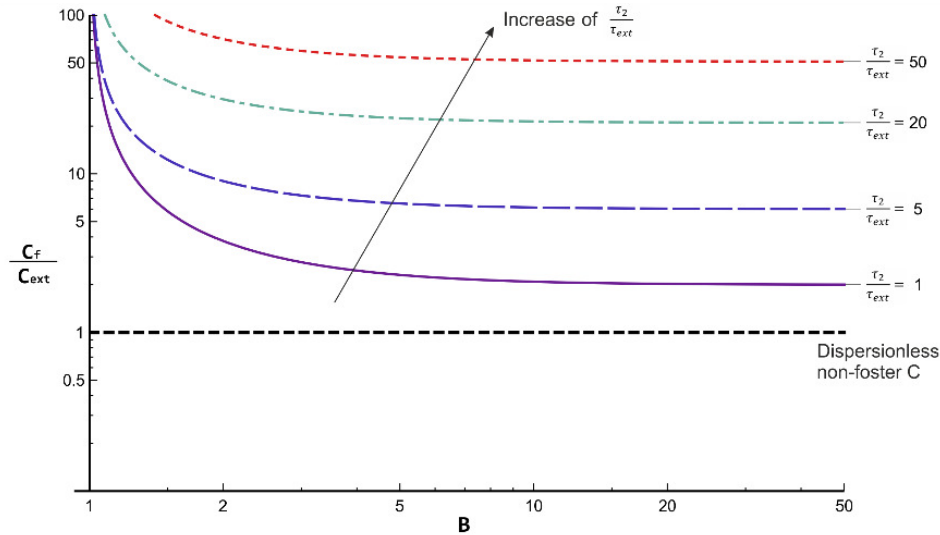
Figure 4-9 (taken from [96]) Bandpass negative capacitor - Maximal stable normalized negative capacitance as a function of amplifier bandwidth B with different values of \tau_2/\tau_{ext}
