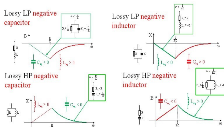
Figure 5-43 An overview of simple passive networks used for construction of stability-robust non-Foster elements.
