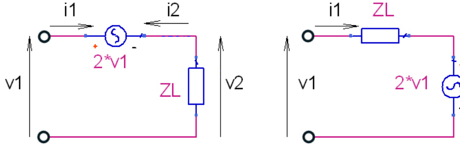
Figure 3-32 Two possible equivalent circuits of VNIC with single voltage source
