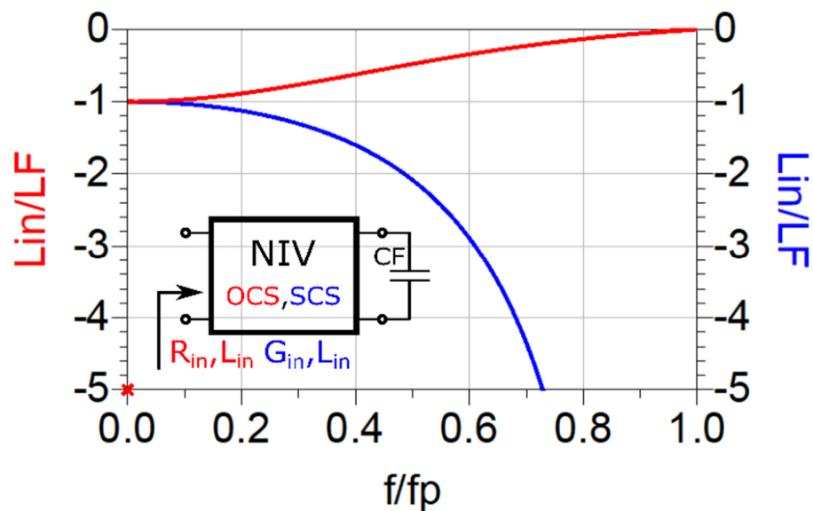
Figure 3-35 Dispersion of inductance of OCS/SCS negative inductor (OCS/SCS NIV terminated by ordinary capacitor)
