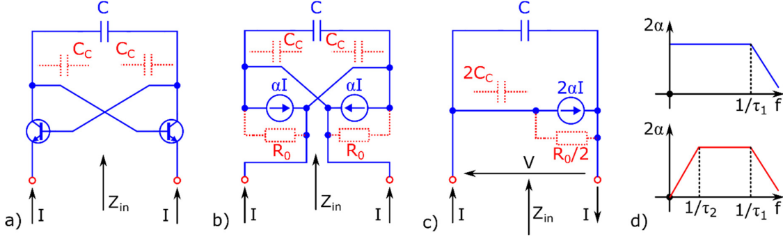
Figure 4-10. OCS negative capacitor based on Linvill's floating NIC
