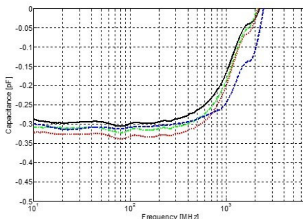
Figure 6-3 Measured input capacitance of SCS Miller negative capacitor integrated circuit with HCBTs with different f_T ( f_T=33 \text{ GHz} – dash-dotted green curve, solid black, f_T=35 \text{ GHz} –solid black curve, f_T=36 \text{ GHz} –dotted red curve, f_T=45 \text{ GHz} , –dotted blue curve.
