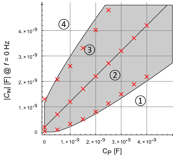
Figure 3-48 (adapted from [91]). Stability regions for lumped network (Fig. 3-2 (a)) containing parallel combination of an ideal positive and a realistic negative capacitor. Solid curves: Results obtained using analytical expressions (3.22, 3.23) and one-pole amplifier model, ( R_G = 50 \Omega , \tau = 10 \text{ ns} , A_0 = 2 , parameters C_P and C_F are varied). Crosses: Results obtained by ADS-SPICE simulation of negative capacitor based on operation amplifier THS 4303 [91].
