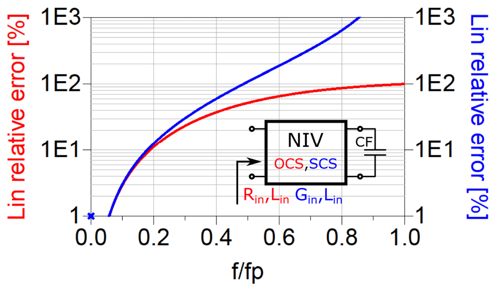
Figure 3-38 Relative error of inductance of OCS/SCS negative inductor (OCS/SCS NIV terminated by ordinary capacitor)
