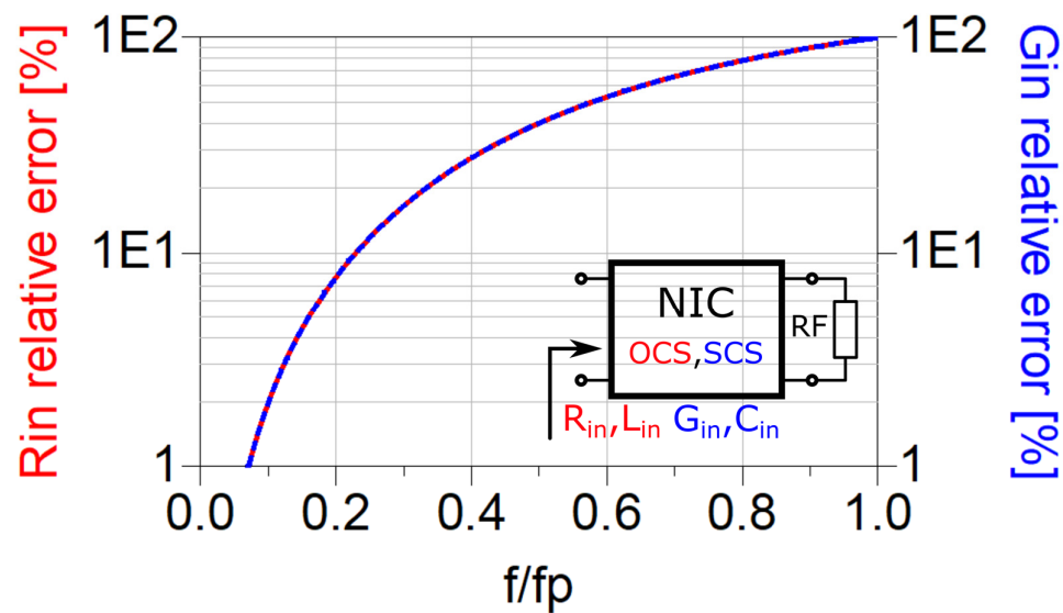
Figure 3-26 Relative error of resistance/conductance of OCS/SCS negative resistor (OCS/SCS NIC terminated by ordinary resistor)
