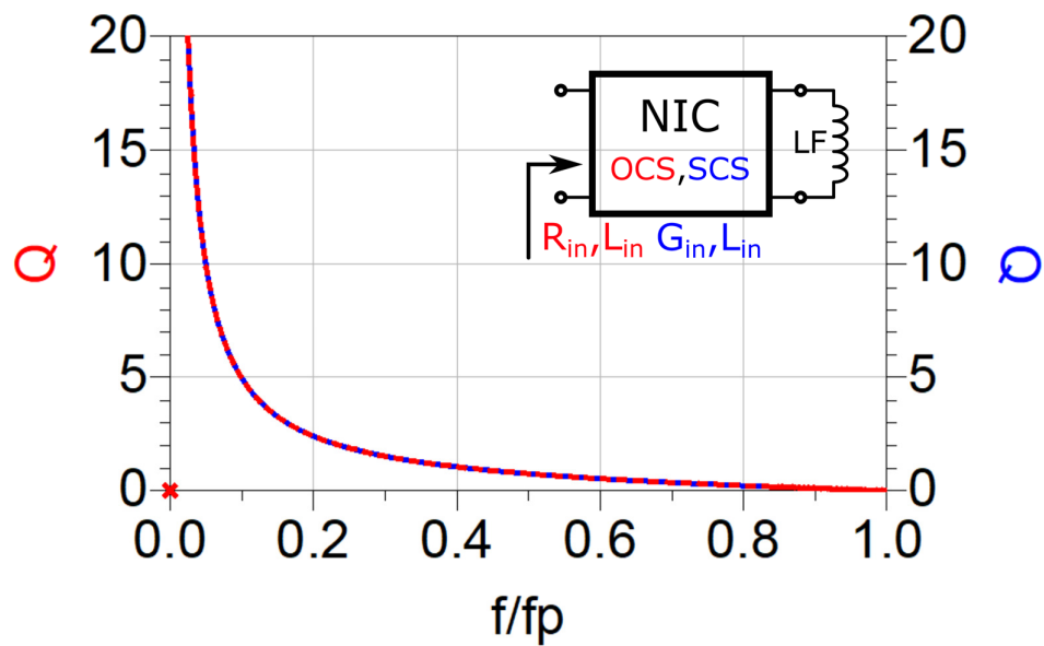
Figure 3-21 Q factor of OCS/SCS negative inductor (OCS/SCS NIC terminated by ordinary inductor)
