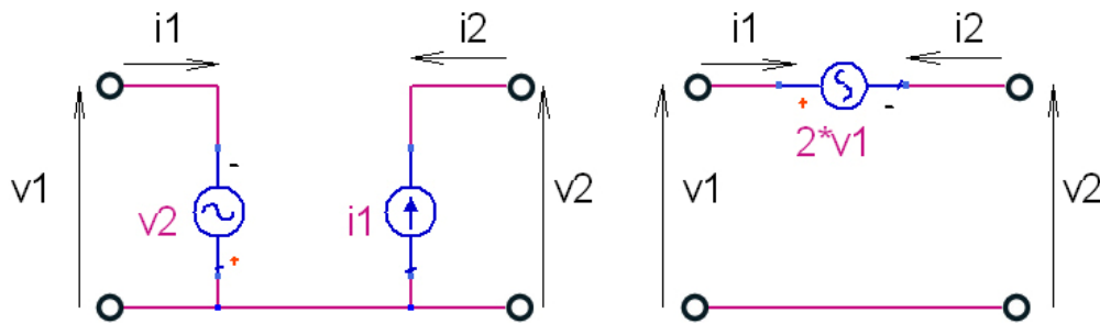
Figure 3-31 Transformation of basic VNIC into a circuit with a single voltage source
