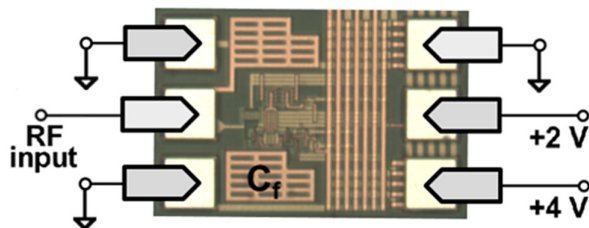
Figure 6-2 A microphotograph of fabricated SCS Miller negative capacitor that mimics low-frequency OPamp approach.
