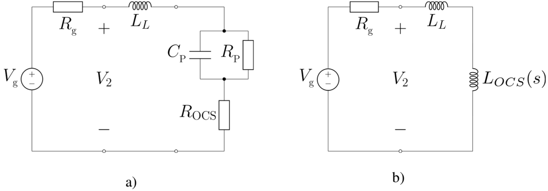
Figure 5-5 (a) Stability testing schematics for novel compensated RC network loaded with external network. (b) Stability testing schematic for ‘classic’ negative inductance constructed based on OCS NIC.
