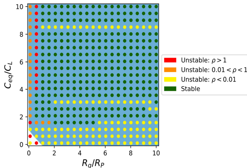
Figure 5-42 Stability area plot of compensated RC network loaded with positive inductance. Plot has been generated using: R_P = 31.4 \, \Omega , L_P = 1.22 \, \text{nH} , R_F = 70.5 \, \Omega , L_F = 320 \, \text{pH} . Painted areas are calculated using simplified analytical approach (Dark blue – range of external impedances that cause stable operation; Light blue - range of external impedances that cause unstable operation). Colored dots are results predicted by commercial system identification software tool STAN™.
