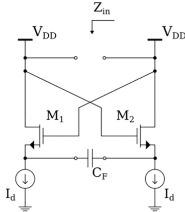
Figure 4-2 (adapted from [43]). A simplified Linvill OCS negative capacitor with two FETs
