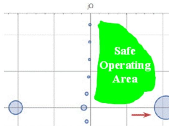
Figure 4-6 General strategy of improving stability properties of NIC/NIV circuits by avoiding potentially unstable areas in complex plane.
