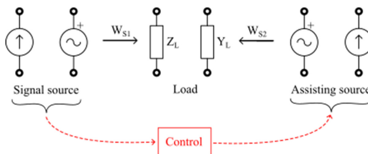
Figure 3-2 Basic idea of generation of electronic immittance by superposition of source signal and 'assisting source' signal. Here W_{s1} and W_{s2} denote energy flows caused by signal source and assisting source, respectively.
