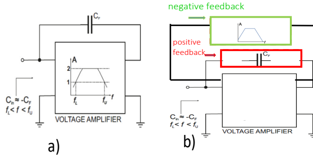
Figure 2-1 a) A basic idea stable 'bandpass' negative b) possible practical implementation [96]
