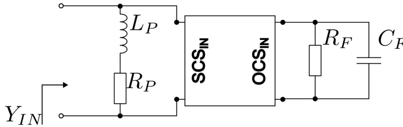
Figure 5-17 Compensated RL structure loaded with OCS negative resistance realized by Linvill NIC from Figure 5-8
