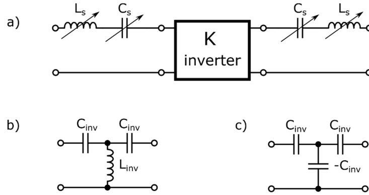
Figure 6-8 (a) Circuit diagram of a two-pole bandpass filter with an impedance inverter and two LC-resonators ( L_s C_s ). (b) Realization of a T-circuit impedance inverter where an equivalent inductor L_{inv} is used for the shunt branch. (c) Realization of an impedance inverter comprising two positive capacitors ( C_{inv} ) located in series branch and a negative ( -C_{inv} ) capacitor located in the shunt branch.
