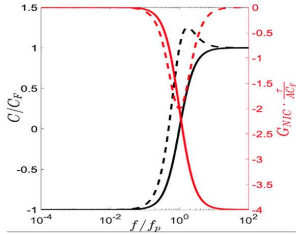
Figure 3-52 (adapted from [120]). Input capacitance (black) and conductance (red) of one-pole (solid) and two-pole (dashed) SCS negative capacitor; ( A_0=2, f_{p2}/f_{p1}=1.5 ).
