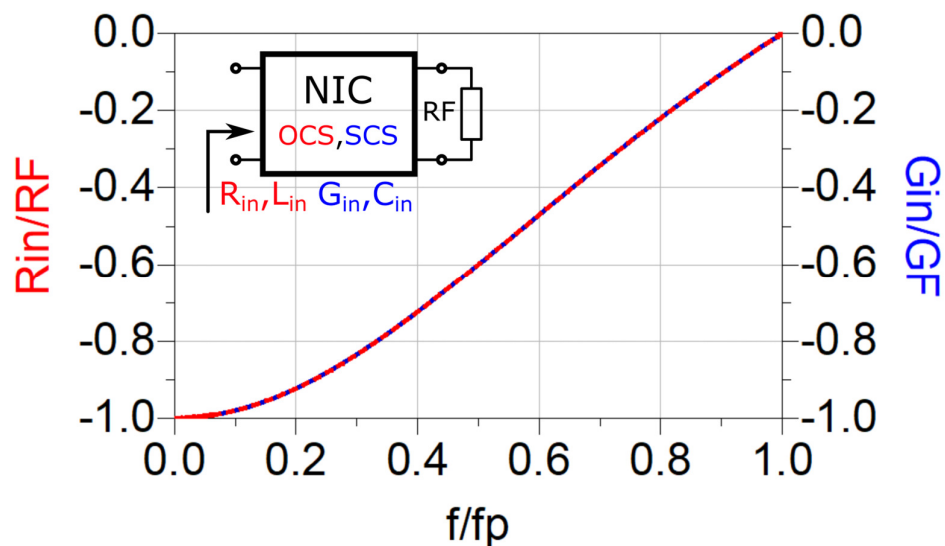
Figure 3-23 Dispersion of resistance/conductance of OCS/SCS negative resistor (OCS/SCS NIC terminated by ordinary resistor)
