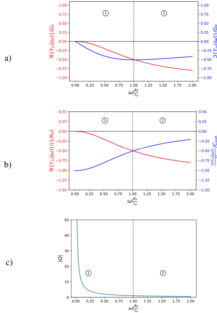
Figure 5-14 (a) Real and imaginary part of input impedance of series L_P and R_P compensated by SCS negative conductance. (b) Equivalent conductance and negative capacitance. (c) Quality factor of the circuit. Plots are obtained with \alpha = G_F/G_P = 1 and \beta = \omega_{pu}/\omega_{rc} = 200
