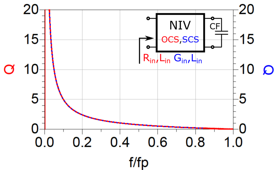
Figure 3-37 Q factor of OCS/SCS negative inductor (OCS/SCS NIV terminated by ordinary capacitor)
