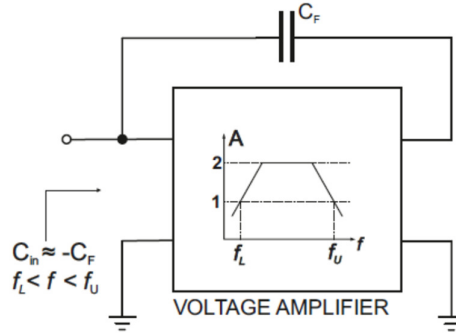
Figure 4-7 (taken from [96]) Implementation of a negative capacitor based on a voltage amplifier, using a ‘bandpass’ design that prevents occurrence of unstable ‘DC pole’
