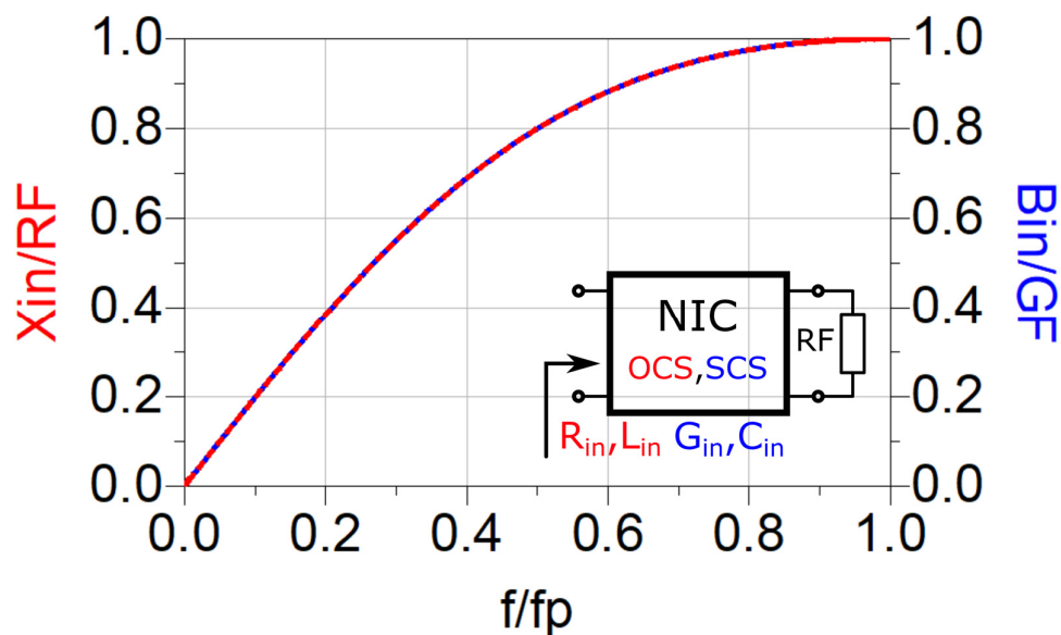
Figure 3-24 Dispersion of 'parasitic' reactance/susceptance of OCS/SCS negative resistance (input 'parasitic' reactance/susceptance of OCS/SCS NIC terminated by ordinary resistor)
