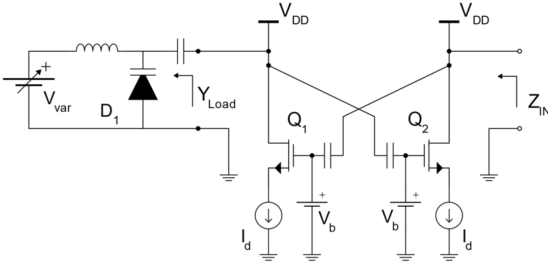
Figure 6-4 RF Koley tunable negative inductor in 40 nm CMOS technology. Gate bias networks are omitted for clarity. Q_1 = Q_2 : W = 32 \cdot 2 \mu\text{m} = 64 \mu\text{m} , L = 40 \text{ nm} . D_1 : W = 2 \mu\text{m} , L = 2 \mu\text{m} , multiplier = 20
