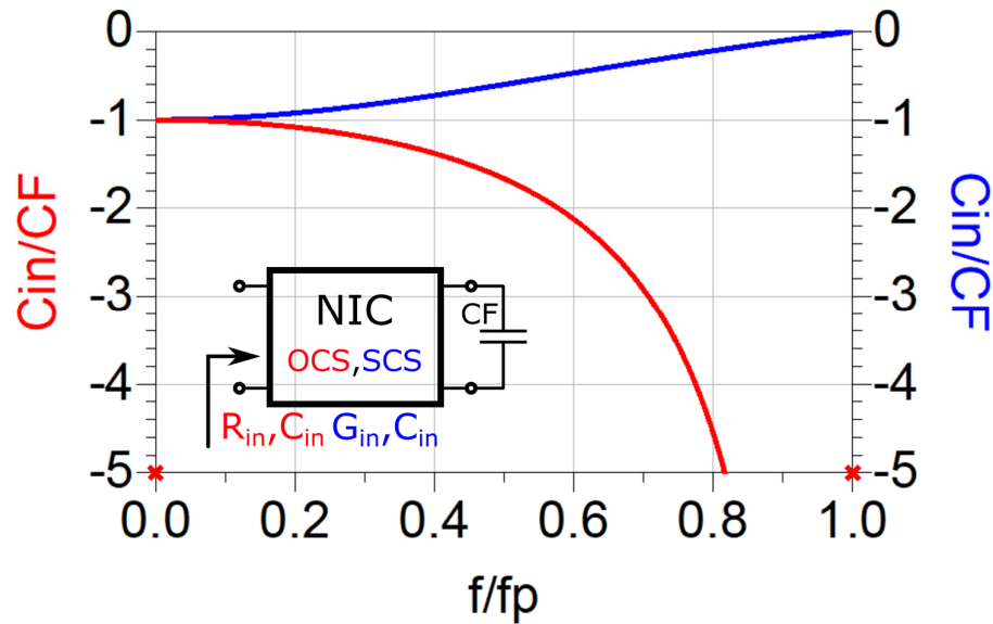
Figure 3-15 Dispersion of capacitance of OCS/SCS negative capacitor (OCS/SCS NIC terminated by ordinary capacitor)
