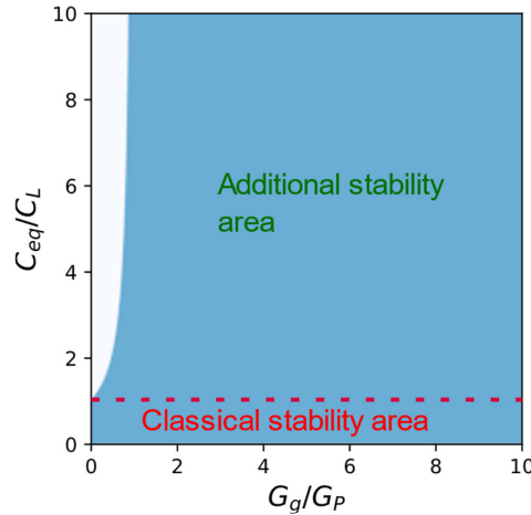
Figure 5-16 Stability area plot of compensated RL network loaded with positive inductance. Plot is generated with \alpha = G_F/G_P = 1 and \beta = \omega_{pu}/\omega_{rc} = 200 . Dark blue – range of normalized external impedances that cause stable operation; Light blue - range of normalized external impedances that cause unstable operation. Please note that in standard negative inductor based on one-pole NIC, maximal stability area would be bounded by C_{eq}/C_L < 1 .
