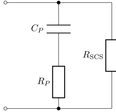
Figure 5-22 Schematic of series RC network compensated by SCS negative resistance.
