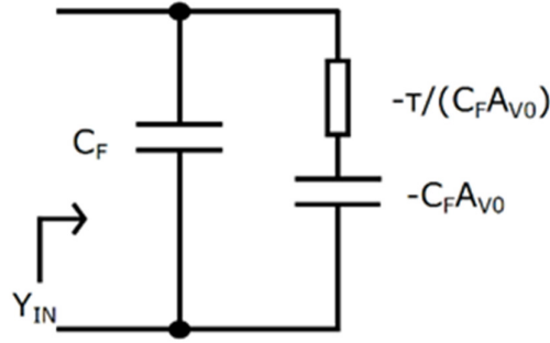
Figure 3-49 Equivalent circuit of SCS negative capacitor based on one-pole Miller NIC
