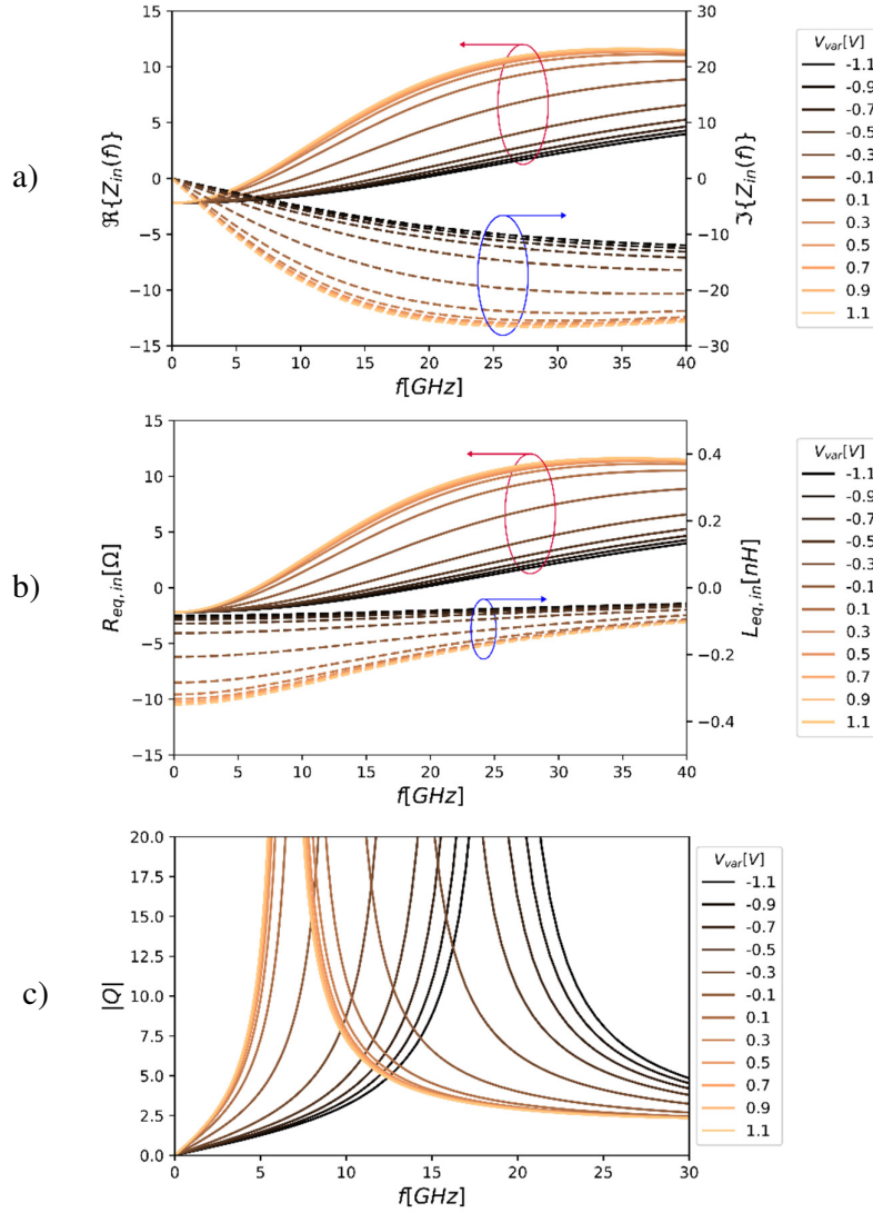
Figure 6-7 Tunable variable inductor obtained with Koley NIV a) Real and imaginary part of input impedance . b) Equivalent resistance and negative inductance. c) Quality factor Q of the circuit..
