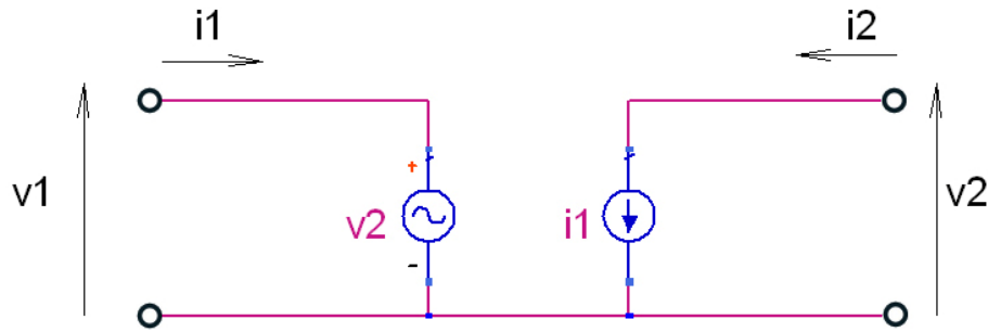
Figure 3-28 h-parameter model of an ideal INIC
