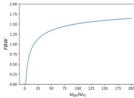
Figure 5-24 Plot of Fractional bandwidth (FBW) as a function of ratio of frequencies \omega_{pu}/\omega_{rc} and ratio of conductances \alpha = G_F/G_P = 0.961 .
