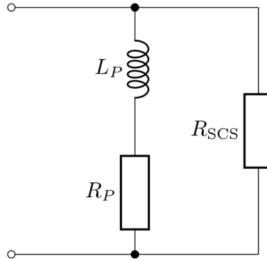
Figure 5-13 Schematic of series RL network compensated by SCS negative resistance.
