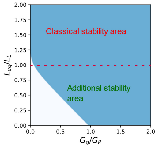
Figure 5-26 Comparison of stability regions of loaded compensated RC structure and loaded SCS negative inductance. Plot is generated with \alpha = G_F/G_P = 0.961 and \beta = \omega_{pu}/\omega_{rc} = 200 . Dark blue – range of external impedances that cause stable operation; Light blue - range of external impedances that cause unstable operation.
