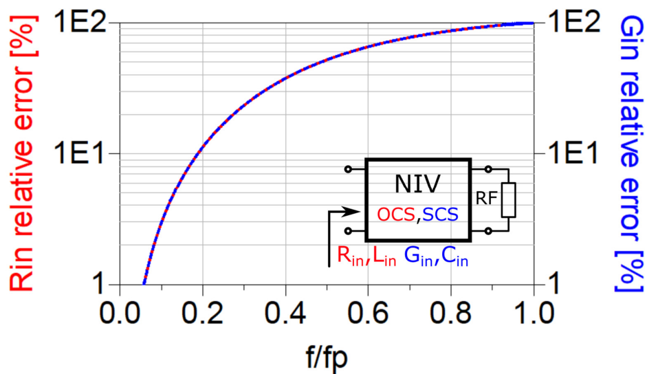
Figure 3-46 Relative error of resistance/conductance of OCS/SCS negative resistor (OCS/SCS NIV terminated by ordinary resistor)
