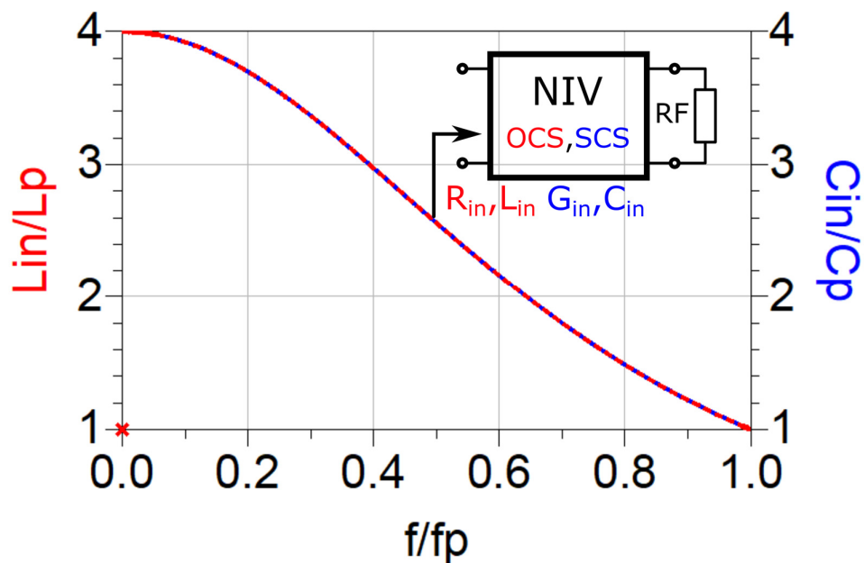
Figure 3-44 Dispersion of 'parasitic' inductance/capacitance of OCS/SCS negative resistance (input 'parasitic' inductance/capacitance of OCS/SCS NIV terminated by ordinary resistor)
