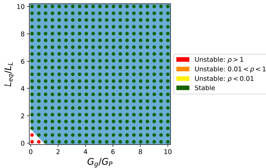
Figure 5-29 Stability area plot of compensated RC network loaded with positive inductance. Plot is generated R_P = 130 \, \Omega , C_P = 2.43 \, \text{pF} , R_F = 85 \, \Omega , C_F = 128 \, \text{fF} . Painted areas are calculated using simplified analytical approach (Dark blue – range of external impedances that cause stable operation; Light blue - range of external impedances that cause unstable operation). Colored dots are results predicted by commercial system identification software tool STAN TM . using STAN TM tool. This again shows that simplified analytical method of stability prediction can be used as starting point for subsequent numerical optimization.
