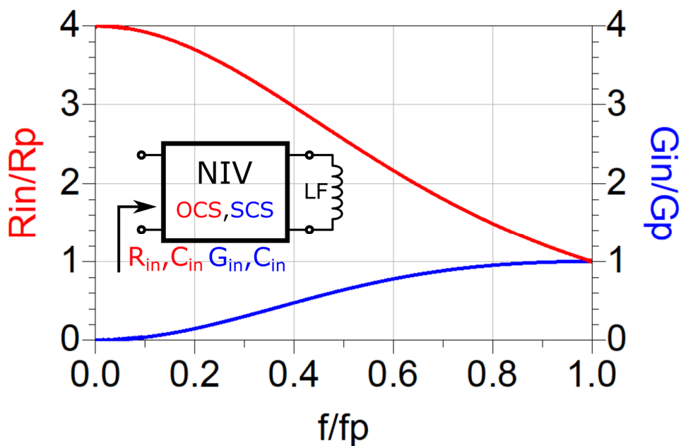
Figure 3-40 Dispersion of 'parasitic' resistance/conductance of OCS/SCS negative capacitance (input 'parasitic' resistance/conductance of OCS/SCS NIV terminated by ordinary inductor)
