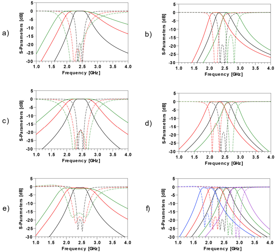
Figure 6-9 Frequency characteristics of different realizations of the proposed filter (S21 in solid lines, S11 in dotted lines). (a) Change of fractional bandwidth for the K-inverter using an inductor (10% black, 20% red, 30% green) and (b) tuning of central frequency (in black) 10% lower (red) and 10% higher (green). (c) Change of fractional bandwidth for the K-inverter using an ideal, dispersionless negative capacitor (10% black, 20% red, 30% green) and (d) tuning of central frequency (in black) 10% lower (red) and 10% higher (green). (e) Change of fractional bandwidth for the K-inverter using loss-compensated negative capacitance from chapter 5.4.1. (10% black, 20% red, 30% green) and (f) tuning of central frequency (in black) 10% lower (red), 20% lower (blue), 10% higher (green) and 20% higher (purple).
