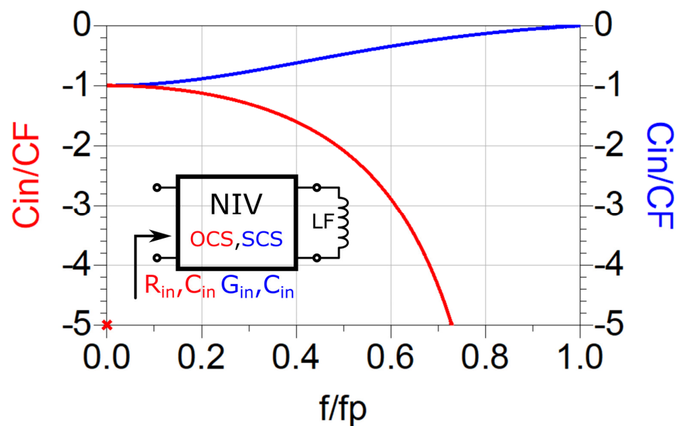
Figure 3-39 Dispersion of capacitance of OCS/SCS negative capacitor (OCS/SCS NIV terminated by ordinary inductor)
