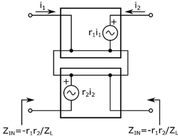
Figure 3-34 Basic OCS NII based on two trans-resistance amplifiers [103]
