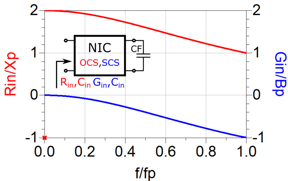
Figure 3-16 Dispersion of ‘parasitic’ resistance/conductance of OCS/SCS negative capacitor (OCS/SCS NIC terminated by ordinary capacitor)
