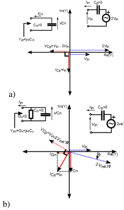
Figure 3-14 Phasor diagram for a negative capacitor based on SCS grounded INIC in Figure 3-10 (a). a) ideal case with zero-valued time delay (there is no phase shift in dependent voltage source) b) realistic case with finite time delay (there is a phase shift in dependent voltage source) (taken from [27]).
