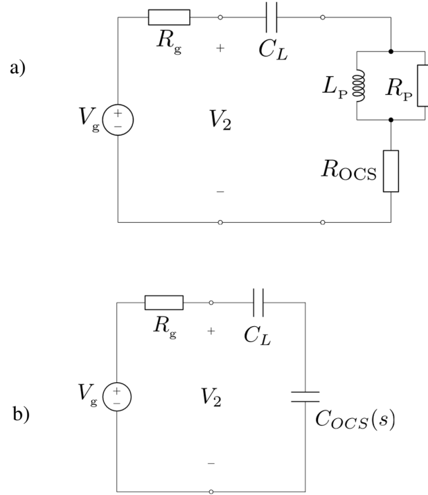
Figure 5-36 Stability testing schematics. a) Compensated RL network loaded with external network, b) ‘Classic’ negative capacitance constructed with OCS NIC
