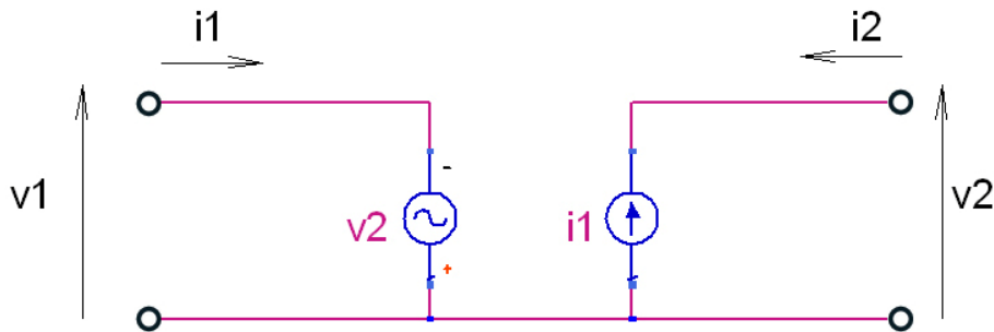
Figure 3-29 h-parameter model of an ideal VNIC
