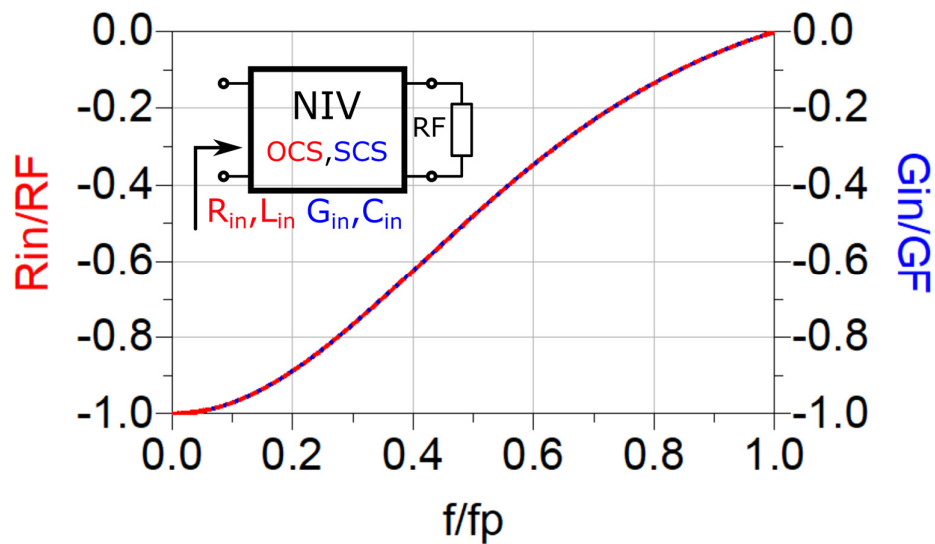
Figure 3-43 Dispersion of resistance/conductance of OCS/SCS negative resistor (OCS/SCS NIV terminated by ordinary resistor)
