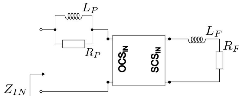
Figure 5-38 Compensated series RL structure loaded with OCS negative resistance.
