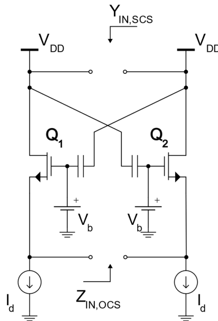
Figure 5-8 Linvill NIC used as compensating negative resistance of proposed negative inductor (designed in 40 nm CMOS technology; Q_1 = Q_2 , W = 32 \cdot 2 \mu\text{m} = 64 \mu\text{m} , L = 40 \text{ nm} . (Gate bias networks are omitted for clarity).
