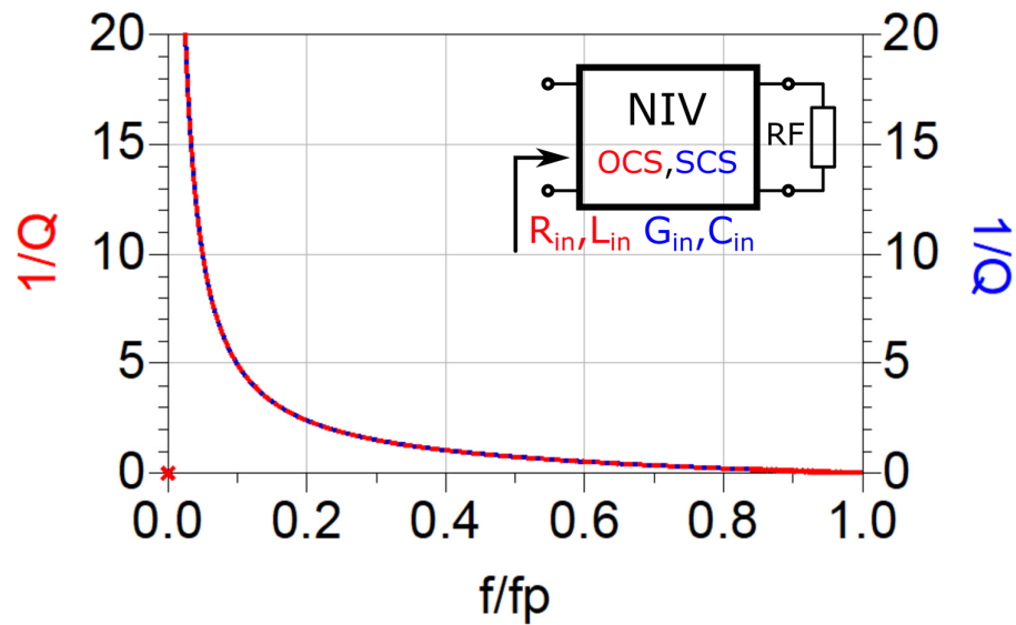
Figure 3-45 Q factor of OCS/SCS negative resistor (OCS/SCS NIV terminated by ordinary resistor)
