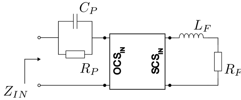
Figure 5-7 Compensated RC structure loaded with OCS negative resistance (based on Linvill NIC from Figure 5-8 )
