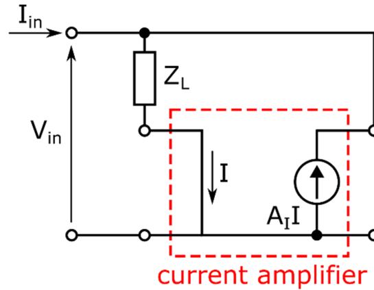
Figure 3-4 System for generation of electronic immittance based on ideal current amplifier with a load located in the positive feedback loop
