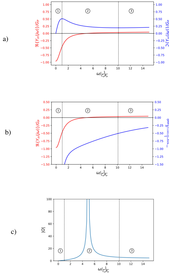
Figure 5-23 a) Real and imaginary part of input impedance of series C_P and R_P compensated by SCS negative conductance. b) Equivalent conductance and negative inductance. c) Quality factor Q of the circuit. Plots are obtained with \alpha = G_F/G_P = 0.961 and \beta = \omega_{pu}/\omega_{rc} = 200
