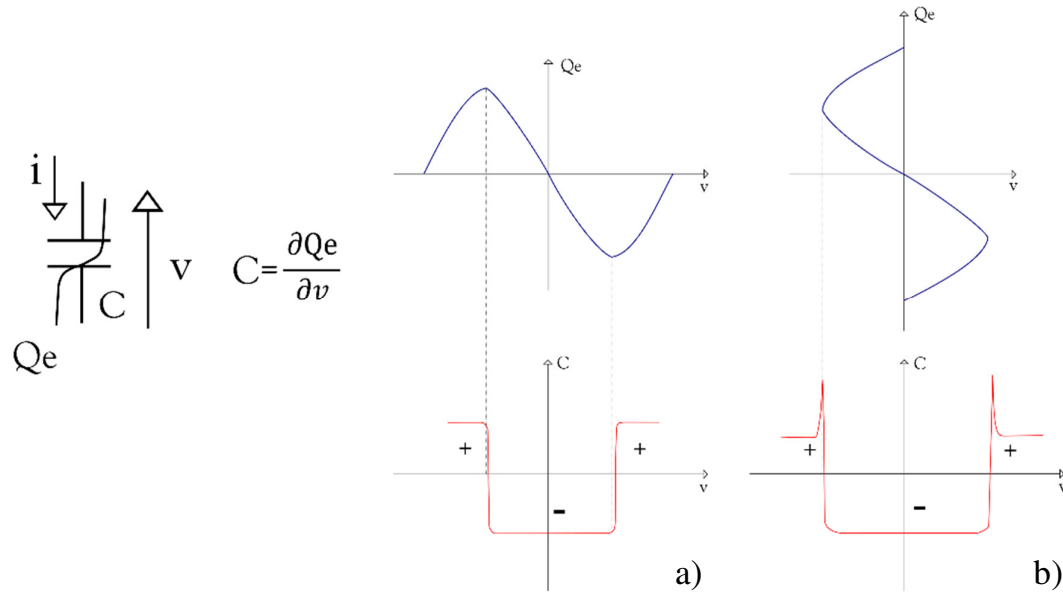
Figure 3-6 Generalized curves of non-linear negative capacitor a) 'N' curve, b) 'S' curve (taken from [44])
