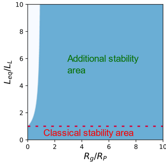
Figure 5-6 Stability area plot of compensated RC network loaded with positive inductance. Plot is generated with A = R_F/R_P = 1 and \beta = \omega_{pu}/\omega_{rc} = 200 . Dark blue – range of normalized external impedances that cause stable operation; Light blue - range of normalized external impedances that cause unstable operation. Please note that in standard negative inductor based on one-pole NIC, maximal stability area would be bounded by L_{eq}/L_L < 1 .
