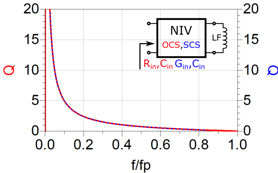
Figure 3-41 Q factor of OCS/SCS negative capacitor (OCS/SCS NIV terminated by ordinary inductor)
