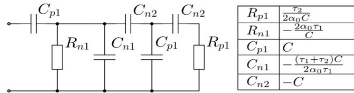
Figure 4-11. (adapted from [107]). Equivalent circuit of 2-pole band-pass OCS negative capacitor
