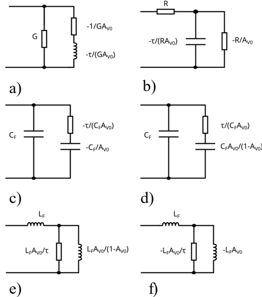
Figure 3-50 Equivalent circuits of various SCS/OCS non-Foster and Negative elements generated using one-pole NICs. (a) SCS negative conductance; (b) OCS negative resistance; (d) SCS negative capacitance; (e) SCS negative inductance; (f) OCS negative inductance
