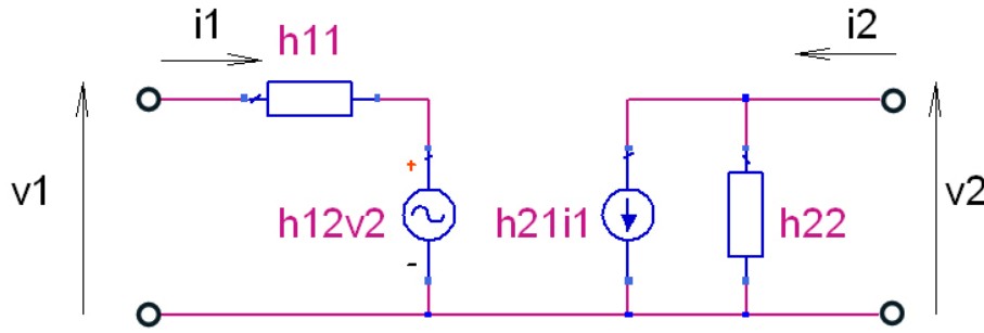
Figure 3-27 General NIC modelled with h-parameters
