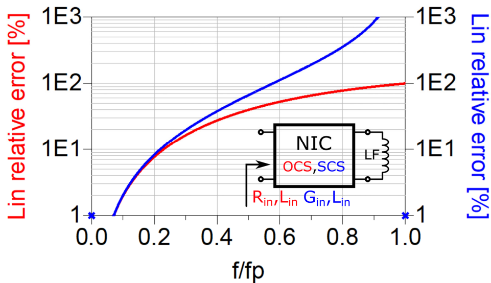
Figure 3-22 Relative error of inductance of OCS/SCS negative inductor (OCS/SCS NIC terminated by ordinary inductor)
