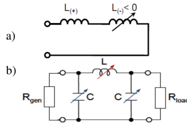
Figure 2-2 a) An idea of tunable non-Foster inductor, b) possible implementation in band-pass filter [42]
