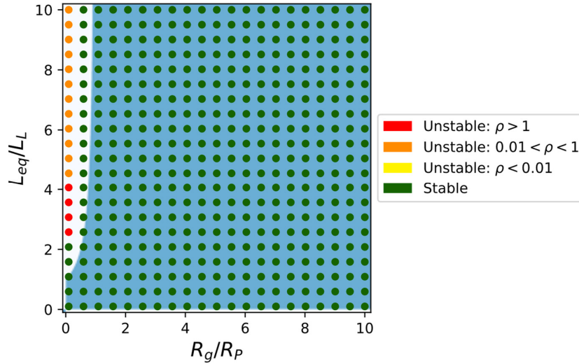
Figure 5-10 Stability area plot of compensated RC network loaded with positive inductance. Plot is generated with R_P = 303 \, \Omega , C_P = 105 \, \text{fF} , R_F = 405 \, \Omega , L_F = 1.8 \, \text{nH} . Painted areas are calculated using simplified analytical approach (Dark blue – range of external impedances that cause stable operation; Light blue - range of external impedances that cause unstable operation). Colored dots are results predicted by commercial system identification software tool STAN TM .
