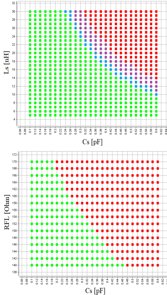
Figure 6-10 Stability analysis of the proposed tunable filter. The results are presented with respect to: (upper) Change of LC-resonator values C_s and L_s depicting the change of fractional bandwidth obtainable while having stable operating conditions. For R_{FL}=157\Omega only green part is stable, while others are unstable, for R_{FL}=154\Omega both blue and green are stable combinations while purple and red are unstable and for R_{FL}=149\Omega only red part is unstable while all rest depict stable operations. (lower) Change of LC-resonator capacitor C_s and R_{FL} used in the negative capacitance depicting the tunability of the central frequency.
