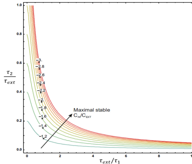
Figure 4-8 (taken from [96]) Bandpass negative capacitor – Contour plot of maximal stable normalized negative capacitance (obtained analytically)
