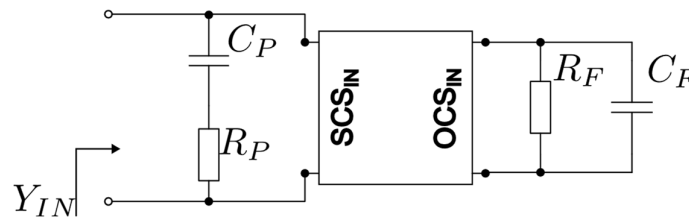
Figure 5-27 Compensated series RL structure loaded with OCS negative resistance.
