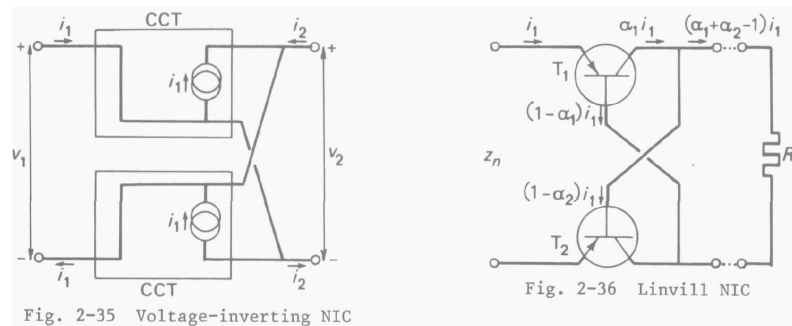
Figure 4-1 (taken from [103]). Direct comparison of differential NIC with two ideal current amplifiers with unity-gain current amplifier and Linvill NIC [16].
