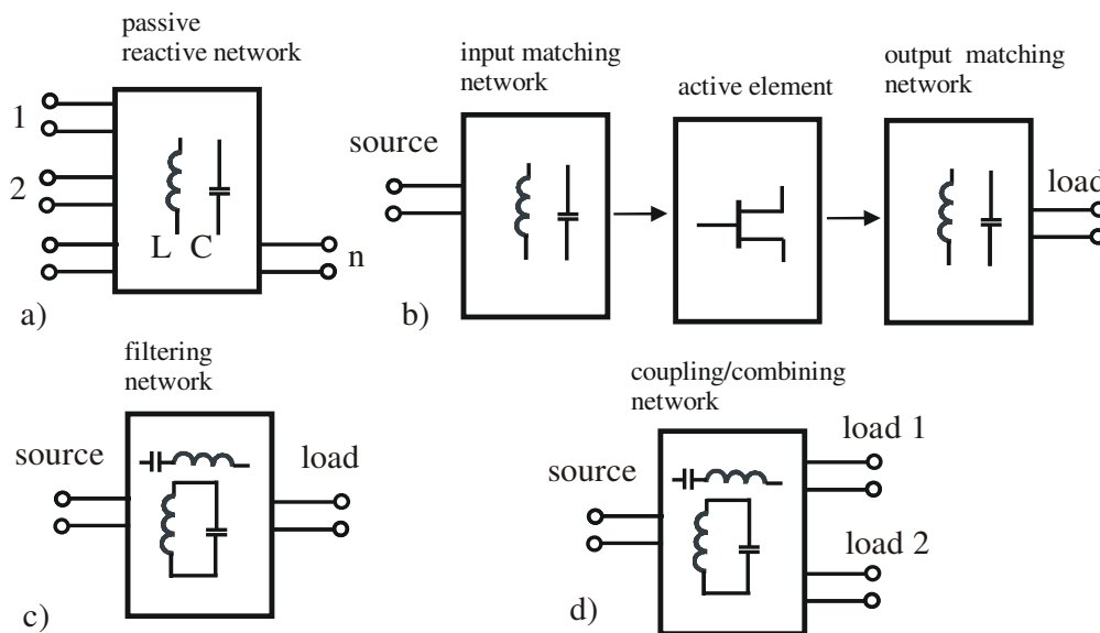
Figure 1-1 a) Definition of a passive reactive network, b) Reactive network as a matching block in an RF amplifier, c) Reactive network as a filtering structure, d) Reactive network as a coupling/splitting/combining structure
