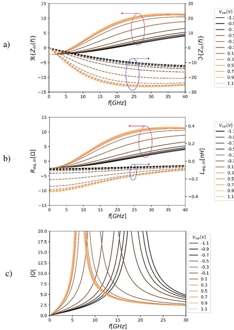
Figure 6-5 Tunable variable inductor obtained with Koley NIV a) Real and imaginary part of input impedance . b) Equivalent resistance and negative inductance. c) Quality factor Q of the circuit.
