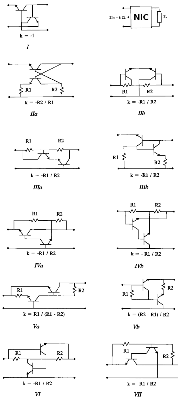
Figure 4-3 Different designs of NIC circuits with two BJTs (taken from [110])
