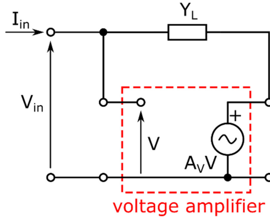
Figure 3-3 System for the generation of electronic immittance based on ideal voltage amplifier with load in positive feedback
