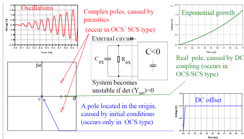
Figure 4-5 Possible types of unstable (RHS) poles that may occur in system that comprises NIC/NII and some external passive network. The graphs have been generated for the case of Miler negative capacitor loaded with external shunt RC network.
