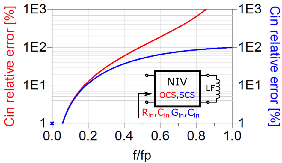
Figure 3-42 Relative error of capacitance of OCS/SCS negative capacitor (OCS/SCS NIV terminated by ordinary inductor)
