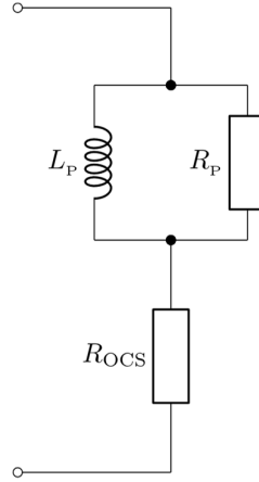
Figure 5-34 Schematic of shunt RL network that emulates negative capacitance, compensated by series OCS negative resistance.
