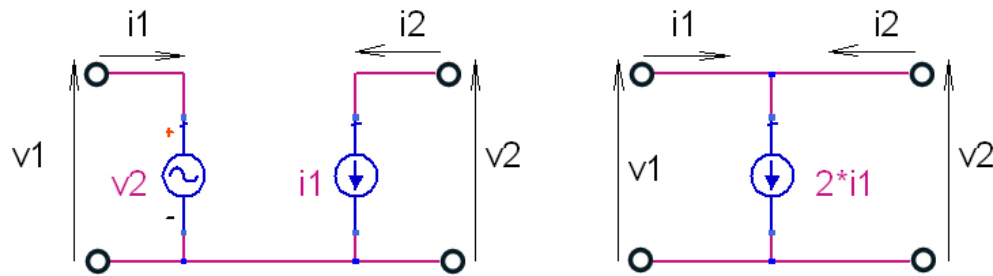
Figure 3-30 Transformation of basic INIC into a circuit with a single current source
