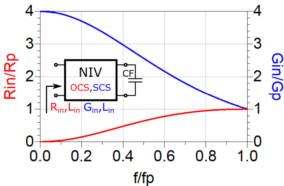
Figure 3-36 Dispersion of 'parasitic' resistance/conductance of OCS/SCS negative inductance (input 'parasitic' resistance/conductance of OCS/SCS NIV terminated by ordinary capacitor)
