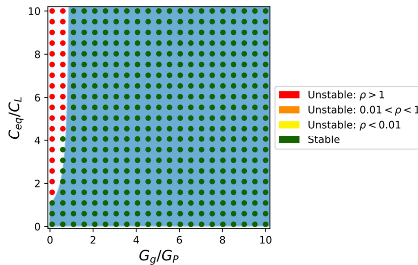
Figure 5-19 Stability area plot of compensated RL network loaded with positive inductance. Plot is generated with the following parameters R_P = 39 \, \Omega , L_P = 1.21 \, \text{nH} , R_F = 1 \, \Omega , C_F = 111 \, \text{fF} . Painted areas are calculated using simplified analytical approach (Dark blue – range of external impedances that cause stable operation; Light blue - range of external impedances that cause unstable operation). Colored dots are results predicted by commercial system identification software tool STAN TM .
