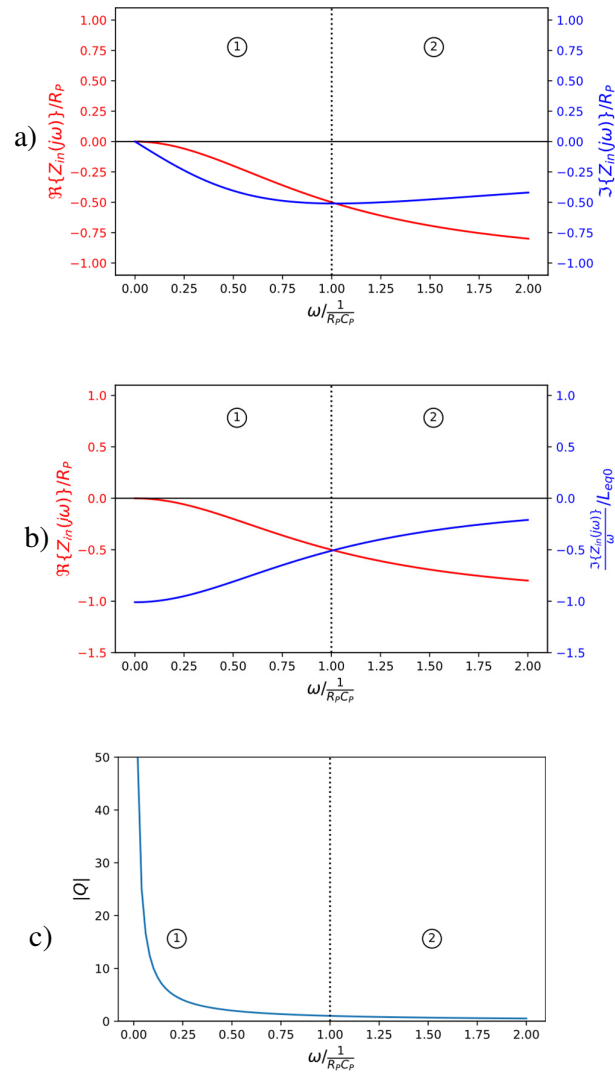
Figure 5-4 (a) Real and imaginary part of input impedance of parallel C_P and R_P compensated by OCS negative resistance. (b) Equivalent resistance and negative inductance. (c) Quality factor Q of the circuit. Plots are obtained with A = R_F/R_P = 1 and \beta = \omega_{pu}/\omega_{rc} = 200
