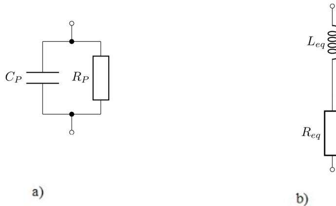
Figure 5-1 Schematic of parallel RC network (a) and its equivalent Z_{IN}(\omega(j\omega)) representation in j\omega domain (b)
