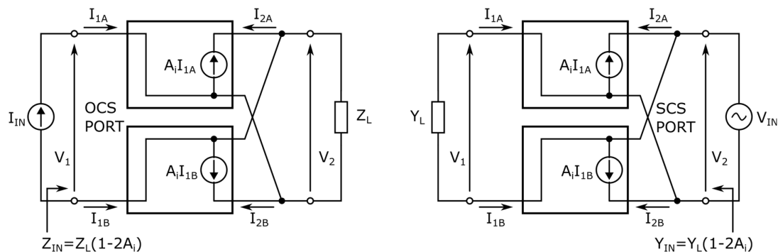
Figure 3-12 Basic schematics of floating voltage inversion NICs (VNIC) based on two ideal current amplifiers. a) OCS implementation, b) SCS implementation
