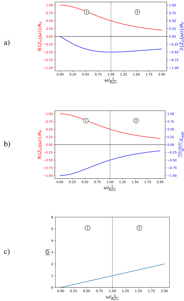
Figure 5-2 Real and imaginary part of input impedance of parallel C_P and R_P (a). Equivalent resistance and negative inductance (b). Quality factor Q of the circuit (c)
