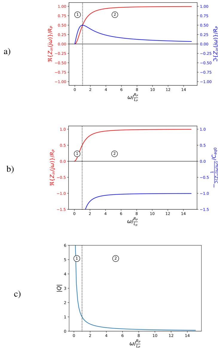
Figure 5-33 a) Real and imaginary part of input impedance of parallel L_P and R_P . b) Equivalent resistance and negative capacitance. c) Quality factor Q
