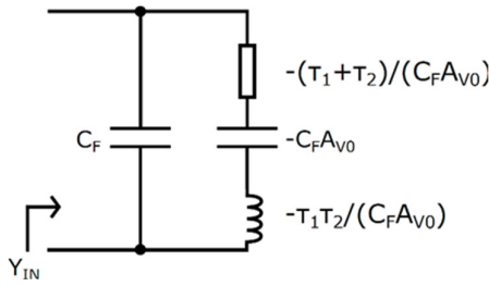
Figure 3-51 (adapted from [120]). Equivalent circuit of SCS negative capacitor based on two-pole NIC.
