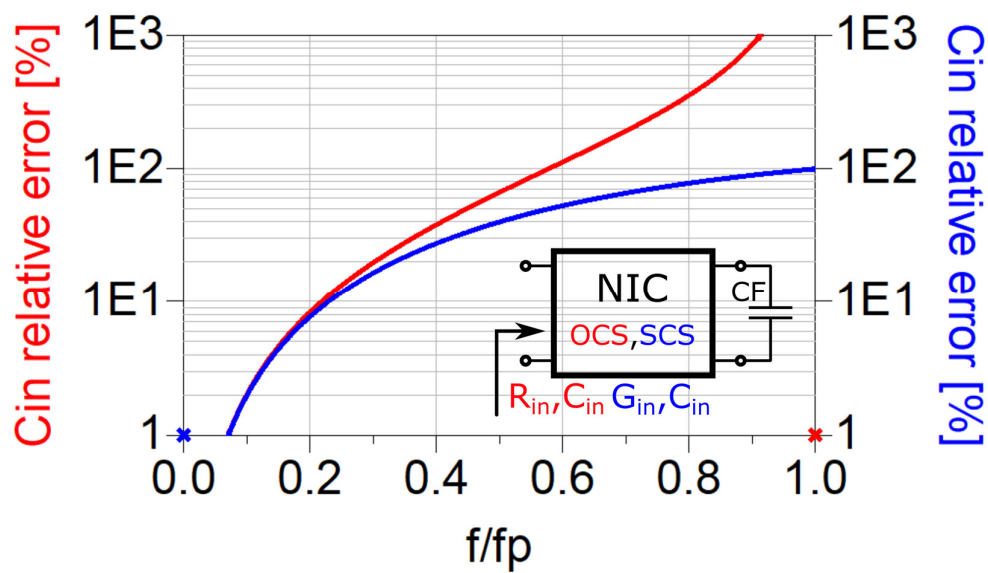
Figure 3-18 Relative error of capacitance of OCS/SCS negative capacitor (OCS/SCS NIC terminated by ordinary capacitor)
