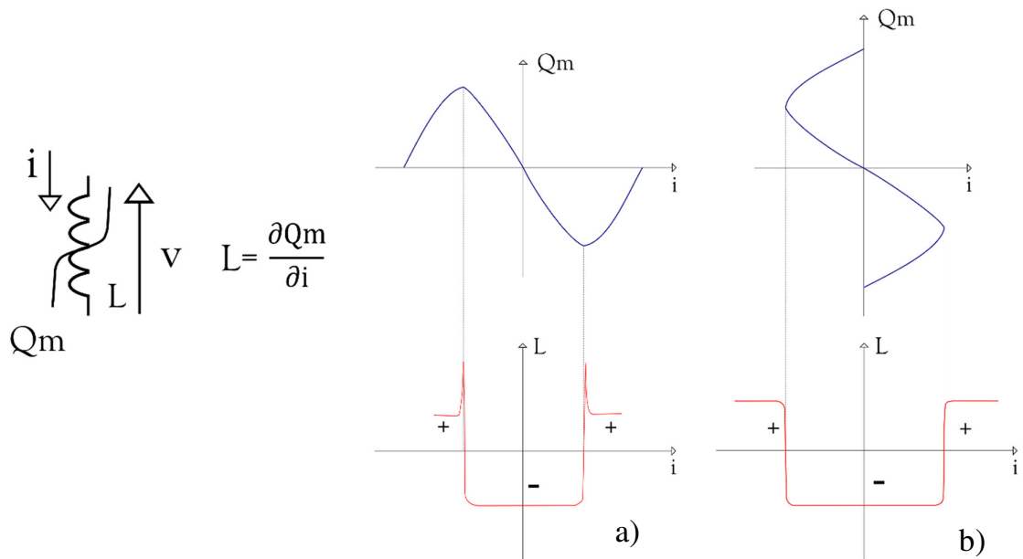
Figure 3-7 Generalized curves of a non-linear negative inductor a) 'N' curve, b) 'S' curve (taken from [44])
