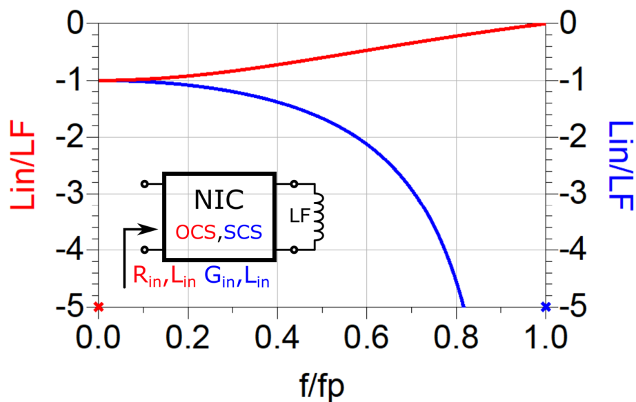
Figure 3-19 Dispersion of inductance of OCS/SCS negative inductor (OCS/SCS NIC terminated by ordinary inductor)
