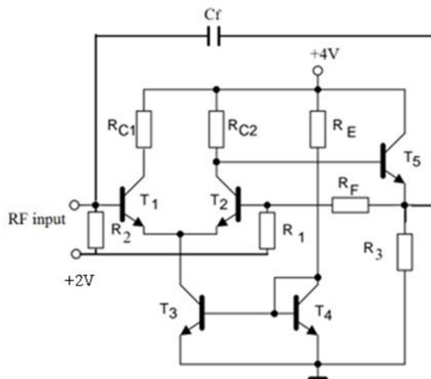
Figure 6-1 Simple SCS Miller negative capacitor that mimics low-frequency OPamp approach. The circuit is designed in HCBT technology.
