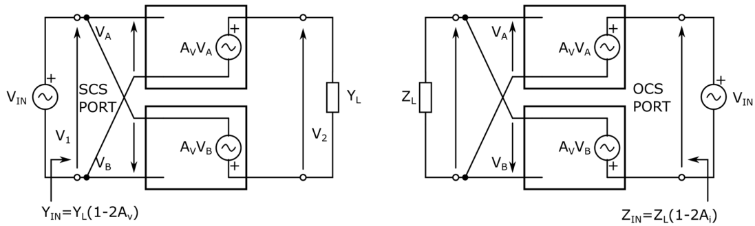
Figure 3-13 Basic schematics of floating current inversion NICs (INIC) based on two ideal voltage amplifiers. a) SCS implementation, b) OCS implementation
