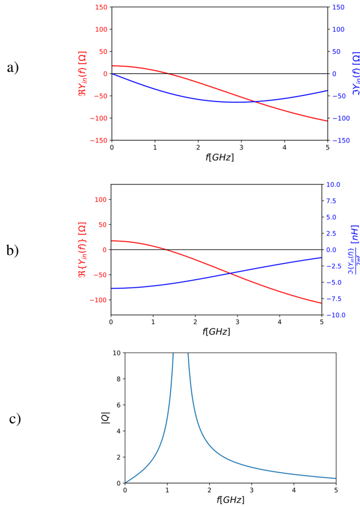
Figure 5-9 Real and imaginary part of input impedance of parallel C_P and R_P compensated by OCS negative resistance (a). Equivalent resistance and negative inductance (b). Quality factor Q of the circuit. Plots are obtained with R_P = 303 \Omega , C_P = 105 \text{ fF} , R_F = 405 \Omega , L_F = 1.8 \text{ nH}
