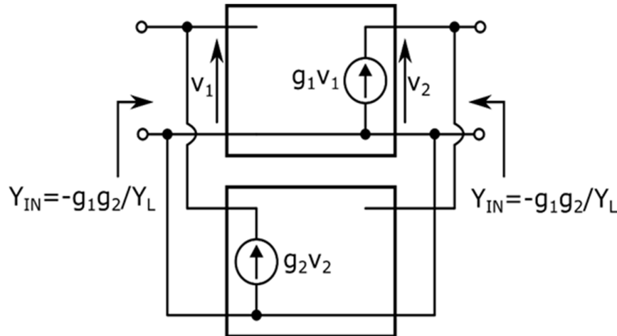
Figure 3-33 Basic SCS NII based on two trans-conductance amplifiers [103]
