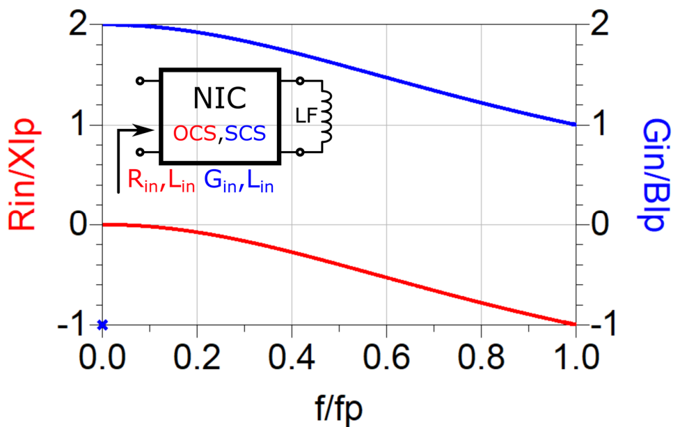
Figure 3-20 Dispersion of ‘parasitic’ resistance/conductance of OCS/SCS negative inductor (OCS/SCS NIC terminated by ordinary inductor)
