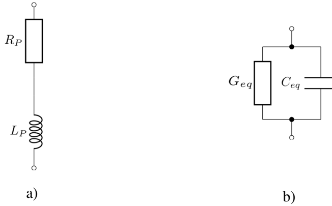
Figure 5-11 Schematic of series R_L network (a) and its equivalent Y_{in}(j\omega) representation in j\omega domain (b)
