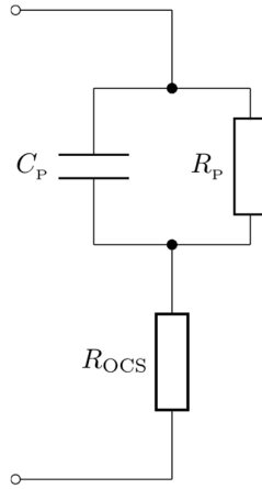
Figure 5-3 Schematic of parallel RC network compensated by OCS negative resistance.
