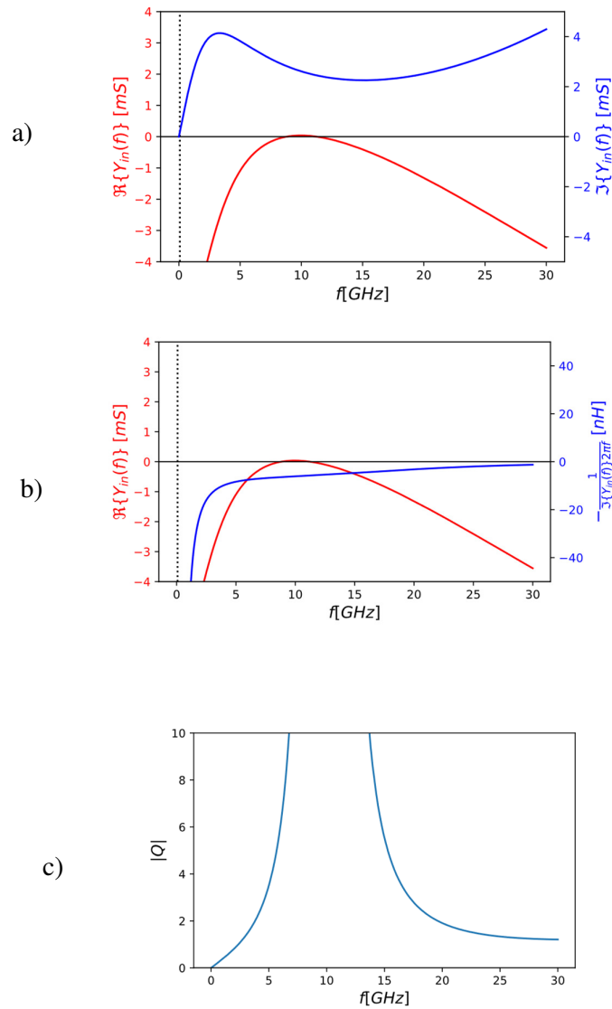
Figure 5-30 a) Real and imaginary part of input impedance of series C_P and R_P compensated by OCS negative resistance. b) Equivalent resistance and negative inductance. c) Quality factor Q of the circuit. Plots are obtained with R_P = 120 \, \Omega , C_P = 398 \, \text{fF} , R_F = 86 \, \Omega , C_F = 122 \, \text{fF} .
