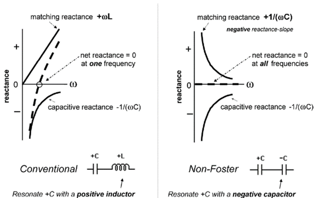
Figure 1-3 Comparison of passive matching (left) and active non-Foster matching (right) of a highly capacitive load (Figure copied from [8], copyrighted to IEEE)
