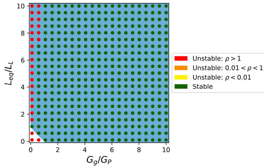
Figure 5-31 Stability area plot of compensated RC network loaded with positive inductance. Plot is generated using : R_P = 120 \, \Omega , C_P = 398 \, \text{fF} , R_F = 86 \, \Omega , C_F = 122 \, \text{fF} . Painted areas are calculated using simplified analytical approach (Dark blue – range of external impedances that cause stable operation; Light blue - range of external impedances that cause unstable operation). Colored dots are results predicted by commercial system identification software tool STAN TM .
