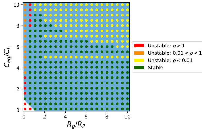
Figure 5-40 Stability area plot of compensated RC network loaded with positive inductance. Plot is generated R_P = 14 \, \Omega , L_P = 2.96 \, \text{nH} , R_F = 54.5 \, \Omega , L_F = 210 \, \text{pH} . Painted areas are calculated using simplified analytical approach (Dark blue – range of external impedances that cause stable operation; Light blue - range of external impedances that cause unstable operation). Colored dots are results predicted by commercial system identification software tool STAN TM .
