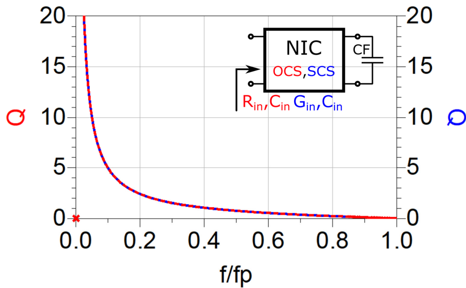
Figure 3-17 Q factor of OCS/SCS negative capacitor (OCS/SCS NIC terminated by ordinary capacitor)
