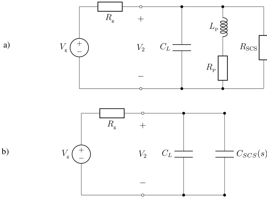
Figure 5-15 Networks used in stability analysis. a) Compensated RL network loaded with external network, b) ‘Classical’ negative capacitance constructed with SCS NIC
