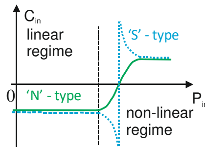
Figure 3-9 Dependence of input capacitance on input signal for circuits in Figure 3-3 and Figure 3-4, assuming the ‘N’ and ‘S’ types of non-linearity, respectively (taken from [44])
