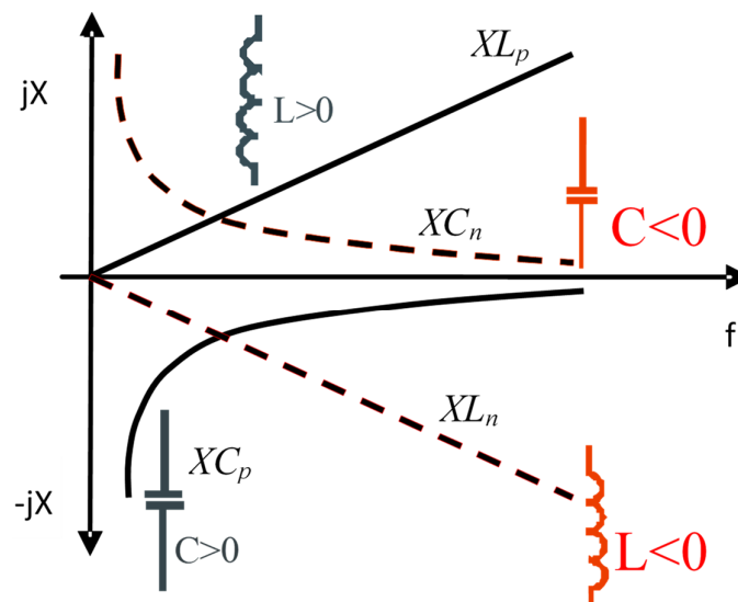
Figure 1-2 Solid: Reactance of positive (Foster) reactive elements, Dashed: Reactance of negative (non-Foster) reactive elements (taken from [7]).
