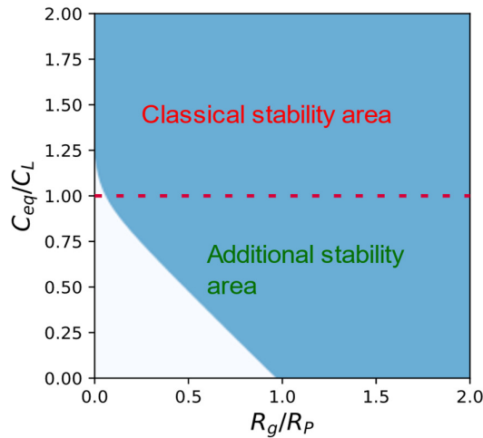
Figure 5-37 Stability area plot of compensated RC network loaded with positive inductance. Plot is generated with \alpha = R_F/R_P = 0.961 and \beta = \omega_{pu}/\omega_{rc} = 200 . Dark blue – range of external impedances that cause stable operation; Light blue - range of external impedances that cause unstable operation. Please note that in standard negative inductor based on one-pole NIC, maximal stability area would be bounded by C_{eq}/C_L > 1
