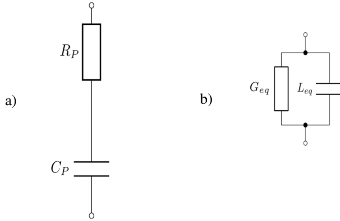
Figure 5-20 Schematic of series RC network (a) and its equivalent Y_{in}(j\omega) representation in j\omega domain (b)
