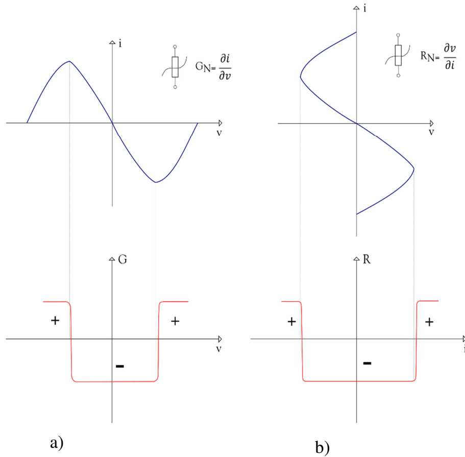
Figure 3-5 Voltage-current curves of negative conductance/resistance elements a) ‘N’ curve, b) ‘S’ curve (adapted from [44])
