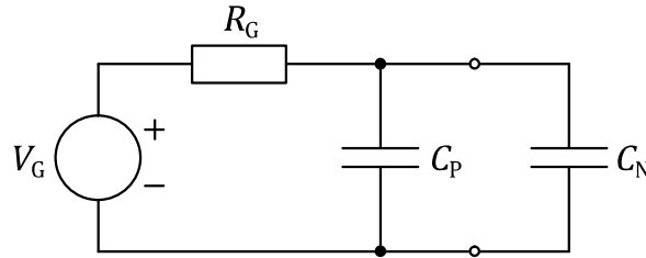
Figure 3-47 Basic network with a parallel combination of positive and negative capacitor, used in stability prediction. Negative capacitor is modelled using a realistic one-pole model
