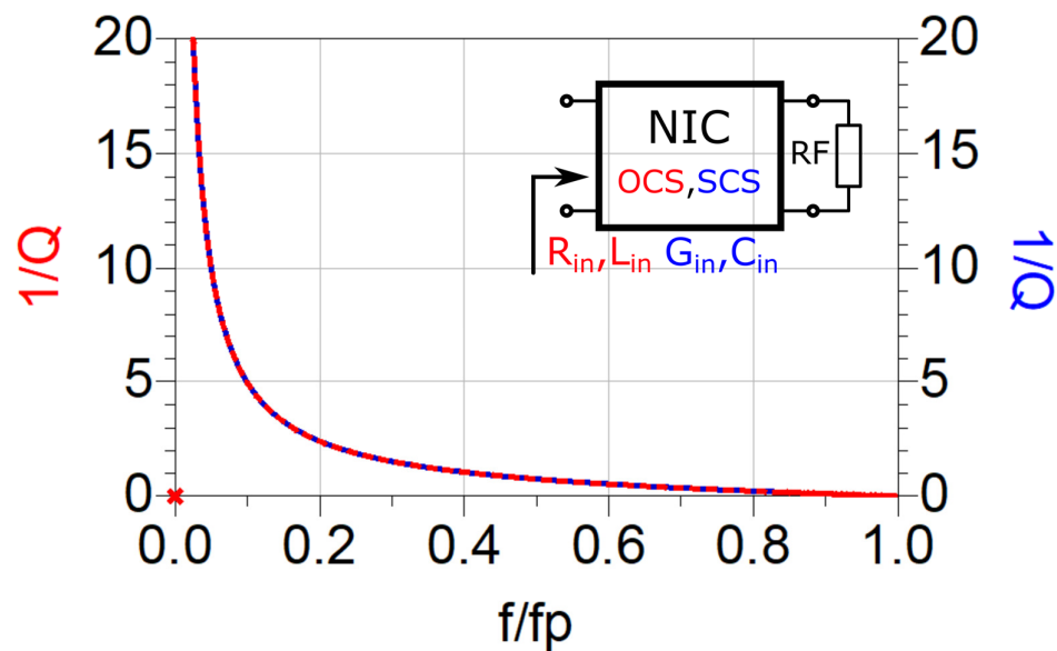
Figure 3-25 Q factor of OCS/SCS negative resistor (OCS/SCS NIC terminated by ordinary resistor)
