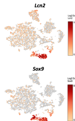
Figure 4. Differentially expressed neural crest markers in Tsc2 +/- mice kidney tumors, include Lcn2 and Sox9 .
