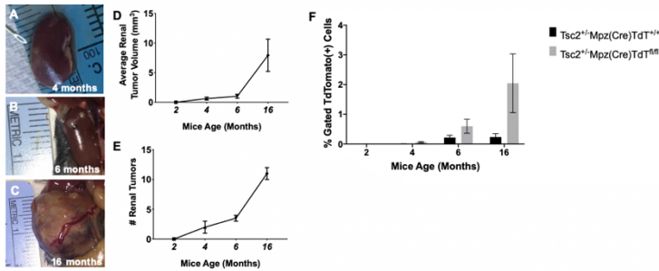
Figure 2: Identification of Neural Crest Lineage Cells in Ectopic Renal Tumor Onset of the Tsc2 +/- mice – A) Earliest reported detection of ectopic renal tumors in the Tsc2 +/- Mpz(Cre)TdT fl/fl mice begins at 4 months of age (A) then pictured at 6 months (B) and at 16 months (C). Tumor volume (D) and number (E) increased proportionally during the same period. Tumors from Tsc2 +/- Mpz(Cre)TdT fl/fl mice were
