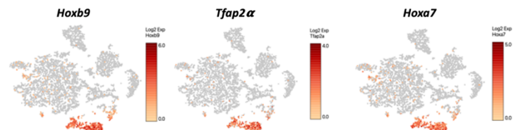
Figure 3. Single Cell Transcriptomic Analysis of TSC tumors in Tsc2 -/- Mpz ( Cre ) TdY fl/fl mice.
