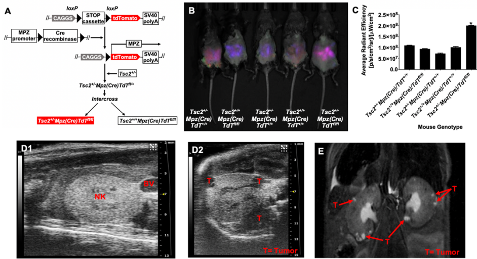
Figure 1: Generation of Tuberous Sclerosis Reporter Mouse Model and Imaging Techniques for Visualizing TS tumors – A) Schematic of genetic crosses to generate Tsc2 +/- reporter mouse models show floxed R26Sor tm9 (CAG-tdTomato) Hze mice (n=10 animals) were crossed with Tg(Mpz-Cre)26Mes mice (n=10 animals) expressing Cre recombinase under the control of myelin protein zero (MPZ) promoter. Mpz(Cre) tm1.1JDar mouse progeny (n=8 animals) were then
