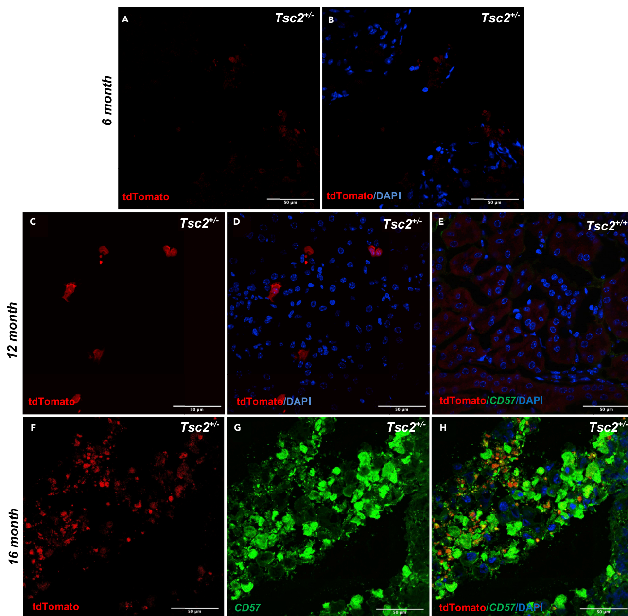
Figure 4. Visualizing neural crest lineage cells in Tsc2^{+/-} mouse renal tumors
