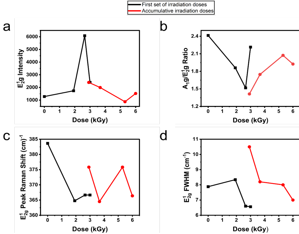
Figure 14. (a) E 2g 1 peak intensity as a function of irradiation dose. (b) A 1g /E 2g 1 peak intensity ratio as a function of irradiation dose. (c) E 2g 1 peak Raman shift as a function of irradiation dose. (d) E 2g 1 peak full width half maximum (FWHM) as a function of irradiation dose
