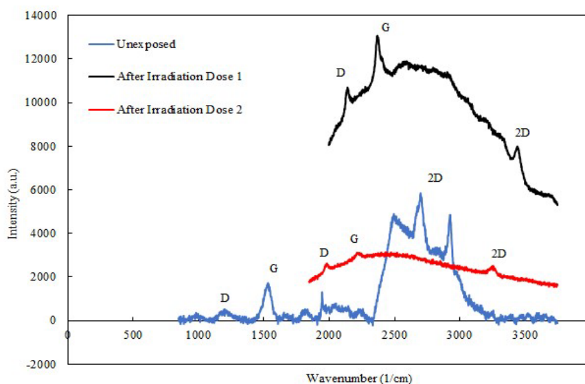
Figure 8. Raman spectra of CVD graphene grown on copper substrate, with and without irradiation doses for sample-3
