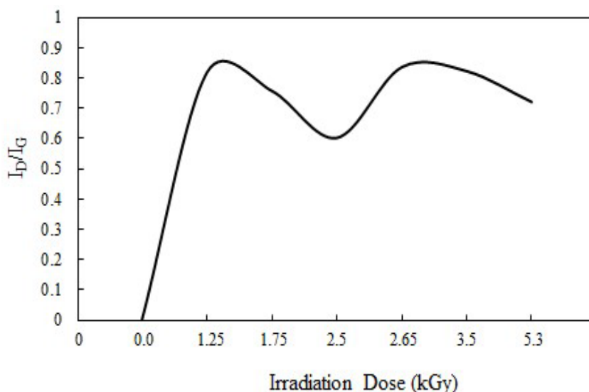
Figure 10. Evolution of I_D/I_G curve as a function of irradiation dose for graphene grown over copper substrate
