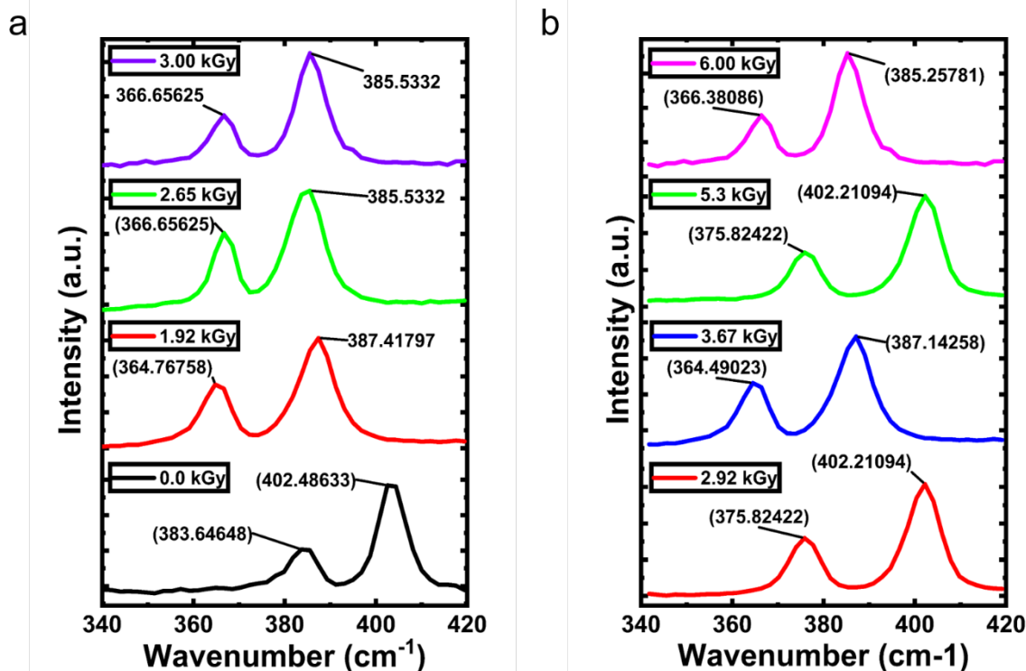
Figure 13. (a) Raman spectra results of monolayer MoS 2 after the first set of irradiation doses. (b) Raman spectra results of monolayer MoS 2 after the second set of irradiation doses (cumulative doses)
