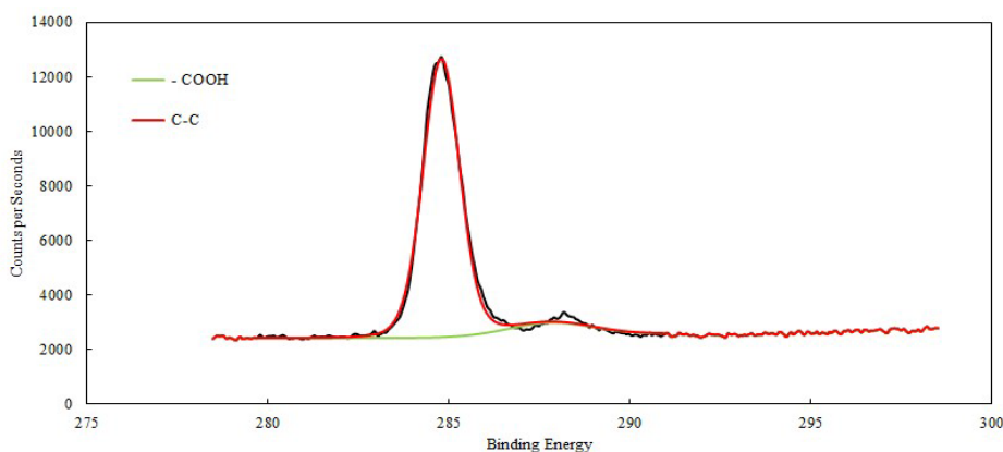
Figure 11. XPS studies of CVD graphene grown on nickel substrate (unexposed)
