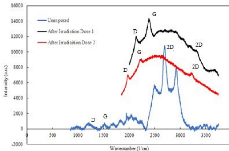
Figure 7. Raman spectra of CVD graphene grown on copper substrate, with and without irradiation doses for sample-2
