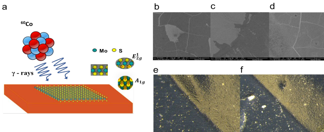
Figure 12. (a) Gamma irradiation on monolayer MoS 2 over copper substrate. (b) SEM image of pristine MoS 2 . (c) SEM image of irradiated MoS 2 with 1.92 kGy. (d) SEM image of irradiated MoS 2 with cumulative dose of 5.30 kGy. (e) Optical image of pristine MoS 2 . (f) Optical image of irradiated MoS 2 with cumulative dose of 6.0 kGy
