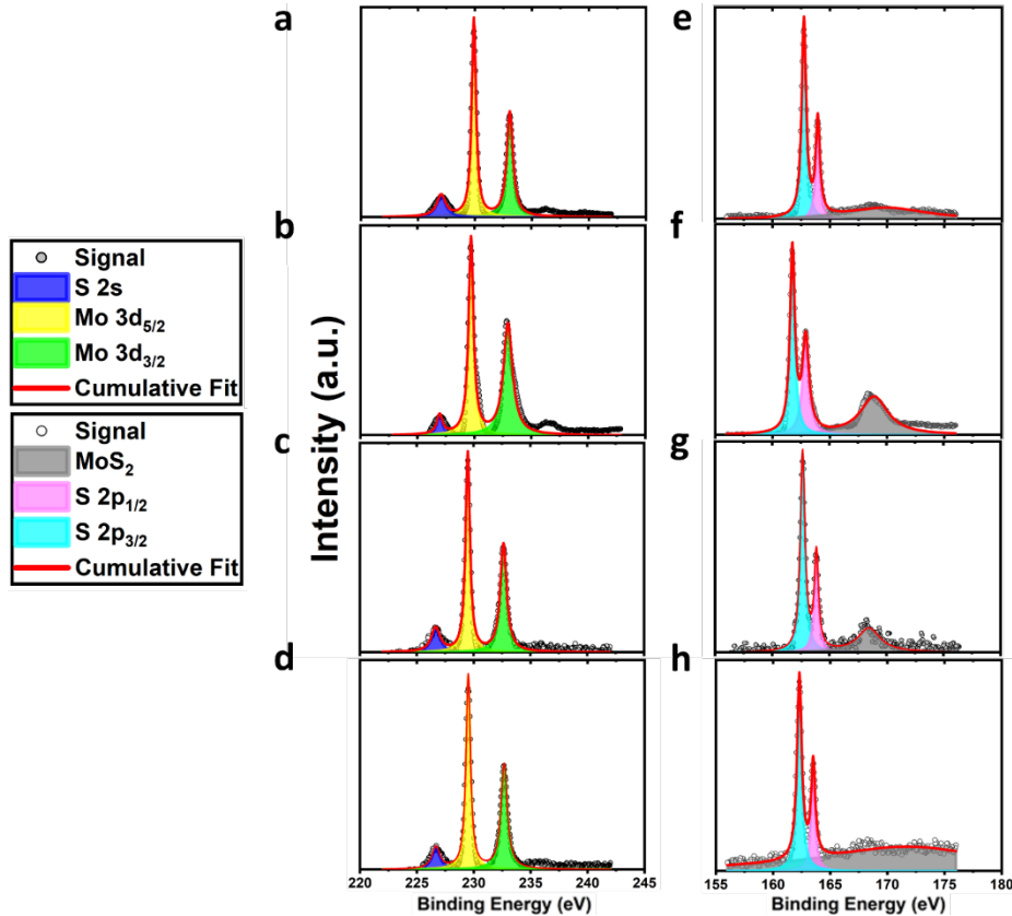
Figure 15. XPS spectra of MoS 2 . Mo d components with (a) 0 kGy; (b) 1.0 kGy; (c) 1.75 kGy; (d) 2.65 kGy of irradiation. S 2p components with (e) 0 kGy; (f) 1.00 kGy; (g) 1.75 kGy; (h) 2.65 kGy of irradiation
