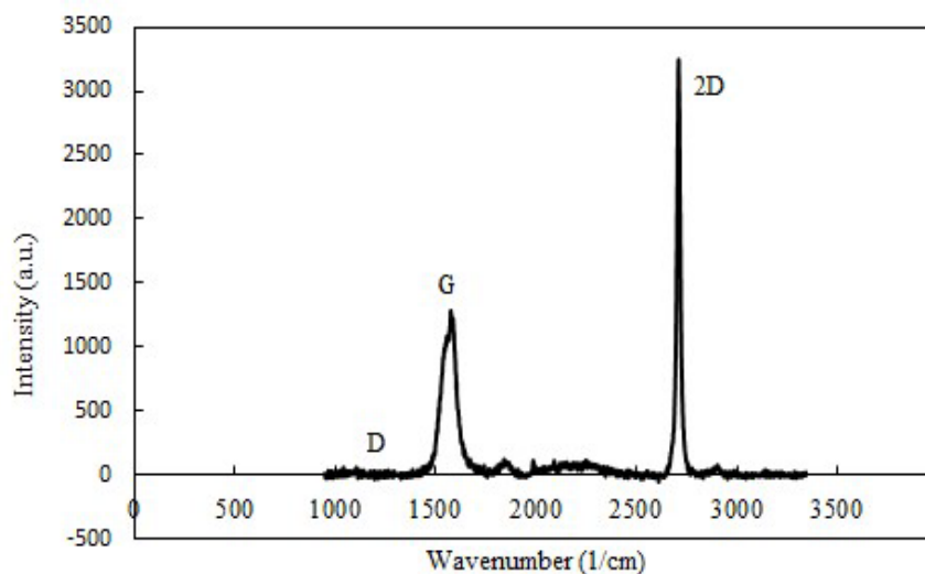
Figure 2. Raman spectrum of monolayer graphene grown over the nickel substrate
