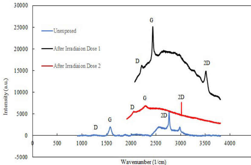
Figure 6. Raman spectra of CVD graphene grown on copper substrate, with and without irradiation doses for sample-1
