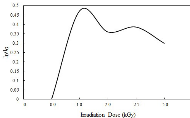
Figure 9. Evolution of I_D/I_G curve as a function of irradiation dose for graphene grown over nickel substrate
