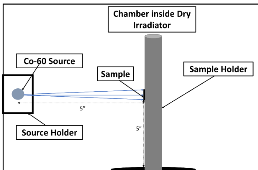
Figure 3. Gamma irradiation experimental setup using ^{60}\text{Co} source inside irradiator
