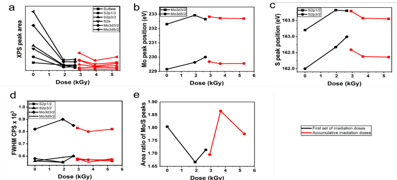
Figure 16. (a) XPS peak area as a function of irradiation dose after the first and second set of irradiation doses. (b) XPS peak position of Mo as a function of irradiation dose. (c) XPS peak position of S as a function of irradiation dose. (d) Full width at half maximum (FWHM) of XPS peaks as a function of irradiation dose. (e) Area ratio of Mo and S peaks as a function of irradiation dose
