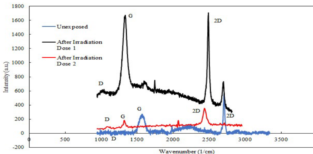
Figure 4. Raman spectra of CVD graphene grown on nickel substrate, with and without irradiation doses for sample-1
