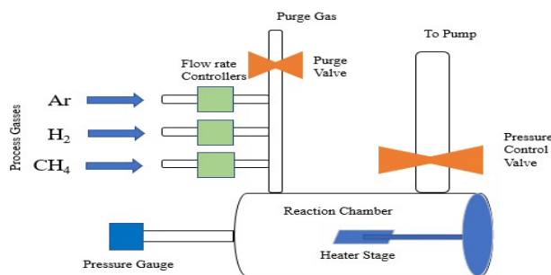
Figure 1. Schematic of gas flow in graphene nanoCVD reactor
