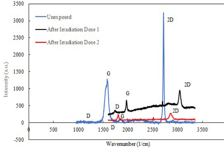
Figure 5. Raman spectra of CVD graphene grown on nickel substrate, with and without irradiation doses for sample-2
