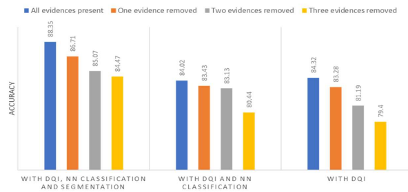
CASE STUDY FOR PREDICTING MOTION FACTOR: AVERAGE ACCURACY 5-FOLD CROSS VALIDATION
