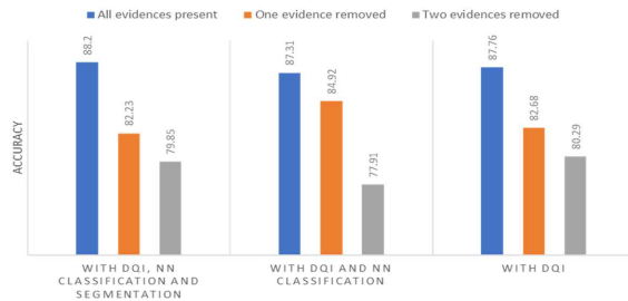
CASE STUDY FOR PREDICTING NOZZLE TIMINGS: AVERAGE ACCURACY 5-FOLD CROSS VALIDATION
