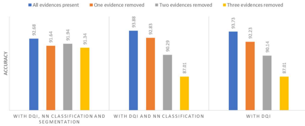
CASE STUDY FOR PREDICTING MOTION FACTOR: AVERAGE ACCURACY 5-FOLD CROSS VALIDATION
