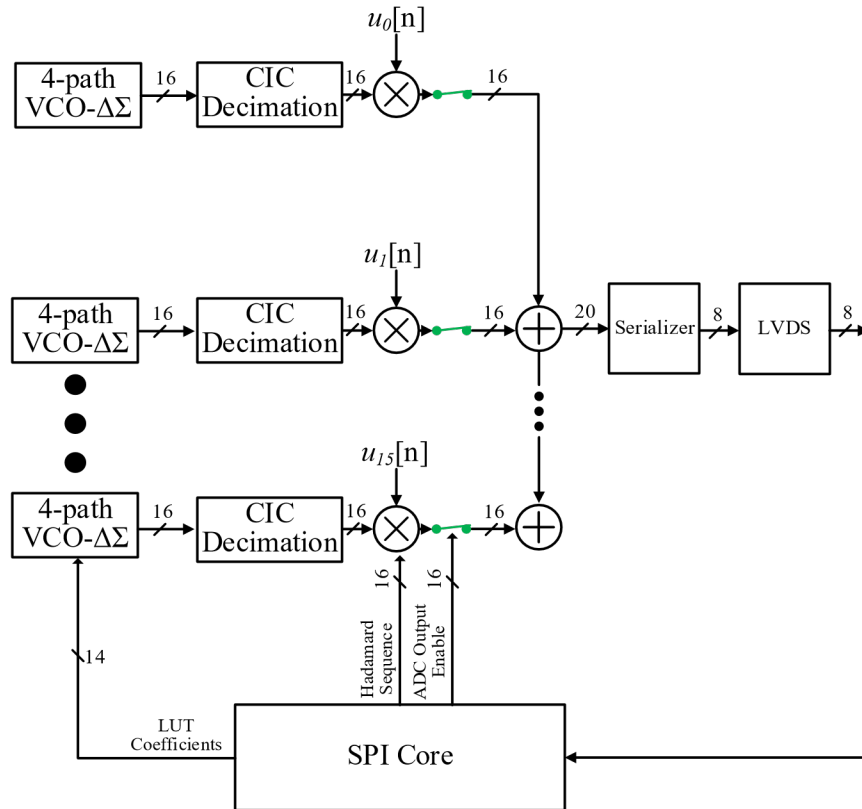
Fig. 7.24. Digital Logic Post-VCO-Based ADC
