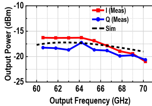
Fig. 5.6. Measured Output Power Curves
