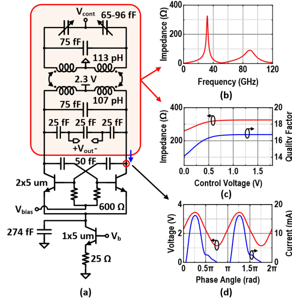
Fig. 6.10. (a) VCO schematic. Other Components of the 4-port Tank Model are not Shown for Brevity (b) Simulated Tank Impedance versus Frequency ( V_{\text{cont}} = 1 V). (c) Simulated |Z_{\text{tank}}| and Q Versus Control Voltage (d) Simulated single-ended Tank Voltage and Current Waveforms ( V_{\text{cont}} = 1 V)
