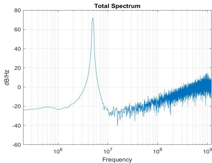
Fig. 7.31. Calibrated Single-Tone Output without Swapping
