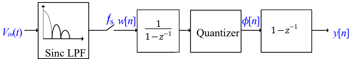
Fig. 7.3. VCO-Based ADC Equivalent Block Diagram
