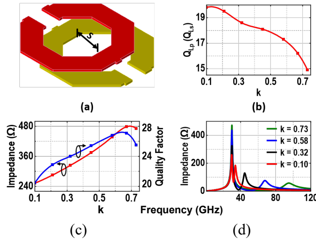
Fig. 6.5. (a) Layout of the transformer in Fig. 6.4(b) with coil separation S = 0\text{--}60\text{ }\mu\text{m} . (b) Simulated Q-factors of individual coils versus k . (c) |Z_{tank}| and Q versus k . (d) |Z_{tank}| versus frequency for different k
