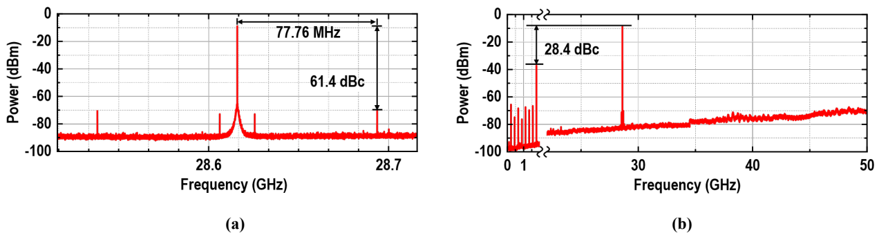
Fig. 6.19. Measured (a) Close-in and (b) Full-span Spectra of the PLL The -28.4 dBc spur near 2 GHz is due to coupling from the strong \div 16 output on the PCB
