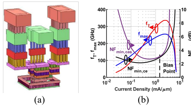
Fig. 3.2. (a) Physical Layout of a Transistor, (b) 4\mu\text{m} Transistor Performance Black, red, and blue curves show single transistor performance. Purple curve shows two cascode connector transistors performance. NFmin results are for 60 GHz operation.
