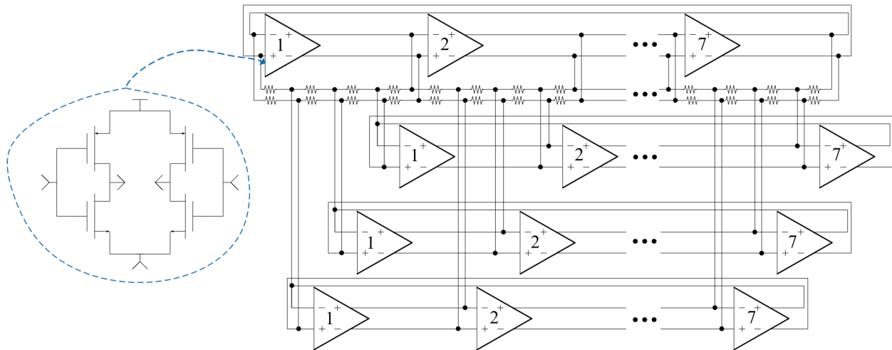
Fig. 7.9. 45-Degree Coupled, Differential ICRO
