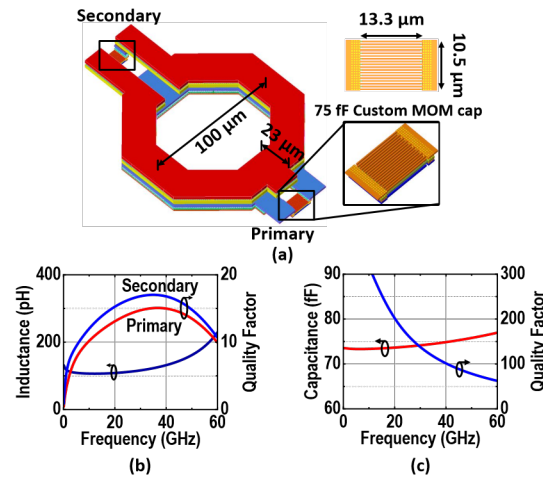
Fig. 6.11. (a) Transformer and MOM Capacitor Layout, (b) Simulated DM inductance and Q-factors of the Transformer Primary and Secondary Coils, (c) Simulated Capacitance and Q-factors of the 75-fF MOM Capacitors
